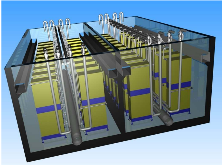
Figure 4.15 TMR140-200D module configuration (Toray Engineering Manuel, 2009)
