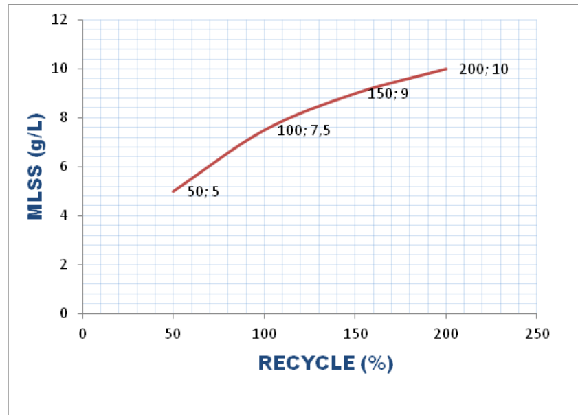
Figure 5.10 The relationship between recycle ratio and MLSS for the separated system
