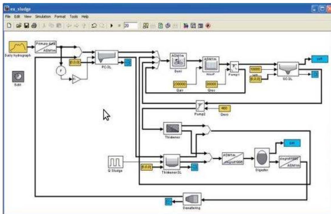
Figure 3.10 SIMBA model of wastewater treatment plant
