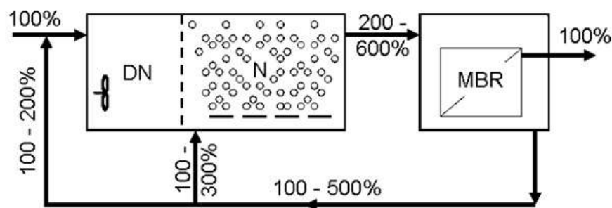
Figure 4.12 General recirculation scheme (Toray Engineering Manuel, 2009)
