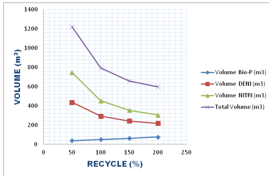
Figure 5.9 The relationship between recycle ratio and volume of bioreactor for the separated system
