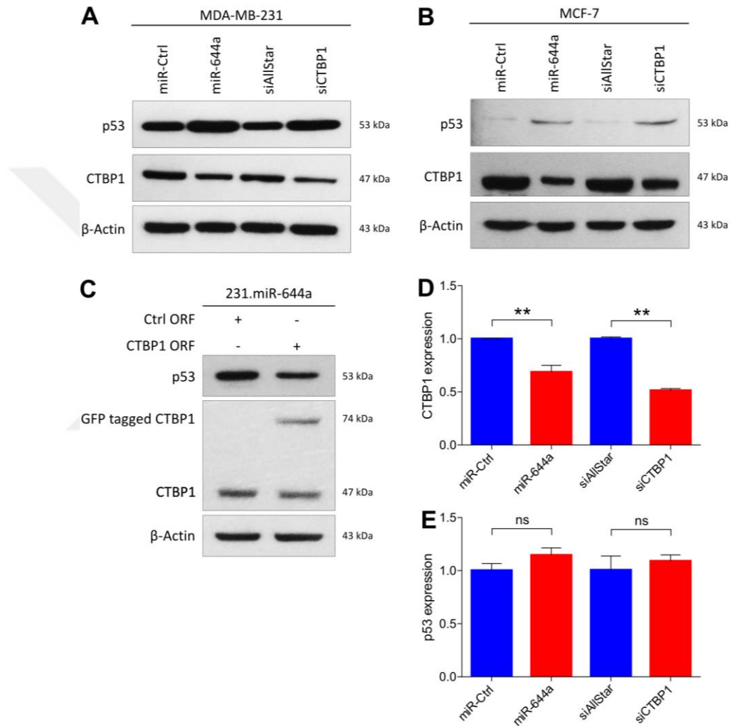
Figure 4.28. miR-644a regulates p53 at post-transcriptional level independent of its mutation status. (A and B) Western Blot analysis showing the regulation of p53 in MDA-MB-231 (A) and MCF-7 cells (B) upon miR-644a overexpression or CTBP1 knockdown. Actin was used as a loading control. (C) Western Blot analysis of p53 and CTBP1 levels in 231.miR-644a cells transfected with either Ctrl ORF or CTBP1 ORF showing downregulation of p53 with rescue of CTBP1 expression. Actin was used as a loading control. (D and E) qRT-PCR analysis of CTBP1 (D) and p53 (E) expression in MCF-7 cells upon miR-644a overexpression or CTBP1 knockdown with siCTBP1-Pool.
