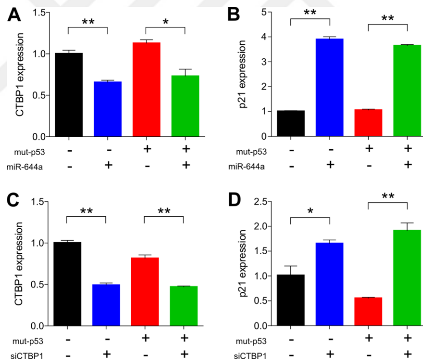
Figure 4.31. Ectopic p53 expression does not affect CTBP1. (A-D) qRT-PCR analysis of CTBP1 ( A and C ) and p21 ( B and D ) expression in p53-wt MCF-7 cells either upon miR-644a overexpression or after knockdown of CTBP1 in the absence or presence of mut -p53.
