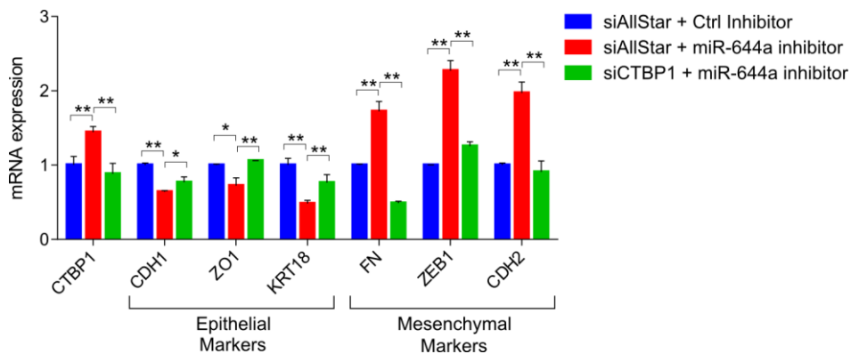
Figure 4.26. Loss of CTBP1 reverses miR-644a inhibition associated mesenchymal phenotype to epithelial like state. qRT-PCR analysis of epithelial and mesenchymal marker gene expression in MCF-12A cells upon CTBP1 rescue by miR-644a inhibitor and further knockdown by siCTBP1.
