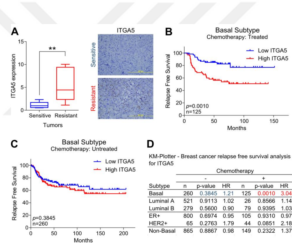
Figure 4.40. ITGA5 is upregulated in doxorubicin resistant tumors and is associated with worst RFS specifically in chemotherapy-treated TNBCs. (A) Expression of ITGA5 in doxorubicin sensitive and resistant tumors at mRNA (left), and protein levels (right). n = 4 . (B and C) Kaplan-Meier survival curves representing the percentage RFS in chemotherapy-treated basal patients ( n = 125 ) (B) and untreated basal patients ( n = 260 ) (C) based on low vs high ITGA5 expression. (D) Table summarizing ITGA5 expression-based Kaplan-Meier RFS analysis of patients representing different breast cancer subtypes either treated or not treated with chemotherapy.
