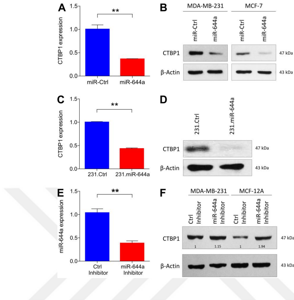
Figure 4.14. Modulating miR-644a expression alters CTBP1 expression inversely in vitro . (A and B) Confirmation of CTBP1 downregulation by miR-644a overexpression at transcript and protein levels with qRT-PCR analysis in MDA-MB-231 (A) and with Western Blot analysis in MDA-MB-231 (left) and MCF-7 (right) (B) cells transfected with either miR-Ctrl or miR-644a mimic. Actin was used as a loading control. (C and D) qRT-PCR (C) and Western Blot (D) analysis of CTBP1 expression in 231.Ctrl and 231.miR-644a cells. Actin was used as a loading control. (E) qRT-PCR analysis of miR-644a expression in MDA-MB-231 cells transfected with either a control Inhibitor (Ctrl Inhibitor) or miR-644a Inhibitor. (F) Western Blot analysis showing the levels of CTBP1 in MDA-MB-231 and MCF-12A cells transfected with either Ctrl Inhibitor or miR-644a Inhibitor. Actin was used as a loading control.
