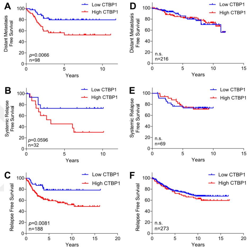
Figure 4.35. CTBP1 expression is associated with poor survival in p53-mut but not in p53-wt breast cancer patients. (A and B) Kaplan Meier survival curves of breast cancer patients with p53 mutation based on CTBP1 median expression levels in datasets GSE58644 ( n = 98 ) representing percentage DMFS (A) and in GSE19536 ( n = 32 ) representing percentage systemic RFS (B) . (C) Kaplan Meier survival curve of breast cancer patients with p53 mutation based on ‘best cut-off’ for CTBP1 expression levels in KM Plotter ( n = 188 ) representing percentage RFS. (D and E) Kaplan Meier survival curves of p53-wt breast cancer patients based on CTBP1 median expression from datasets in GSE58644 (D) and in GSE19536 (E) . (F) Kaplan Meier survival curve of p53-wt breast cancer patients based on best cut-off for CTBP1 expression levels in KM Plotter ( n = 273 ) representing percentage RFS.
