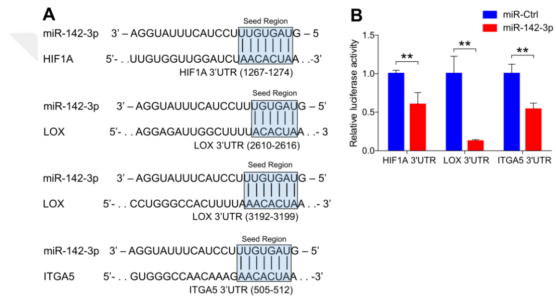
Figure 4.61. miR-142-3p directly targets HIF1A, LOX and ITGA5. (A) Graphical representation of miR-142-3p binding sites within the 3'-UTRs of HIF1A, LOX and ITGA5. (B) Luciferase activity of a reporter construct fused with 3'-UTRs of HIF1A, LOX or ITGA5 in 231.Luc.GFP cells transfected with miR-Ctrl or miR-142-3p.
