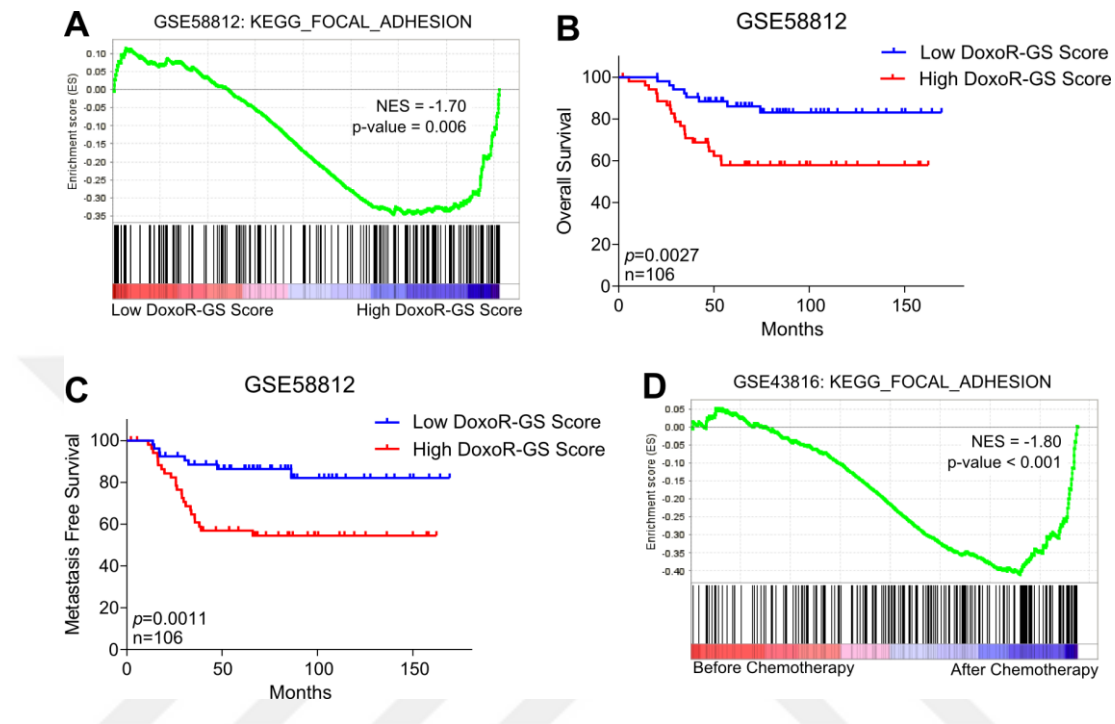
Figure 4.39. DoxoR-GS having enriched integrin/focal adhesion signaling predicts worst survival in chemotherapy-treated TNBC. (A) Enrichment plot of chemotherapy-treated TNBC tumors from GSE58812 ( n = 106 ) with low or high DoxoR-GS scores. Genes associated with focal adhesion signaling are enriched in tumors with high DoxoR-GS scores. (B and C) Kaplan-Meier survival curve representing the percentage OS (B) and MFS (C) in chemotherapy-treated TNBC patients from GSE58812 ( n = 106 ) based on low vs high DoxoR-GS scores. (D) Enrichment plot of TNBC patients from GSE43816 showing that genes associated with focal adhesion signaling get enriched after chemotherapy treatment.
