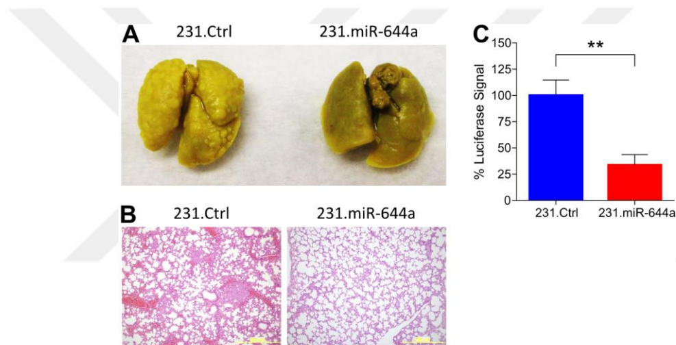
Figure 4.9. miR-644a inhibits metastasis in vivo . (A) Representative images of lungs collected from nude mice injected intravenously with 231.Ctrl or 231.miR-644a cells. Mice were sacrificed at week 7 and lungs were fixed in Bouin's Solution. (B) Representative Hematoxylin and Eosin staining of metastatic nodules in lungs from (A). (C) Luciferase signal coming from metastatic nodules in lungs of (A) as quantified by a luciferase assay. n = 4 .
