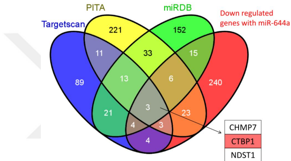
Figure 4.12. Venn diagram for the combinatorial target prediction analysis of miR-644a.
