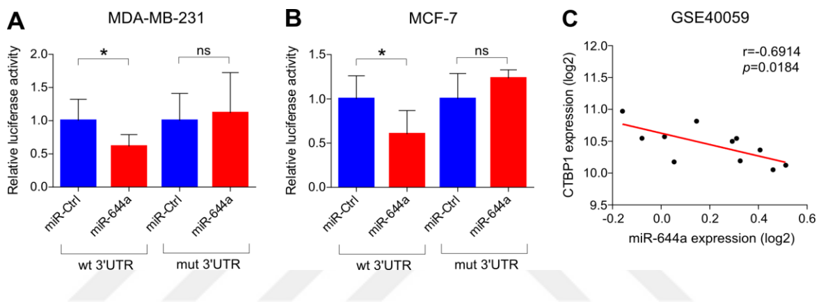
Figure 4.15. miR-644a directly targets CTBP1 and inversely correlates with CTBP1 expression in breast cancer cell lines. (A and B) Luciferase activity of a reporter construct fused with either a wt or mut CTBP1 3'-UTR co-transfected with miR-Ctrl or miR-644a mimic in MDA-MB-231 (A) and MCF-7 (B) cells. n = 5 . (C) Expression of miR-644a negatively correlates with CTBP1 mRNA expression in 9 breast cancer cell lines and 2 normal breast cell line from GSE40059.
