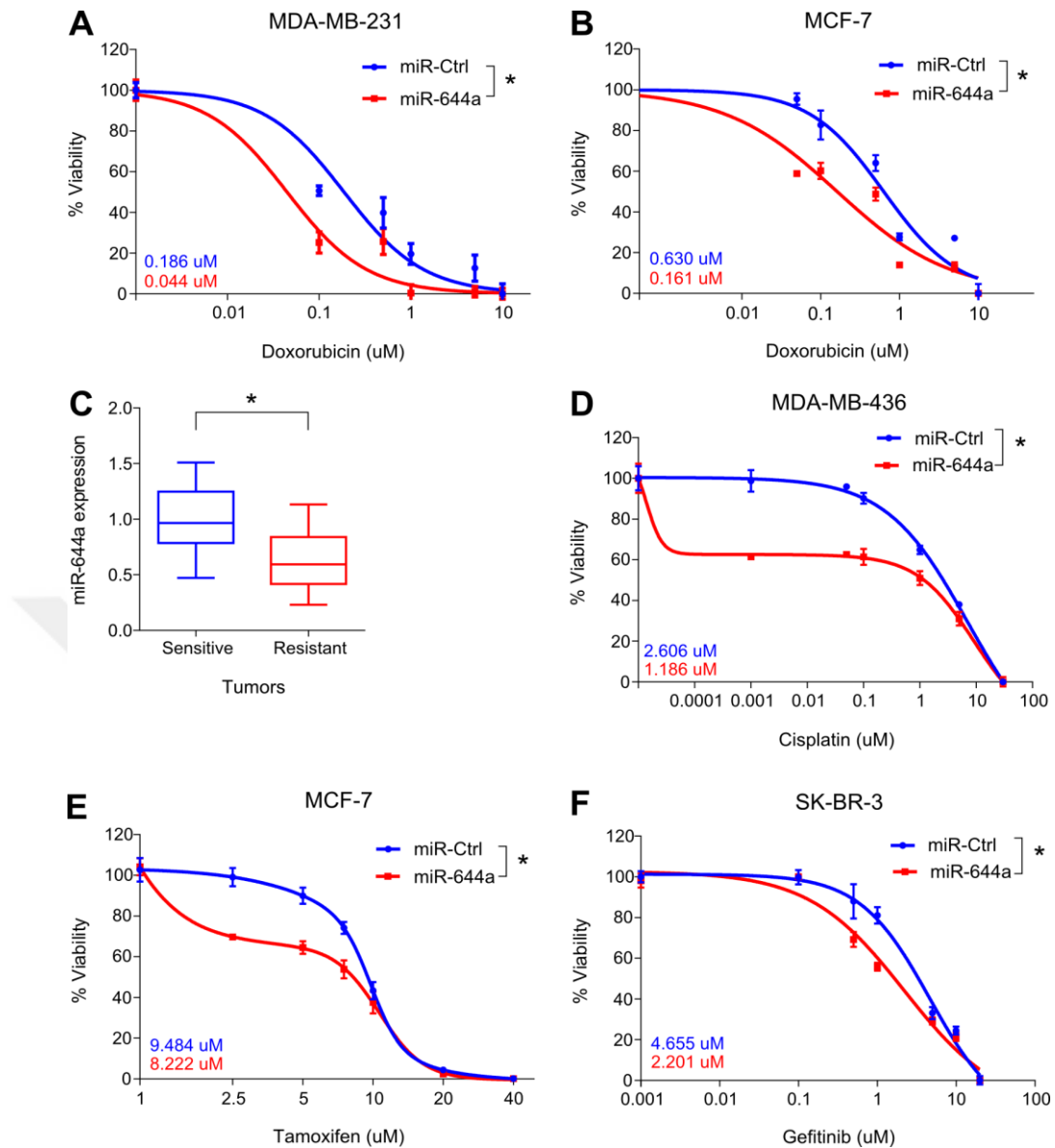
Figure 4.11. miR-644a overexpression acts as a therapy sensitizer in breast cancer cells and its expression correlates with doxorubicin resistance in vivo . (A and B) Effect of miR-644a overexpression on the response of MDA-MB-231 (A) and MCF-7 (B) cells to doxorubicin. n = 4 . (C) qRT-PCR analysis of miR-644a expression in sensitive or resistant xenografts selected based on changes in tumor volumes upon successive doxorubicin treatments. n = 5 . (D- F) Effect of miR-644a overexpression on the response of MDA-MB-436 cells to cisplatin (D), MCF-7 cells to tamoxifen (E), and SKBR-3 cells to gefitinib (F). n = 4 . IC50 values for each condition are given on the left bottom corners of each curve with a color code.
