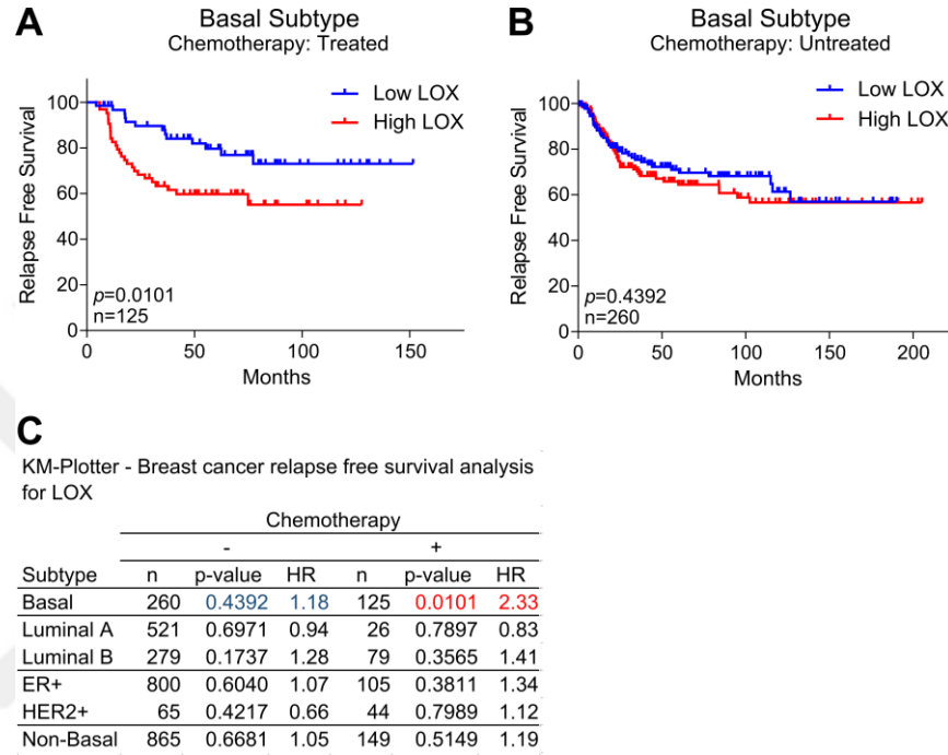
Figure 4.47. LOX is associated with poor RFS in chemotherapy-treated TNBC patients. (A and B) Kaplan-Meier survival curve representing the percentage RFS in chemotherapy-treated ( n = 125 ) (A) and untreated basal patients ( n = 260 ) (B) based on LOX expression. (C) Table summarizing LOX expression based Kaplan-Meier RFS analysis results of patients representing different breast cancer subtypes either treated or not treated with chemotherapy.
