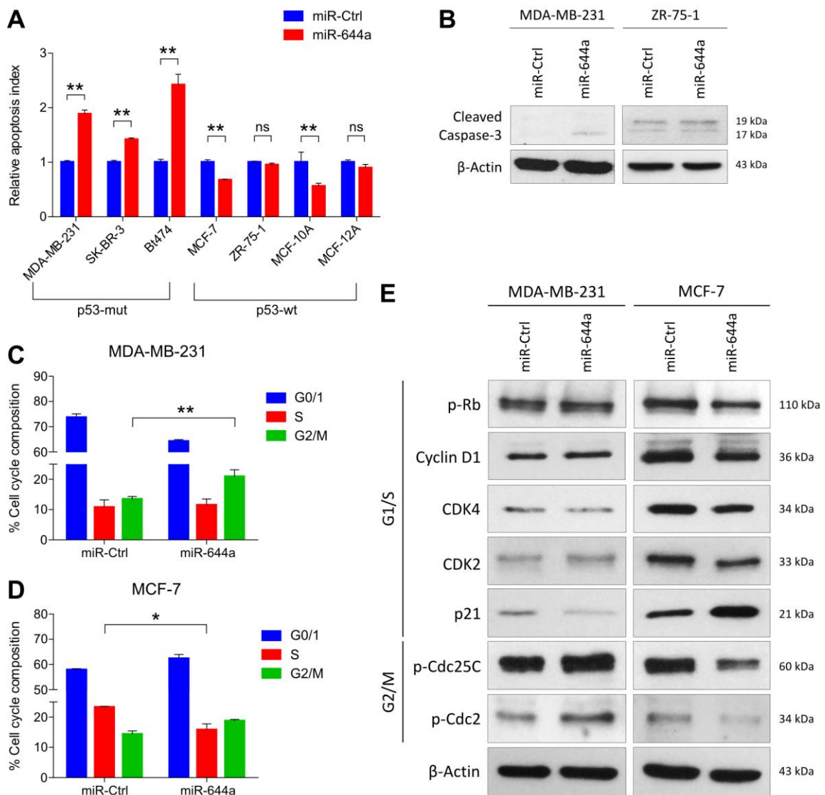
Figure 4.2. miR-644a promotes apoptosis in p53-mut but G1 cell cycle arrest in p53-wt breast cancer cells in vitro . (A) Changes in the apoptosis index based on Caspase-3/7 cleavage in 5 breast cancer and 2 normal breast cell line transfected with either miR-Ctrl or miR-644a mimic. n = 4. (B) Western Blot analysis showing the levels of cleaved Caspase-3 in p53-mut
