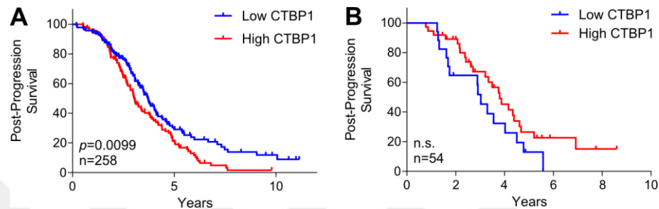
Figure 4.36. CTBP1 expression is associated with poor post-progression survival in p53- mut but not in p53- wt ovarian cancer patients. (A) Kaplan Meier survival curve of ovarian cancer patients with p53 mutation based on ‘best cut-off’ for CTBP1 expression levels in KM Plotter ( n = 258 ) representing percentage post-progression survival. (B) Kaplan Meier survival curve of p53- wt ovarian cancer patients based on best cut-off for CTBP1 expression levels in KM Plotter ( n = 54 ) representing percentage post-progression survival.
