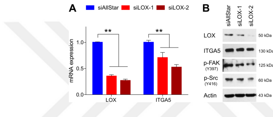
Figure 4.49. LOX hyperactivates integrin signaling by regulating ITGA5. (A) qRT-PCR analysis showing changes in the mRNA expression of LOX and ITGA5 48 hours after transfection with siAllStar or siLOX. (B) Western Blot analysis showing changes in LOX, ITGA5, p-FAK (Y397) and p-Src (Y416) 48 hours after transfection with siAllStar or siLOX. Actin was used as a loading control.
