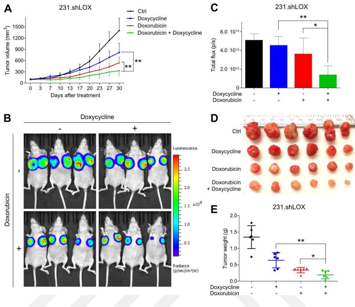
Figure 4.52. Knocking down LOX increases tumor suppressive effects of doxorubicin in TNBCs in vivo . A) Tumor volume changes upon shLOX induction and doxorubicin treatment alone or in combination as compared to control in nude mice ( n = 6 ). B) IVIS images of mice from (A) . C) Bar graph showing changes in luciferase intensity from tumors in (B) . D) Images showing isolated tumors from (B) . E) Dot plot showing changes in tumor weights from (D) .
