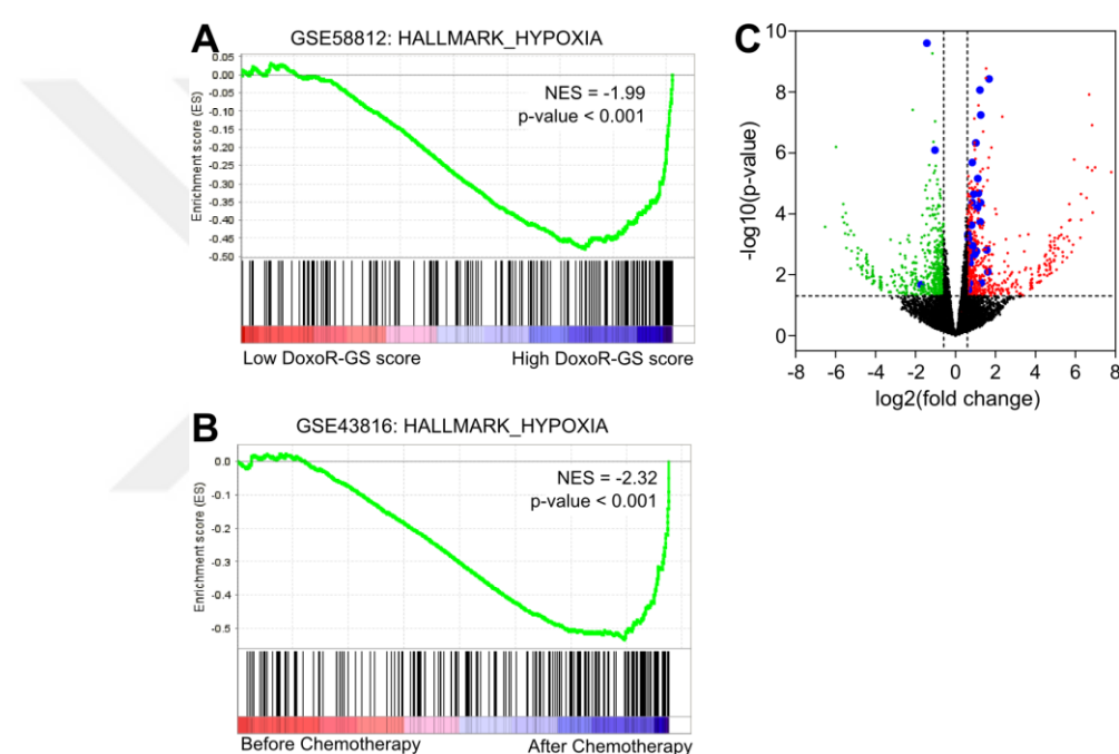
Figure 4.43. Hypoxia signaling is associated with chemotherapy resistance and HIF1A signaling is predicted to be activated in doxorubicin resistant xenografts. (A) Enrichment plot of chemotherapy-treated TNBC patients from GSE58812 (n = 106) with low or high DoxoR-GS scores. Genes upregulated upon low levels of oxygen are enriched in patients with high DoxoR-GS score. (B) Enrichment plot of TNBC patients from GSE43816 showing that genes upregulated upon low levels of oxygen get enriched after chemotherapy treatment. (C) Volcano plot showing significantly downregulated genes (green), upregulated genes (red) and the genes in IPA-based HIF1A gene signature (blue) in doxorubicin resistant versus sensitive tumors.
