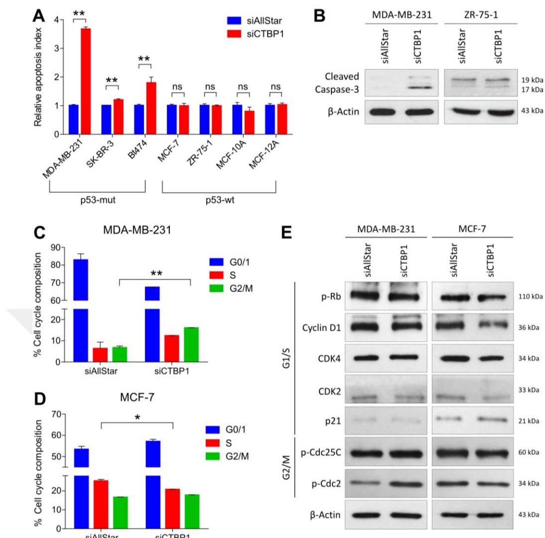
Figure 4.17. CTBP1 knockdown promotes apoptosis in p53- mut but G1 cell cycle arrest in p53- wt breast cancer cells in vitro . (A) Changes in the apoptotic index based on Caspase-3/7 cleavage in 5 breast cancer cell lines and 2 normal breast cell line transfected with siAllStar or siCTBP1-Pool. n = 4. (B) Western Blot analysis showing the levels of cleaved Caspase-3 in p53- mut MDA-MB-231 (left) and p53- wt MCF-7 cells (right) 72 hours after transfection with siAllStar or siCTBP1-Pool. Actin was used as a loading control. (C and D) Flow cytometric analysis of cell cycle in cells transfected with siAllStar or siCTBP1-Pool showing G2/M arrest in siCTBP1-Pool transfected MDA-MB-231 cells (C) and G1 arrest in siCTBP1-Pool transfected MCF-7 cells (D). (E) Western Blot analysis showing the levels of cell cycle proteins related to G2/M (p-Cdc25C and p-Cdc2) and G1/S (pRb, Cyclin D1, CDK4, CDK2 and p21) transition in p53- mut MDA-MB-231 and p53- wt MCF7 cells after 48 hours transfection with siAllStar or siCTBP1-Pool. Actin was used as a loading control.
