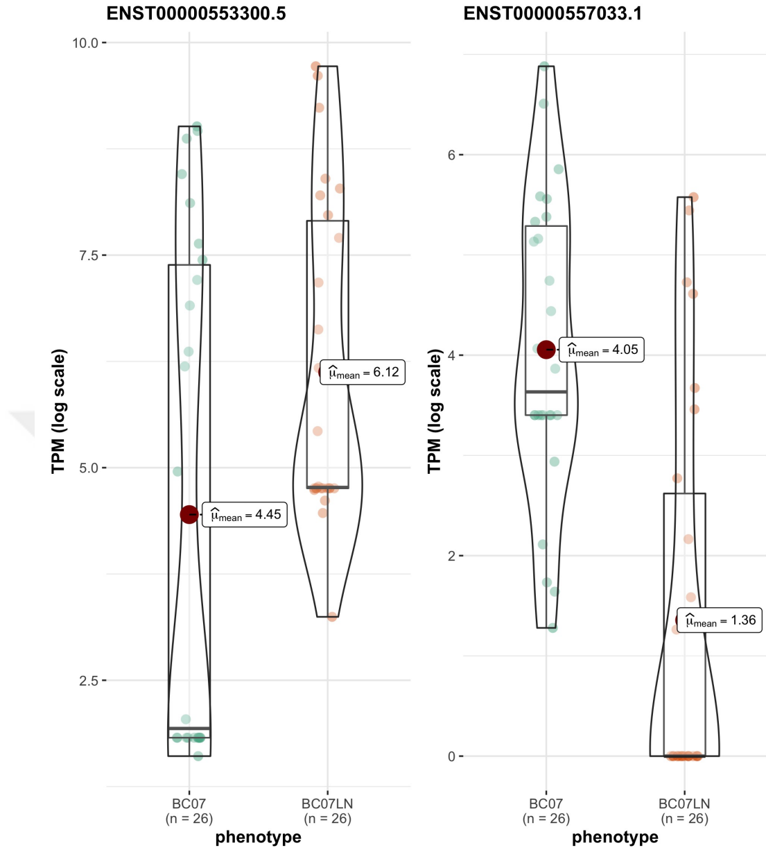
Figure 4.10: Violin plot for isoform switching case HNRNPC(ENSG00000092199) between protein coding ENST00000553300(3'UTR) and protein coding ENST00000557033(5'UTR)
