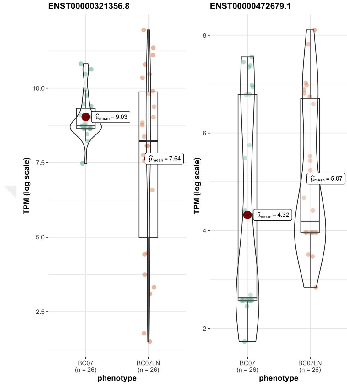
Figure 4.2: Violin plot for isoform switching case CLK1(ENSG00000013441) between protein coding ENST00000321356(Exonic) and retained intron ENST00000472679(3'UTR)
