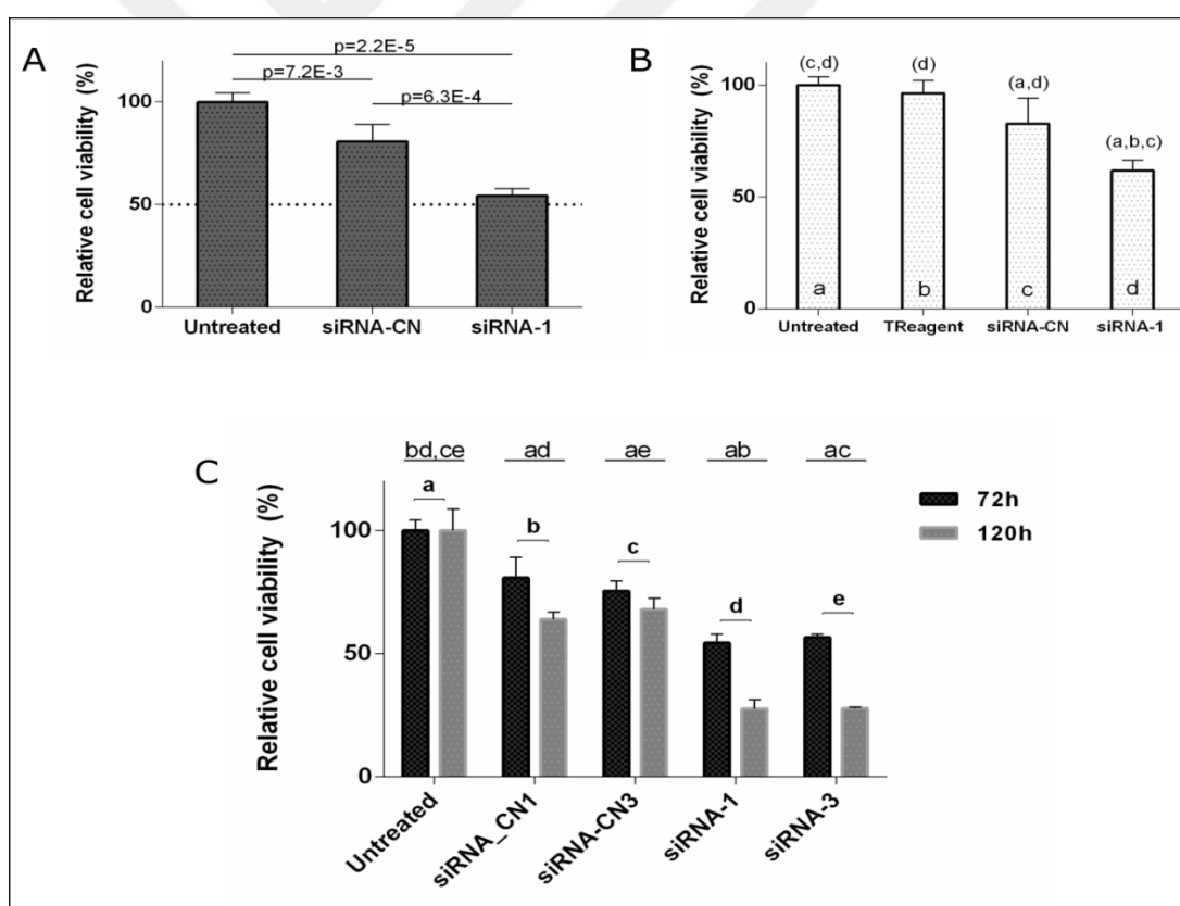
Figure 3.10: Effects of CHRNA5 depletion on MCF7 cell viability.
