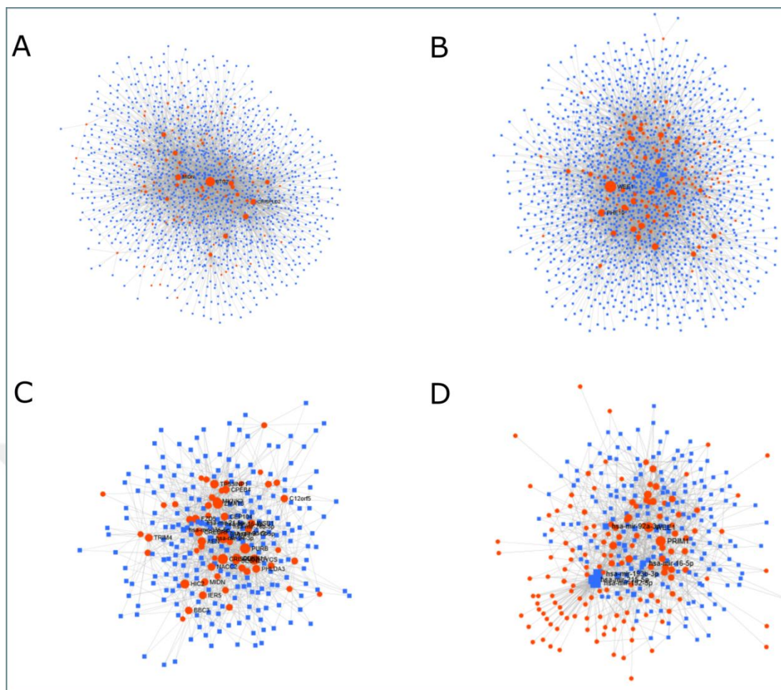
Figure 3.23: Common signatures between topoisomerase inhibitors and siRNA-1 treatment.
