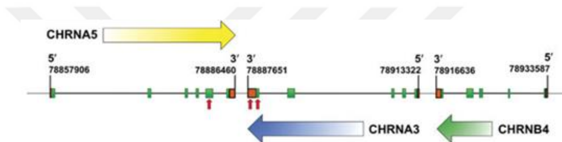
Figure 1.5: \alpha 3/\alpha 5/\beta 4 gene cluster.
