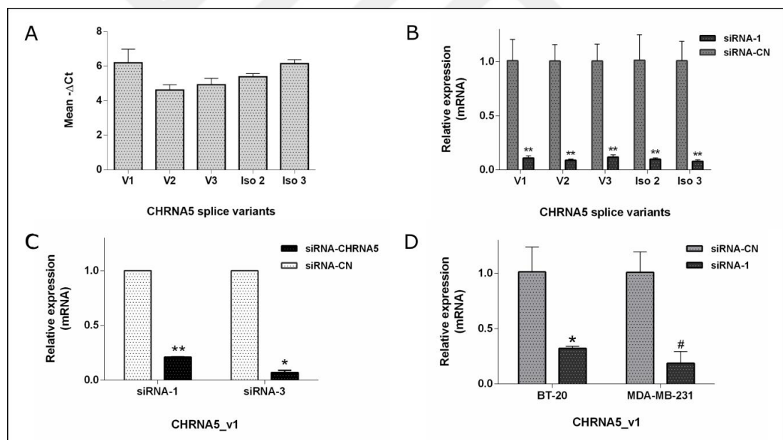
Figure 3.5: CHRNA5 isoform expression and downregulation using RNAi.
