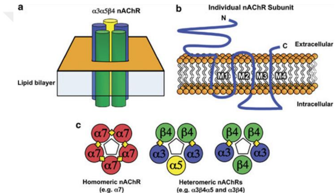
Figure 1.4: Structure of nAChRs.
