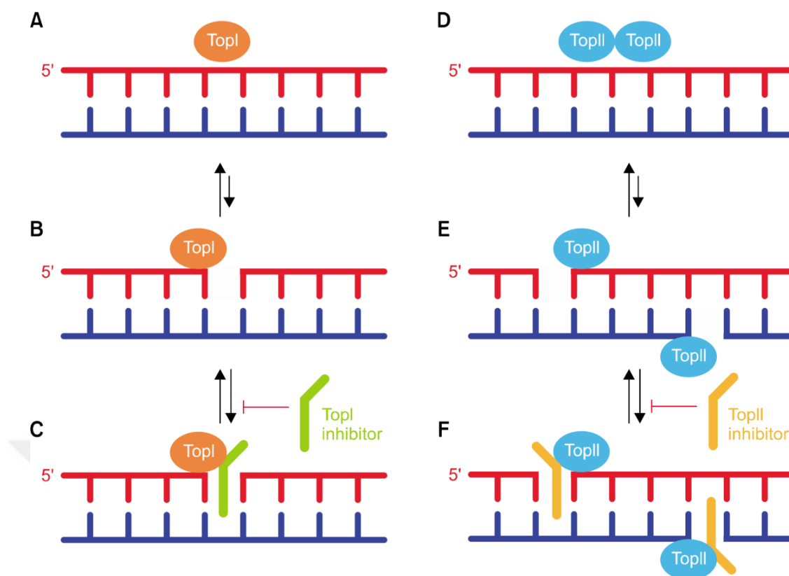
Figure 1.1: Activity of topoisomerase enzymes and their inhibitors.
