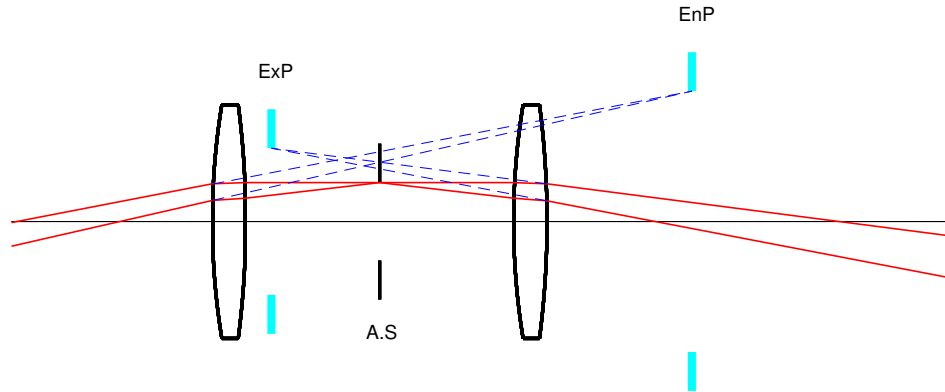
Figure 2.6 Aperture stop, entrance pupil and exit pupil for a two-lens system.
