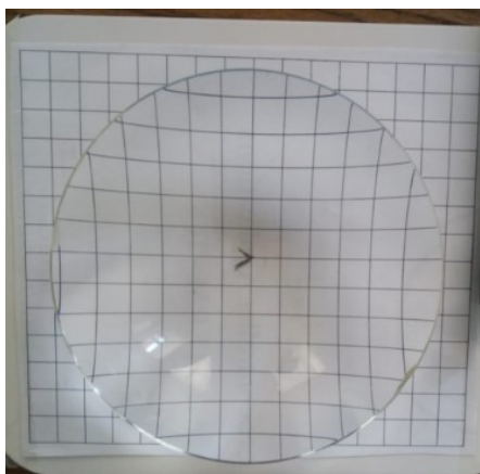
Figure 2.19 Pincushion distortion aberration
