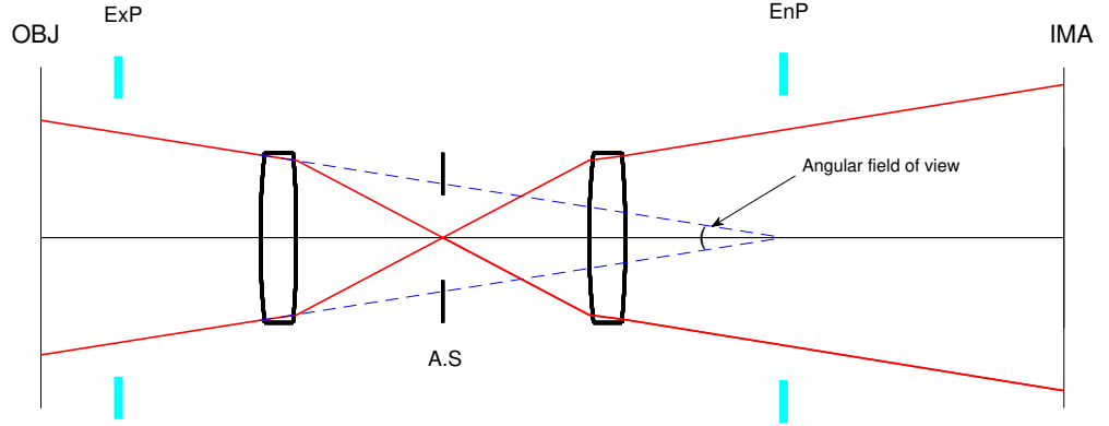
Figure 2.9 Angular field of view of the system
