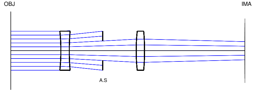
Figure 2.5 As bundle of rays propagates lens system from object plane to image plane, the aperture stop truncates the bundle of the rays at the upper and lower rim.
