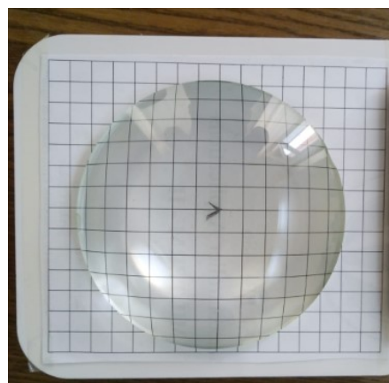
Figure 2.20 Barrel distortion aberration
