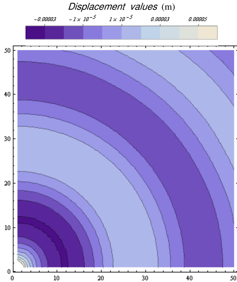
Figure 5. Real Part of Domain Response to the Unit Sinusoidal Stimulation on the Coordinate Center, G_{\text{Foundation}}=8.686\text{GPa} and G_{\text{Soil}}=24\text{MPa}
