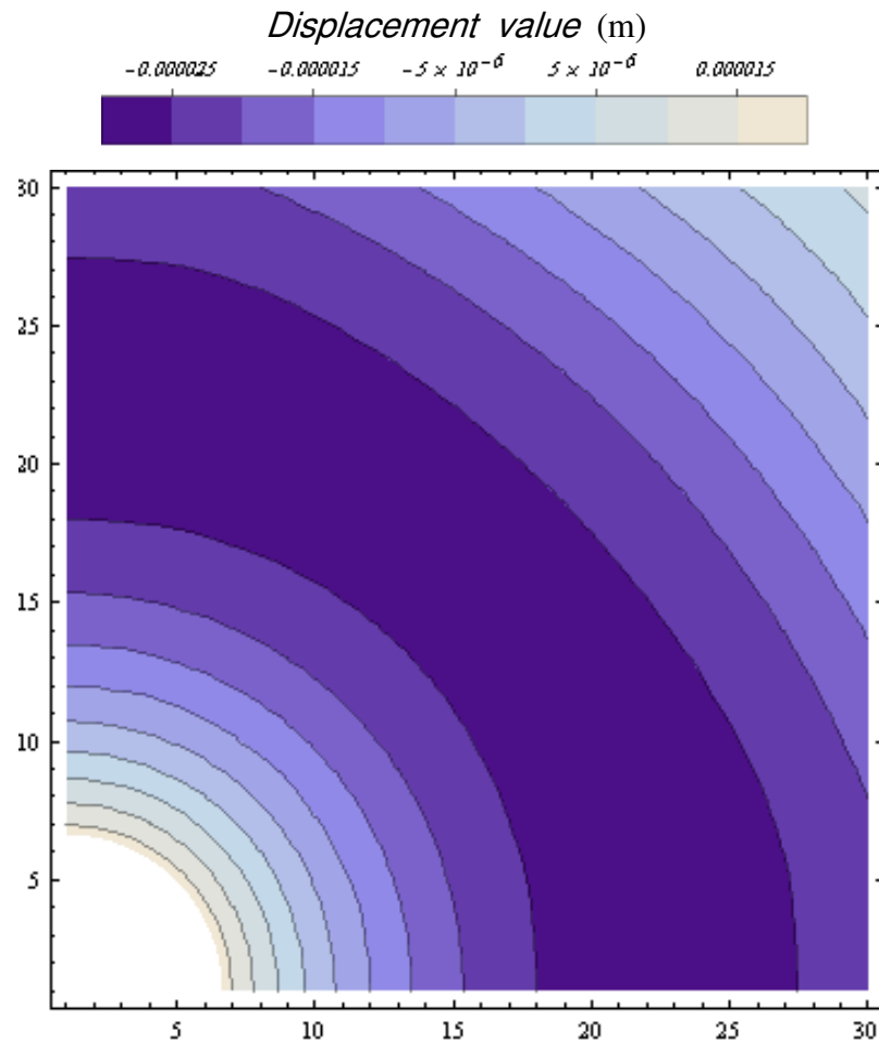
Figure 14. Real Part of Domain Response to the Unit Sinusoidal Stimulation on the Coordinate Center, G_{\text{Foundation}}=8.686\text{GPa} and G_{\text{Soil}}=96\text{MPa}
