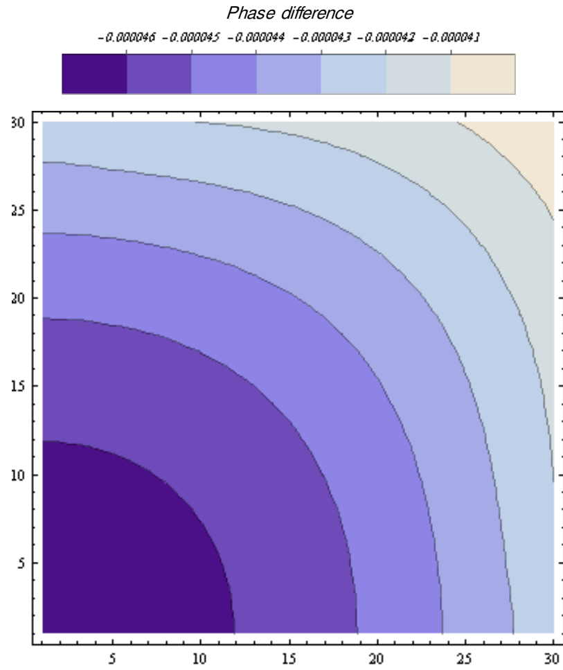
Figure 19. Imaginary Part of Domain Response to the Unit Sinusoidal Stimulation on the Coordinate Center- G_{\text{Foundation}}=8.686\text{GPa} and G_{\text{Soil}}=1.9\text{GPa}
