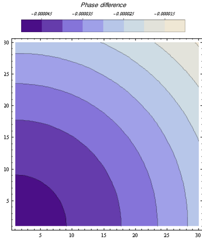
Figure 17. Imaginary Part of Domain Response to the Unit Sinusoidal Stimulation on the Coordinate Center, G_{\text{Foundation}}=8.686\text{GPa} and G_{\text{Soil}}=480\text{MPa}
