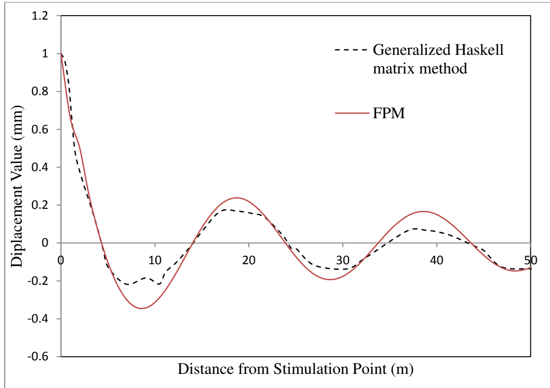
Figure 21. Real Part of a Domain Response to the Sinusoidal Dirac-Delta Dirichlet Motivation, Shear modulus of the Soil 10 MPa
