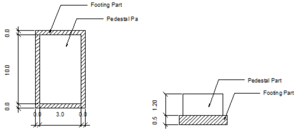
(a) Plan of the Foundation (b) Section of the Foundation Figure 24. Sketch of Plan and Section of the Foundation Designed for Air Blower [97]
