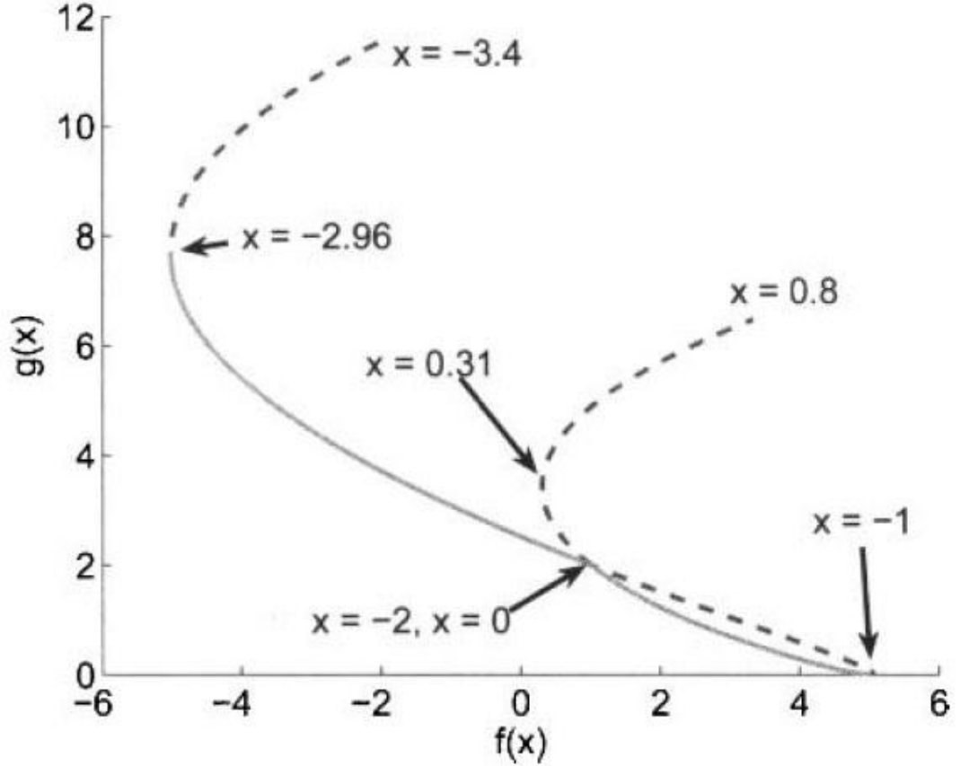
Figure 3.5 The plot of g(x) as the function of f(x) as x varies from -3.4 to 0.8 . The solid line is the Pareto front. (Simon, 2013)
