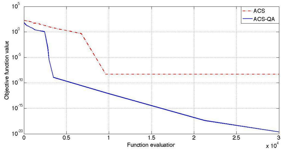
Figure 5.3 Convergence rates of the original ACS and the proposed ACS-QA algorithms for the Sphere function
