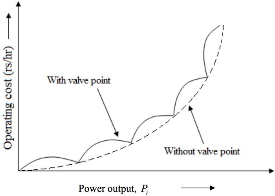
Figure 2.3 Operating cost curve with valve-point effects (Kaur, 2011)
