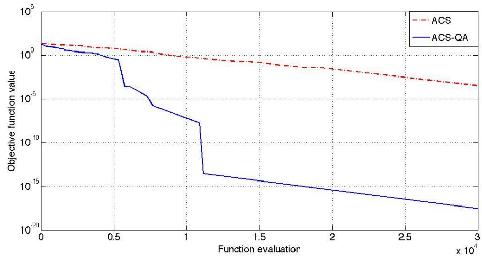
Figure 5.2 Convergence rates of the original ACS and the proposed ACS-QA algorithms for the Ackley function
