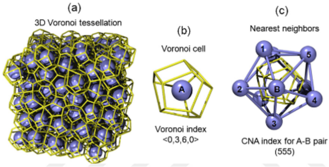
Figure 1.11: a) Voronoi tessellation, b) voronoi cell and c) the nearest neighbors [16].
