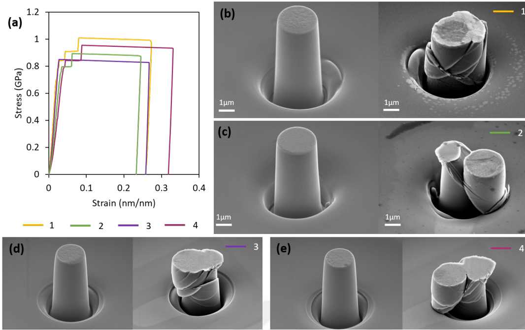
Figure 3.2: Al 90 Tb 10 fully amorphous (a) Stress strain diagram of 4 samples, (b), (c), (d) and (e) SEM images of micro pillars and fracture surfaces.
