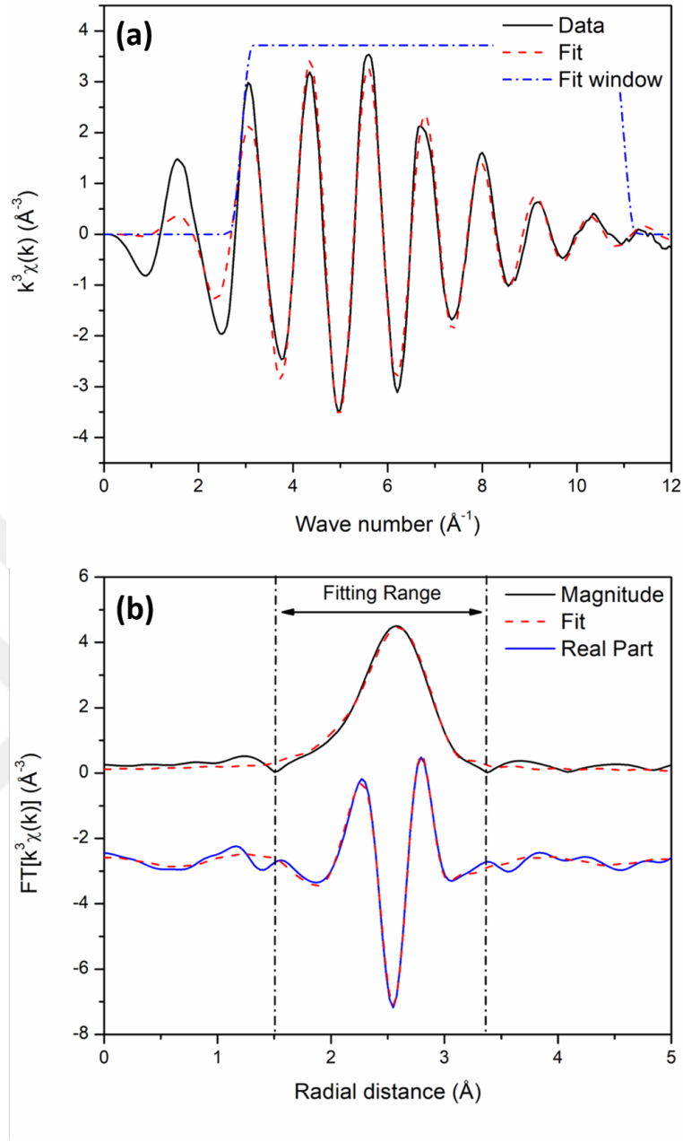
Figure 2.5: (a) Tb L 3 edge EXAFS data of Al 90 Tb 10 melt-spun ribbon, inversed Fourier transformed in k-space and (b) Fourier transformed in r-space.
