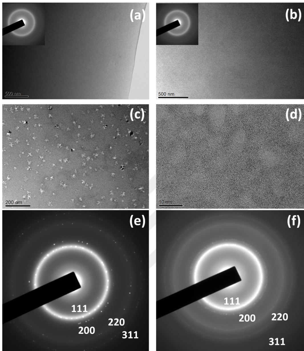
Figure 2.7: (a, b) Bright-field images and corresponding SAD patterns (in-sets), (c, d) bright-field images and (e, f) SAD after initial crystallization of as-quenched ribbon and thin-film Al 90 Tb 10 , respectively. SAD indexing represents fcc-Al reflections.
