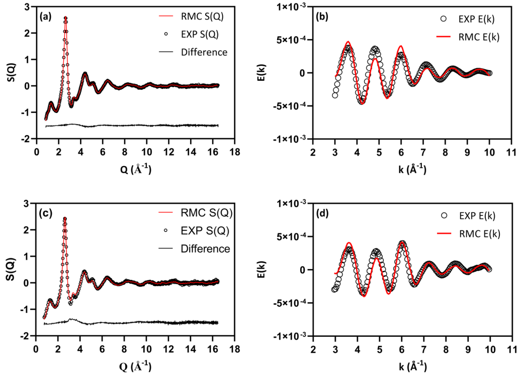
Figure 2.2: (a), (c) Total X-ray structure factors and (b), (d) EXAFS experimental data with their corresponding RMC fits for melt-spun ribbon and magnetron sputtered film, respectively.
