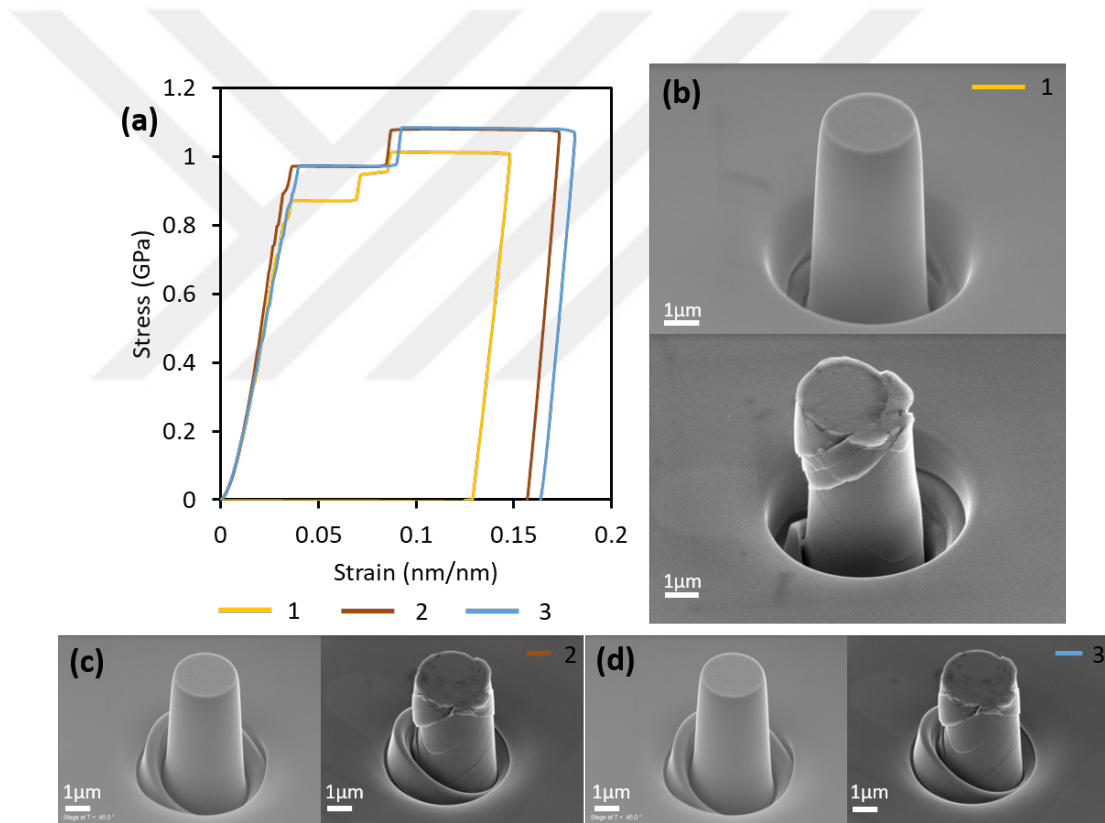
Figure 3.3: \text{Al}_{90}\text{Tb}_{10} 241 °C heat treated (a) Stress strain diagram of 3 samples, (b), (c) and (d) SEM images of micro pillars and fracture surfaces.
