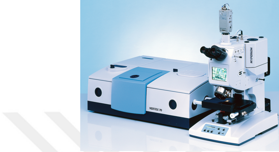
Figure 3.5: Bruker - Vertex 70v and Hyperion microscope
