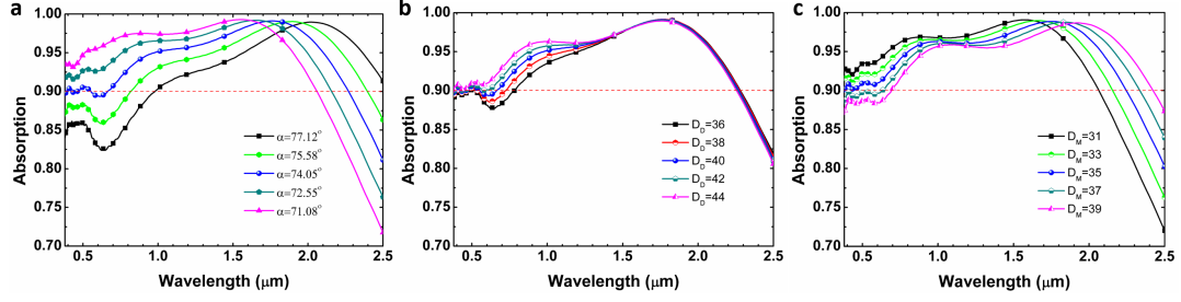
Figure 4.8: Optimization process of TiC. (a) The impact of \alpha when other parameters are D_M = 35nm , D_D = 40nm . (b) The impact of the thickness of the dielectric layer when other parameters are D_M = 35nm , \alpha = 74.05^\circ . (c) The impact of the thickness of TiC layer when other parameters are D_D = 44nm , \alpha = 74.05^\circ .
