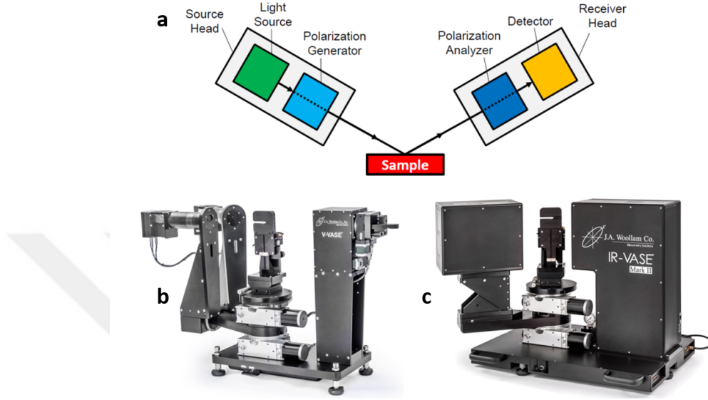
Figure 3.6: (a) General scheme of an ellipsometer. (b) V-VASE and (c) IR-VASE model of J.A. Woollam Co. Inc.
