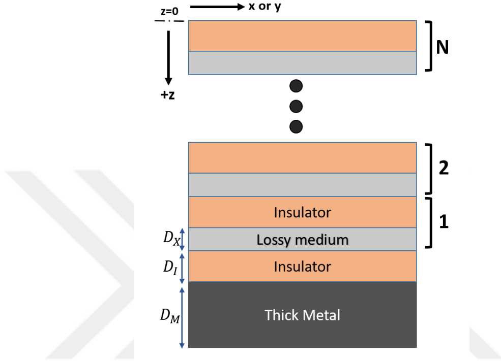
Figure 2.1: Generalized representation of the MI(MI) N design
