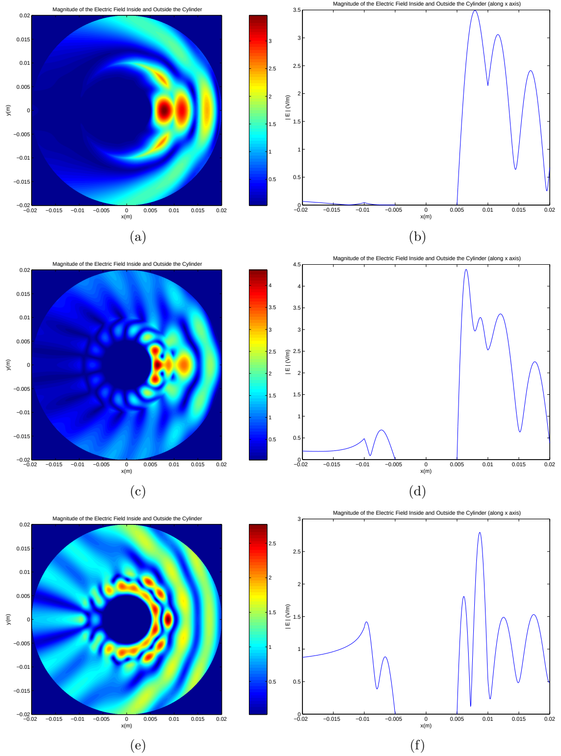
Figure 2.10: Magnitude of the electric field inside and outside the cylinder. (a)-(b) \varepsilon_r = -1 , \mu_r = -1 , (c)-(d) \varepsilon_r = -2 , \mu_r = -2 , (e)-(f) \varepsilon_r = 2 , \mu_r = 2
