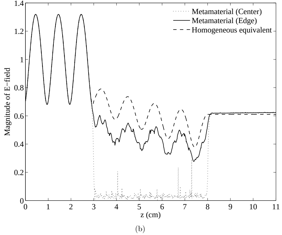
Figure 4.11: Magnitudes of E-field inside and outside the metamaterial medium and its homogeneous equivalent at (a) f = 10.8 GHz, (b) f = 15.0 GHz.
