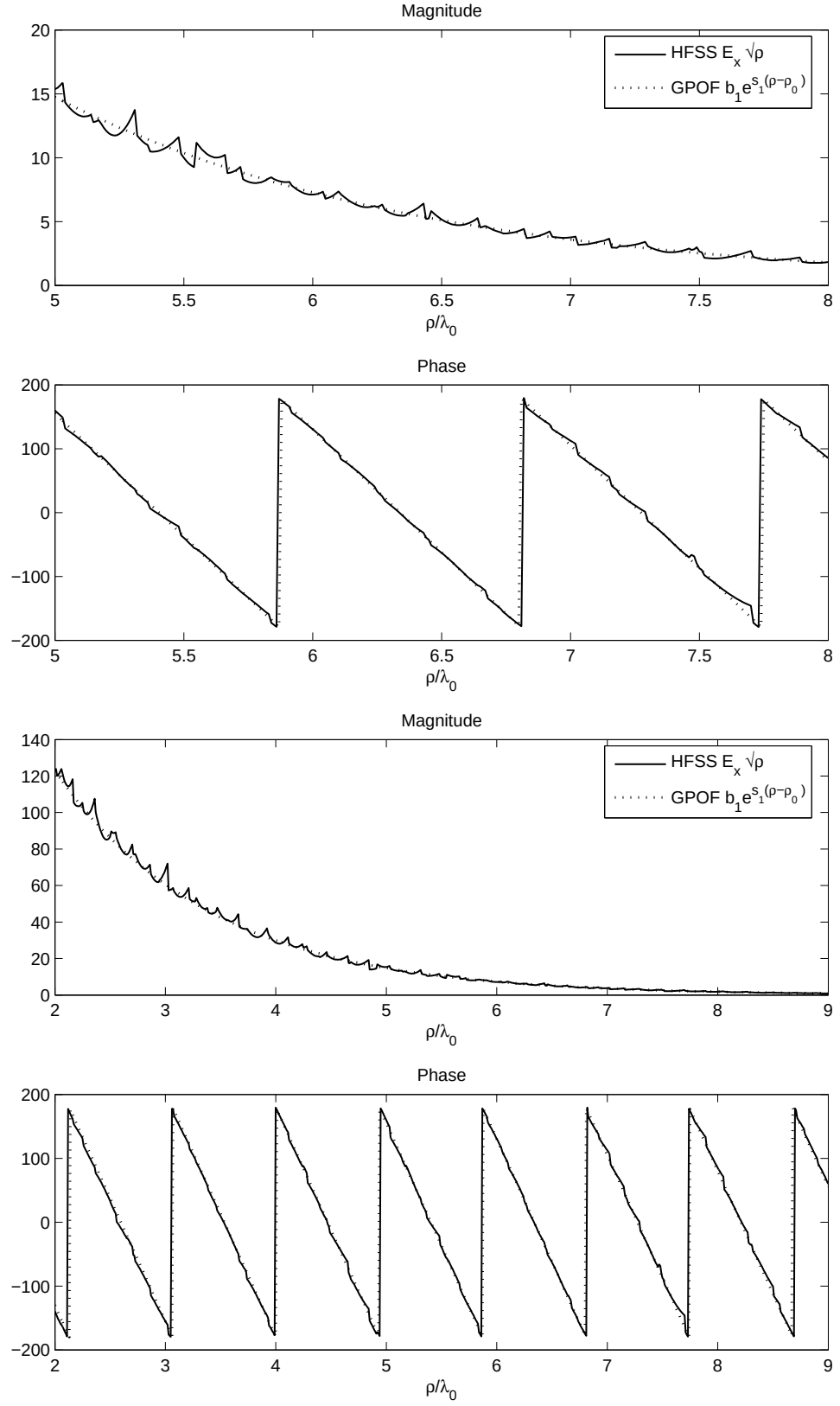
Figure 4.20: Comparison of GPOF approximation with HFSS data and its Extrapolation . ( f = 30\text{GHz} , \lambda_0 = 1\text{cm} , th = 0.1\lambda_0 , \varepsilon_r = 2.55 , \rho_{start} = 5\lambda_0 , \rho_{end} = 8\lambda_0 , N = 101 )
