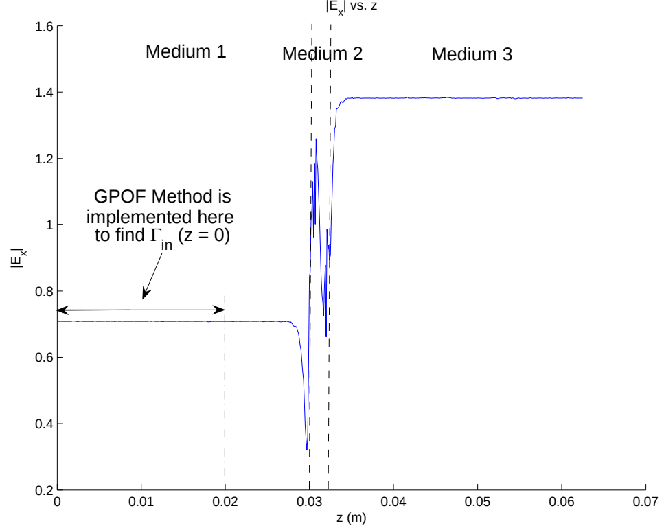
Figure 4.6: |E_x| vs. z ( f = 10GHz , N_z = 1 ).
