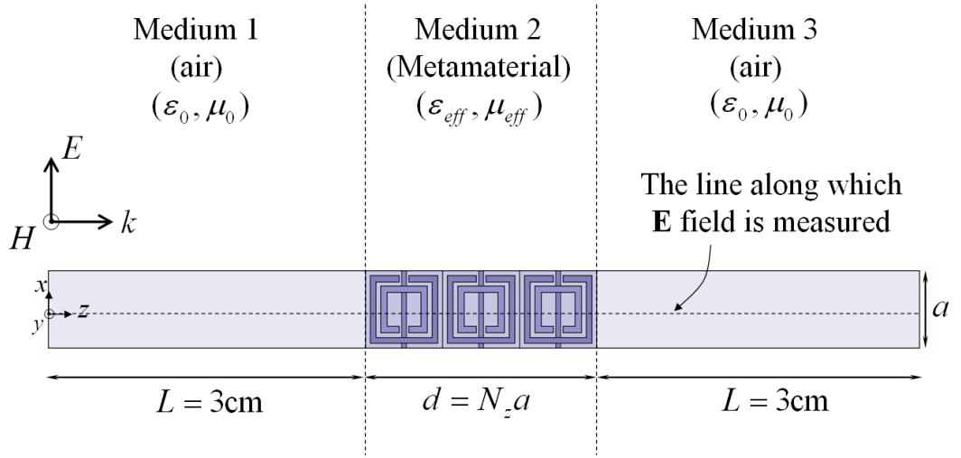
Figure 4.5: Problem geometry (cross-section view, for N_z = 3 ).
