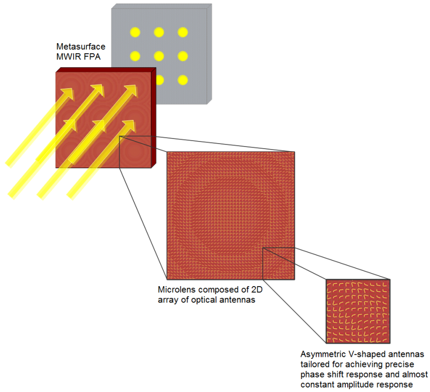
Figure 4.1: Schematic representing the geometry of the proposed metasurface-based microlensed focal plane array (FPA) design. [Reprinted/Adapted] with permission from ref [101], [Optical Society of America]
