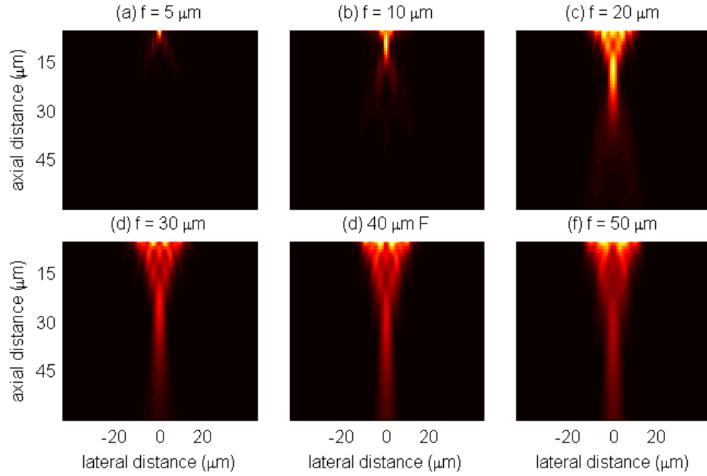
Figure 4.6: Intensity distributions of the cross-polarized field obtained by illuminating the central unit cell of the proposed metasurface-based FPAs. [Reprinted/Adapted] with permission from ref [101], [Optical Society of America]
