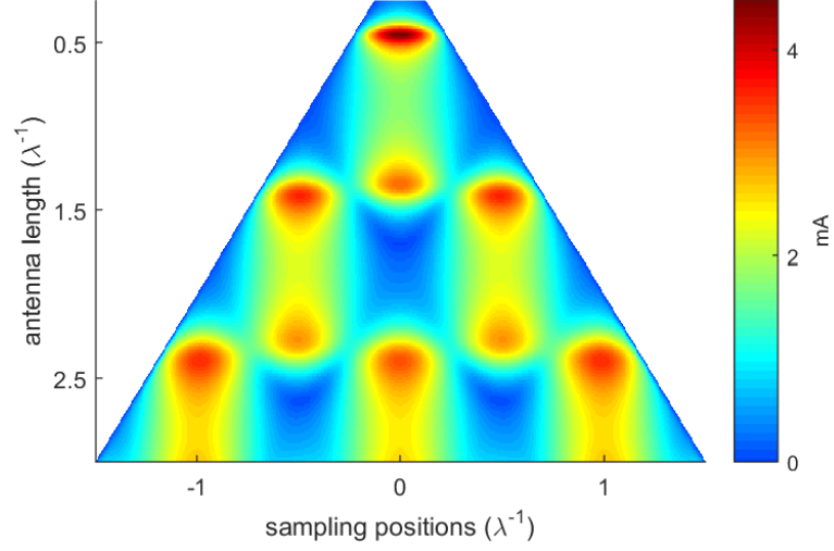
Figure 2.8: Amplitude of the current distributions on rod antennas.
