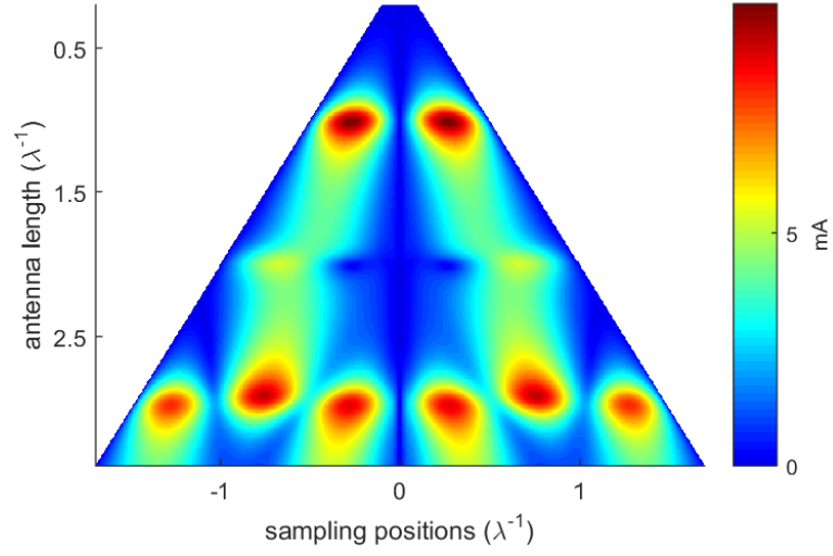
Figure 2.23: Amplitudes of the current distributions on V-shaped nanoantennas with symmetric excitation.
