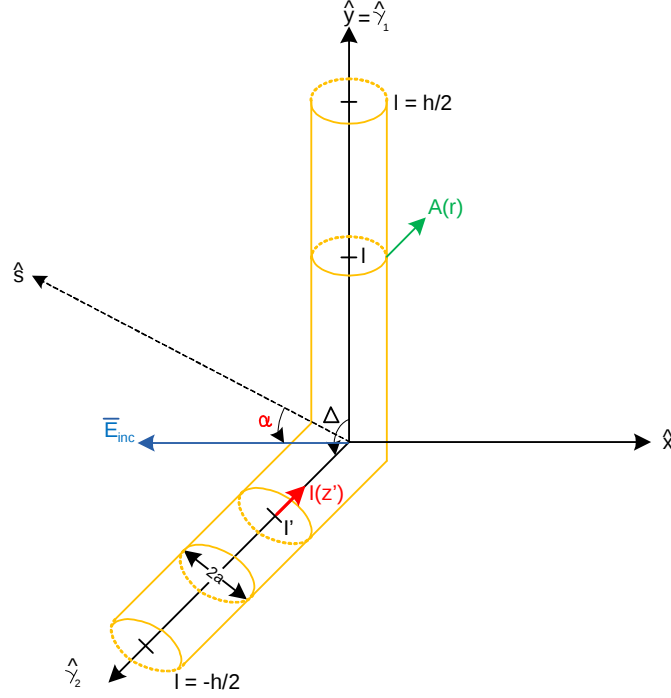
Figure 2.20: Depiction of the simplified geometry of V-shaped nanoantennas.
