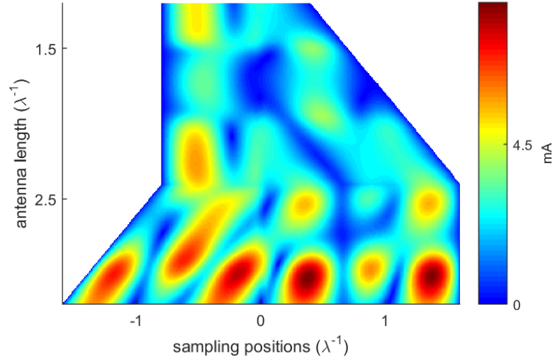
Figure 2.14: Amplitudes of the current distributions on L-shaped nanoantennas with symmetric excitation.
