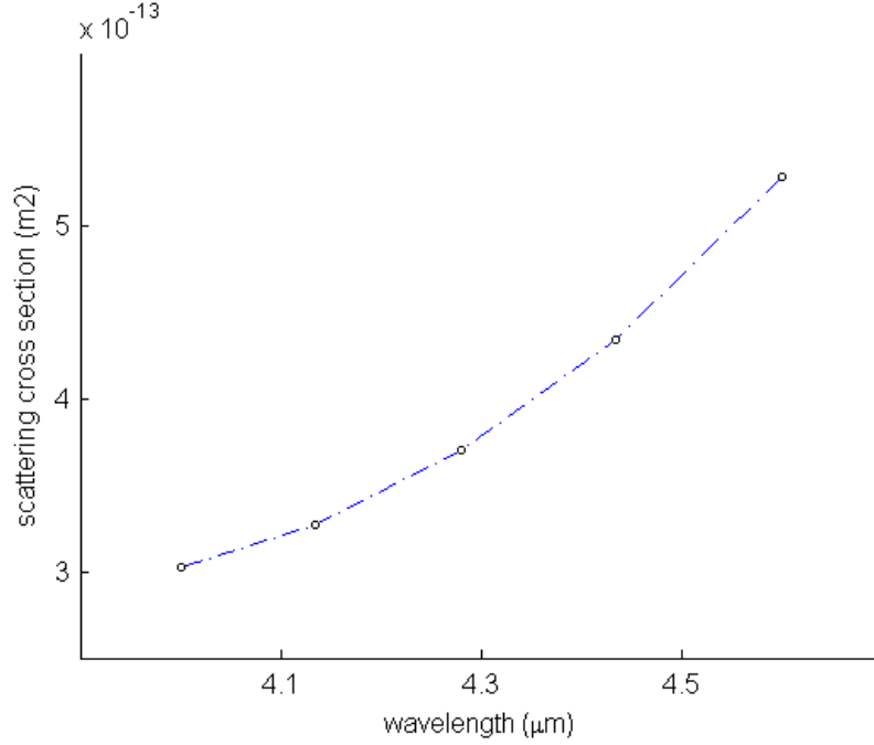
Figure 4.5: Scattering cross-section of the V-shaped nanoantenna having equal arm lengths of 395 nm and an opening angle of 78^\circ .
