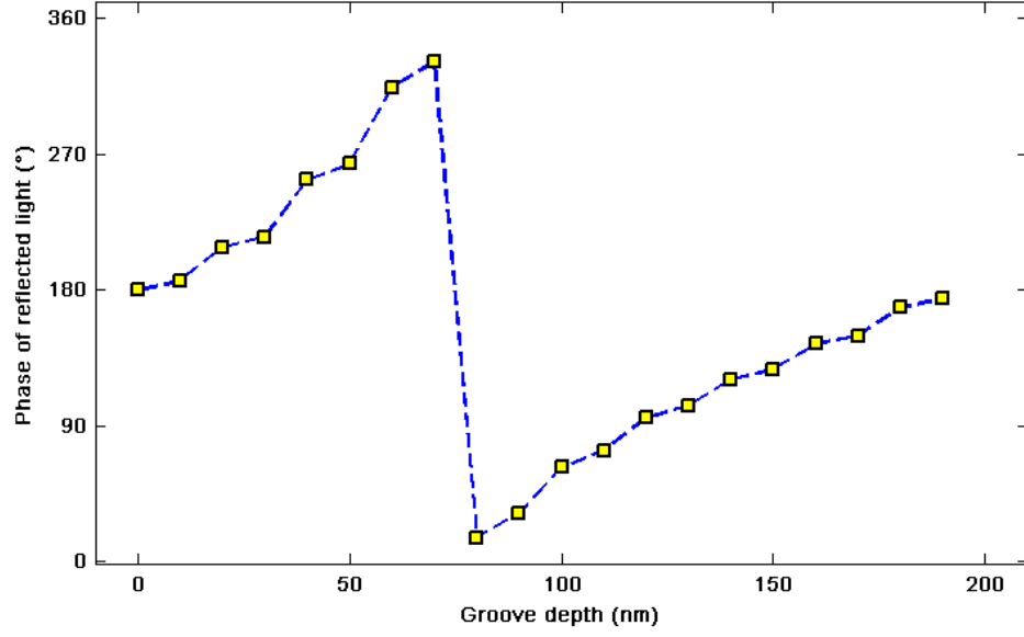
Figure 3.13: Phase shift imposed by the metasurface mirrors with varying nanogroove (without CdTe) depths.
