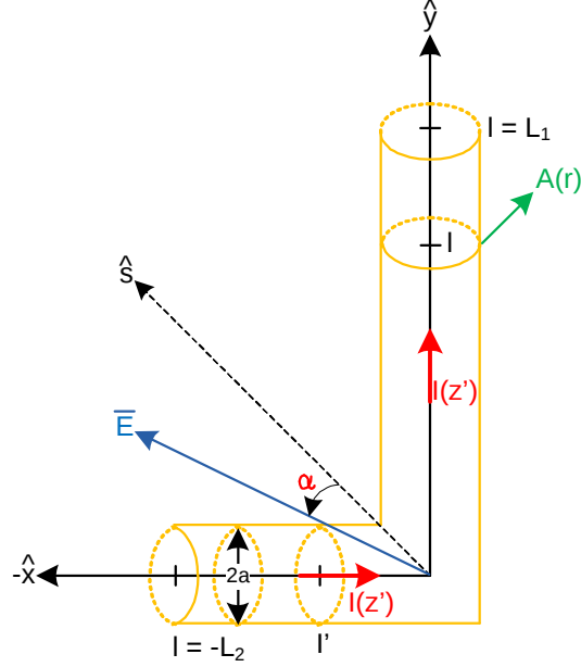
Figure 2.12: Depiction of the simplified geometry of L-shaped nanoantennas.
