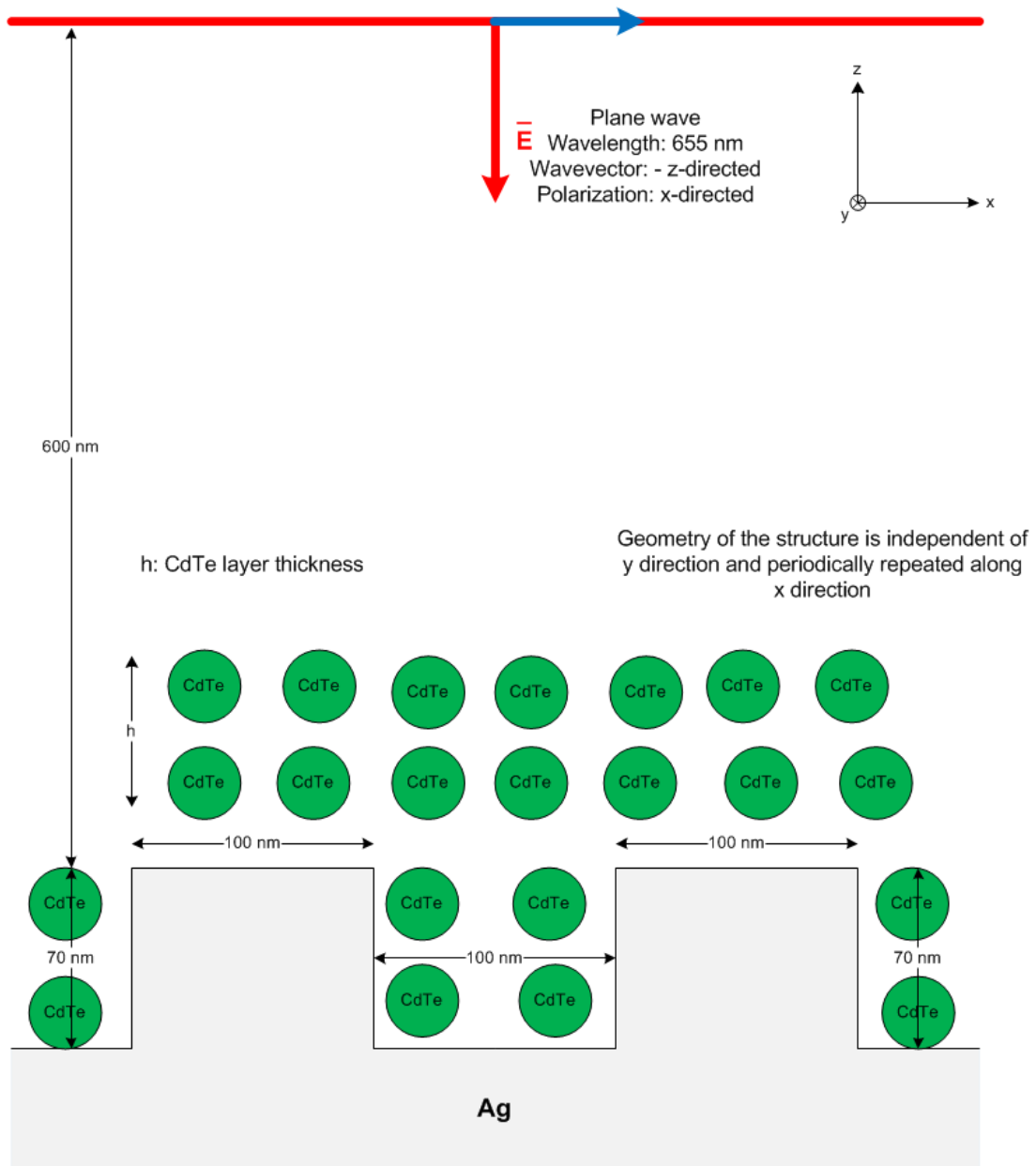
Figure 3.10: Schematic of the metamirror with CdTe quantum dots on top.
