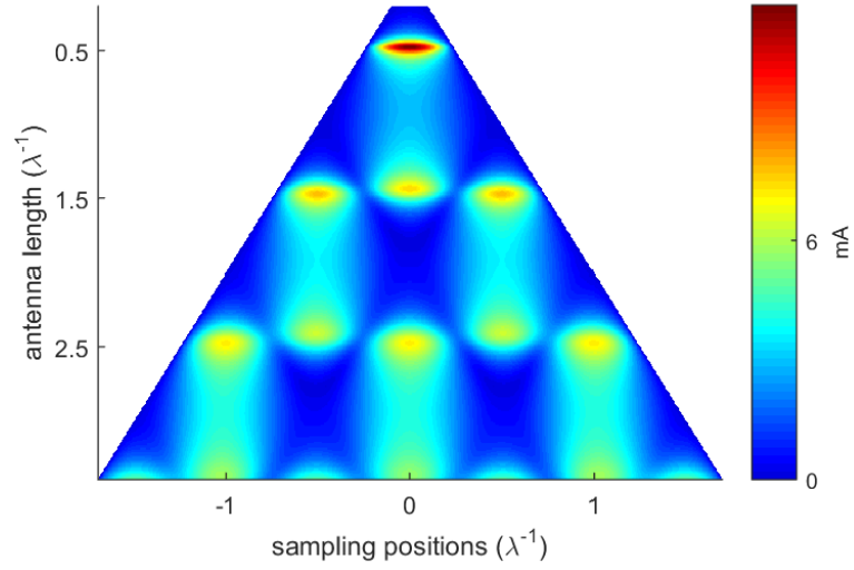
Figure 2.24: Amplitudes of the current distributions on V-shaped nanoantennas with antisymmetric excitation.
