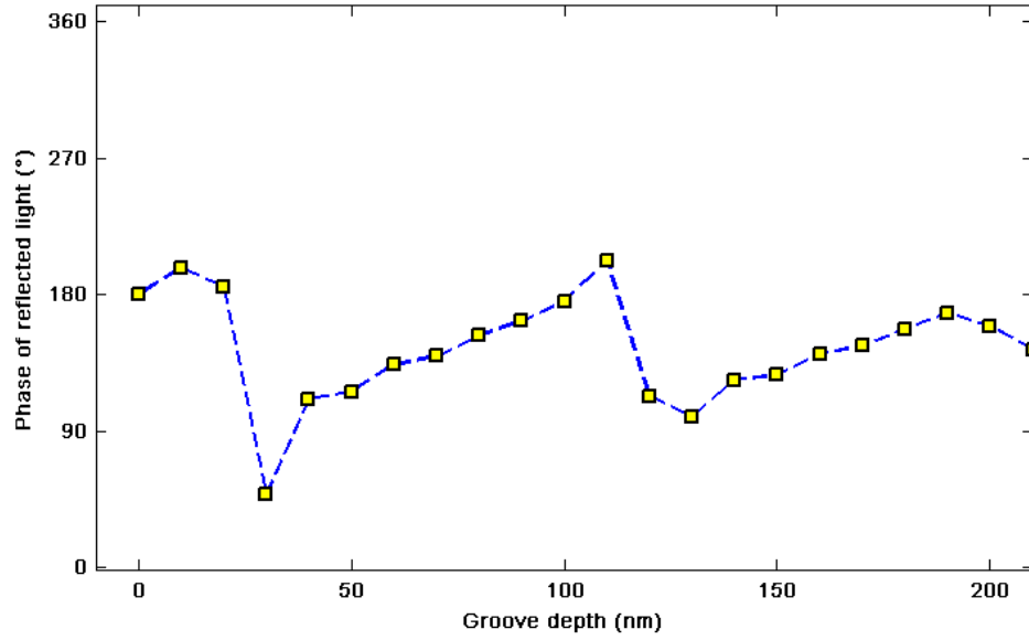
Figure 3.14: Phase shift imposed by the metasurface mirrors with varying nanogroove (filled with CdTe) depths.
