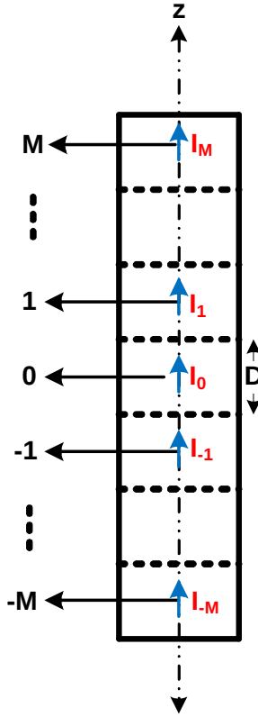
Figure 2.7: Current discretization on a rod antenna.
