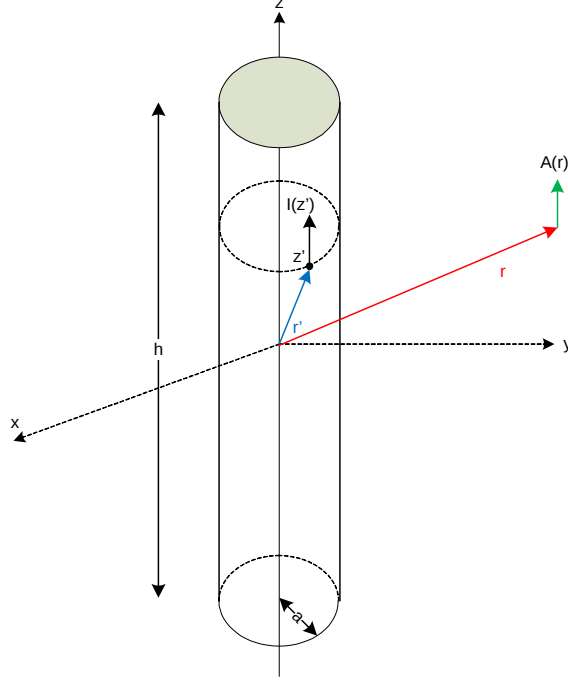
Figure 2.6: Thin-wire model of a rod antenna.
