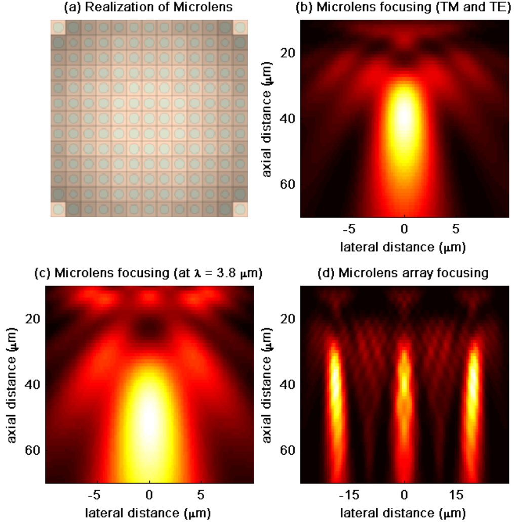
Figure 5.2: (a) Realization of the optimized central microlens design using silicon nanodisks (where color of unit cells are graded within constant phase regions). (b) Far-field intensity distribution of light focused by the central microlens of the optimized design when excited with either TM- or TE-polarized light. (c) Far-field intensity distribution of light focused by the central microlens of the optimized design for the wavelength of 3.5 \mu m , which is different from the design wavelength. (d) Far-field intensity distribution of light focused by different pixels of the optimized microlens array design.
