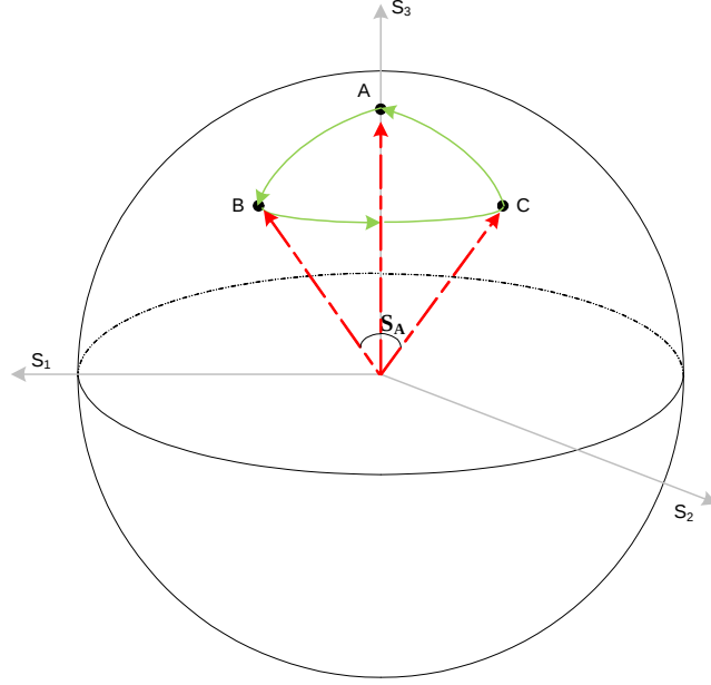
Figure 2.1: Cyclic polarization state transitions on the Poincaré sphere.
