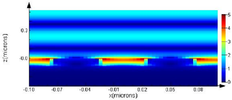
Figure 3.12: TM polarized field distribution on the top of the metasurface magnetic mirror.
