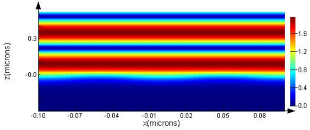
Figure 3.11: TE polarized field distribution on the top of the metasurface magnetic mirror.
