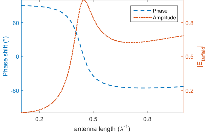
Figure 2.11: Calculated phase and normalized amplitude responses of PEC rod antennas.
