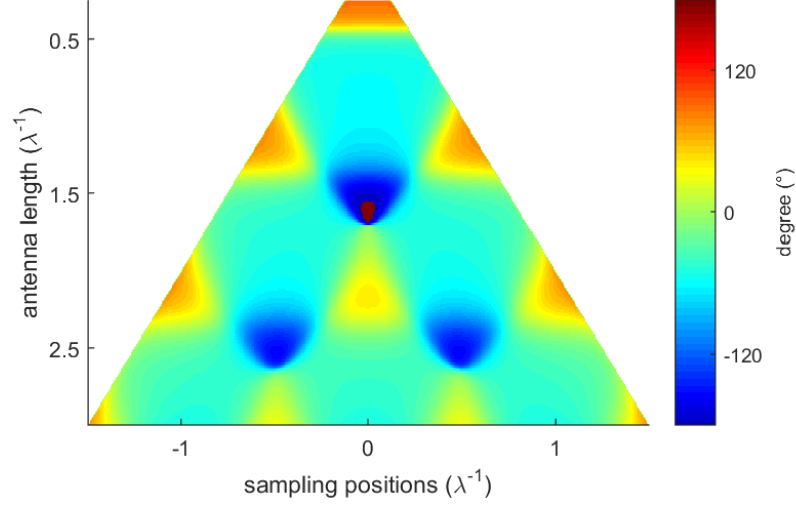
Figure 2.9: Phase of the current distributions on rod antennas.
