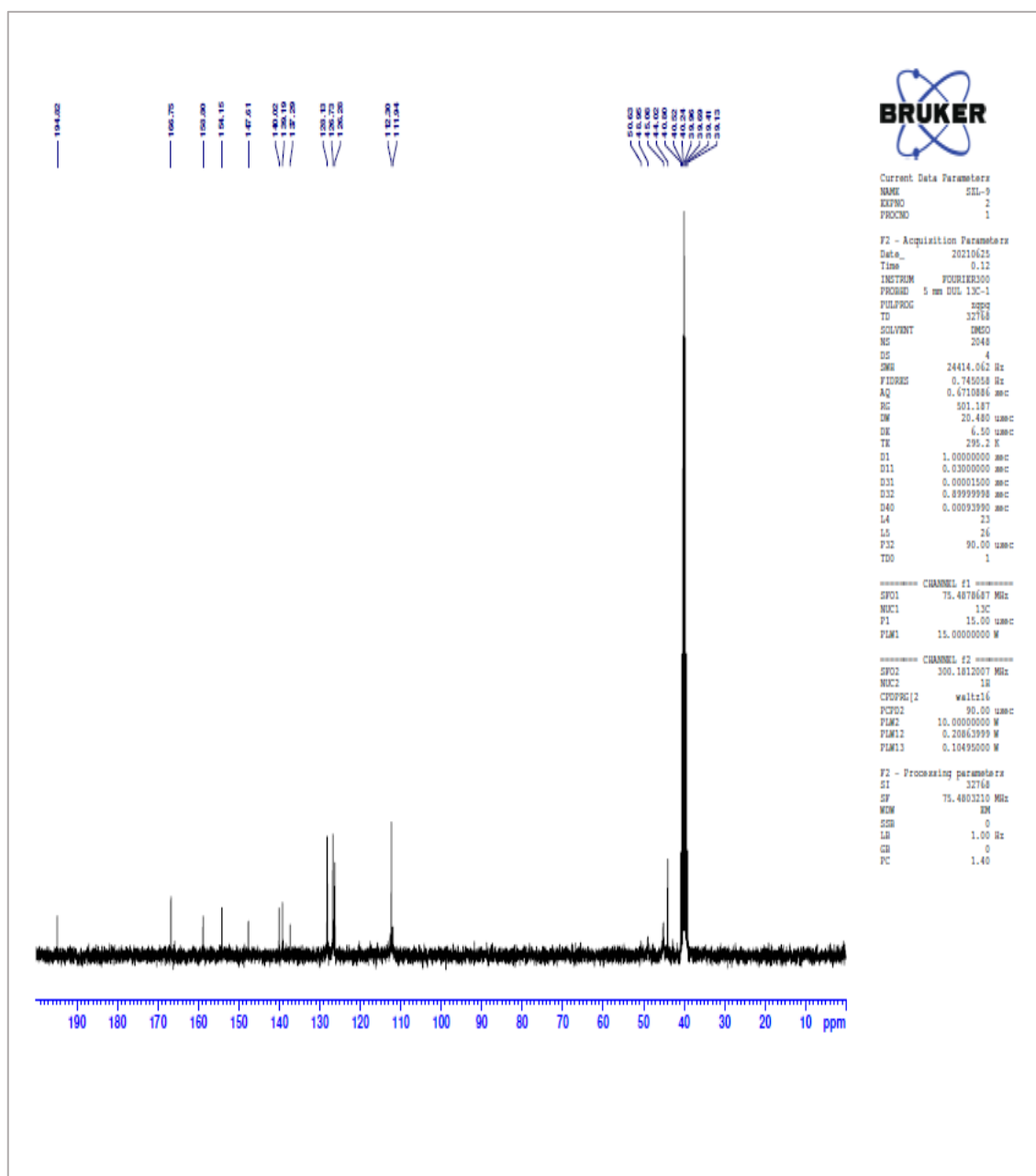
Figure 5.18. ^{13}\text{C} -NMR spectrum of Compound 5i .
