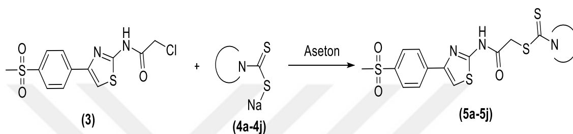
Figure 4.5. Synthesis of Target Compounds (5a-5j). 35
