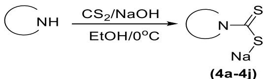
Figure 4.4. Synthesis of Dithiocarbamate Derivatives (4a-4j).
