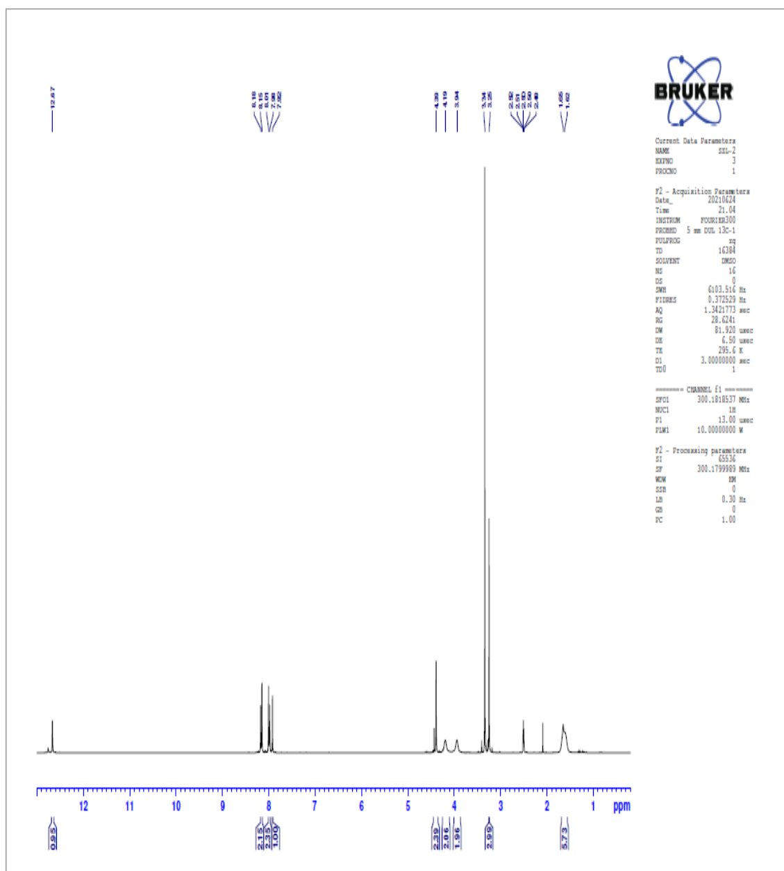
Figure 5.3. ^1\text{H} -NMR spectrum of Compound 5b .
