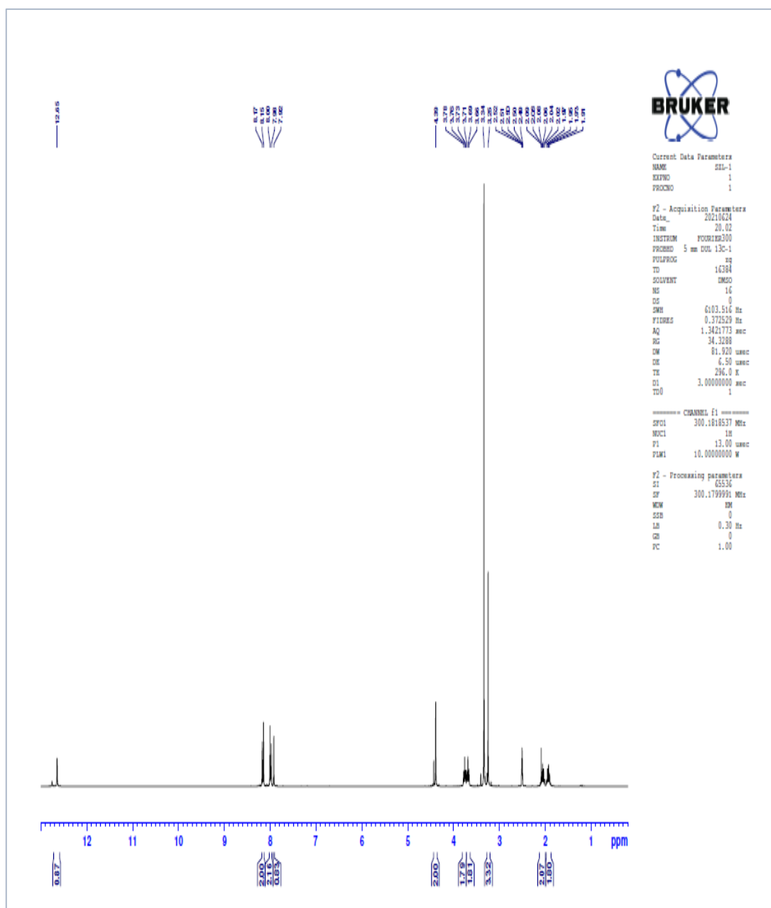
Figure 5.1. ^1\text{H} -NMR spectrum of Compound 5a
