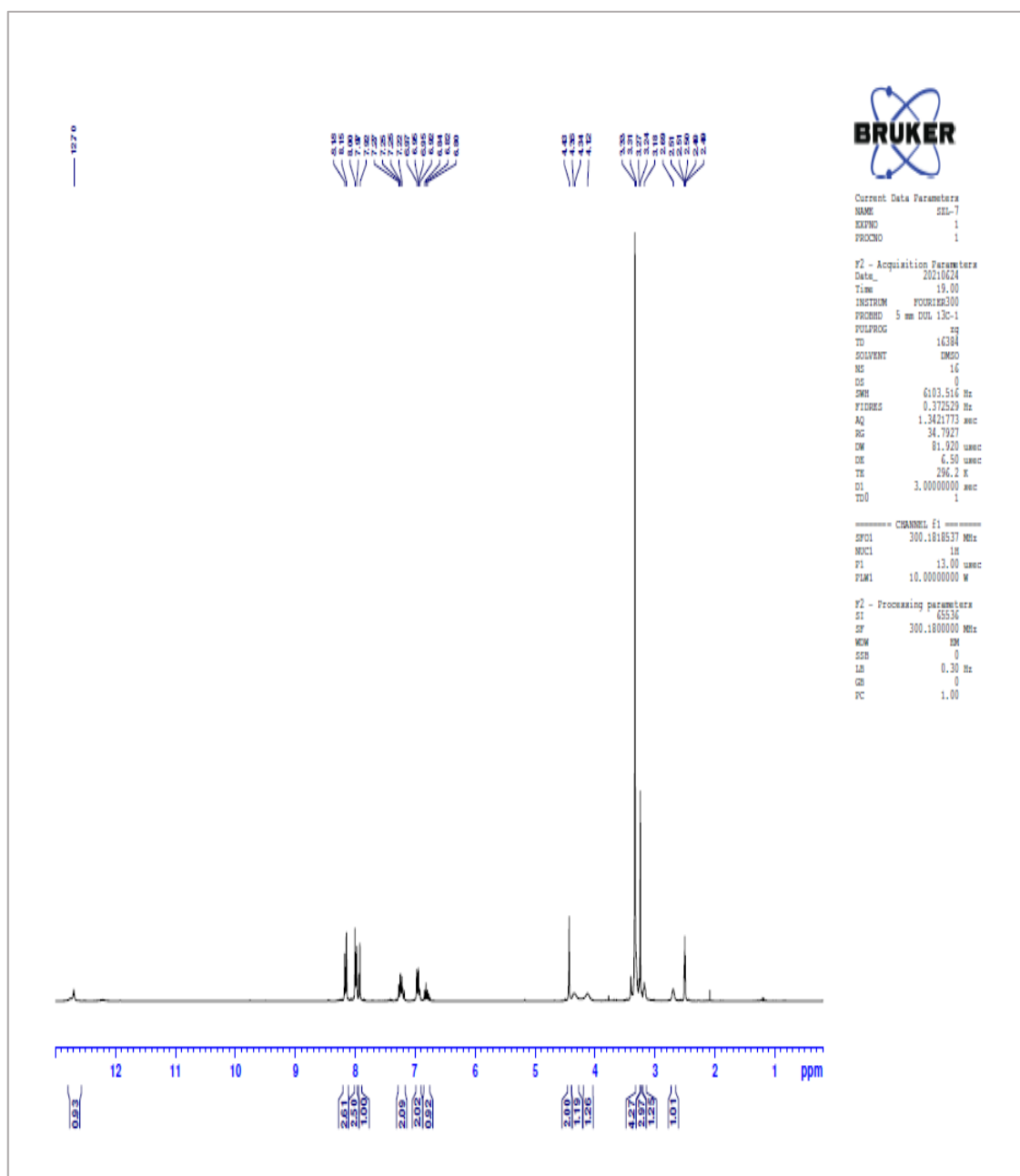
Figure 5.13. 1 H-NMR spectrum of Compound 5g.
