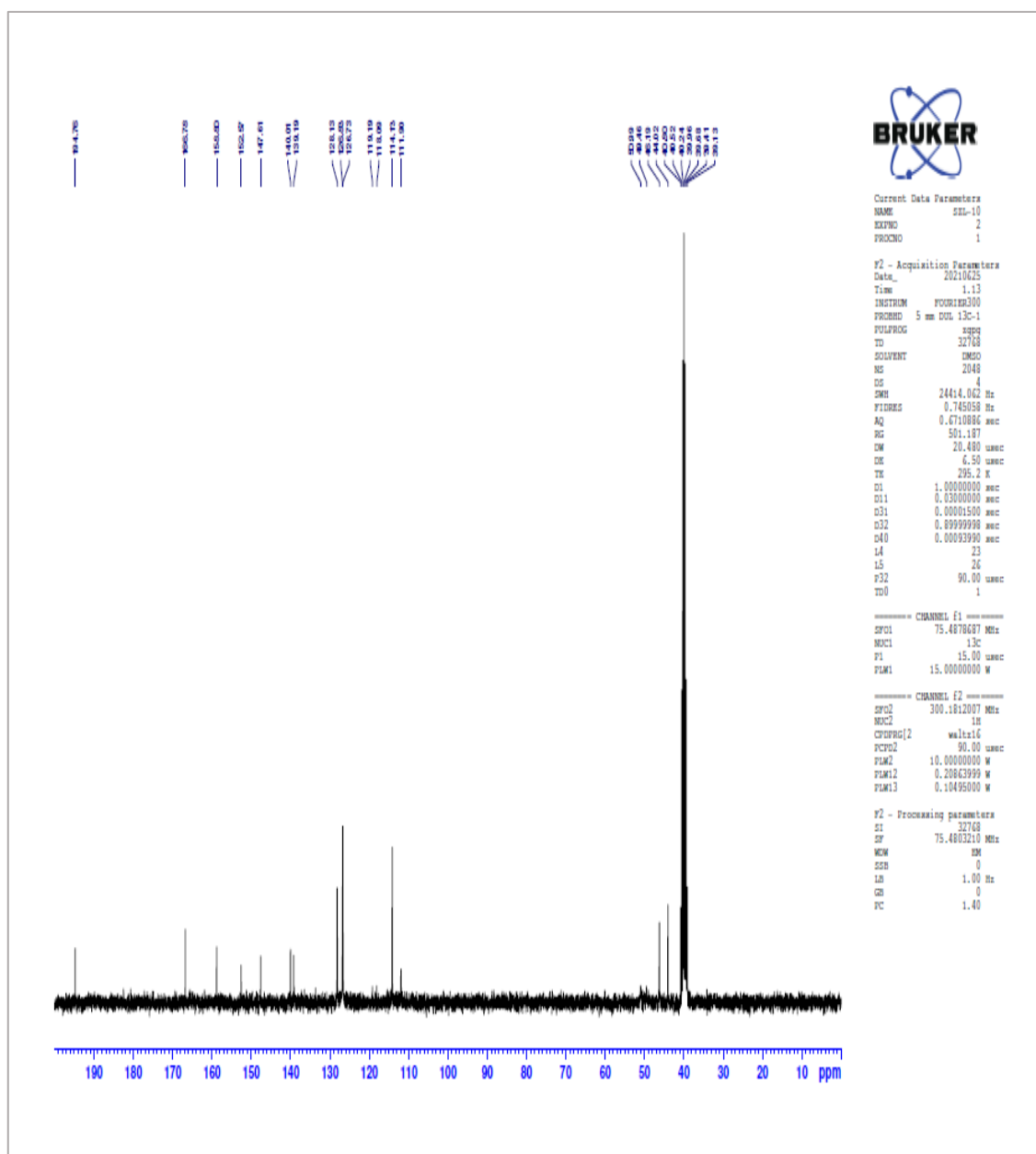
Figure 5.20. ^{13}\text{C} -NMR spectrum of Compound 5j.
