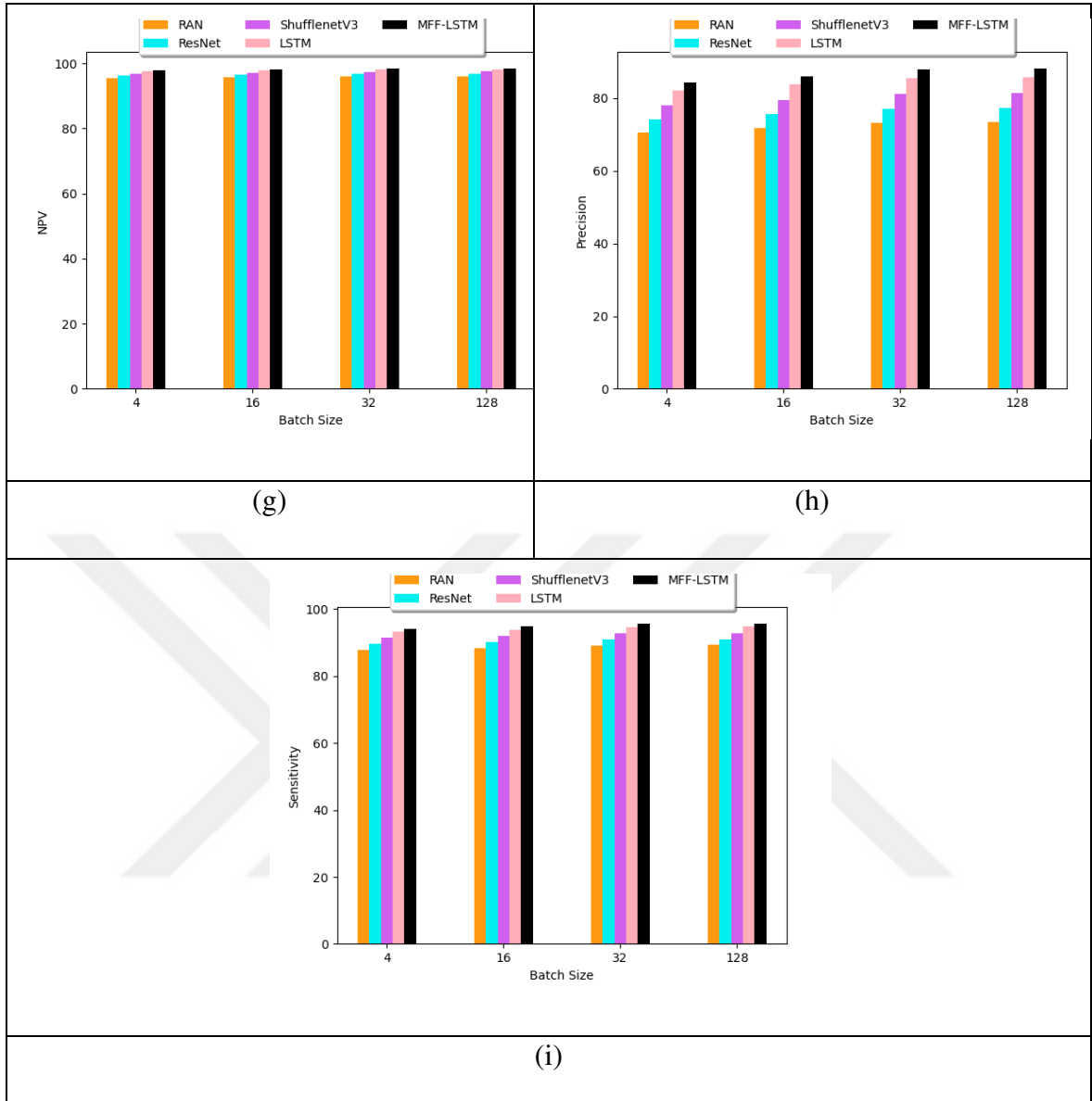
Figure 4.3: The Batch Size Evaluation of the Suggested Fake News Detection Model over Diverse Traditional Classifier for Catasnet 2 Concerning “ (a) Accuracy, (b) F1-score, (c) FDR, (d) FNR, (e) FPR, (f) MCC, (g) NPV, (h) Precision, (i) Sensitivity."Figure Continued"
