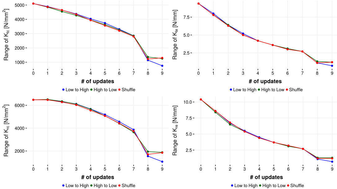
Figure D.3: Ranges of cutting force coefficients with respect to updates for experiment #3 in Table 4.4.
