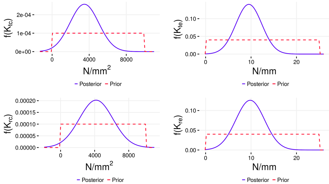
Figure B.3: Posterior ( blue lines ) and prior ( red dashed lines ) distributions of the force coefficients for the tool having 0.4 mm diameter and 40 \mu\text{m} depth of cut.
