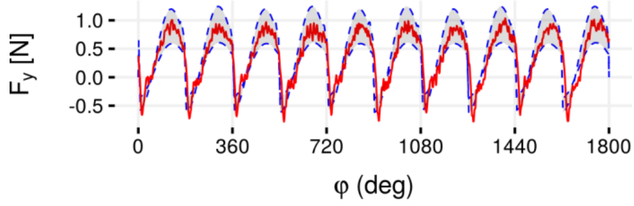
Figure 3.4: Simulated and measured force predictions for 2\mu\text{m}/\text{tooth} feed slot milling with a. normal distribution b. uniform prior distribution
