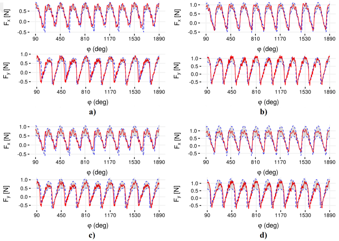
Figure 3.3: Simulated (blue dashed lines) and measured (red solid lines) force predictions for a. 0.4\text{ }\mu\text{m/tooth-normal} distribution b. 2\text{ }\mu\text{m/tooth-normal} distribution c. 0.4\text{ }\mu\text{m/tooth-uniform} distribution d. 2\text{ }\mu\text{m/tooth-uniform} distribution
