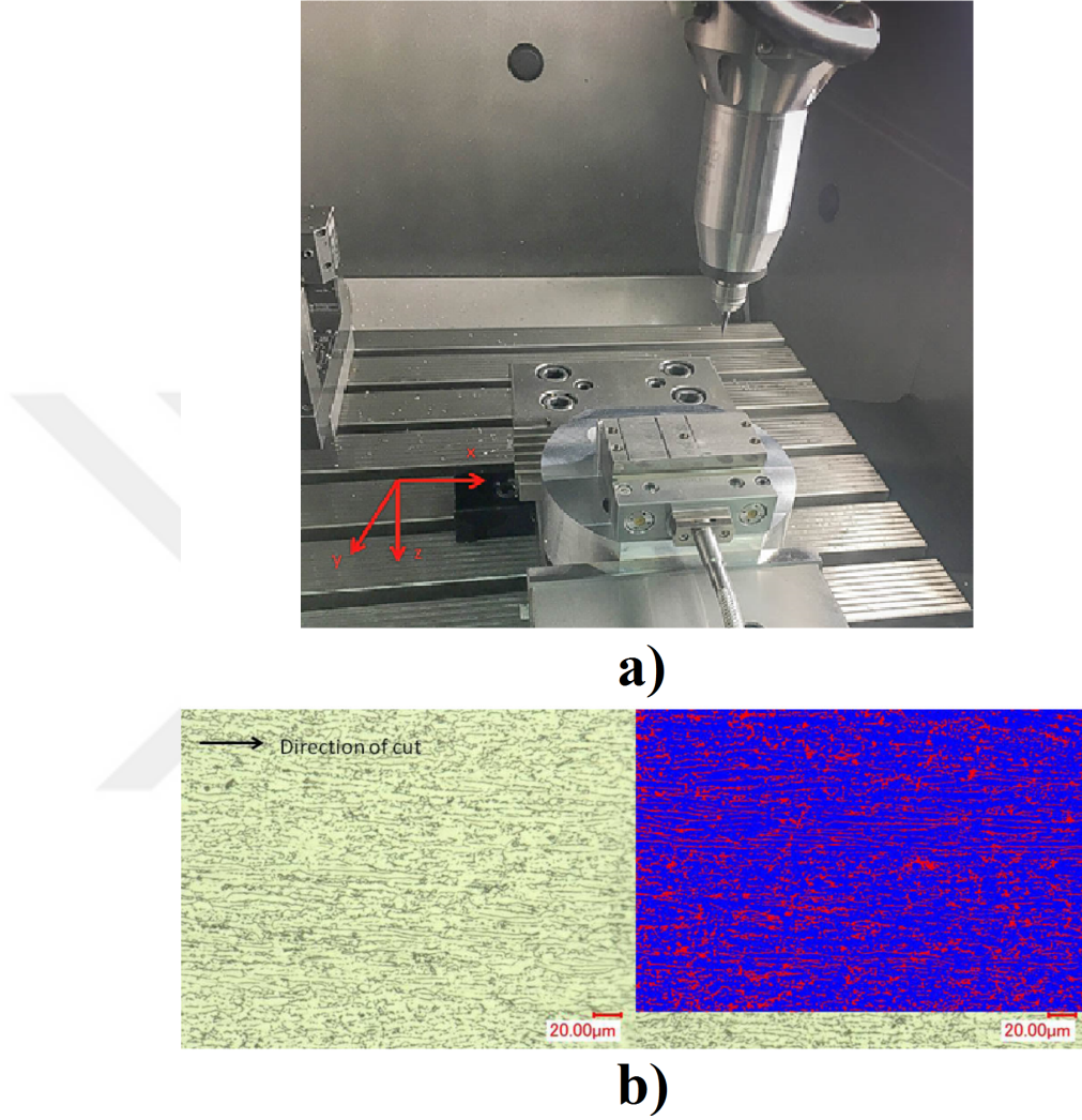
Figure 2.1: a. Experimental setup of milling experiments. b. Microstructure of the material
