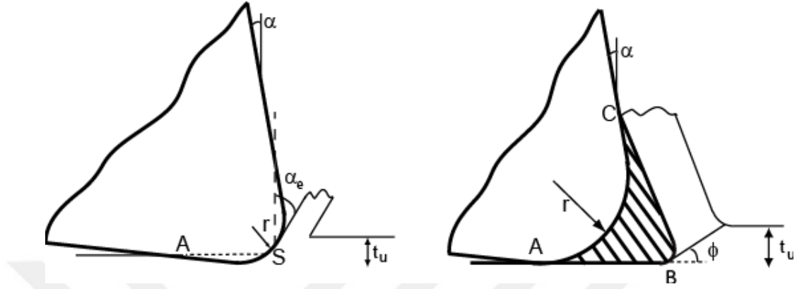
Figure 2.4: Two possible configurations of microscale cutting. Stagnation point assumption ( left ) and BUE formation ( right ).
