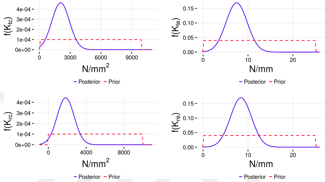
Figure B.2: Posterior ( blue lines ) and prior ( red dashed lines ) distributions of the force coefficients for the tool having 0.4 mm diameter and 80 \mu\text{m} depth of cut.
