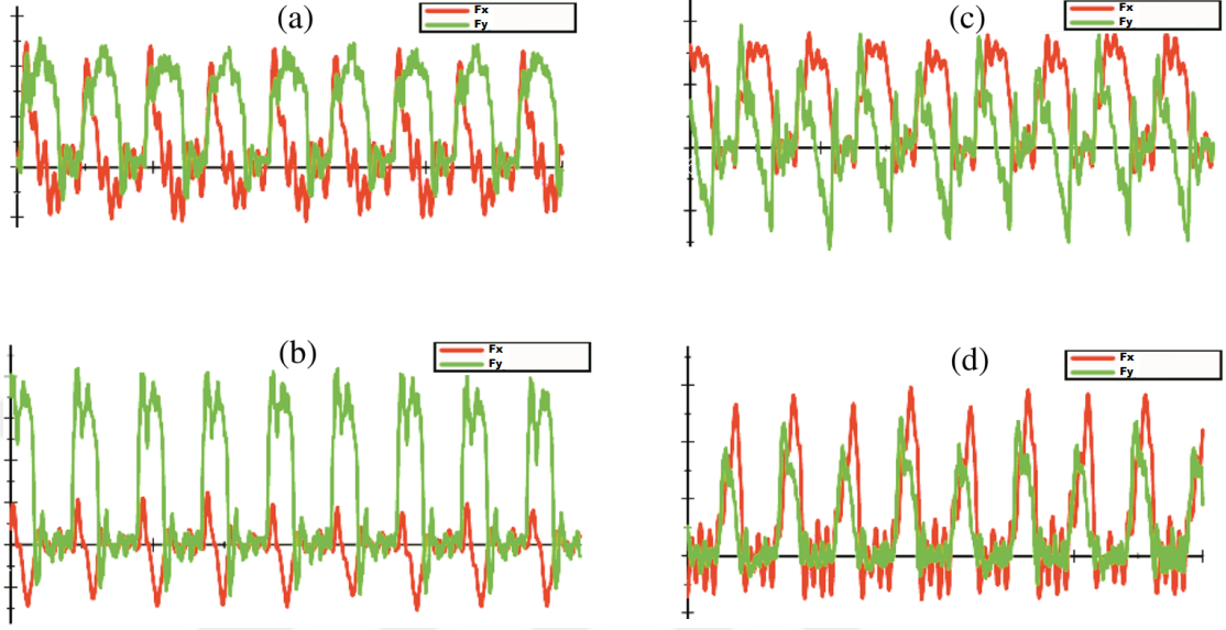
Figure 3.5: Measured micromilling forces at 2\text{ }\mu\text{m/tooth} and axial depth of cut 40\text{ }\mu\text{m} . a. 60% RI-downmilling. b. 25% RI-downmilling. c. 60% RI-upmilling. d. 25% RI-upmilling
