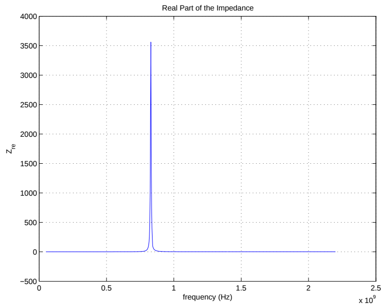
Figure 3.5: Real part of the impedance.
