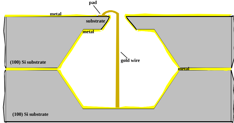
Figure 4.2: Initial design.
