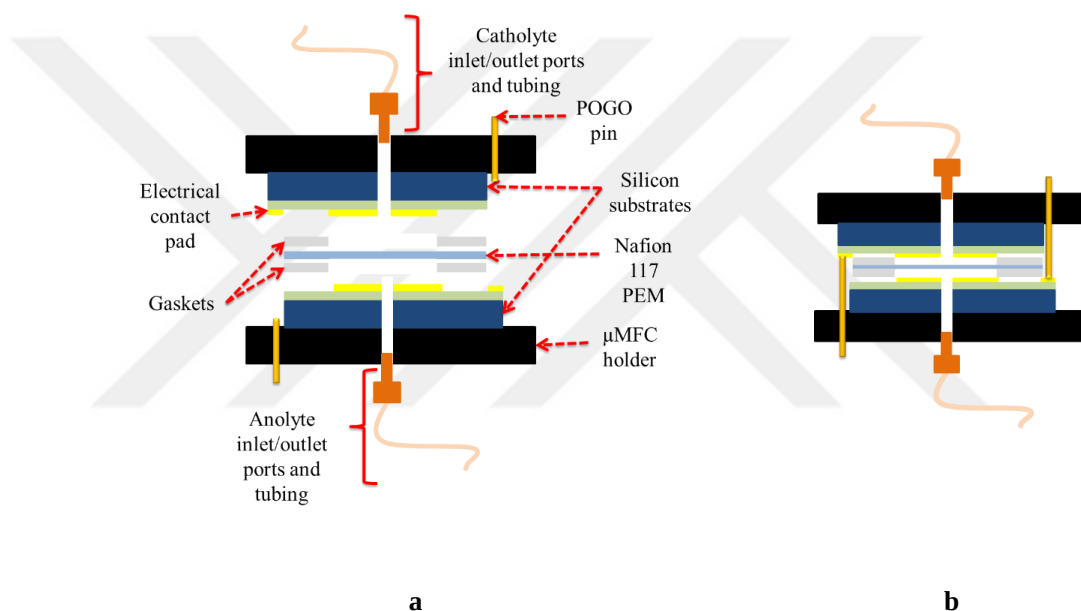
Figure 3.23. Schematic of \mu MFC. a: extended view; b: assembled view.
