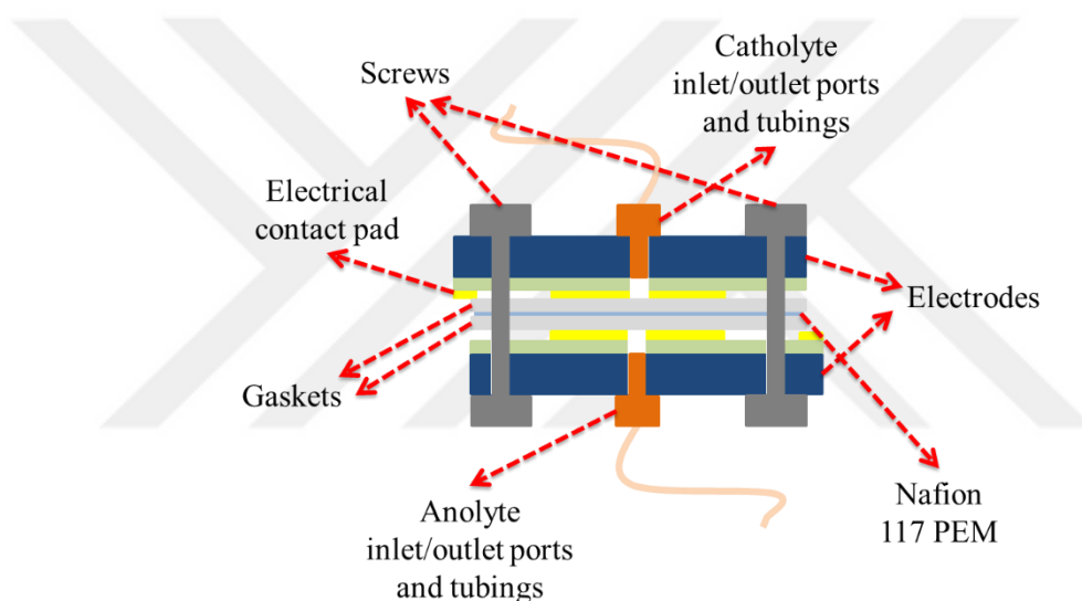
Figure 3.18. Designed schematic for \mu MFC assembly.
