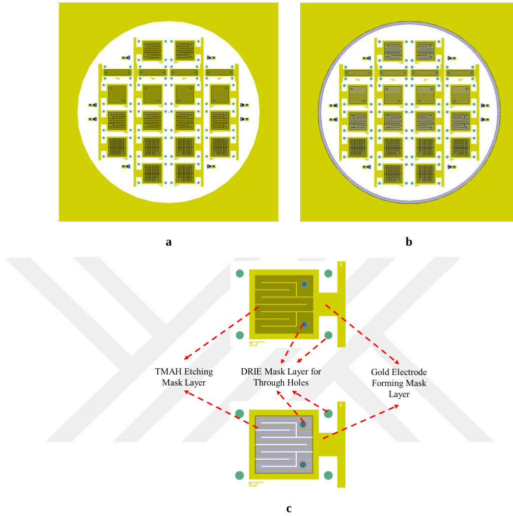
Figure 3.1. Designs of 4" mask for microfabrication of 1 st generation electrodes. a: Mask including serpentine electrodes on wafer level; b: Mask including serpentine ultra-micro electrodes on wafer level; c: Die level masks for SE and S-UME electrode designs used in the study.
