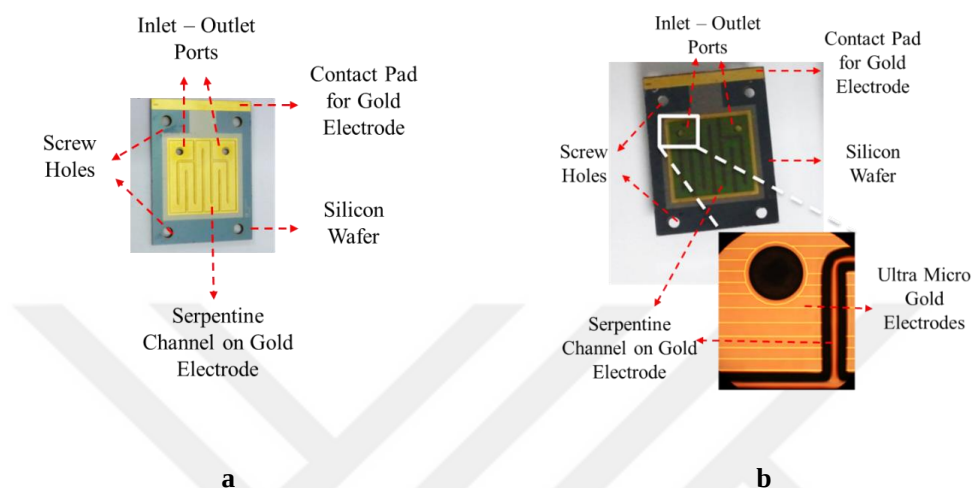
Figure 3.4. Diced 1 st generation electrodes. a: Serpentine electrodes; b: Serpentine ultra-micro electrodes.
