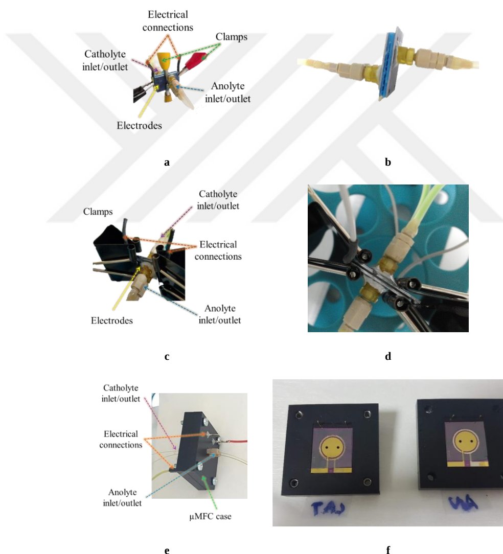
Figure 4.2. Assembly of \mu MFC at different stages of the study. a, b: Deep chamber \mu MFC; c, d: Shallow chamber \mu MFC; e, f: Shallow chamber \mu MFC with holder.
