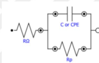
Figure 2.7. Simplified Randle's model as an equivalent circuit. R\Omega : electrolyte resistance, R_p : polarization resistance, C/CPE: Capacitance/Constant phase element.
