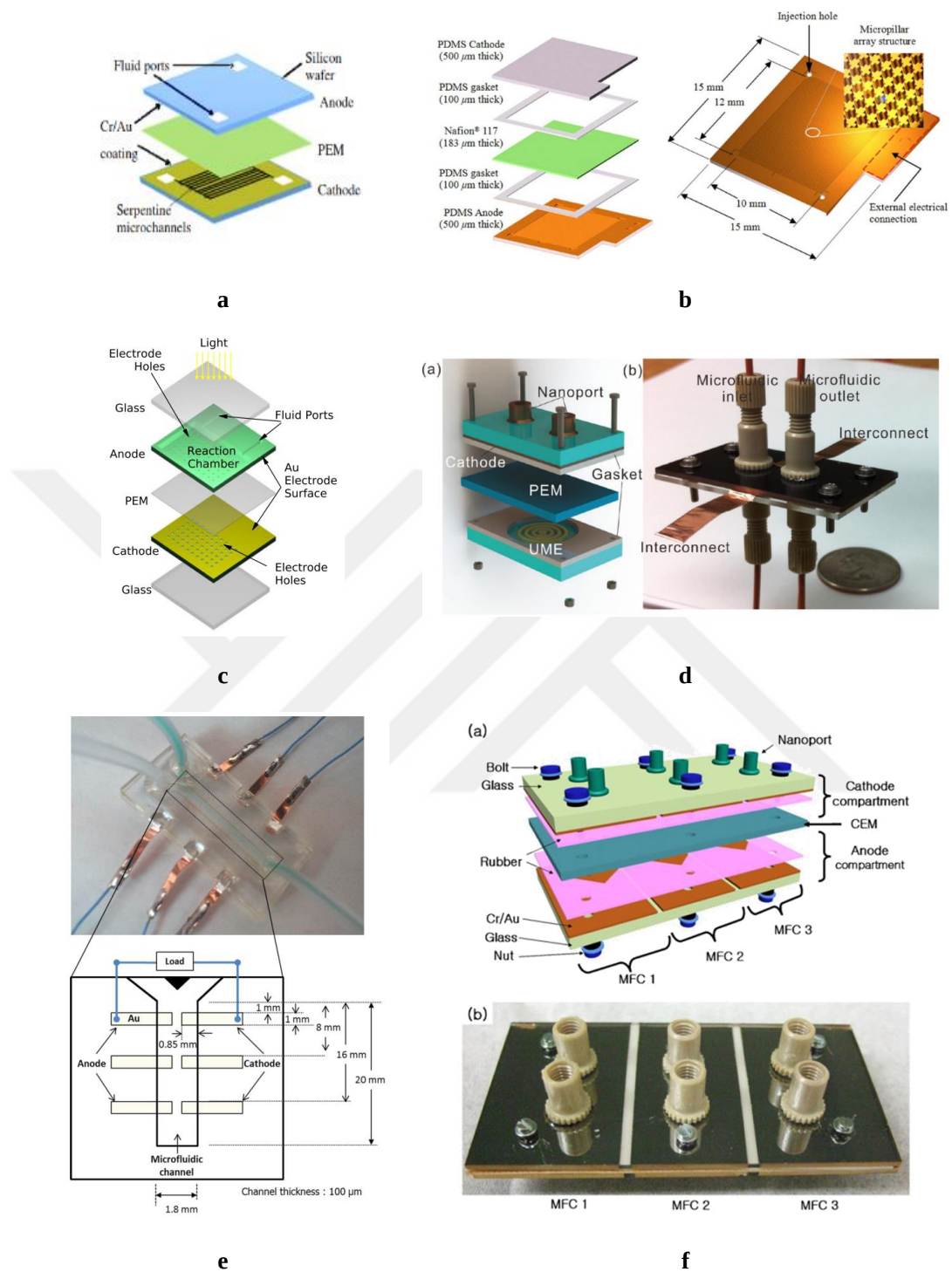
Figure 2.5. a: Exploded view of a double chamber \mu MFC [31]; b: Schematic image of a PDMS \mu MFC [76]; c: Schematic of a photosynthetic MFC [31]; d: Schematic and image of a glass \mu MFC [31]; e: Schematic and image of a laminar flow \mu MFC [110]; f: Schematic and image of a \mu MFC stack [111].
