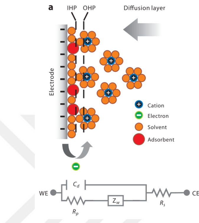
Figure 2.9. Top: an electrified interface in which the electrode is negatively charged and counter cations are aligned along the electrified surface; Bottom: electrical circuit elements corresponding to each interface component for an idealized Randles electrical equivalent circuit for the interface ( C_d , double-layer capacitor; CE, counter electrode; IHP, inner Helmholtz plane; OHP, outer Helmholtz plane; R_p , polarization resistance; R_s , solution resistance; WE, working electrode; Z_w , Warburg impedance) [132].
