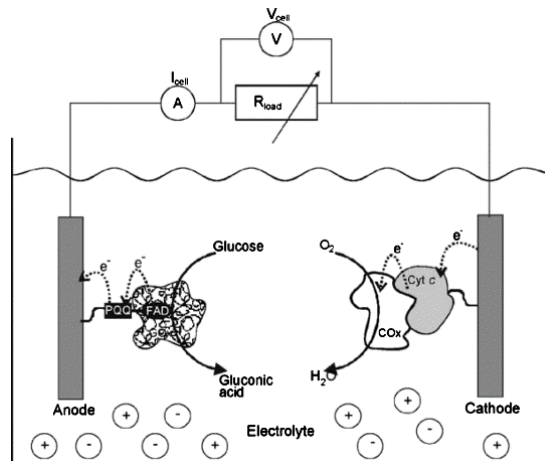
Figure 2.3. A single chamber enzymatic fuel cell running on glucose and O_2 [52].
