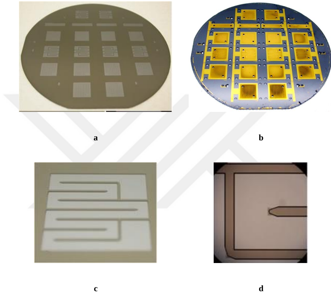
Figure 3.3. Microfabricated 1 st generation electrodes. a: TMAH etched silicon wafer; b: Silicon wafer after sputtering of gold layers and before dicing; c: TMAH etched serpentine channels on silicon; d: Close-up of serpentine channel before gold sputtering where blunt corners were observed outer on right-angles due to TMAH etching.
