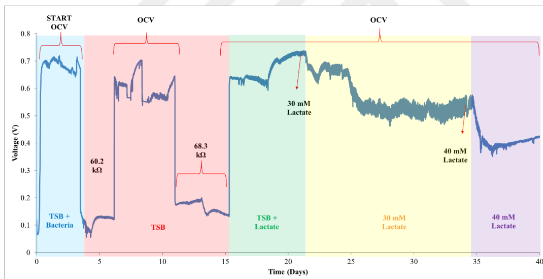
Figure 5.5. Operation of an \mu MFC with SE for 40 days. System was started at OCV conditions and fed with different anolytes were throughout 40 days.
