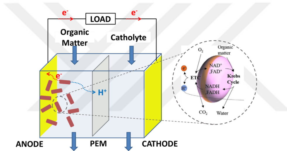
Figure 2.1. Microbial fuel cell mechanism (adapted from [36]), Krebs Cycle: cycle for cellular respiration; PEM: Proton Exchange Membrane; NADH, NAD^+ , FADH , FAD^+ : coenzymes for electron transport, ETC: Electron transport chain.
