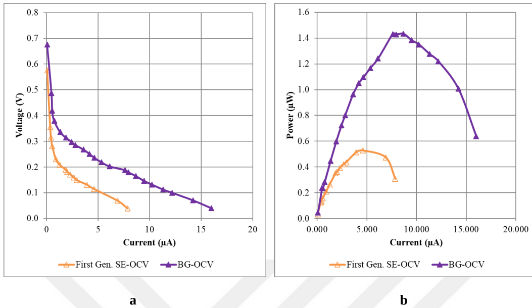
Figure 5.12. Comparison of polarization and power curves of 1 st (SE) and 2 nd generation (round) μMFC systems operated with TSB under OCV conditions.
