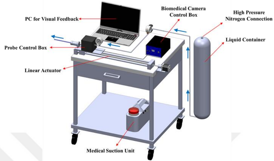
Figure 2.5. Final design of the cavitation-based device for medical treatment. The blue arrow shows the direction of the liquid inside the hydrodynamic cavitation section of the device.
