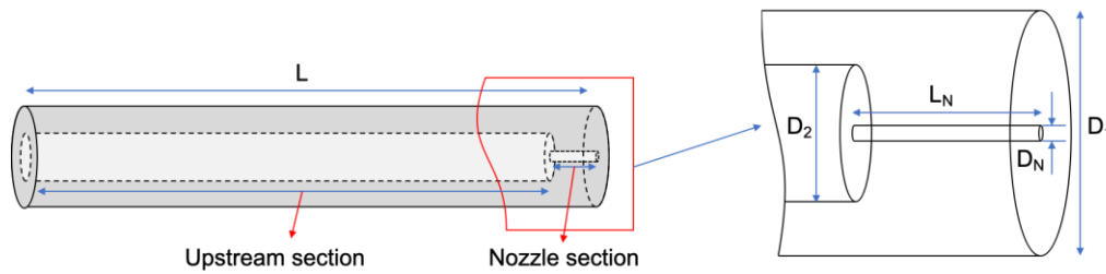
Figure 2.2. Schematic of the test nozzle.
