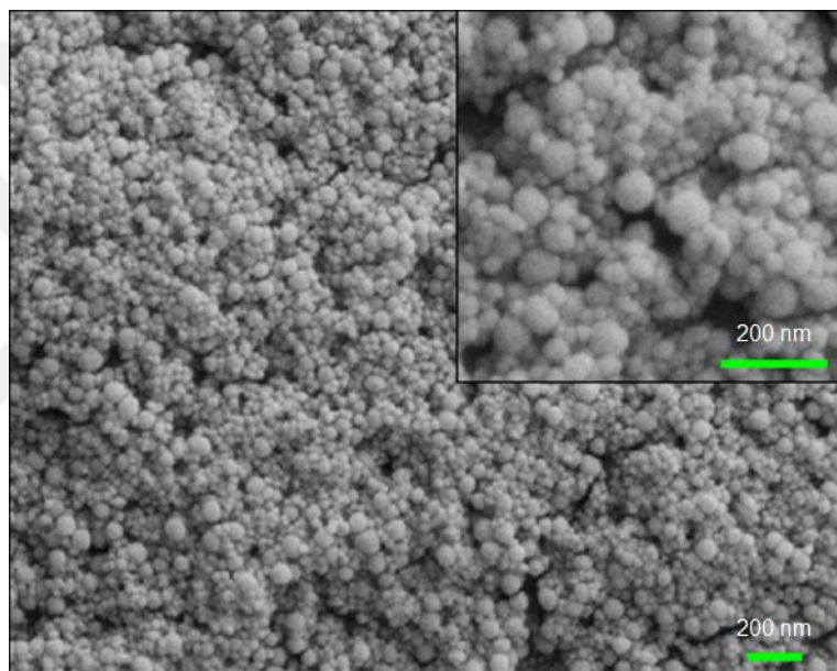
Figure 2.3. SEM image of the layer-by-layer assembled surface on a quartz plate.
