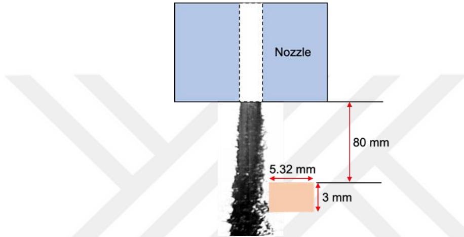
Figure 3.2. Position of the window used for spray visualization during droplet measurements.
