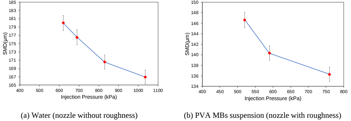
Figure 4.8. Effect of cavitation on overall SMD.
