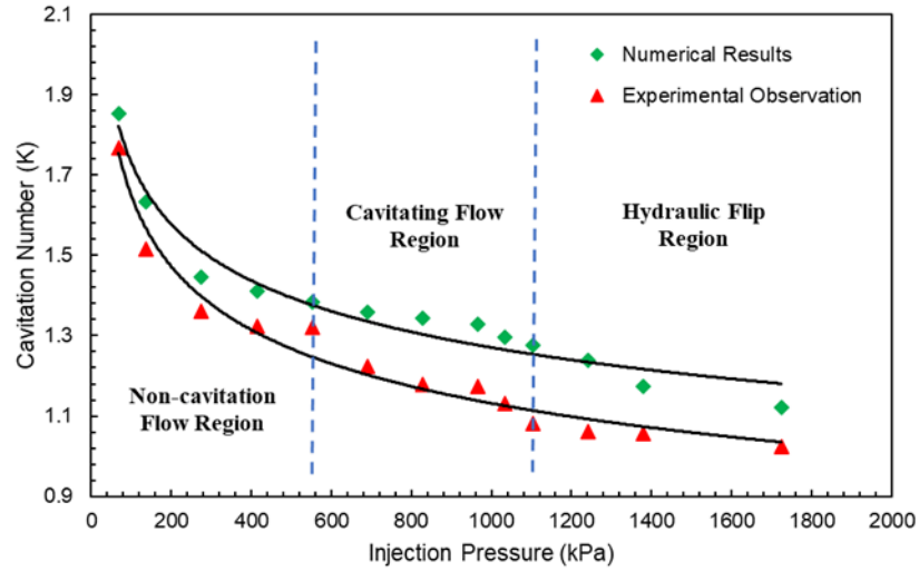
Figure 4.13. Variation of cavitation number with respect to the injection pressure.
