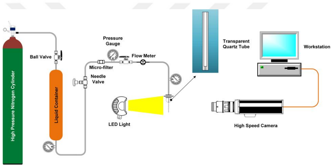
Figure 2.1. Schematic of the experimental setup.
