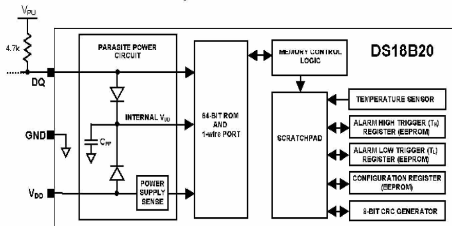
DS18B20 BLOCK DIAGRAM Figure 1
