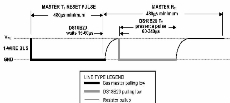
INITIALIZATION TIMING Figure 13
