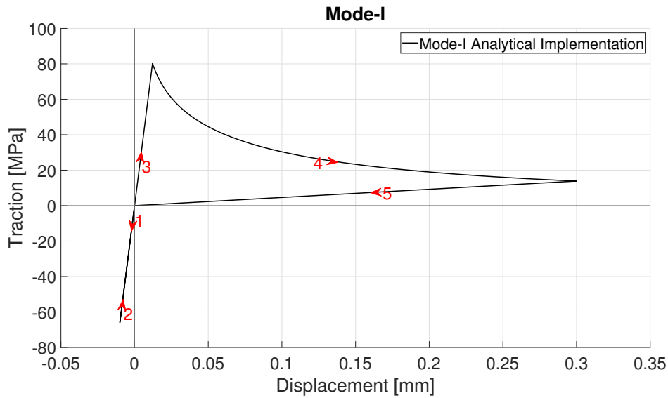
Figure 3.5: Traction versus displacement response to mode-I loading/unloading.
