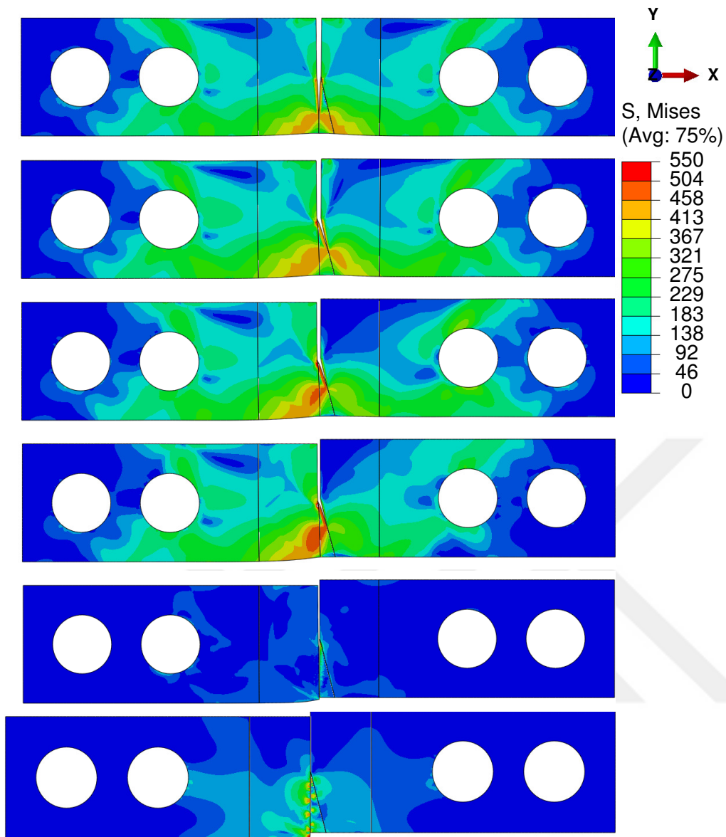
Figure 4.56: Von Mises stress at total displacement 1mm for different loading holes in SEN specimen. From top to bottom holes 1 to 6 are used.
