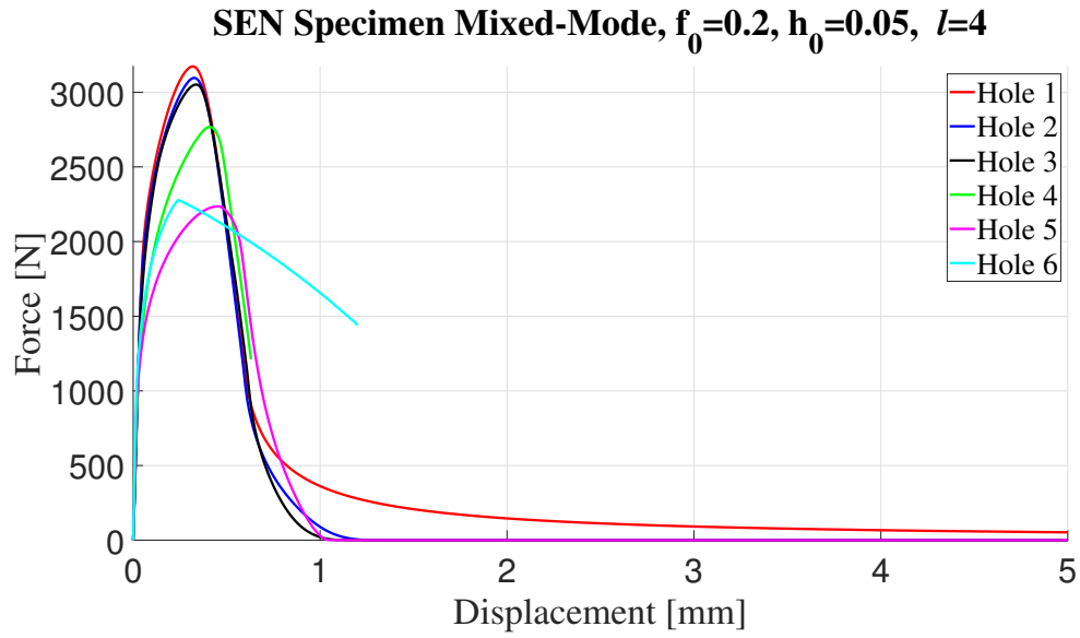
Figure 4.51: Force displacement response for loading through different holes.
