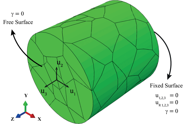
Figure 5.1: The representation of the boundary value problem with 100 grains.
