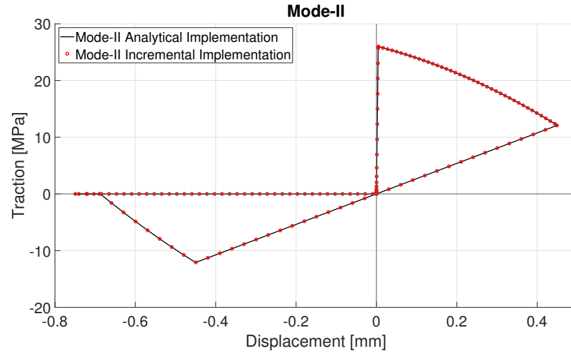
Figure 3.9: Traction versus displacement response to mode-II loading/unloading for incremental and analytical model.
