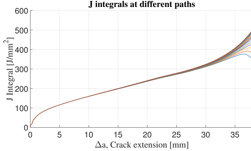
Figure 4.10: Path dependence of J integral for elasto-plastic models. \sigma_y = 500 MPa, f_0 = 0.1 , h_0 = 0.1 mm.
