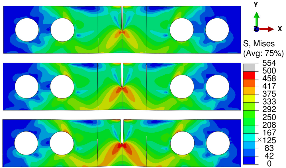
Figure 4.24: Von Mises stress contours just before softening begins. h_0 's are equal to: 0.05 (top), 0.1 (middle), 0.2 (bottom).
