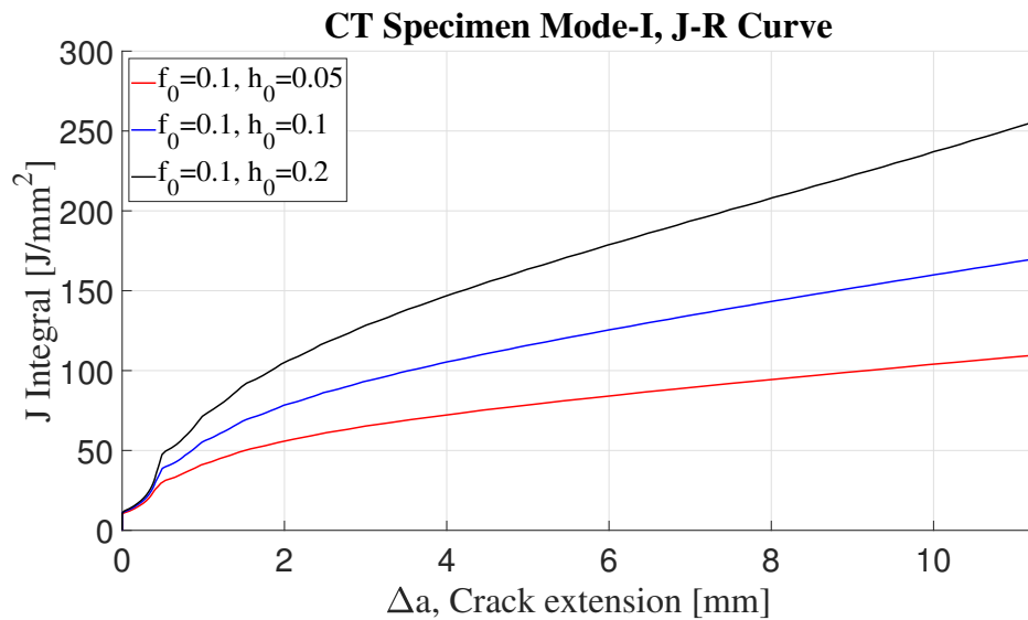
Figure 4.12: J-R curve constant f_0 , and changing h_0 .
