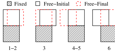
Figure 3.6: Mode-II loading history.
