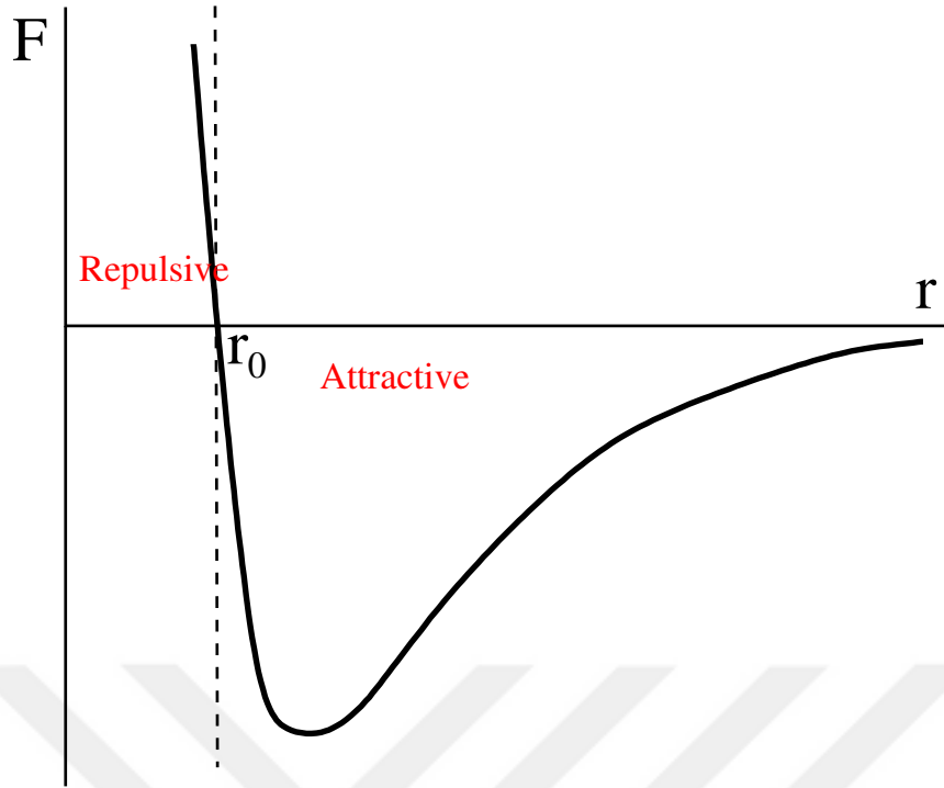
Figure 1.2: Repulsive and attractive forces with respect to distance between atoms.
