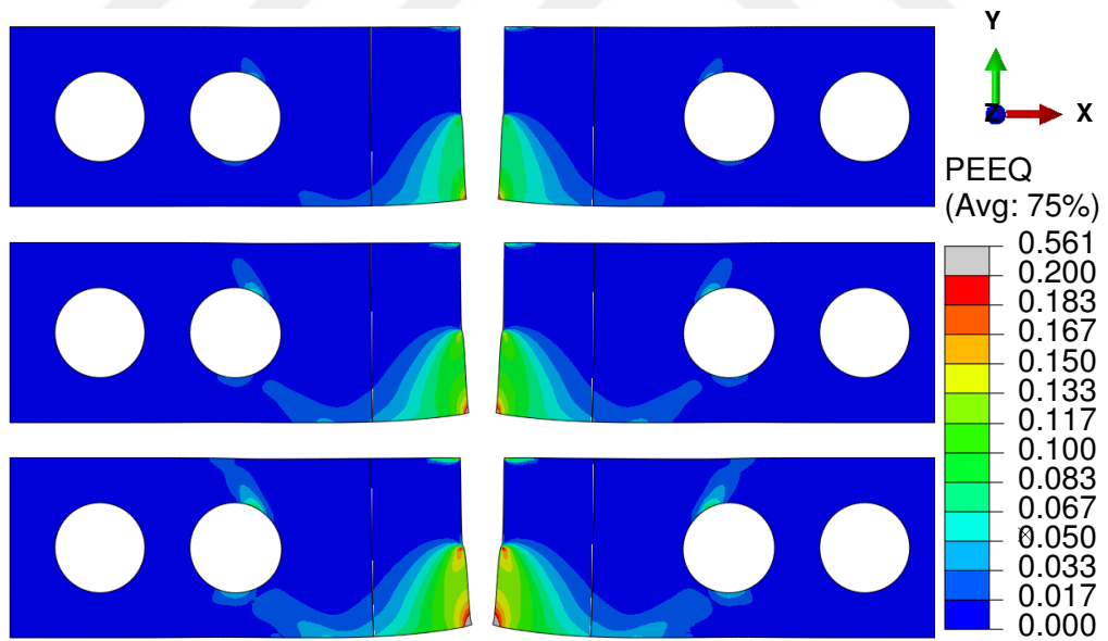
Figure 4.25: Equivalent plastic strain after failure. h_0 's are equal to: 0.05 (top), 0.1 (middle), 0.2 (bottom).
