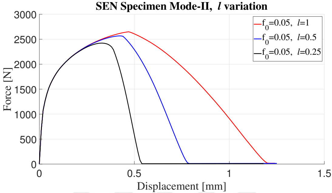
Figure 4.35: Force displacement response under mode-II loading for changing pore spacing, l .
