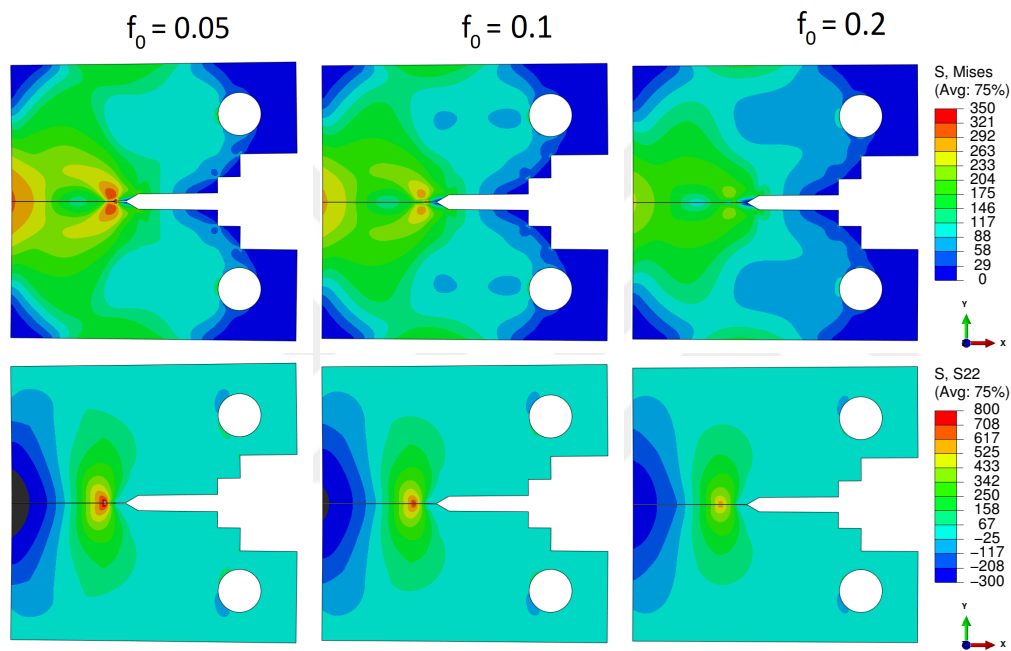
Figure 4.3: Stress contours for different initial pore fractions are shown, where the top row is the von Mises stress and the bottom row is the normal stress in the y-direction.
