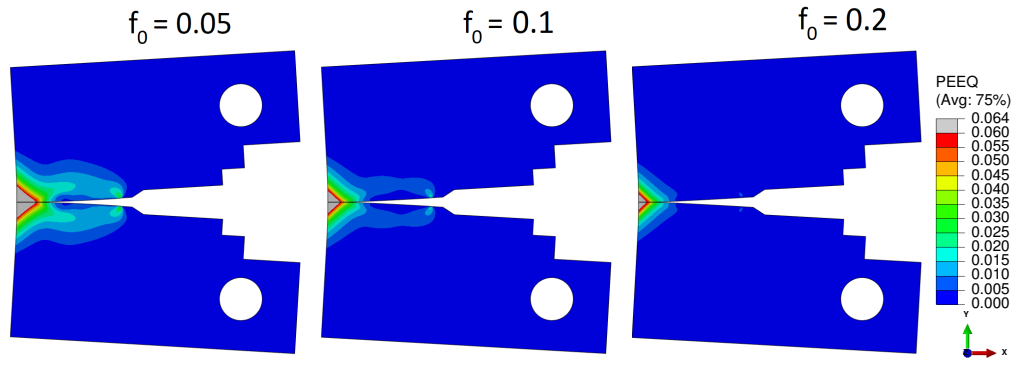
Figure 4.6: Equivalent plastic strain distributions for different initial pore fractions.
