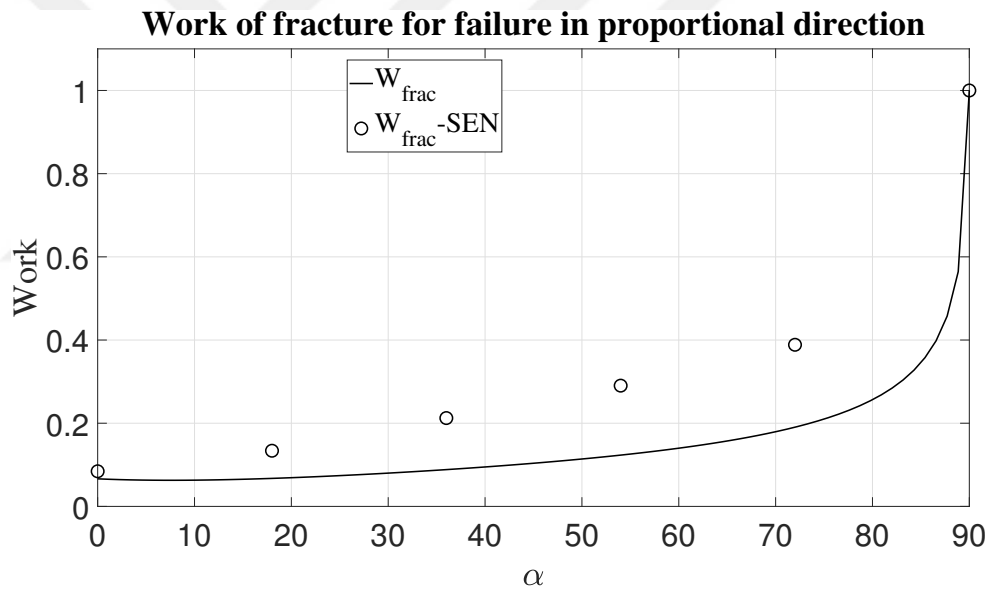
Figure 4.50: Comparison of fracture energy for SEN specimen and single material point tests.
