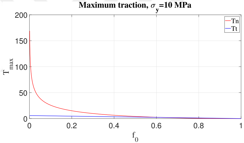
Figure 4.47: Maximum traction depending on f_0 .
