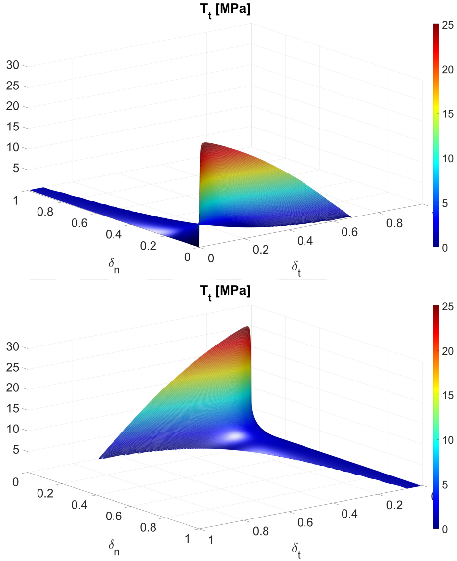
Figure 3.14: Tangential traction surface for proportional loading from different view angles. MBCZM model parameters are: \sigma_y=50 MPa, h_0=0.1 mm, f_0=0.1 , l=1 mm, E_n=700 GPa, E_t=70 GPa
