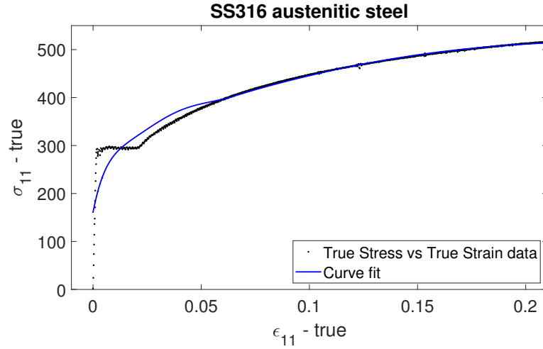
Figure 4.1: True stress-strain data for SS316LN steel.
