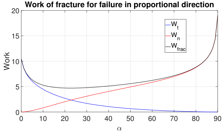
Figure 3.15: Work of fracture for proportional loading. MBCZM model parameters are: \sigma_y=50 MPa, h_0=0.1 mm, f_0=0.1 , l=1 mm, E_n=700 GPa, E_t=70 GPa
