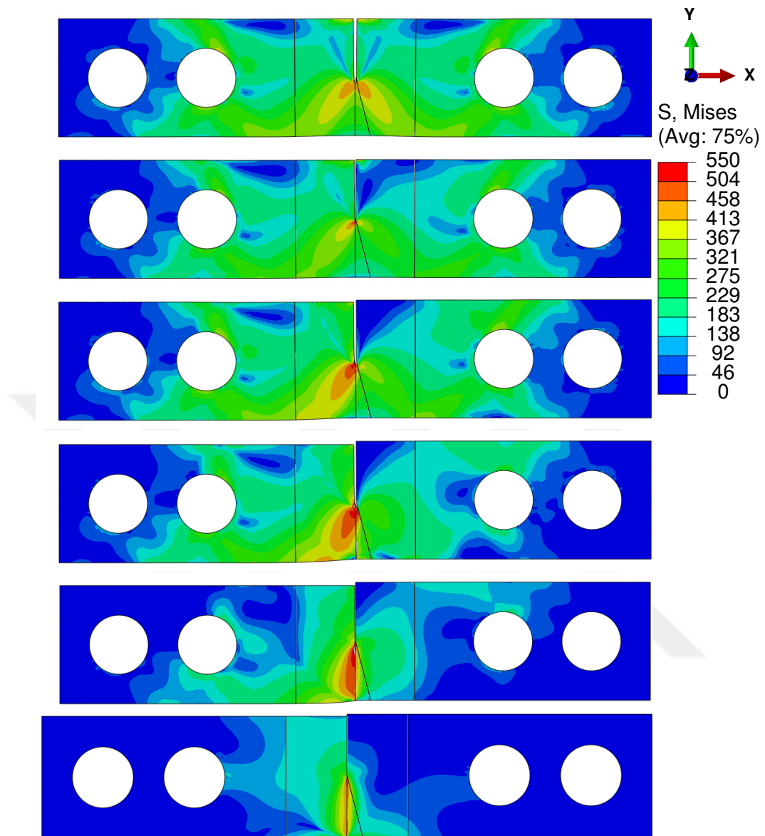
Figure 4.55: Von Mises stress just before softening for different loading holes in SEN specimen. From top to bottom holes 1 to 6 are used.
