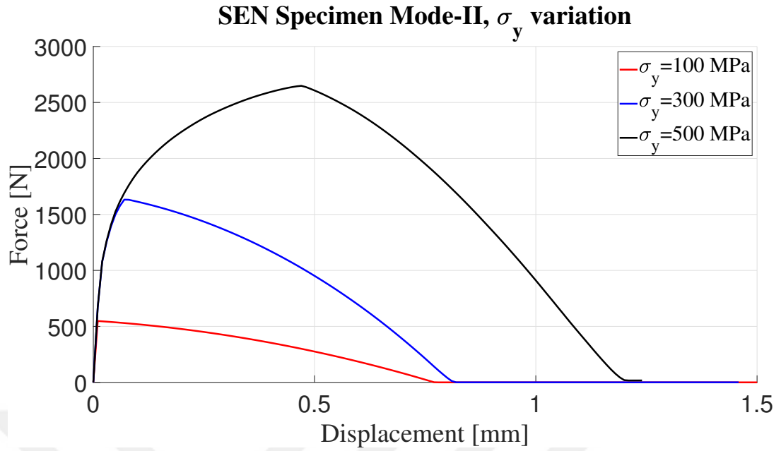
Figure 4.39: Force displacement response under mode-II loading for changing yield stress, \sigma_y .
