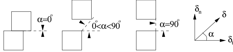
Figure 3.12: Proportional loading of cohesive element where \alpha is proportionality ratio.
