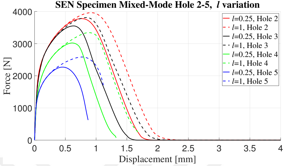
Figure 4.44: Force displacement response under mixed-mode loading for changing pore spacing, l .
