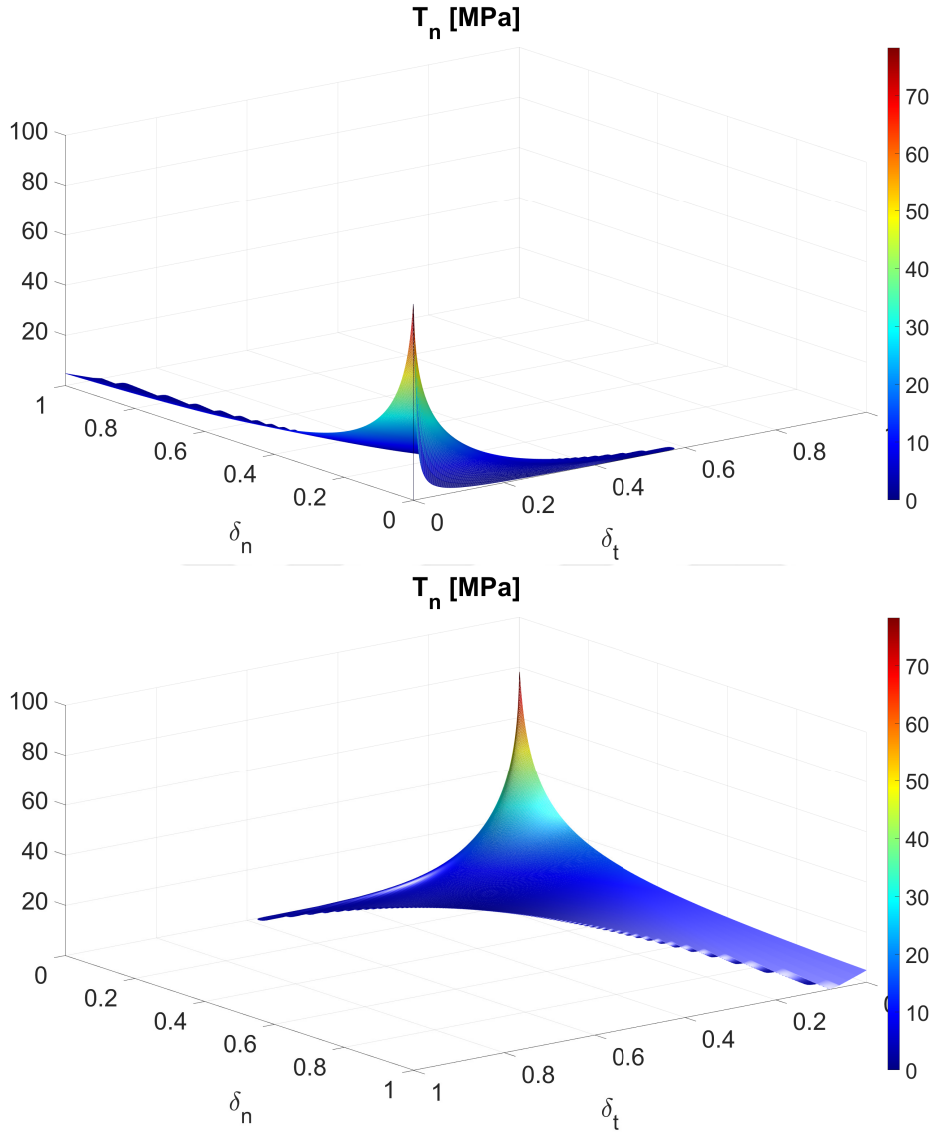
Figure 3.13: Normal traction surface for proportional loading from different view angles. MBCZM model parameters are: \sigma_y=50 MPa, h_0=0.1 mm, f_0=0.1 , l=1 mm, E_n=700 GPa, E_t=70 GPa
