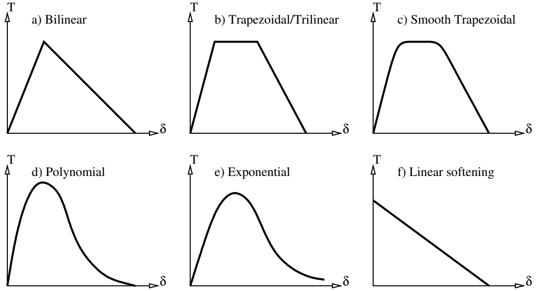
Figure 1.3: Some common types of traction-separation laws. Bilinear (a), trapezoidal (b), smooth trapezoidal (c), polynomial (d), exponential (e), linear softening (f).
