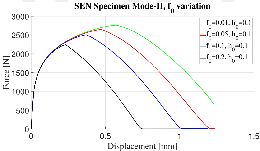
Figure 4.29: Force displacement response under mode-II loading for changing initial pore fraction, f_0 .
