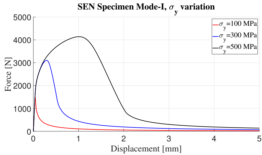
Figure 4.27: Force displacement response under mode-I loading for changing yield stress, \sigma_y .
