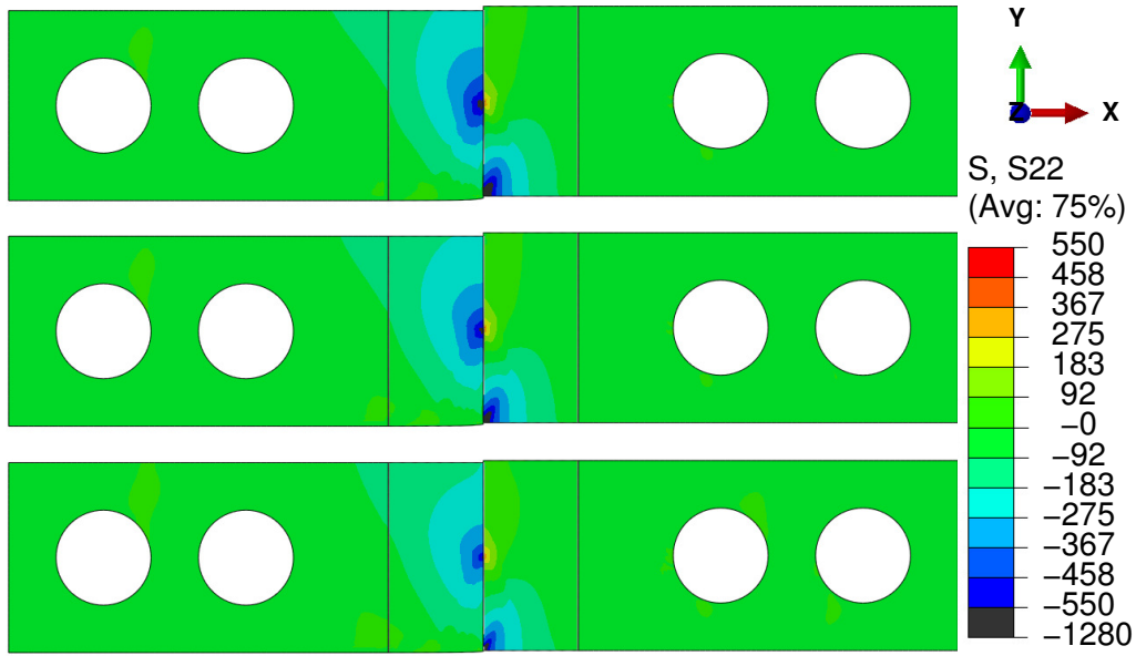
Figure 4.31: S_{yy} stress component, just before softening begins. f_0 's are equal to: 0.05 (top), 0.1 (middle), 0.2 (bottom).
