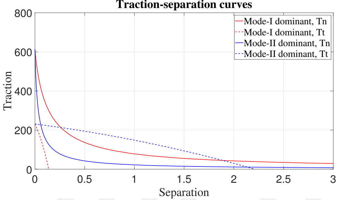
Figure 4.45: Traction separation curves for parameters in Table 4.3.
