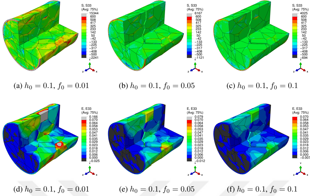
Figure 5.5: Contour plots for the stress ( \sigma_{zz} ) (a, b, c) and strain ( \epsilon_{zz} ) (d, e, f) at 5% global strain for different initial pore fractions, f_0 = 0.01 (a, d), f_0 = 0.05 (b, e), f_0 = 0.1 (c, f).
