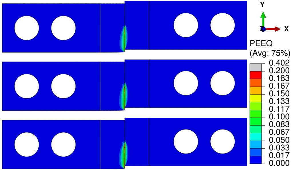
Figure 4.37: Equivalent plastic strain after failure. l 's are equal to: 0.25 (top), 0.5 (middle), 1 (bottom).
