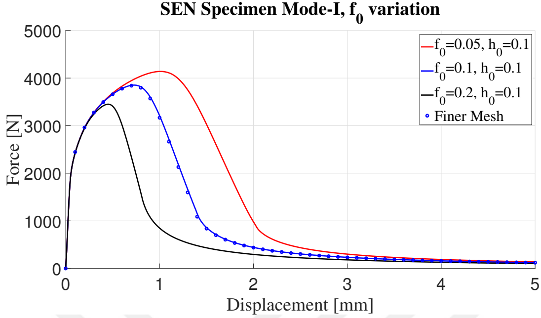
Figure 4.18: Force displacement response under mode-I loading for changing initial pore fraction, f_0 .
