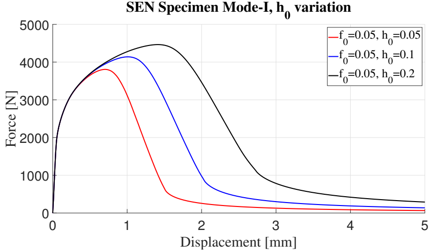
Figure 4.23: Force displacement response under mode-I loading for changing initial pore height, h_0 .
