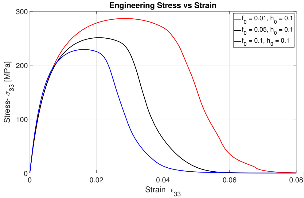
Figure 5.3: Engineering stress vs. strain response of a polycrystalline cylindrical specimen with 25\mu\text{m} diameter and 25\mu\text{m} length including 100 grains deformed under tensile loading for variable initial pore fraction, f_0 and constant initial pore height, h_0 .
