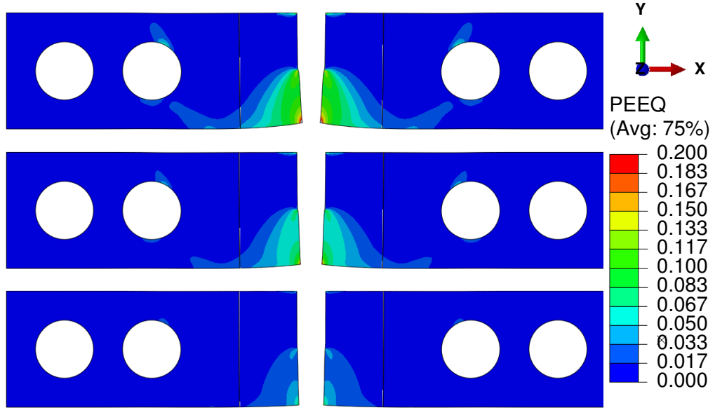
Figure 4.19: Equivalent plastic strain after failure. f_0 's are equal to: 0.05 (top), 0.1 (middle), 0.2 (bottom).
