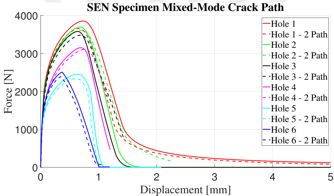
Figure 4.54: Force displacement response for loading through different holes. Straight lines represent 1 crack path model, and dotted lines are for 2 crack paths model.
