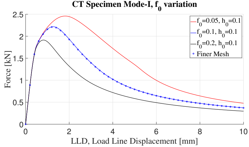
Figure 4.4: Force-LLD response for constant h_0 , and changing f_0 .
