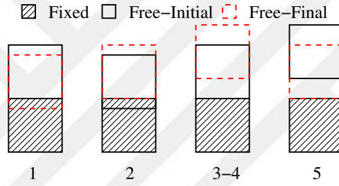
Figure 3.4: Mode-I loading history.
