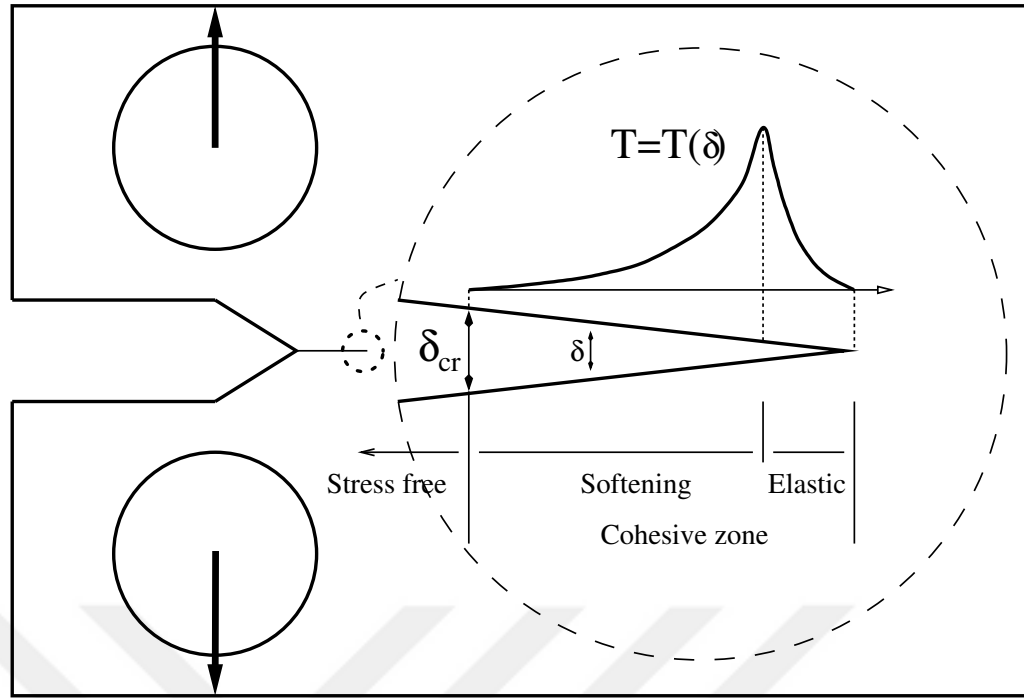
Figure 1.1: Cohesive zone concept at the crack tip. Traction of crack surfaces, T , is a function of crack face separation, \delta .
