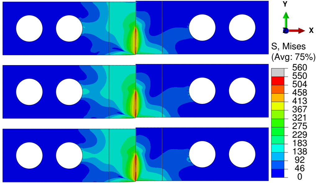
Figure 4.36: Von Mises stress contours just before softening begins. l 's are equal to: 0.25 (top), 0.5 (middle), 1 (bottom).
