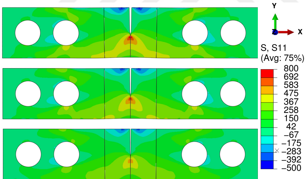
Figure 4.21: S_{xx} stress component, just before softening begins. f_0 's are equal to: 0.05 (top), 0.1 (middle), 0.2 (bottom).
