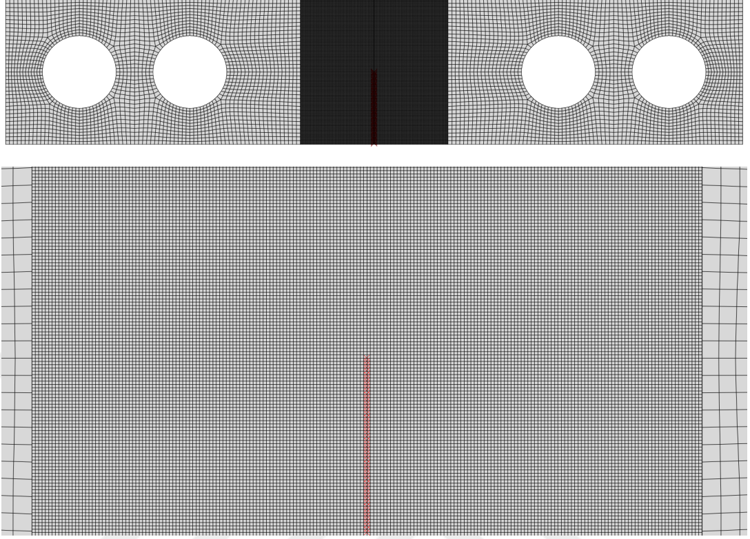
Figure 4.17: Mesh of the SEN specimen and close-up view of crack tip region.
