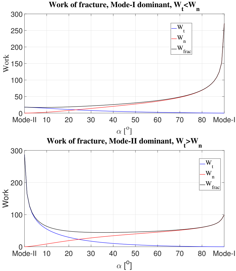
Figure 4.48: Work of fracture depending on loading angle \alpha , for mode-I dominant set (top) and mode-II dominant set (bottom).
