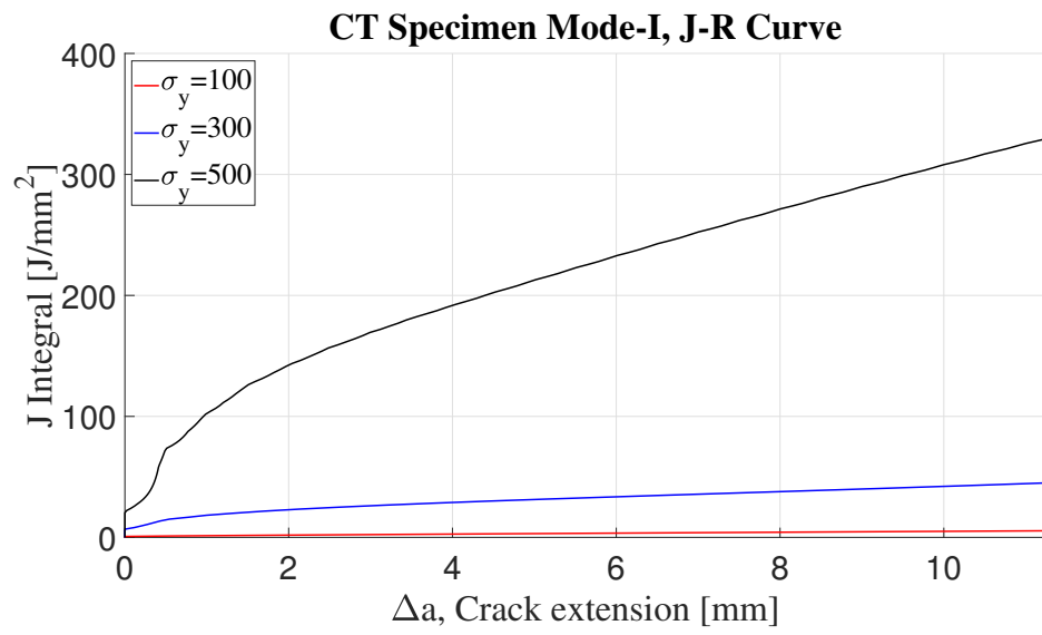
Figure 4.13: J-R curve changing \sigma_y .
