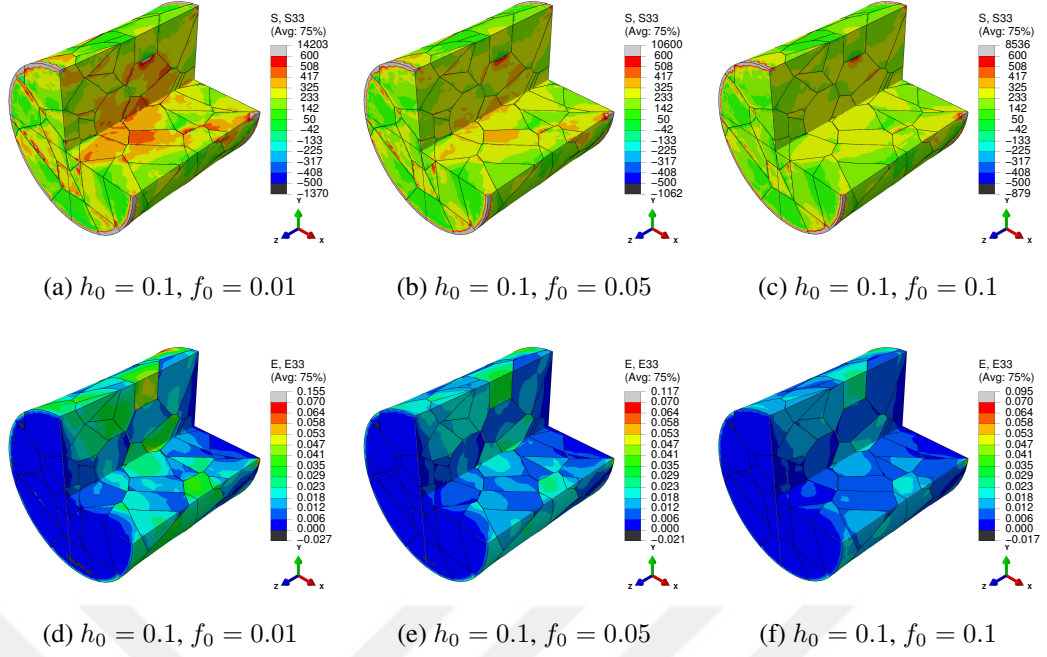
Figure 5.4: Contour plots for the stress ( \sigma_{zz} ) (a, b, c) and strain ( \varepsilon_{zz} ) (d, e, f) at the peak engineering stress increment in for different initial pore fractions, f_0 = 0.01 (a, d), f_0 = 0.05 (b, e), f_0 = 0.1 (c, f).
