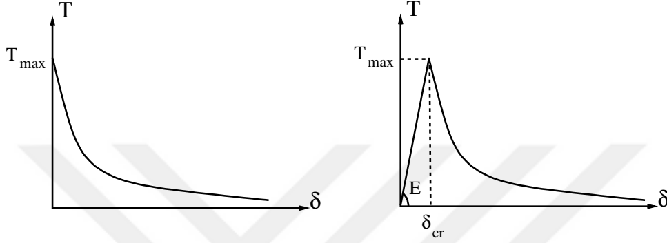
Figure 3.2: Initially rigid (extrinsic) and initially elastic (intrinsic) traction separation laws.
