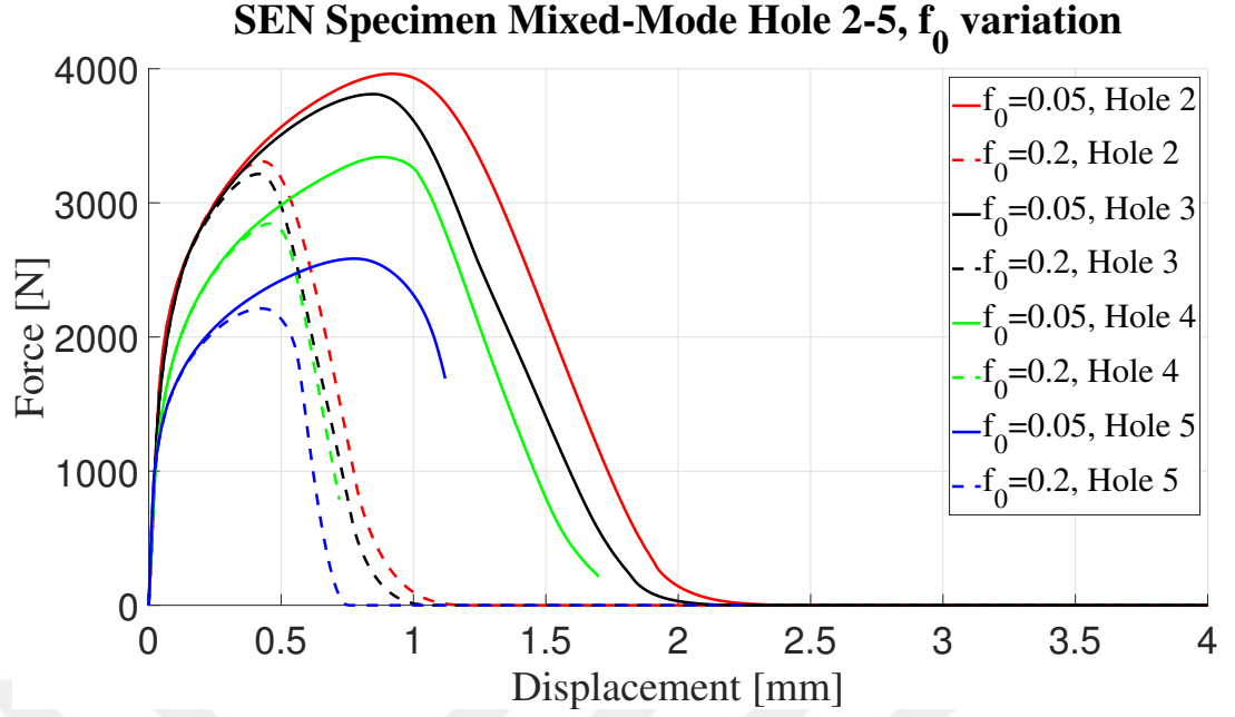
Figure 4.42: Force displacement response under mixed-mode loading for changing initial pore fraction, f_0 .
