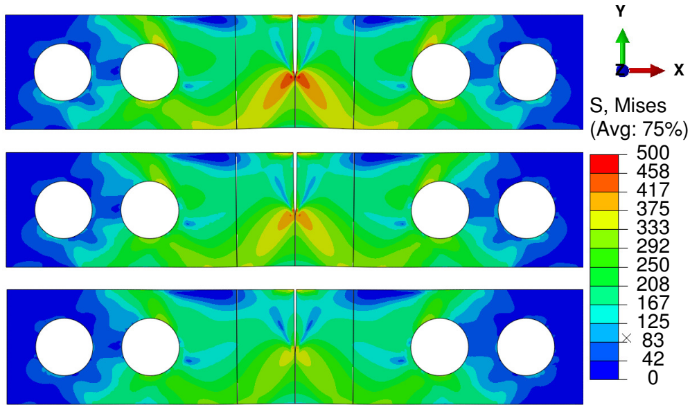
Figure 4.20: Von Mises stress contours just before softening begins. f_0 's are equal to: 0.05 (top), 0.1 (middle), 0.2 (bottom).
