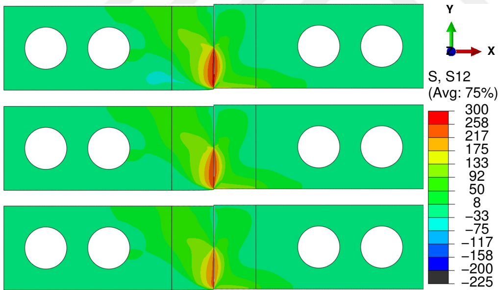
Figure 4.32: S_{xy} stress component, just before softening begins. f_0 's are equal to: 0.05 (top), 0.1 (middle), 0.2 (bottom).
