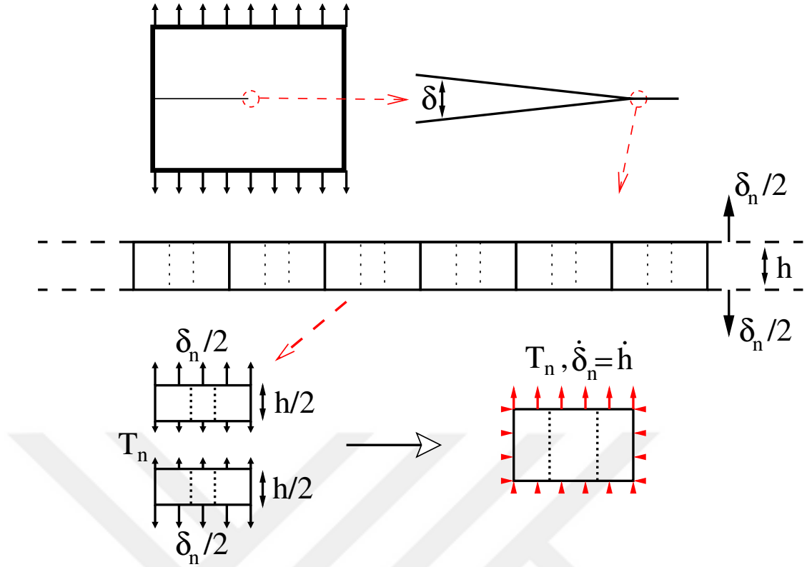
Figure 2.2: Crack opening represented by RVEs under mode-I loading.
