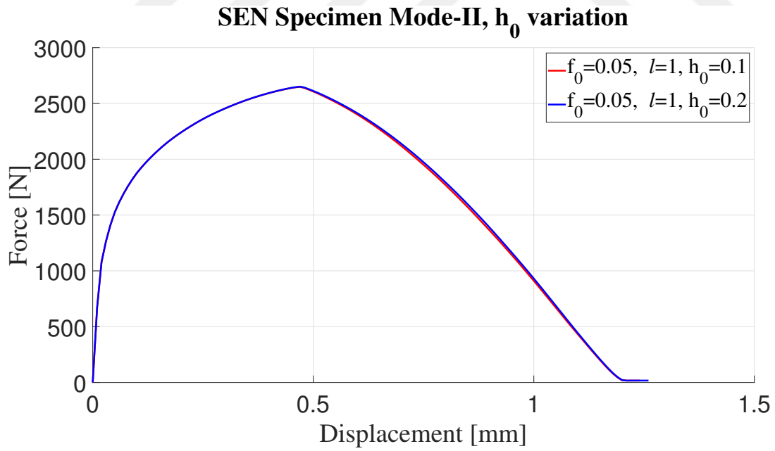
Figure 4.38: Force displacement response under mode-II loading for changing initial pore fraction, h_0 .
