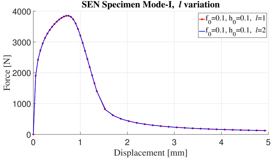
Figure 4.26: Force displacement response under mode-I loading for changing pore spacing, l .
