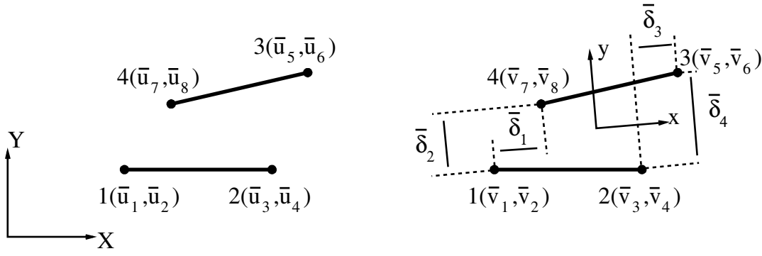
Figure 3.1: 2D linear cohesive surface element and nodal displacements in the global (left) and the local (right) coordinates.
