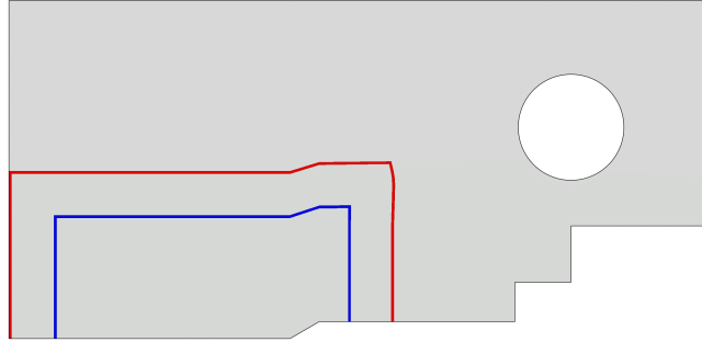
Figure 4.9: Paths used to calculate J integral. Innermost (blue) and outermost (red) paths are shown in the figure.
