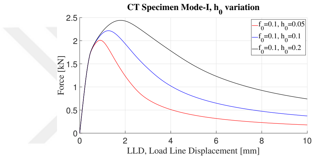
Figure 4.7: Force-LLD response for constant f_0 , and changing h_0 .
