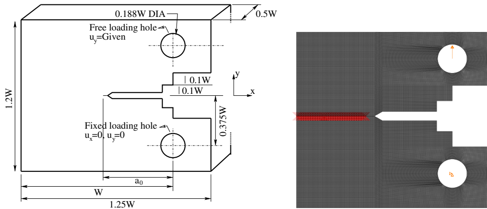
Figure 4.2: ASTM-E1820 CT Specimen and the FE model with W = 100mm .
