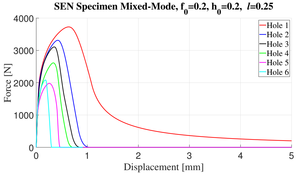
Figure 4.49: Force displacement response for loading through different holes.
