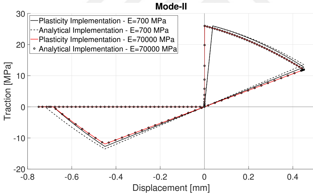
Figure 3.11: Traction versus displacement response to mode-II loading/unloading using mixed-mode implementation.
