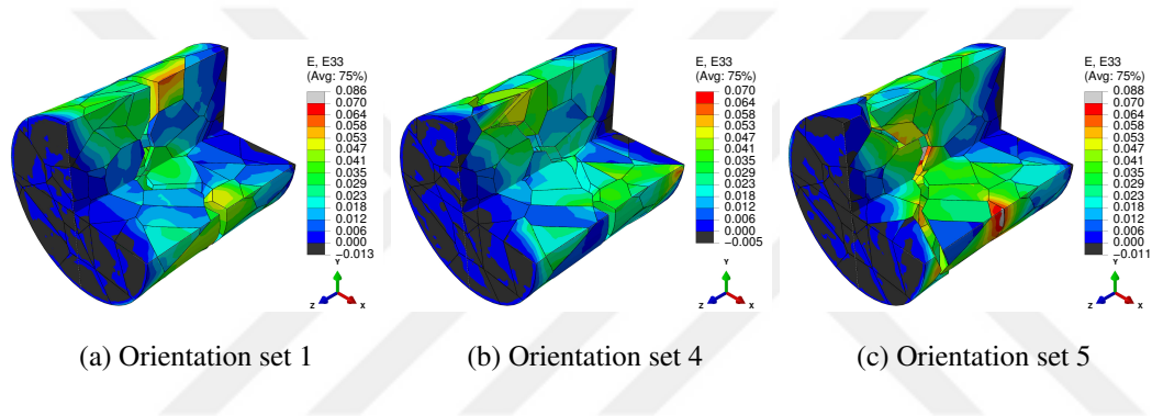
Figure 5.7: Contour plots for the strain ( \varepsilon_{zz} ) at 8% global strain level for different orientation sets: set 1 (a), set 4 (b), and set 5 (c).
