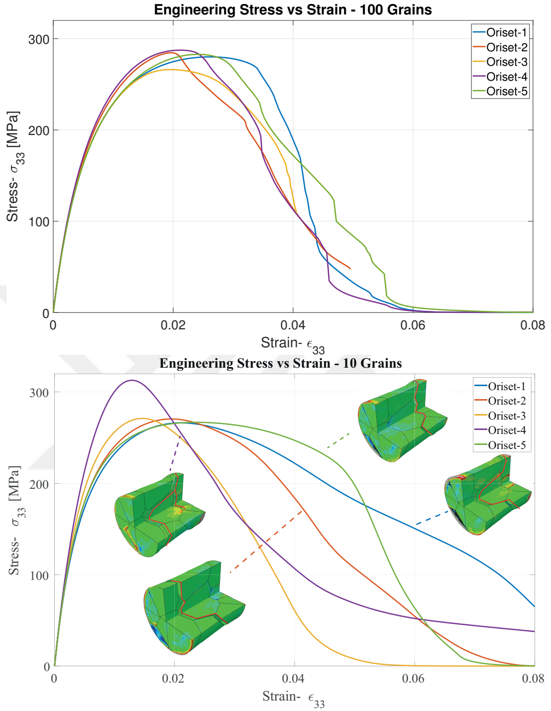
Figure 5.6: Engineering stress vs strain response of a polycrystalline cylindrical specimen with 25\mu\text{m} diameter and 25\mu\text{m} length including 100 grains (top) and 10 grains (bottom), deformed under tensile loading for different sets of randomly generated grain orientations.
