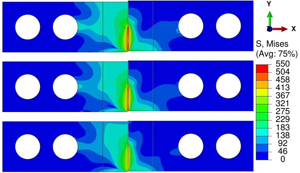
Figure 4.30: Von Mises stress contours just before softening begins. f_0 's are equal to: 0.05 (top), 0.1 (middle), 0.2 (bottom).
