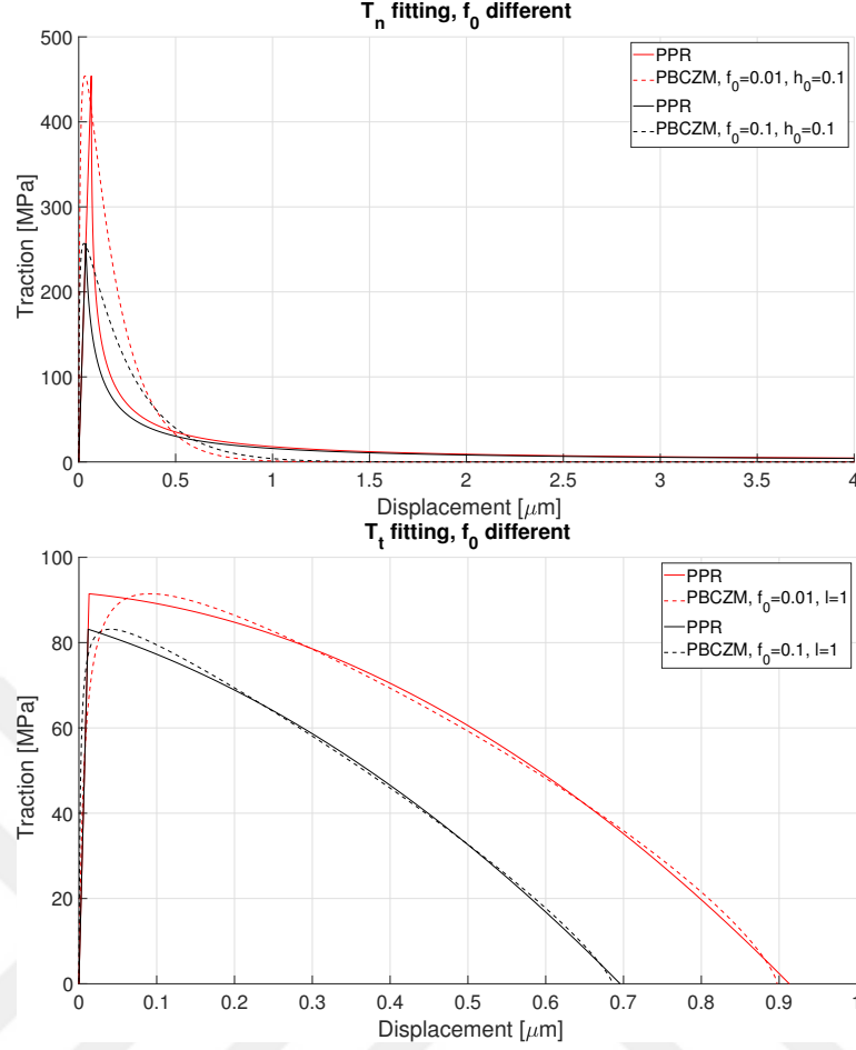
Figure 5.2: Comparison of PPR and MBCZM traction-separation laws after fitting for mode-I (top) and mode-II (bottom).
