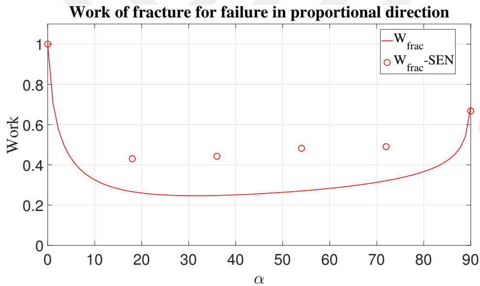
Figure 4.52: Comparison of fracture energy for SEN specimen and single material point tests.
