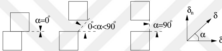
Figure 4.41: Proportional loading of cohesive element where \alpha is proportionality ratio.
