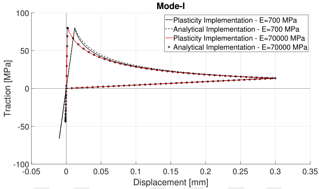
Figure 3.10: Traction versus displacement response to mode-I loading/unloading using mixed-mode implementation.
