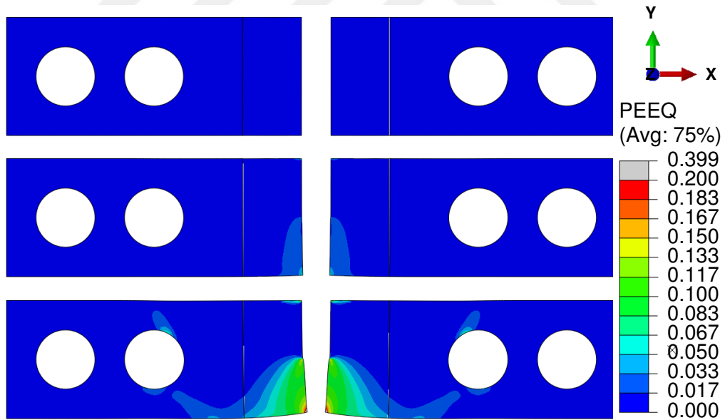
Figure 4.28: Equivalent plastic strain after failure. \sigma_y 's are equal to: 100 MPa (top), 300 MPa (middle), 500 MPa (bottom).
