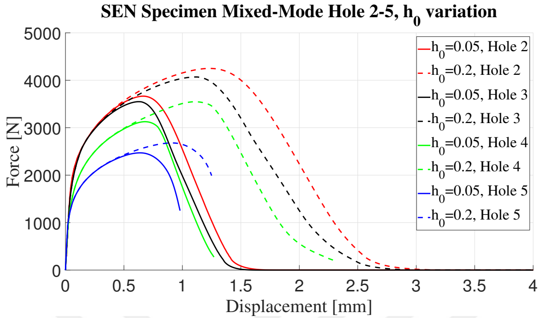
Figure 4.43: Force displacement response under mixed-mode loading for changing initial pore height, h_0 .
