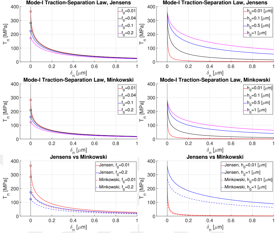
Figure 2.3: Dependence of Mode-I traction-separation law on initial volume fraction and height of voids for \sigma_y = 100 MPa and h_0 = 0.2\mu m (left) and f_0 = 0.01 (right), by using Jensen's inequality (top) and Minkowski inequality (middle), and a comparison of them (bottom).
