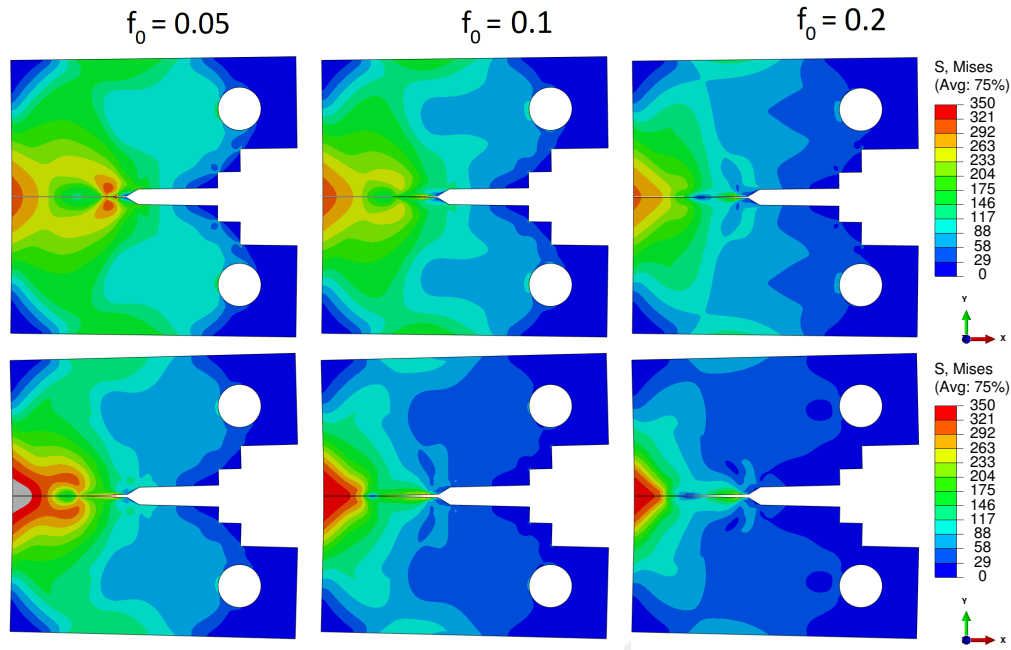
Figure 4.5: Stress distributions at the same time increment for different initial pore fractions. Load line displacement is 2 mm (top) and 4 mm (bottom).
