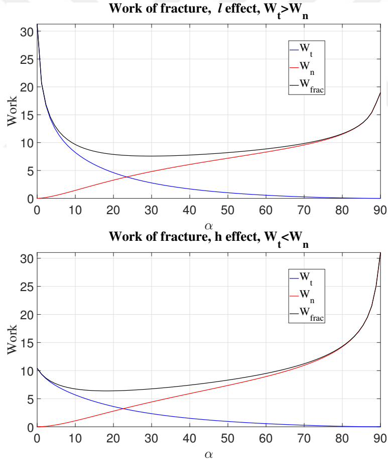
Figure 3.16: Effect of h and l is shown on work of fracture. h_0 = 0.1\text{mm} , l = 3\text{mm} (top), h_0 = 0.2\text{mm} , l = 1\text{mm} (bottom)
