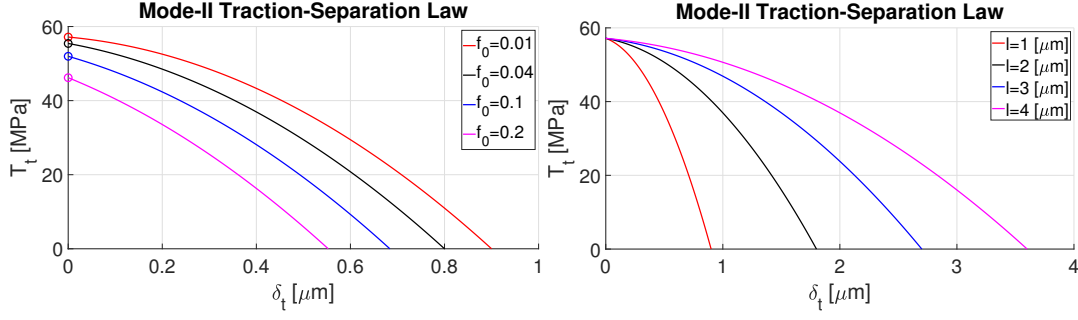
Figure 2.6: Mode-II traction-separation equation for \sigma_y = 100 MPa and l = 1\mu m with changing f_0 (left), and f_0 = 0.01 with changing l (right).
