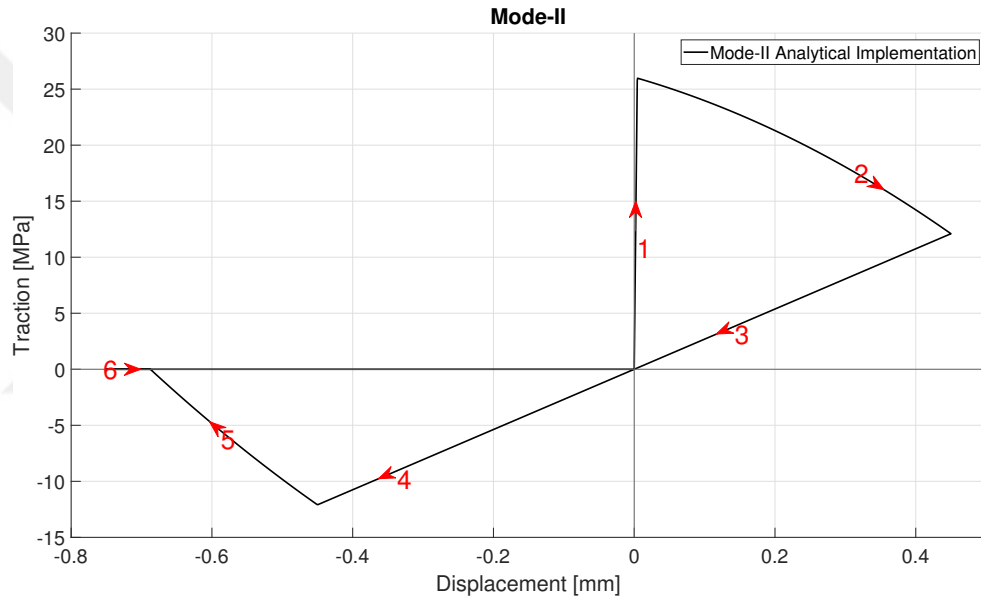
Figure 3.7: Traction versus displacement response to mode-II loading/unloading.
