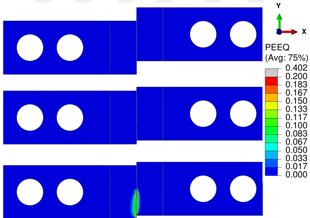
Figure 4.40: Equivalent plastic strain after failure. \sigma_y 's are equal to: 100 MPa (top), 300 MPa (middle), 500 MPa (bottom).
