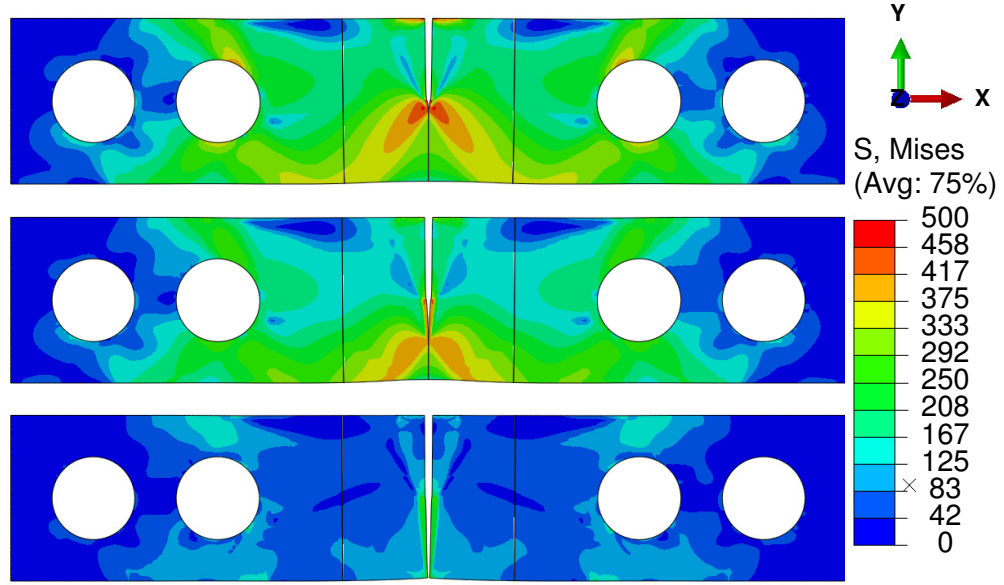
Figure 4.22: Von Mises stress at the same displacement, 1mm . f_0 's are equal to: 0.05 (top), 0.1 (middle), 0.2 (bottom).
