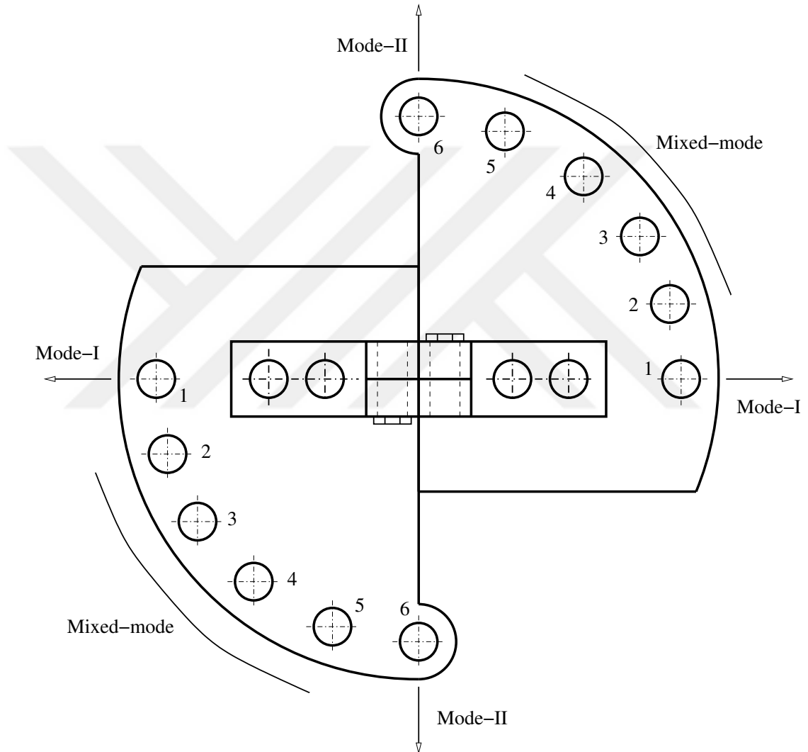
Figure 4.15: Test apparatus used to load SEN specimen with mode-I, mode-II and mixed-mode loading [4].
