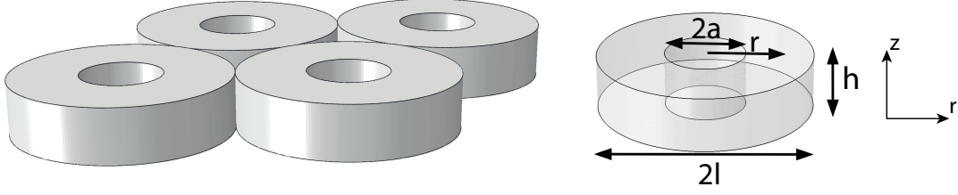
Figure 2.1: Idealization of pores within a plane as cylinders and dimensions of the RVE.
