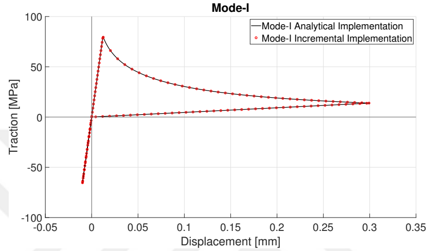
Figure 3.8: Traction versus displacement response to mode-I loading/unloading for incremental and analytical model.
