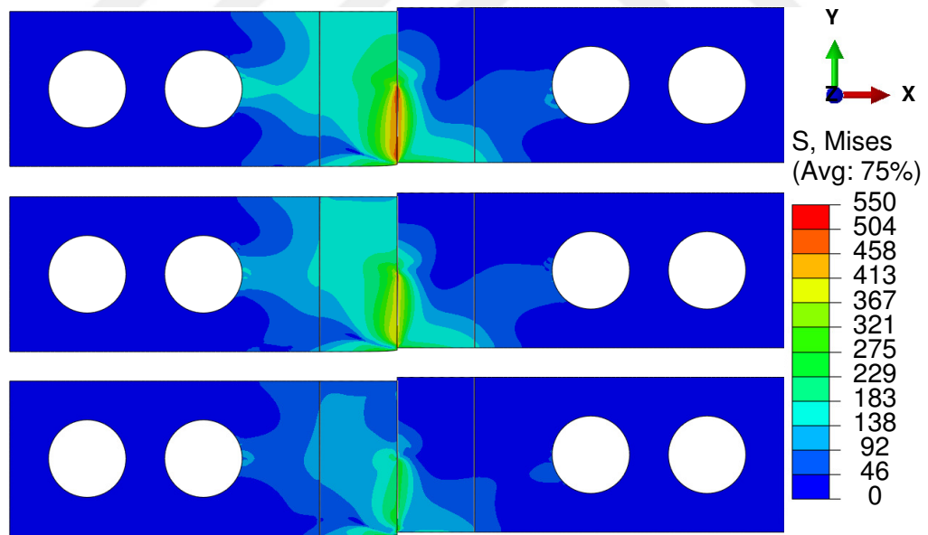
Figure 4.34: Von Mises stress at the same displacement, 0.5mm. f_0 's are equal to: 0.05 (top), 0.1 (middle), 0.2 (bottom).
