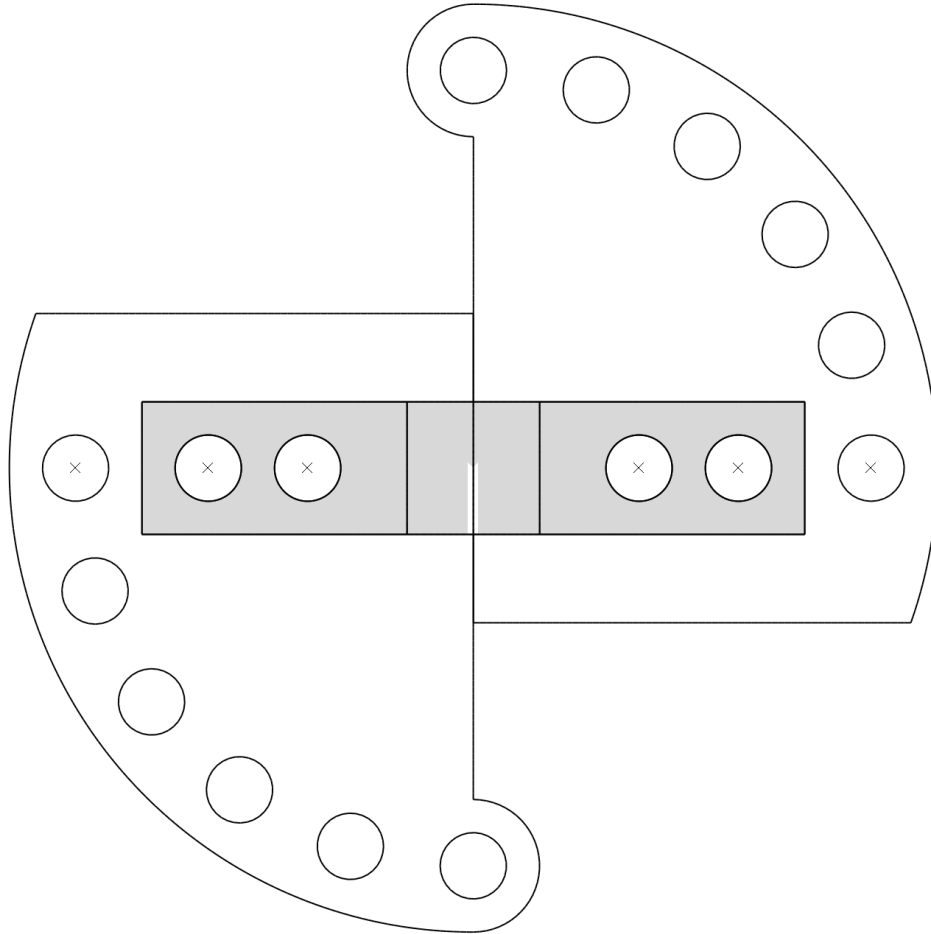
Figure 4.16: FE model of the test apparatus in Fig. 4.15.
