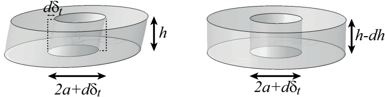
Figure 2.5: Geometry change under shear loading.
