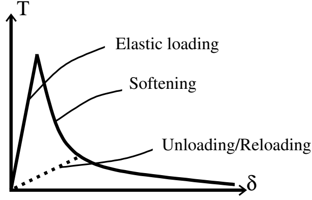
Figure 3.3: Regions of traction-separation law.
