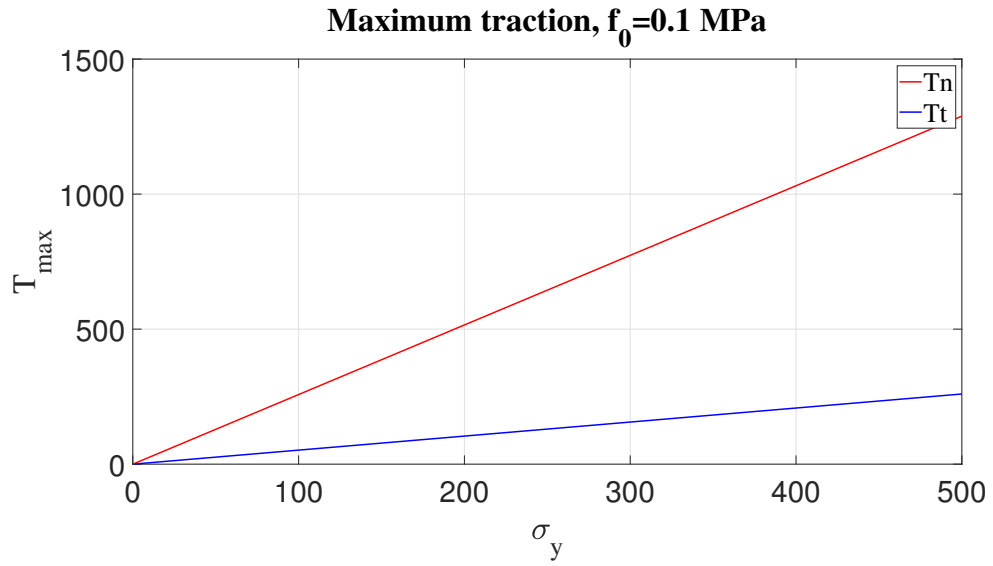
Figure 4.46: Maximum traction depending on \sigma_y .
