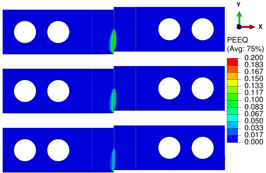
Figure 4.33: Equivalent plastic strain after failure. f_0 's are equal to: 0.05 (top), 0.1 (middle), 0.2 (bottom).
