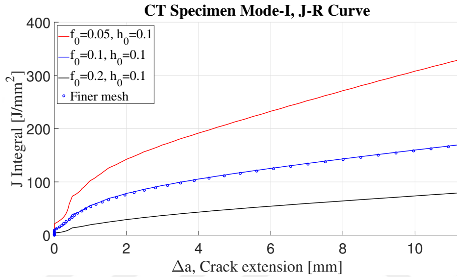
Figure 4.11: J-R curve for constant h_0 , and changing f_0 .
