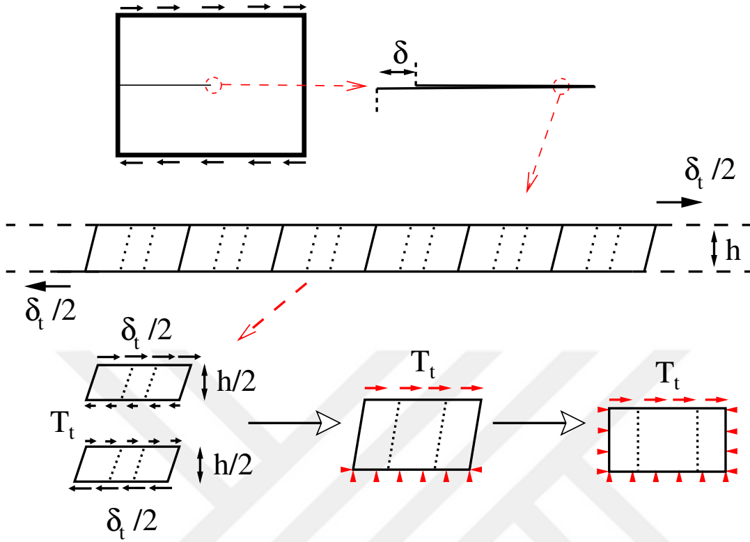
Figure 2.4: Crack opening represented by RVEs under mode-I loading.
