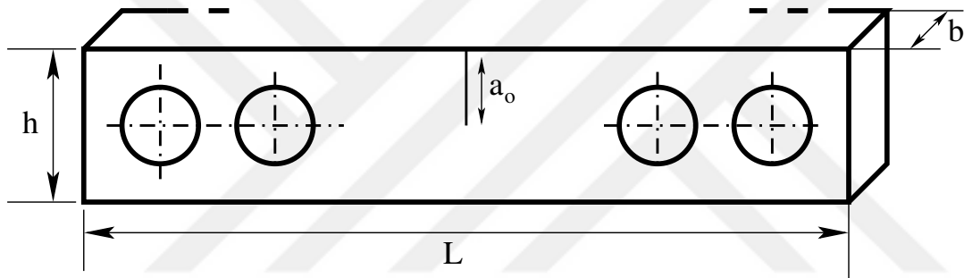
Figure 4.14: Single edge notch (SEN) specimen geometry.
