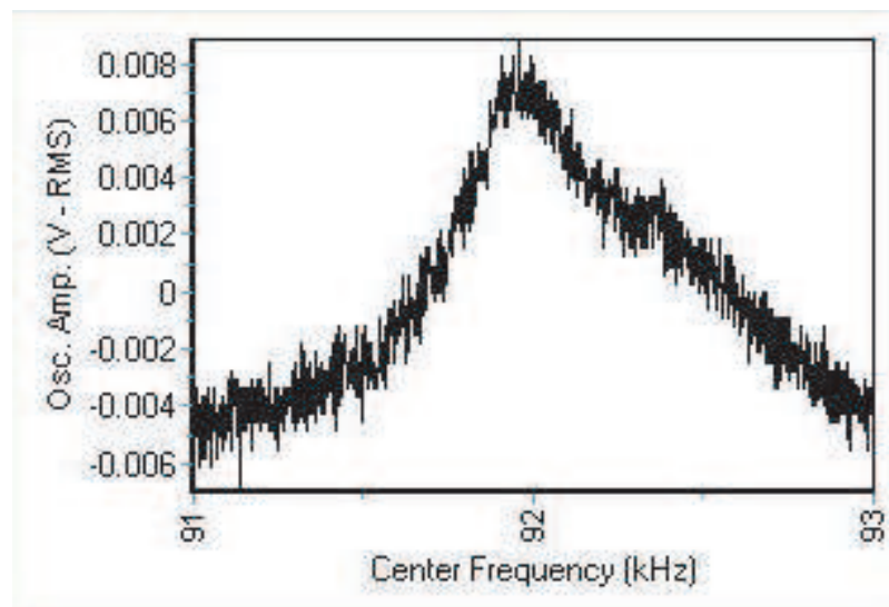
Figure 4.15: The measured resonance curve for SOI cantilever#3
