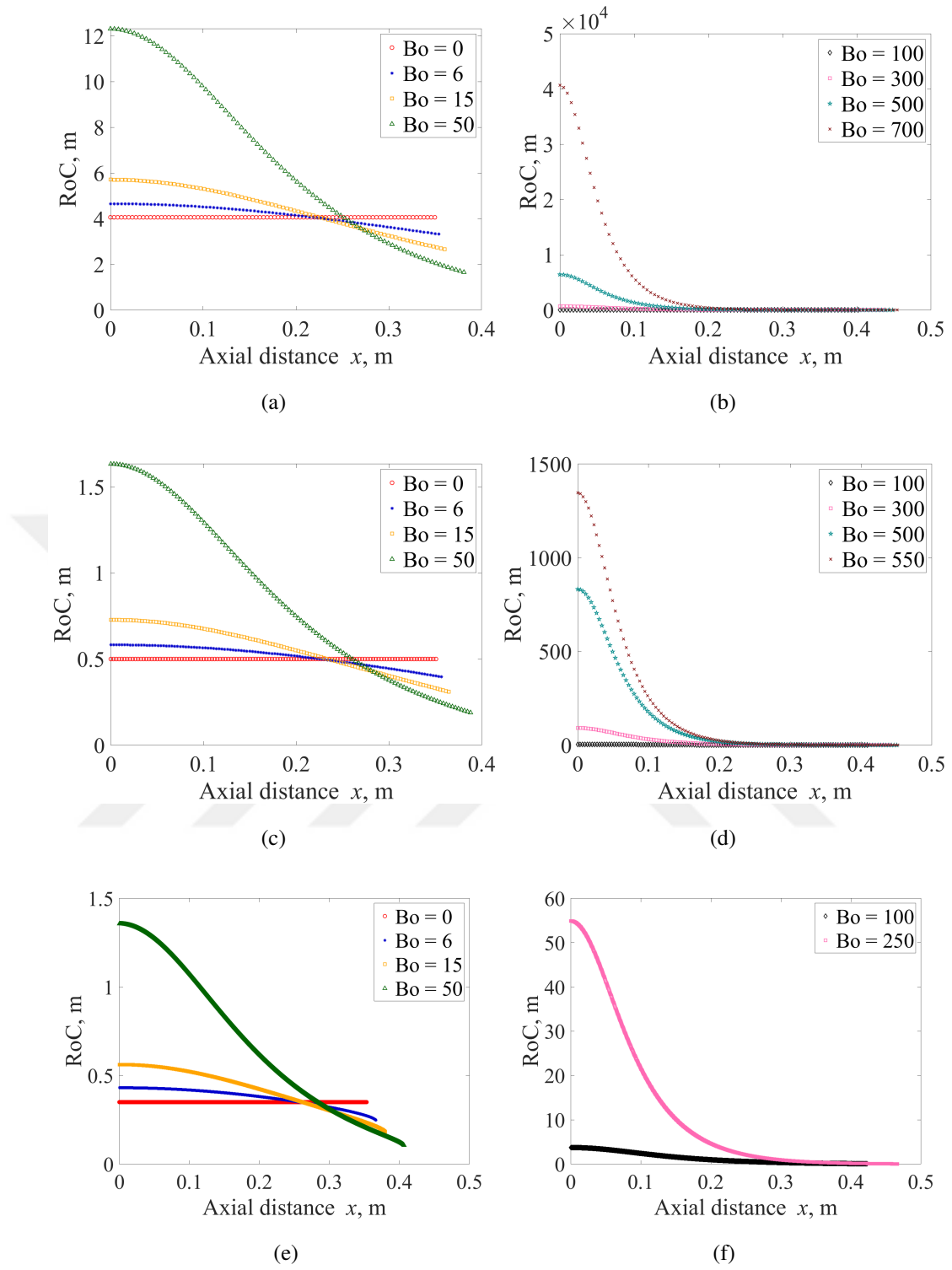
Figure 4.20: Non-dimensional analysis on the effect of Bond number to the radius of curvature values of droplets having different contact angles (a) First set of results for \alpha = 5^\circ , (b) Second set of results for \alpha = 5^\circ , (c) First set of results for \alpha = 45^\circ , (d) Second set of results for \alpha = 45^\circ , (e) First set of results for \alpha = 85^\circ , (f) Second set of results for \alpha = 85^\circ
