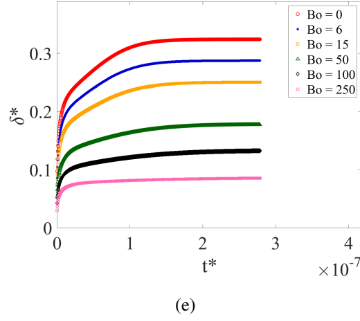
Figure 4.18: Non-dimensional analysis on the effect of Bond number to the bridge heights of droplets having different contact angles (a) \alpha = 5^\circ , (b) \alpha = 25^\circ , (c) \alpha = 45^\circ , (d) \alpha = 65^\circ , (e) \alpha = 85^\circ
