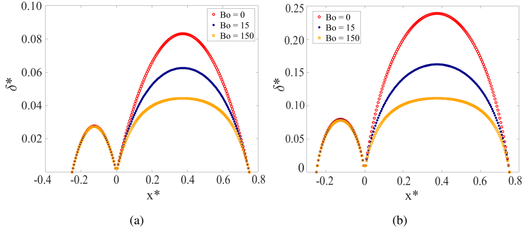
Figure 4.31: Effect of the Bond number on droplets having 1 : 3 initial length ratios. Initial droplet profiles for (a) contact angle \alpha = 25^\circ and (b) contact angle \alpha = 65^\circ .
