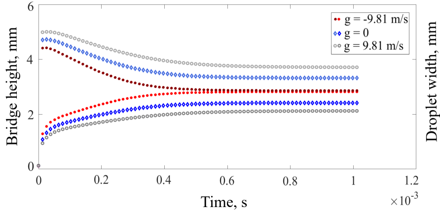
Figure 4.10: Bridge height and merged droplet size variation in time for water-copper pair with \alpha = 72^\circ . Decreasing trends represent the droplet size, while increasing lines are for the bridge height.
