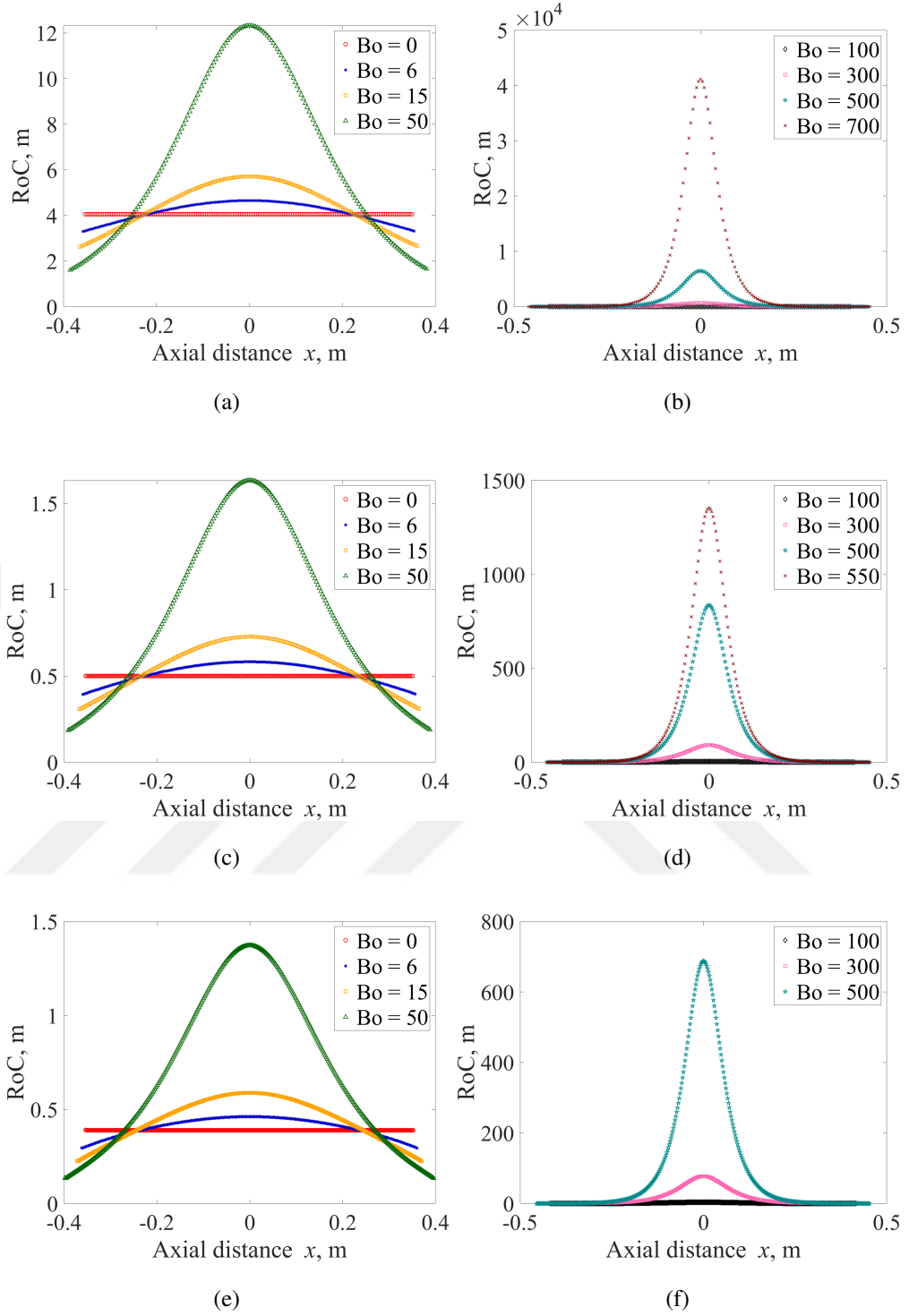
Figure 4.28: Non-dimensional analysis on the effect of Bond number to the radius of curvature values of droplets having different contact angles (a) First set of results for \alpha = 5^\circ , (b) Second set of results for \alpha = 5^\circ , (c) First set of results for \alpha = 45^\circ , (d) Second set of results for \alpha = 45^\circ , (e) First set of results for \alpha = 65^\circ , (f) Second set of results for \alpha = 65^\circ
