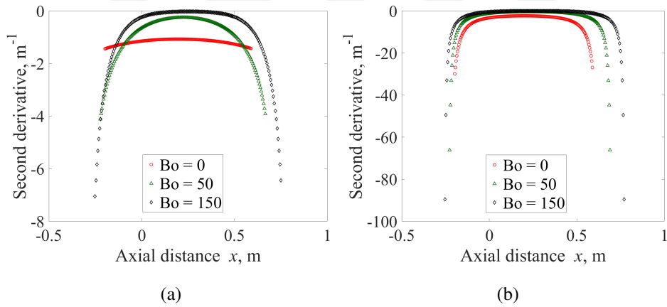
Figure 4.35: Non-dimensional analysis on the effect of Bond number to the second derivative values at the steady state. Results for (a) contact angle \alpha = 25^\circ , (b) contact angle \alpha = 65^\circ .
