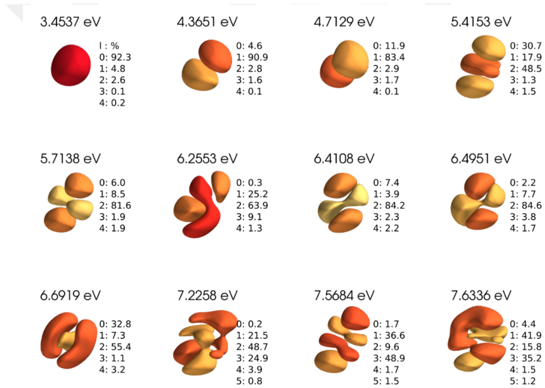
Figure 3.3: Conduction band wavefunction envelopes of freestanding hemispherical InAs QD with 10 nm diameter.
