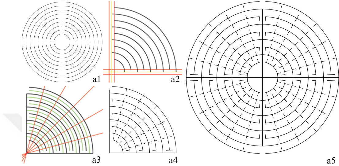
Figure 3.5: Plan drawings showing the phases of the WL design.
