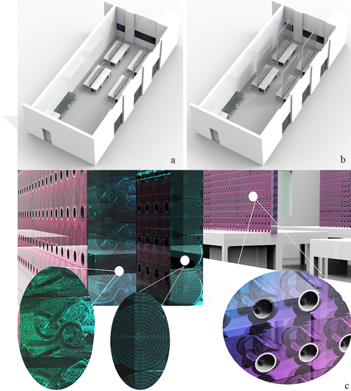
Figure 4.6: Studio#2 a) 3D Model with design proposal \frac{1}{5} height of the room AMM panels, b) with design proposal using \frac{3}{4} height of the room AMM panels, c) panels with DNA5 on one side and WL on the other, with a 7.5 cm gap in between, shown in Studio#1 and Studio#2.
