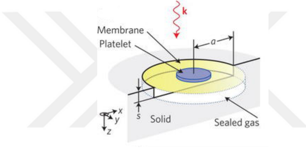
Figure 2.6: The schematic structure of the ultrathin membrane-type AMM (meta-surface) [6].
