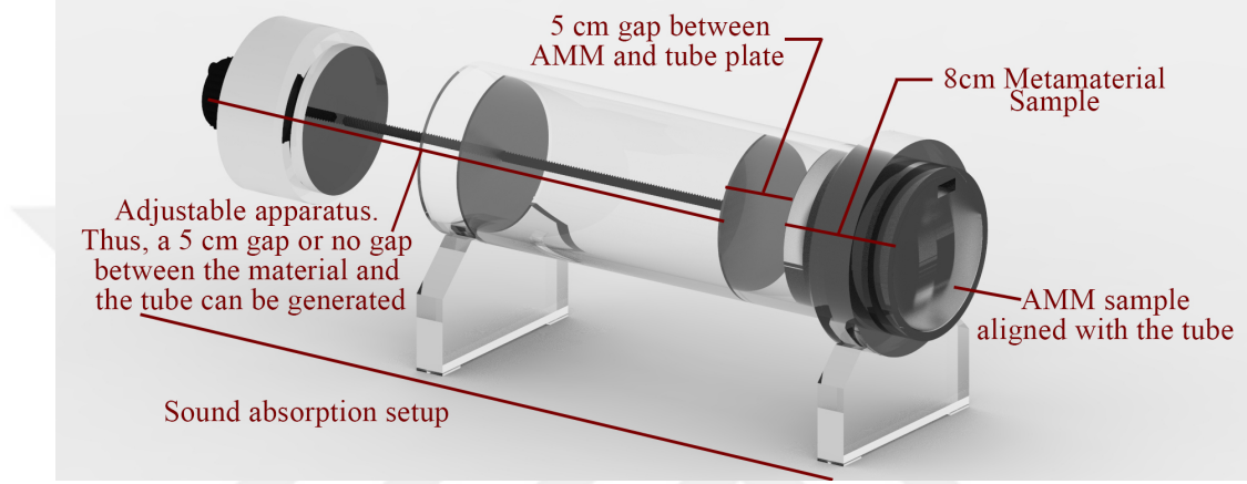
Figure 4.2: Sound absorption coefficient measurement set-up: abstracted 3D model of impedance tube indicating AMM sample locations under different configurations (prepared by the author).
