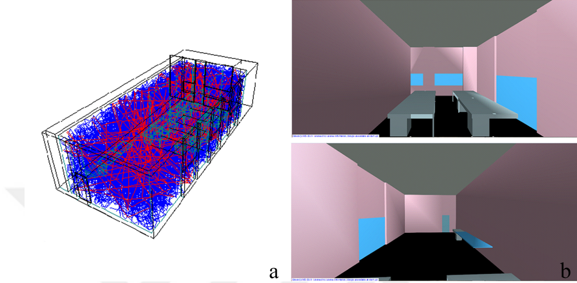
Figure 5.6: Studio#2 simulated-current situation: a) ray tracing acoustic simulation, b) 3D OpenGL views.
