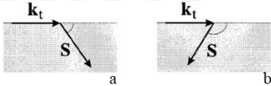
Figure 2.2: a) Positive refraction \mathbf{S} \cdot \mathbf{k}_t \geq 0 , b) negative refraction \mathbf{S} \cdot \mathbf{k}_t \leq 0 [2].
