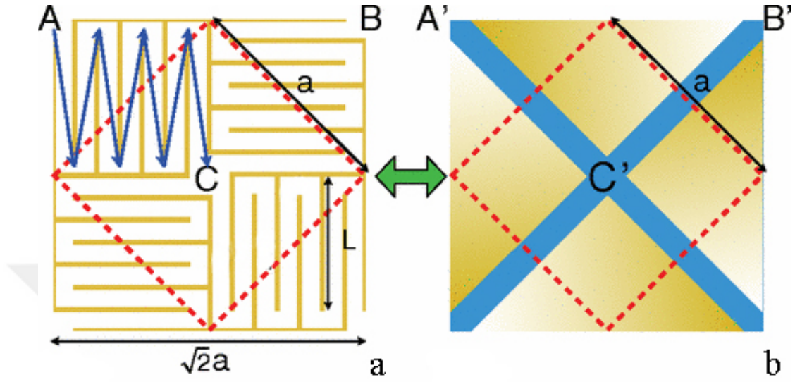
Figure 2.7: a) Schematic diagram of metamaterial-repeating units in coiling up space. The connected arrows show the zigzag path of the propagation of acoustic waves, b) the simplified view with straightened channels [7].
