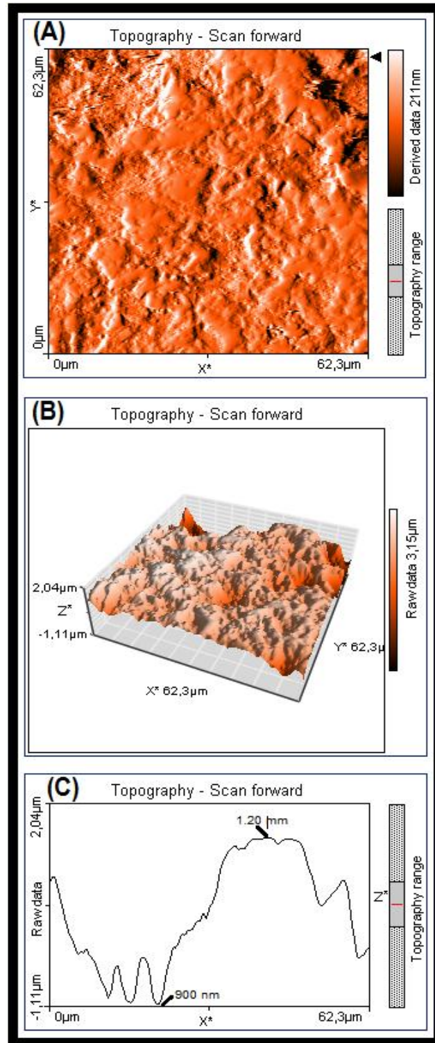
Figure 3.14 The atomic force microscope (AFM) micrographs were taken as two different 3-D (three-dimensional) morphologies (A) and (B), and one 2-D (two-dimensional) graphic (C) for Oltu-stone. The grain sizes of the matrix components display a libration with a minimum of 900 nm and a maximum of 1.2 \mu\text{m} .
