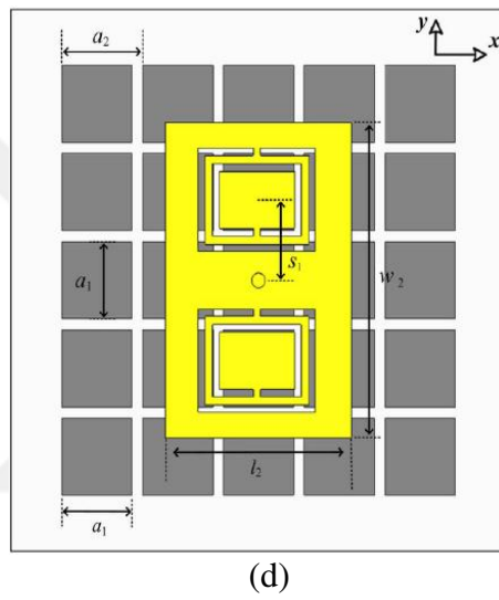
Figure 4.1 c) side view of [17], d) top view of [17], e) top view of current work
