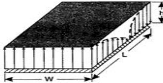
Figure 2.2 Distributed electric field into the microstripe cavity [32]
