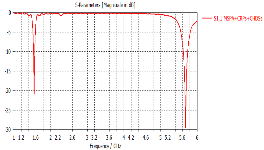
Figure 4.18 Return loss of complementary antenna (MSPA+CRPs+CHDSs)
