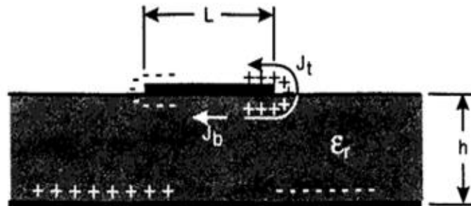
Figure 2.1 The streaming current density with spread of charges on MPA [32]
