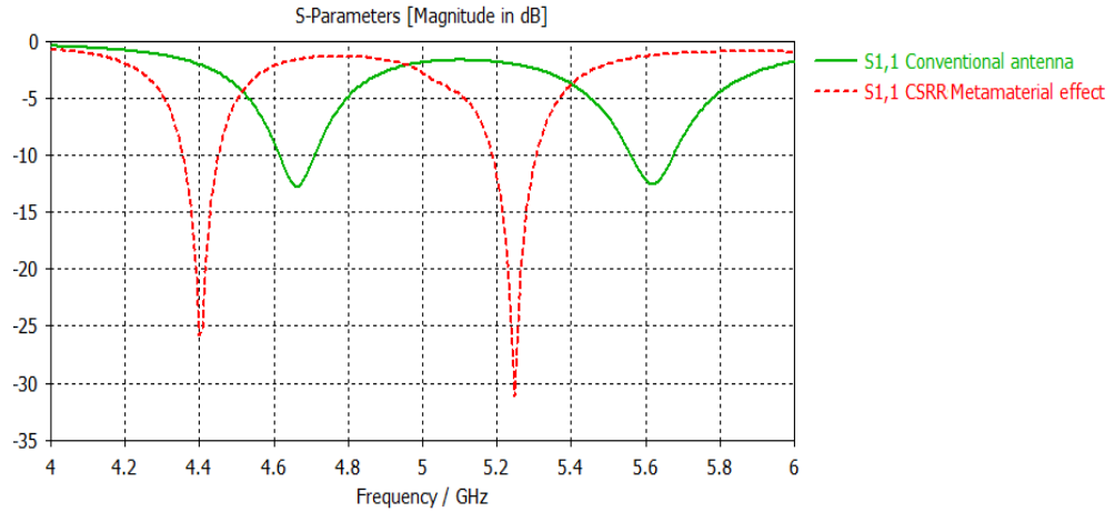
Figure 4.12 Comparison of return losses between conventional and CSRR antennas
