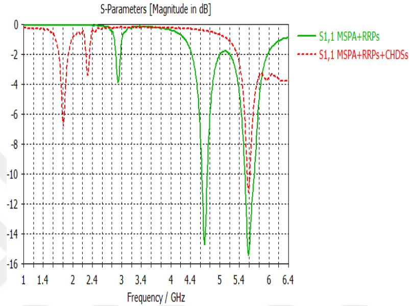
Figure 4.25 Comparison between the RRP antenna and the effect of CHDS behavior
