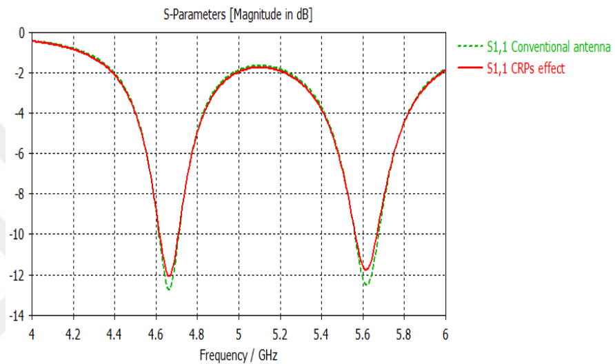
Figure 4.11 Comparison of return losses between MSPA and CRPs antenna
