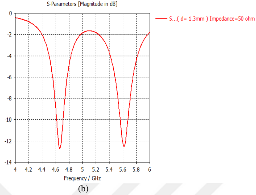
Figure 3.4 b) Return loss at matching impedance of 50 ohm and 1.3mm diameter
