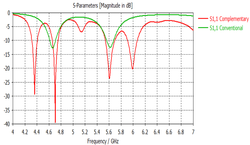
Figure 4.14 Return losses of complementary and conventional antennas
