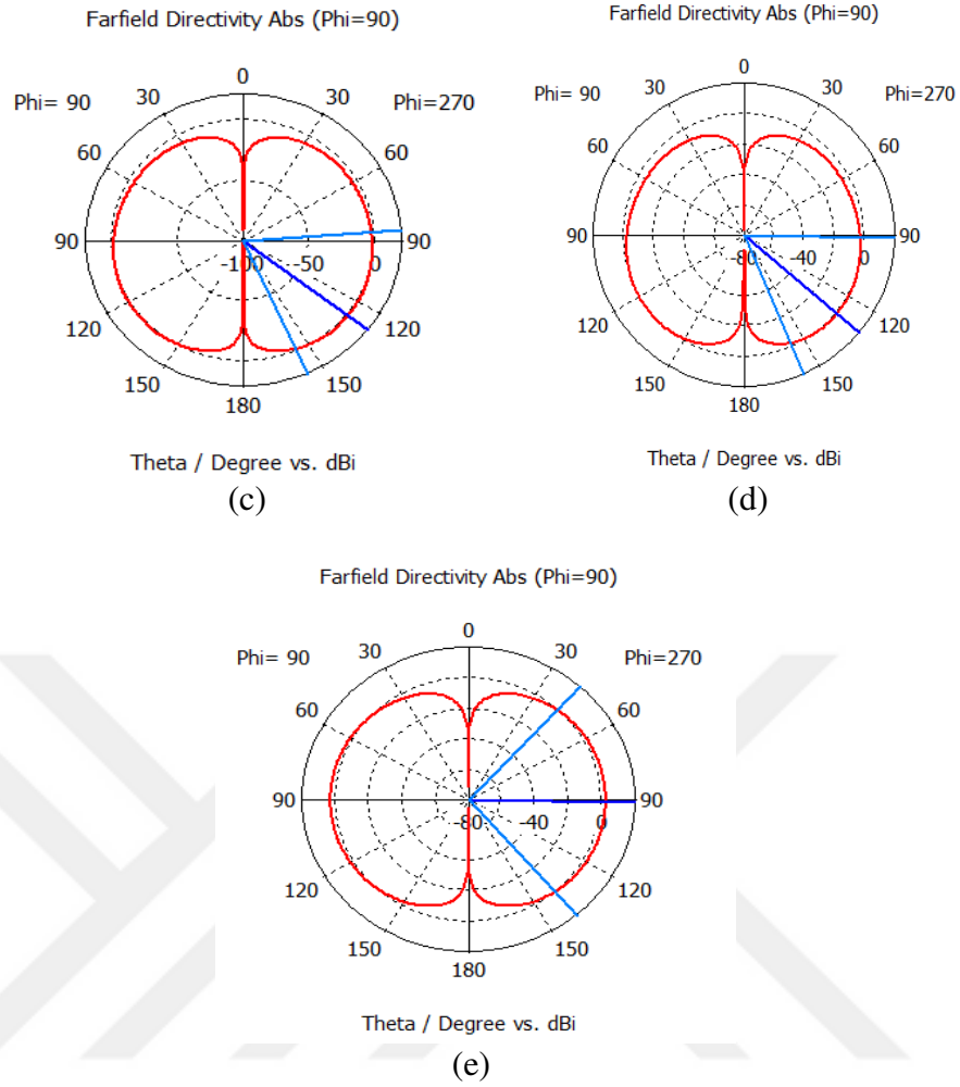
Figure 4.10 c) PP of MSPA at 5.61 GHz, d) PP of CP at 5.65 GHz, e) PP of CP at 2.65 GHz
