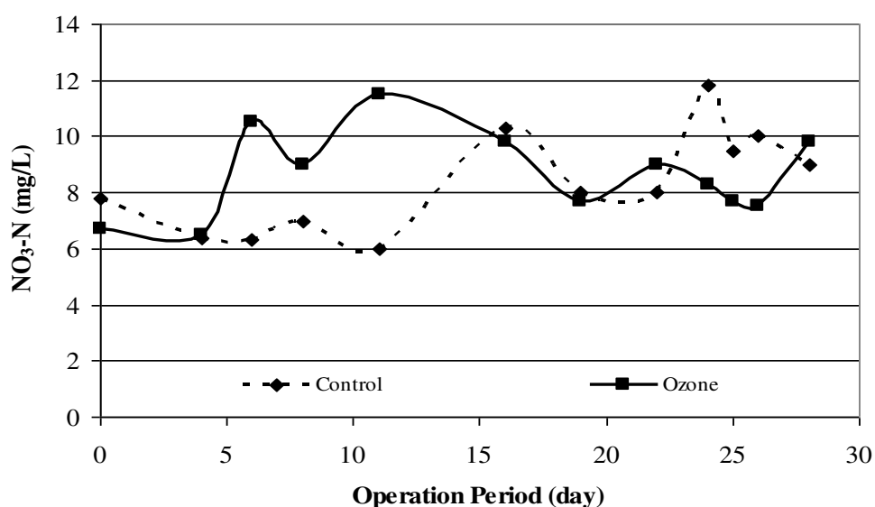
Figure 4.36 NO 3 concentration of effluent for control and ozone run
