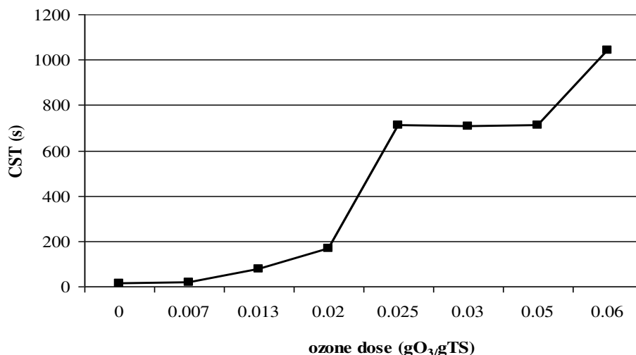
Figure 4.26 Changes of CST with different ozone doses
