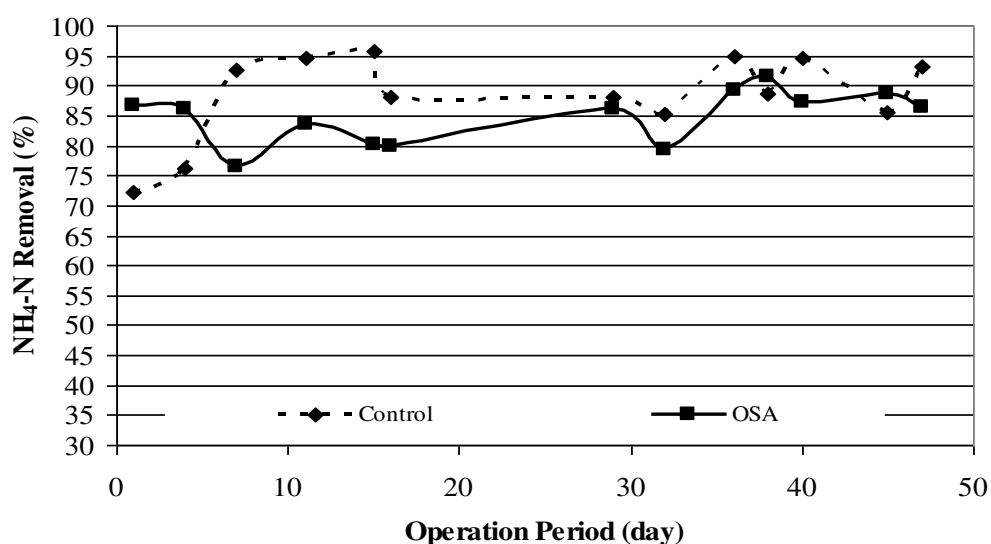
Figure 4.61 Changes of \text{NH}_4\text{-N} removal efficiencies (%) for OSA and control run
