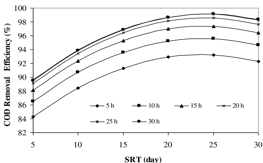
Figure 4.5 COD removal efficiencies versus SRT at different HRTs ( COD_i=500 mg/L)
