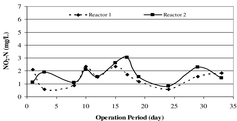
Figure 4.18 \text{NO}_2\text{-N} concentrations of effluent
