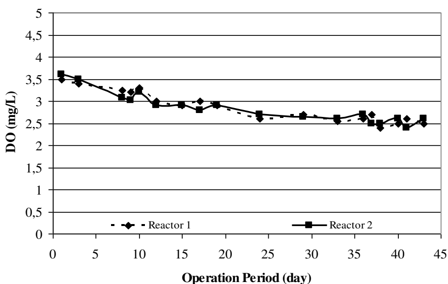
Figure 4.9 DO changes of aeration tanks
