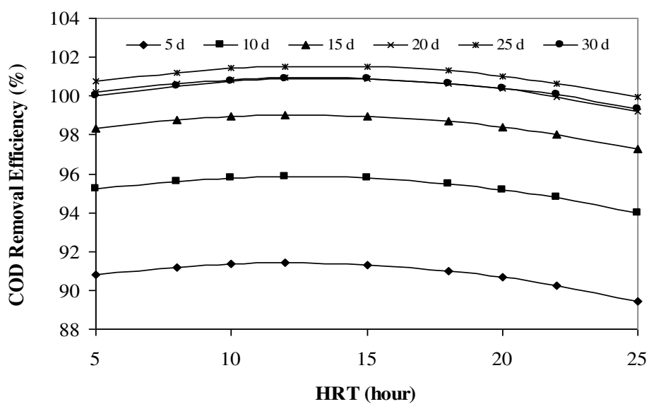
Figure 4.2 COD removal efficiencies versus HRT at different SRTs ( COD_i=300 mg/L)
