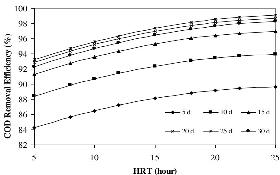
Figure 4.6 COD removal efficiencies versus HRT at different SRTs ( COD_i=500 mg/L)
