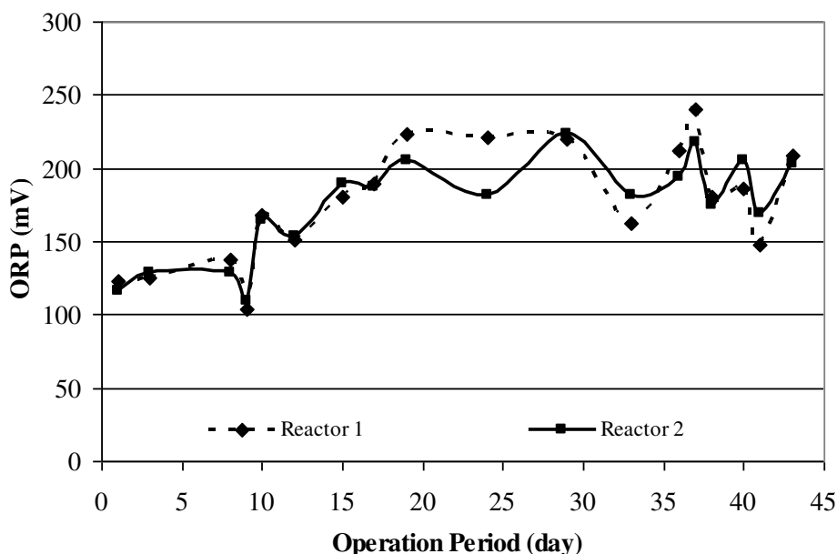
Figure 4.10 ORP changes of aeration tanks
