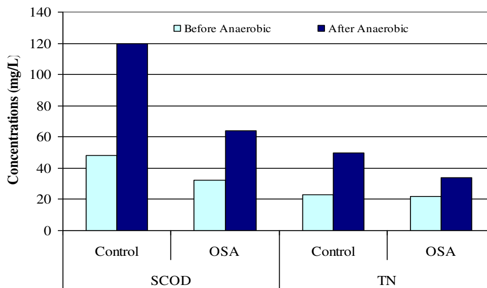
Figure 4.74 SCOD and TN concentrations of control and OSA batch experiment
