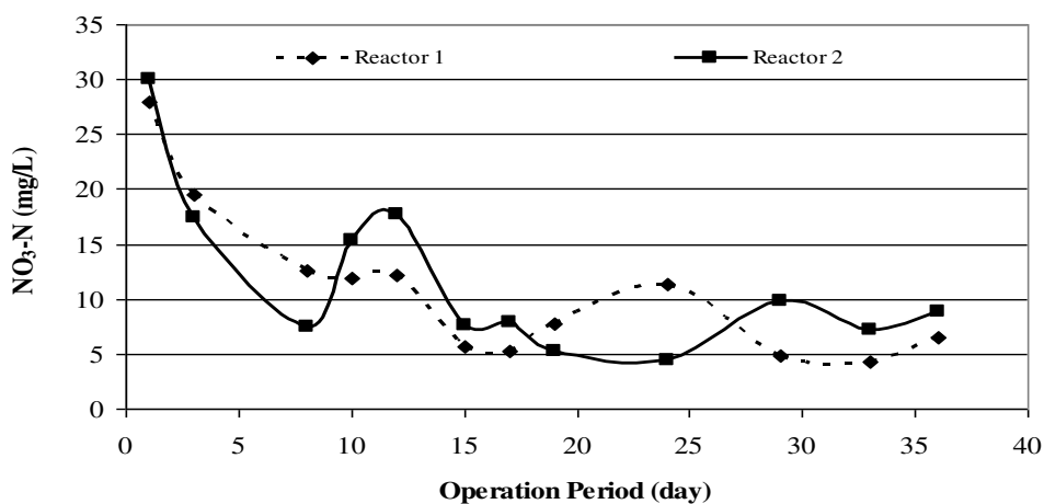
Figure 4.17 \text{NO}_3 concentrations of the effluent
