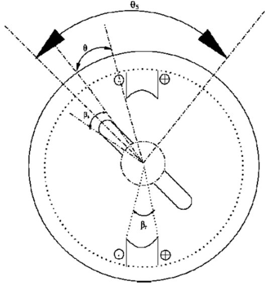
Fig. 2.4. Basic rotor position in a two pole SRM [40]
