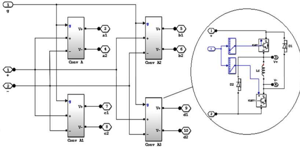
Fig. 4.14. Converter circuit
