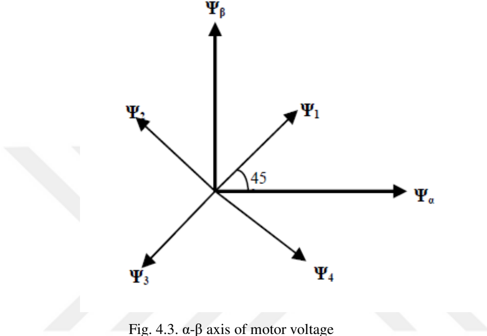
Fig. 4.3. \alpha - \beta axis of motor voltage
