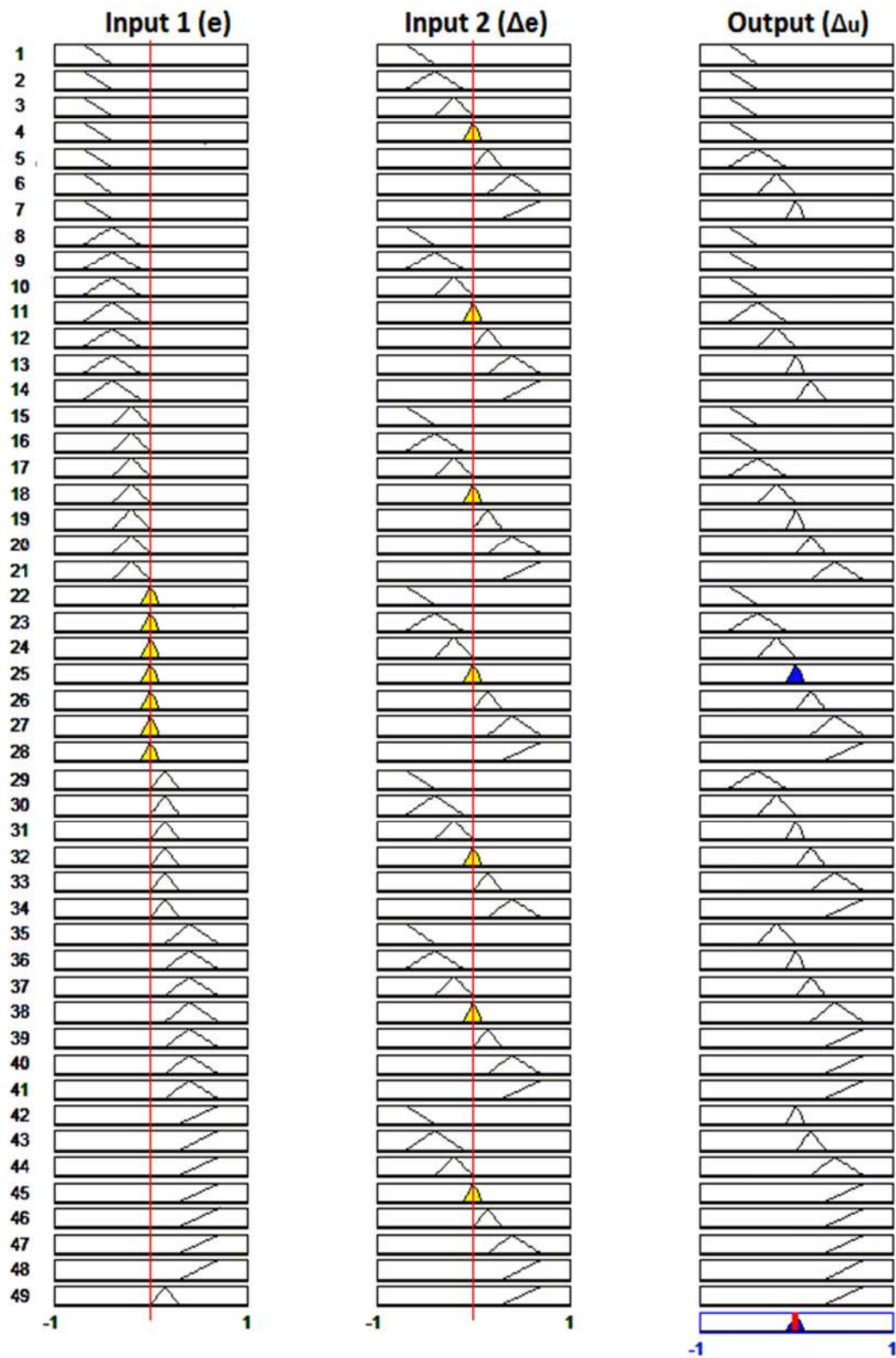
Fig. 4.12. Fuzzy Rules
