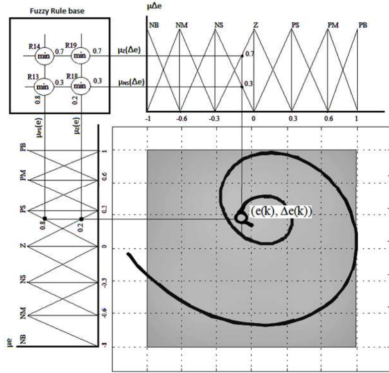
Fig. 4.9. Fuzzy reasoning
