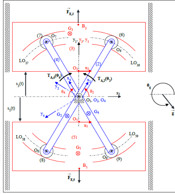
Figure 4.7. Schematic diagram of the TaR mechanism [3]
