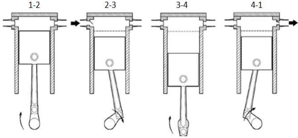
Figure 2.3. Fundamental Phases of a Reciprocating Compressor [13]
