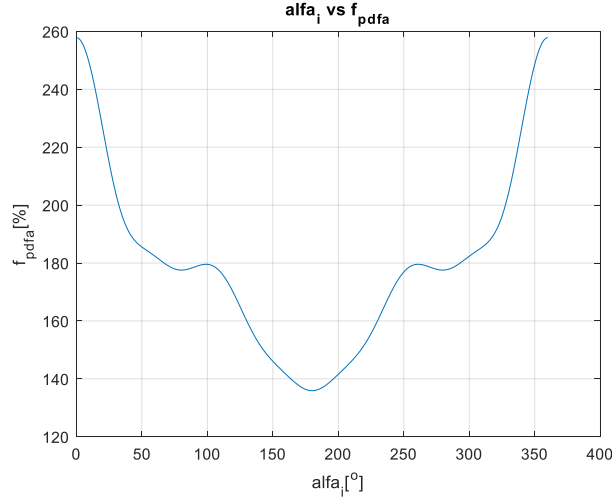
Figure 4.22. Variation of \{f_{\Sigma}(\theta)\}_{pdfa} , where f(\theta) is \tau(\theta) , for a Compressor Which Utilizes Two MinFaS-TaR Mechanisms
