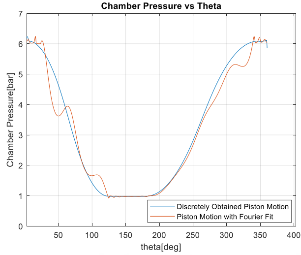
Figure 4.14. The Chamber Pressure for Fourier Fitted Motion and Discrete Motion
