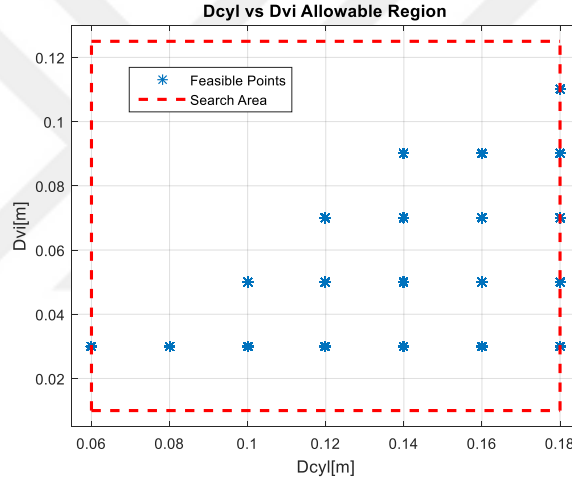
Figure 4.8. Check for the Inequalities involving only D_{vi} and D_{cyl}
