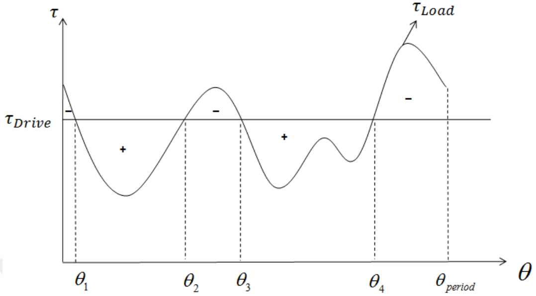
Figure 3.1. Actuator and Load Torque vs. Crank Angle of a Typical Machine
