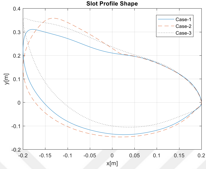
Figure A.28. Slot Profile of Slot 3a Based on Optimum Piston Motion for Case-1, 2 and 3 for Minimization of Objective-2 ( b_2 = 0.2 [m])
