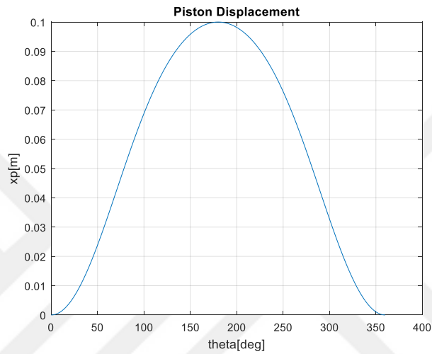
Figure A.1. Piston Displacement of the Conventional, Slider Crank Based Reciprocating Compressor
