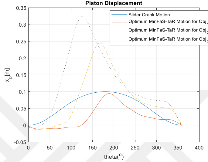
Figure A.22. The Piston Displacements of the Optimum MinFaS-TaR based Compressor and the Slider Crank Based Compressors for Case-1
