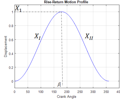
Figure 3.16. Rise Return Motion Profile
