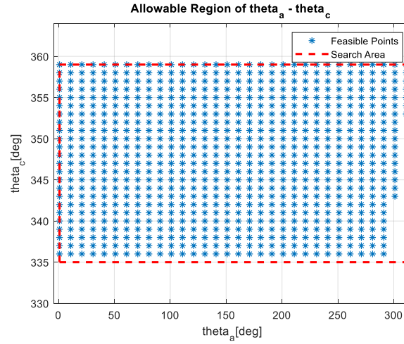
Figure 4.10. The Feasible \theta_a and \theta_c Points
