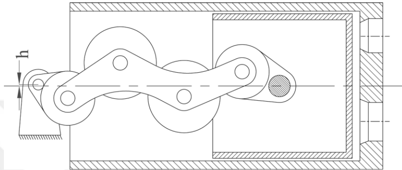
Figure 1.5. Geared Five Bar Mechanism[7]
