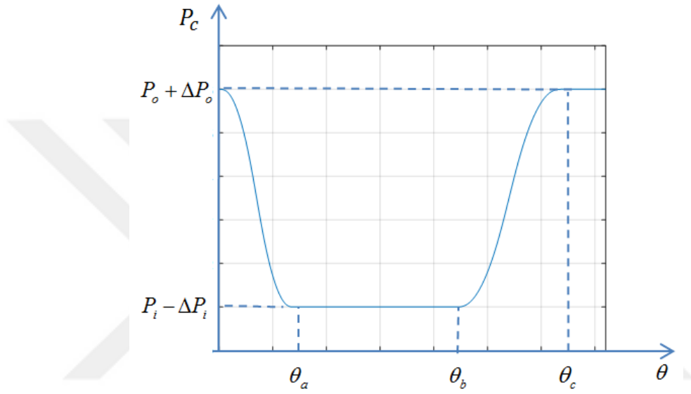
Figure 4.4. Assumed Optimal Chamber Pressure Function for a Reciprocating Compressor
