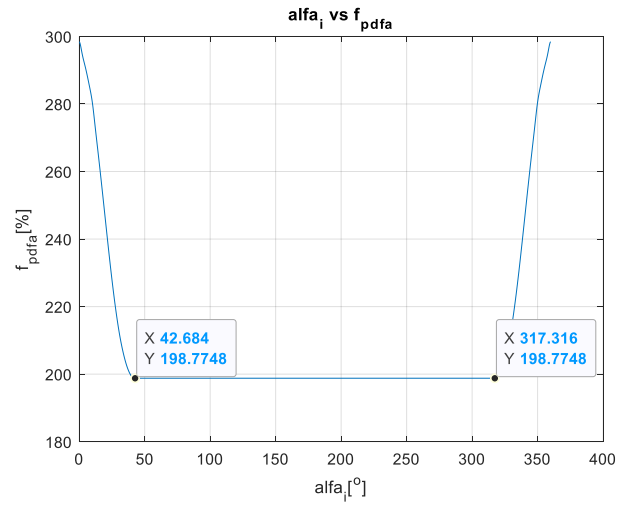
Figure 4.20. Variation of \{f_{\Sigma}(\theta)\}_{pdfa} , where f(\theta) is \dot{m}_o(\theta) , for a Compressor Which Utilizes Two MinFaS-TaR Mechanisms
