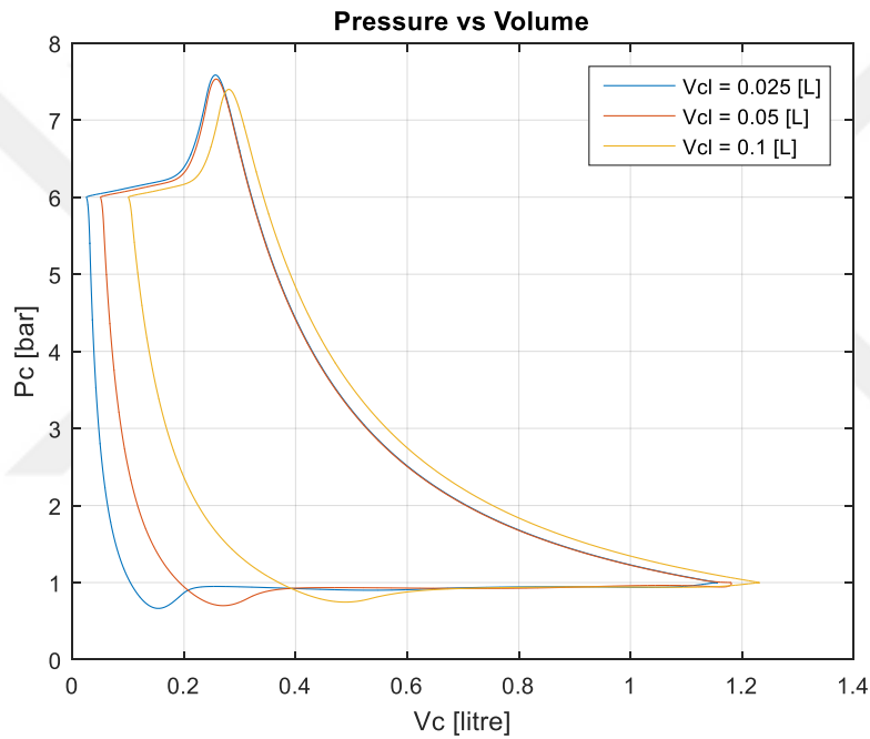
Figure 3.9. P-V Diagram for the Parametric Analysis of Clearance Volume
