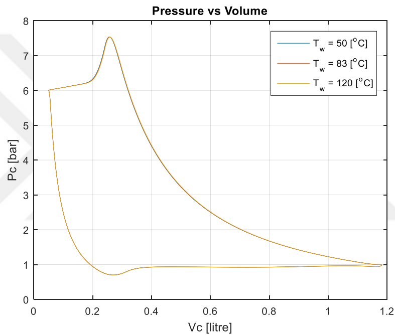
Figure 3.12. P-V Diagram for the Parametric Analysis of Wall Temperature
