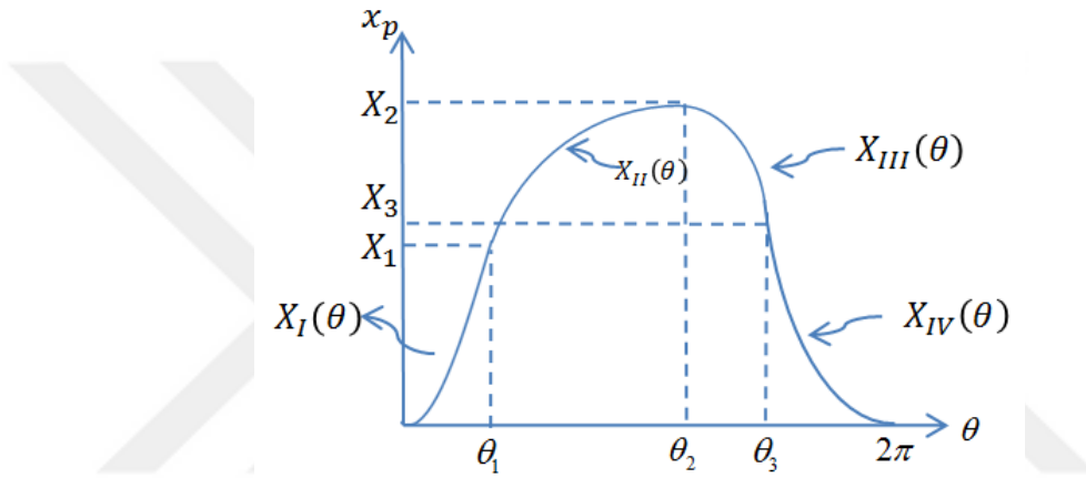
Figure 4.1. An Example of 6-5-6-5 Motion Curve
