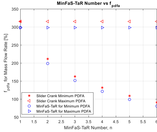
Figure 4.23. Minimum and Maximum Values of \{f_{\Sigma}(\theta)\}_{pdfa} , where f(\theta) is \dot{m}_o(\theta) , for Multi-Cylinder Slider Crank Based Compressors and for Compressors Which Utilize Multiple MinFaS-TaR Mechanisms
