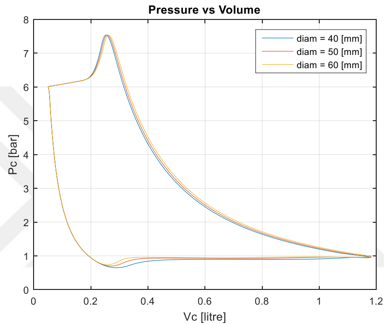
Figure 3.6. P-V Diagram for the Parametric Analysis of Inlet Valve Diameter
