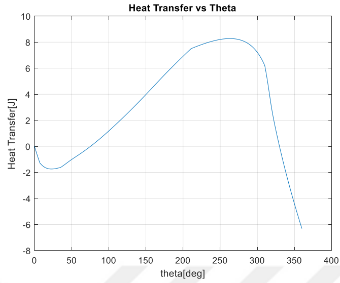
Figure A.9. Heat Transfer for the Conventional, Slider Crank Based Reciprocating Compressor
