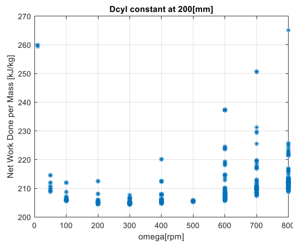
Figure 4.12. Variation of W_{net}^{pm} with respect to \theta_a and \theta_c for D_{cyl} = 200 mm
