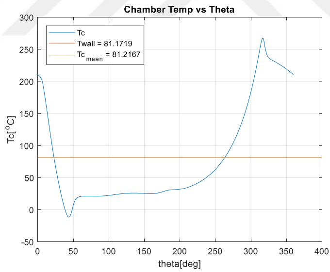
Figure A.6. Chamber Temperature of the Conventional, Slider Crank Based Reciprocating Compressor
