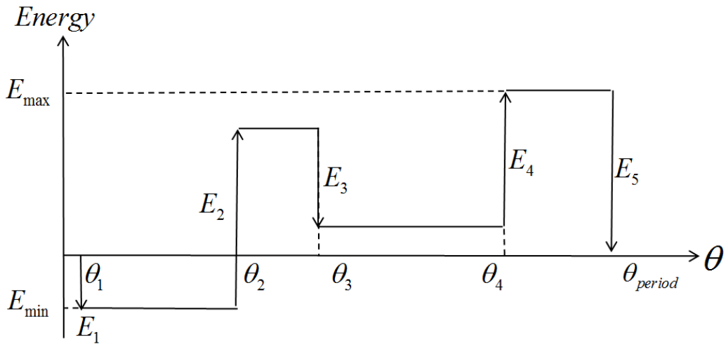
Figure 3.2. Energy Line Diagram of a Machine
