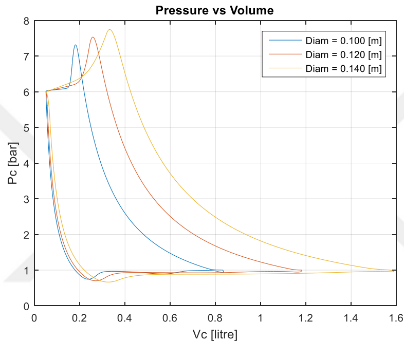
Figure 3.11. P-V Diagram for the Parametric Analysis of Piston Diameter
