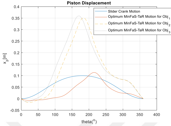
Figure A.24. The Piston Displacements of the Optimum MinFaS-TaR based Compressor and the Slider Crank Based Compressors for Case-3
