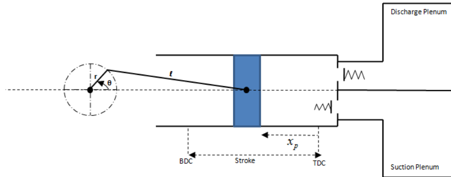
Figure 1.3. A Conventional Reciprocating Compressor
