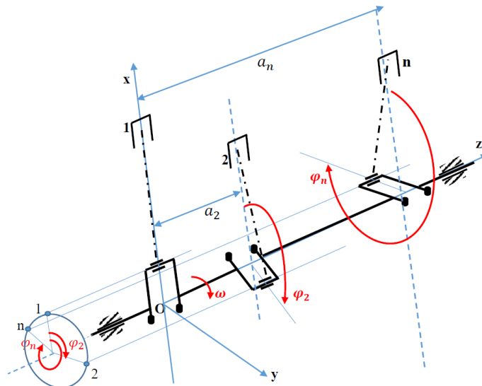
Figure 4.19. n-cylinder In-Line Reciprocating Piston Arrangement [22]
