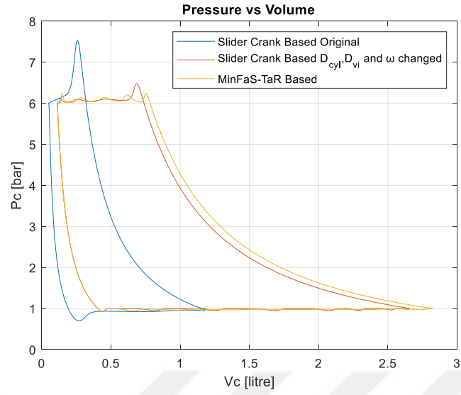
Figure 4.16. The PV Diagrams of the Optimum MinFaS-TaR based Compressor and the Slider Crank Based Compressors
