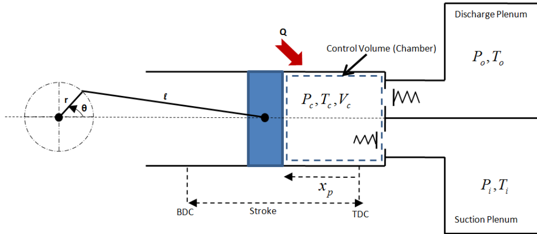
Figure 2.1. Reciprocating Compressor
