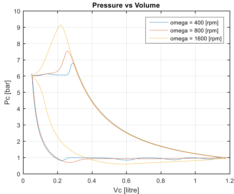
Figure 3.4. P-V Diagram for the Parametric Analysis of Motor Speed
