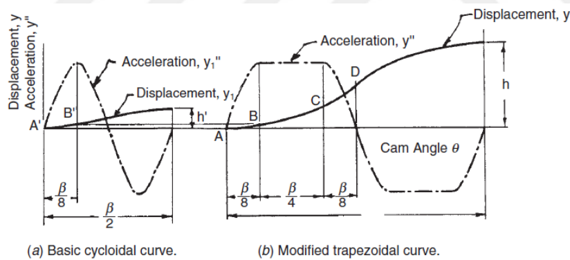
Figure 3.15. The Modified Trapezoidal Motion Curve [19]
