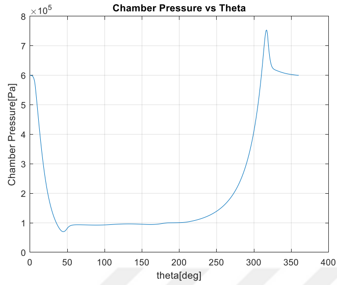
Figure A.5. Chamber Pressure of the Conventional, Slider Crank Based Reciprocating Compressor
