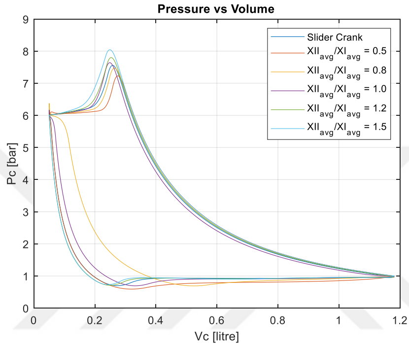
Figure A.16. PV Diagrams of Case A1 for Cases M1-M6
