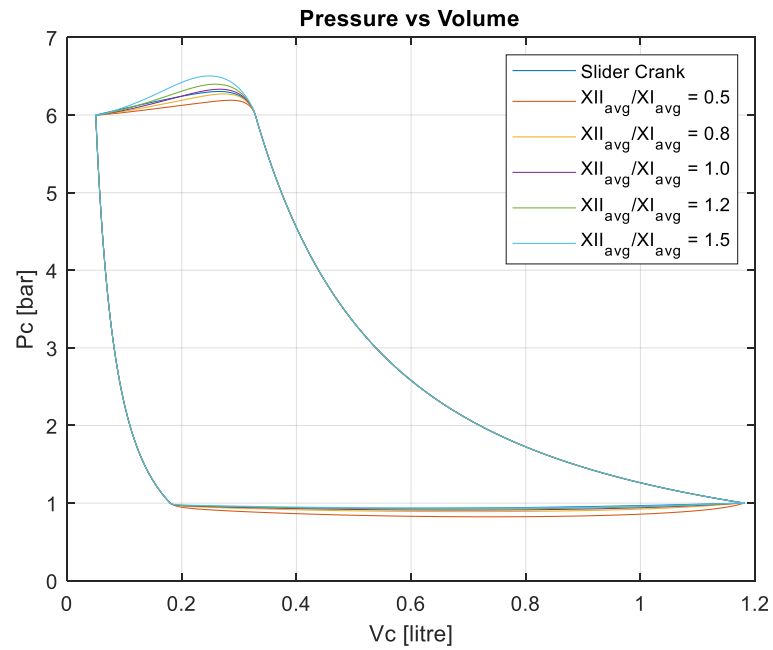
Figure A.17. PV Diagrams of Case A2 for Cases M1-M6
