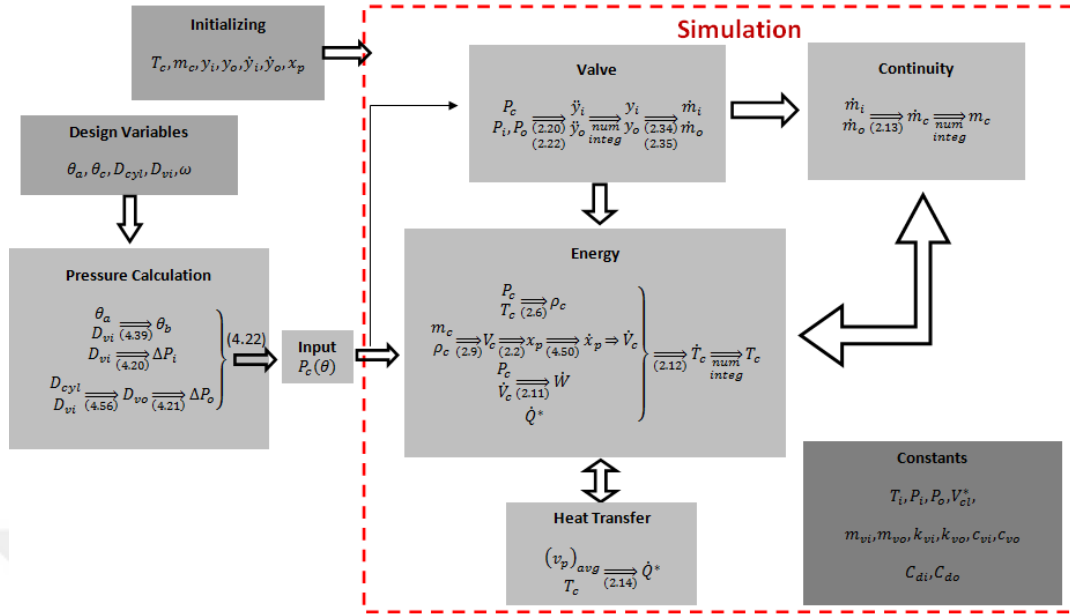
Figure 4.5. Simulation Block Diagram for the Thermo-Fluid Model of a Reciprocating Compressor using the Pressure, P_c(\theta) , as the Input
