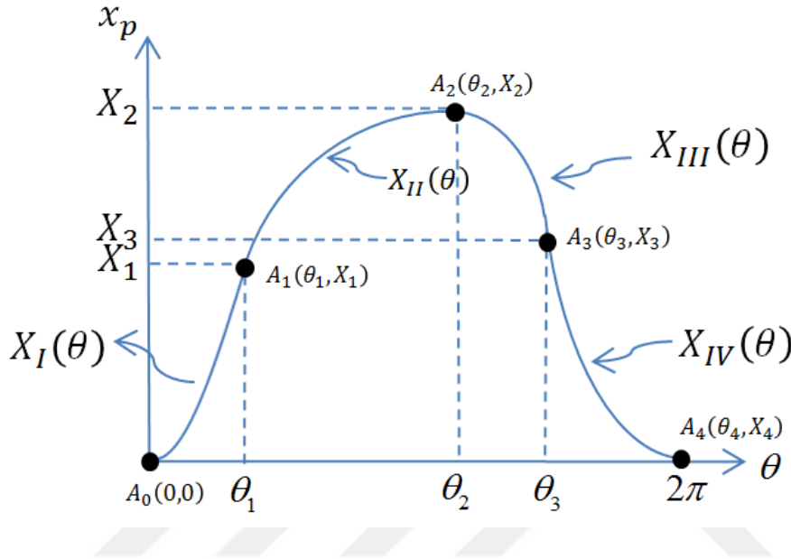
Figure A.21. 6-5-6-5 Polynomial
