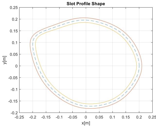
Figure 4.27. Slot Profile of Slot 3a Based on Optimum Piston Motion for Case-1 for Minimization of Objective-1( b_2 = 0.2 [m])
