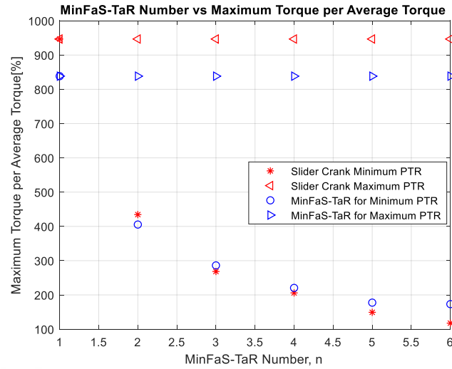
Figure 4.25 Minimum and Maximum Values of PTR for Multi-Cylinder Slider Crank Based Compressors and for Compressors Which Utilize Multiple MinFaS-TaR Mechanisms
