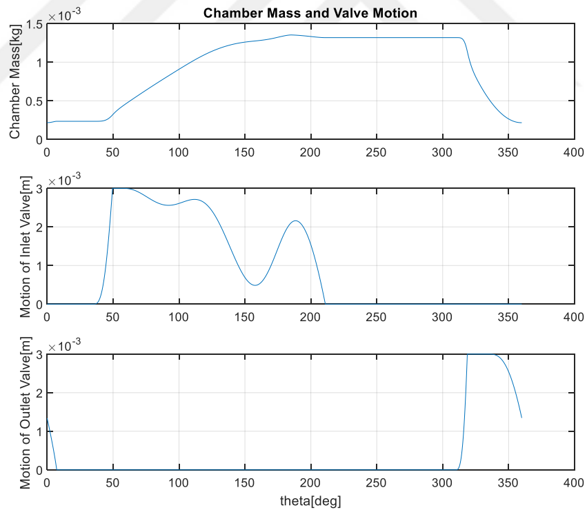
Figure A.10. Chamber Mass and Valve Motion of the Conventional, Slider Crank Based Reciprocating Compressor
