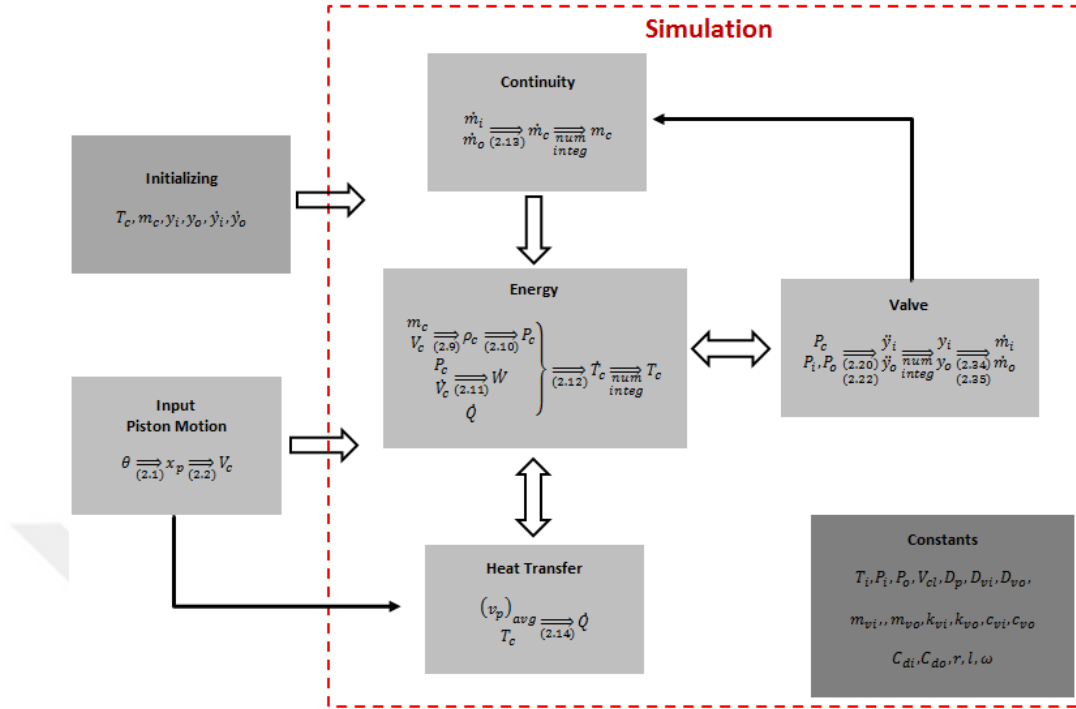
Figure 2.6. Simulation Block Diagram
