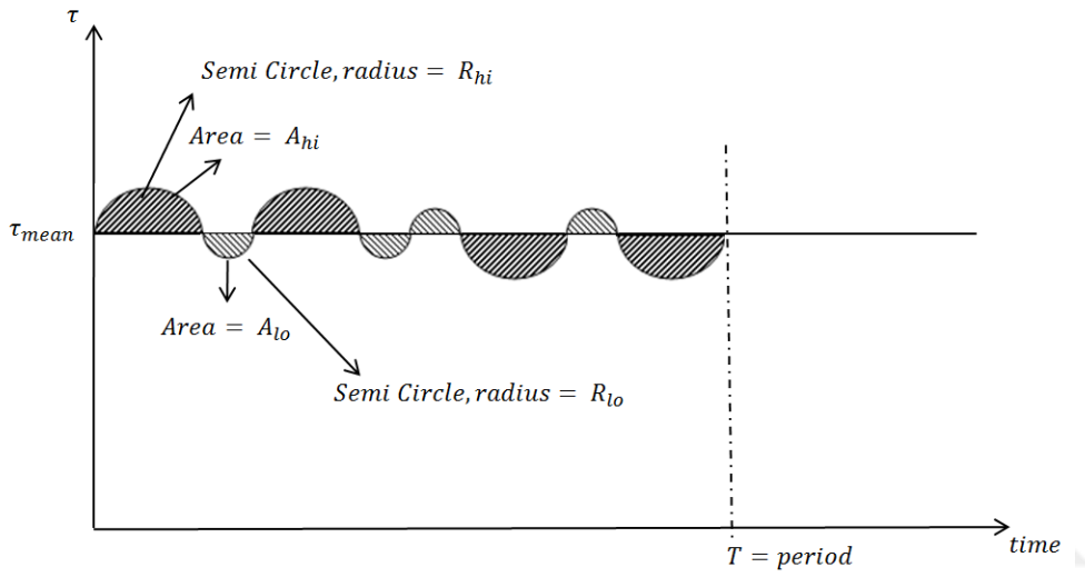
Figure A.11. Torque Versus Time Plot of the First Counter Example
