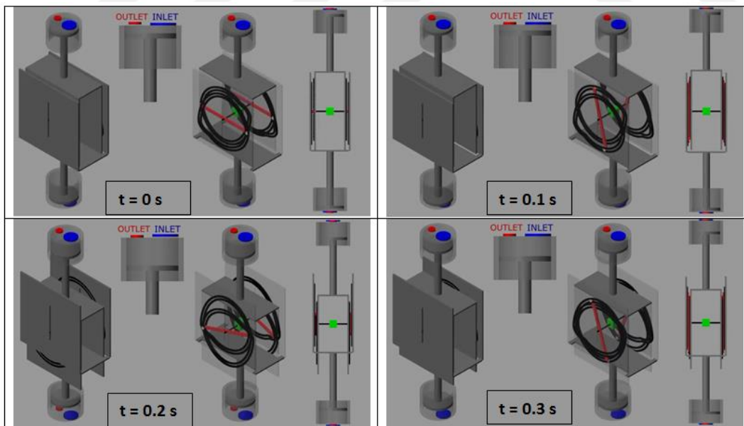
Figure 4.30. Snapshots of the Visual Simulation of the MinFaS-TaR based Compressor
