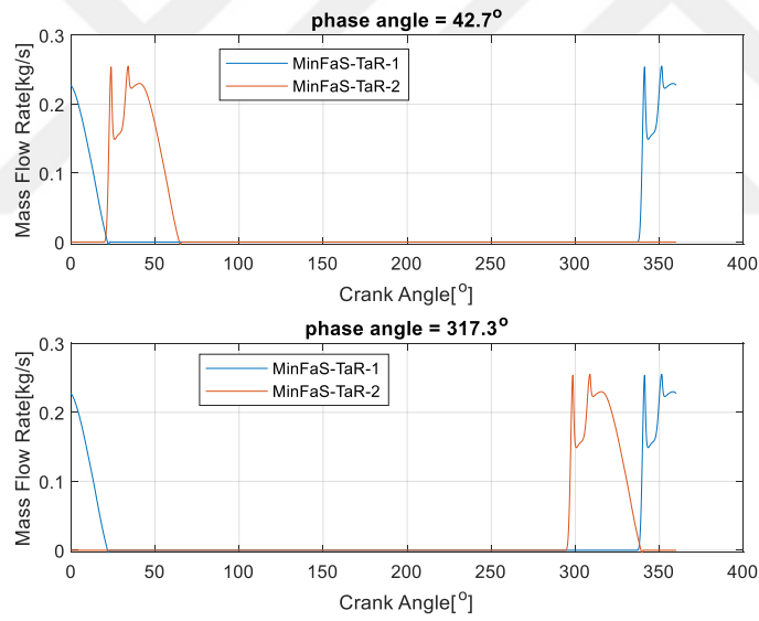
Figure 4.21. The Mass Flow Rate of a Compressor Which Utilizes Two MinFaS-TaR Mechanisms with Different Phase Angle Solutions
