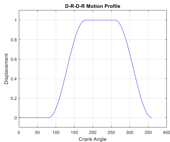
Figure 3.13. A D-R-D-R Type Cam Motion Curve
