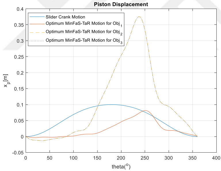
Figure A.25. The Piston Displacements of the Optimum MinFaS-TaR based Compressor and the Slider Crank Based Compressors for Second Stage of Two-Stage Compressor for Case-4
