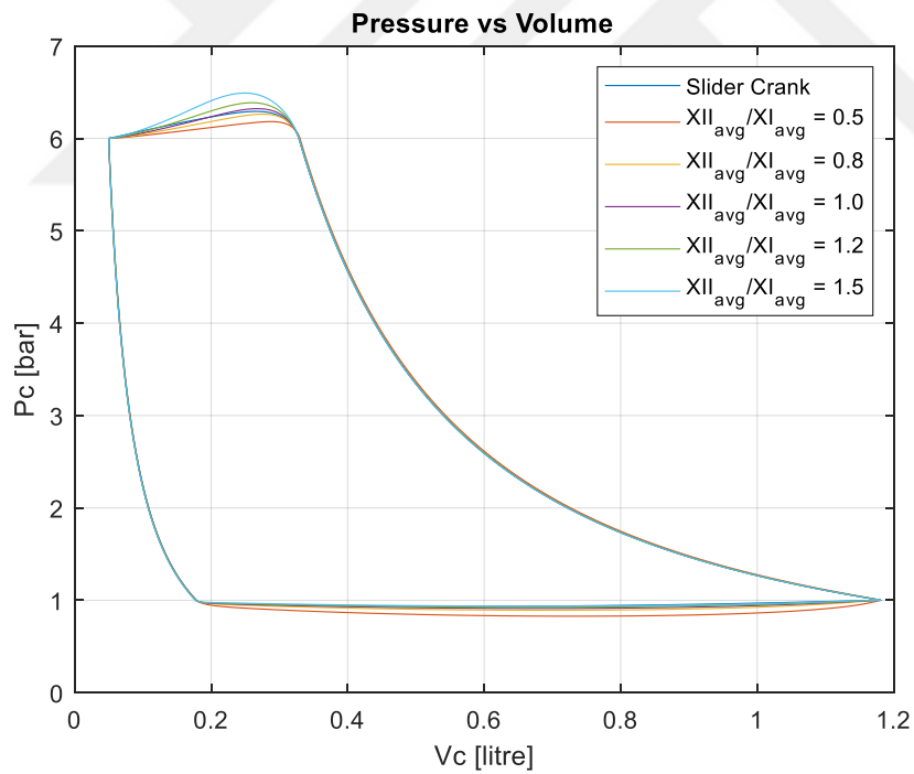
Figure A.19. PV Diagrams of Case A4 for Cases M1-M6
