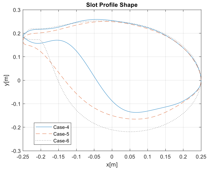
Figure A.29. Slot Profile of Slot 3a Based on Optimum Piston Motion for Case-4, 5 and 6 for Minimization of Objective-2 ( b_2 = 0.25 [m])
