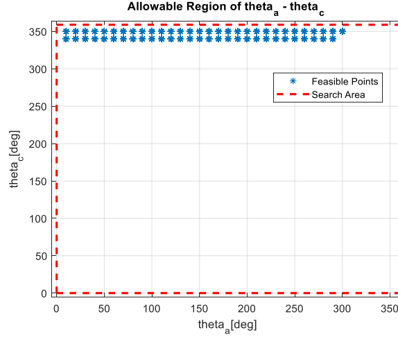
Figure 4.9. Feasible Points in the \theta_a - \theta_c Plane
