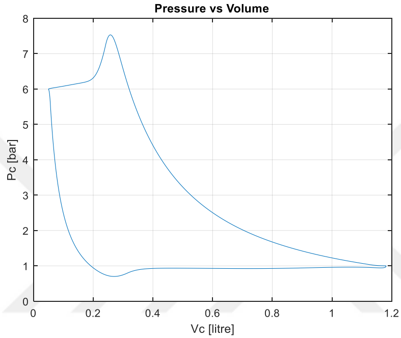
Figure 2.7. Pressure vs Chamber Volume for the Slider Crank Based, Single Cylinder Reciprocating Compressor
