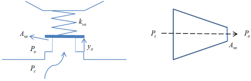
Figure 2.4. Mass Spring Model and Nozzle Diagram of the Discharge Valve
