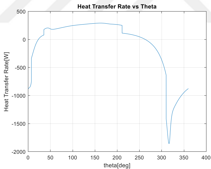
Figure A.8. Heat Transfer Rate of the Conventional, Slider Crank Based Reciprocating Compressor
