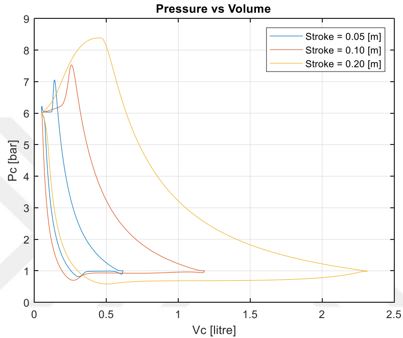
Figure 3.10. P-V Diagram for the Parametric Analysis of Stroke
