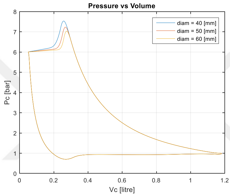
Figure 3.5. P-V Diagram for the Parametric Analysis of Outlet Valve Diameter
