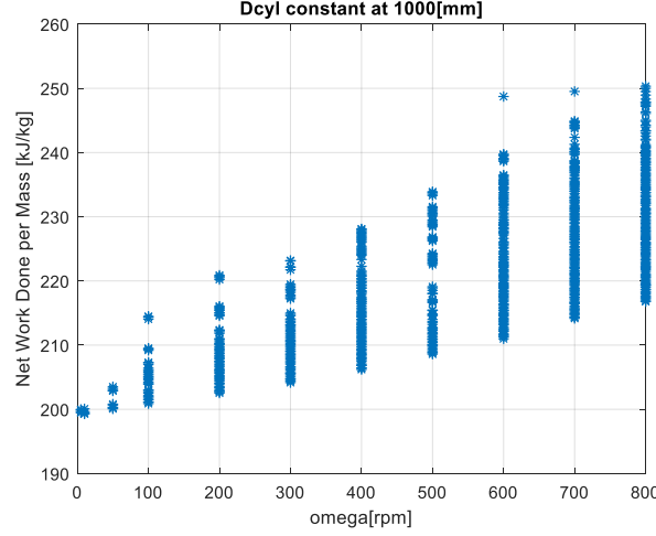
Figure 4.13. Variation of W_{net}^{pm} with respect to \theta_a and \theta_c for D_{cyl} = 1000 mm
