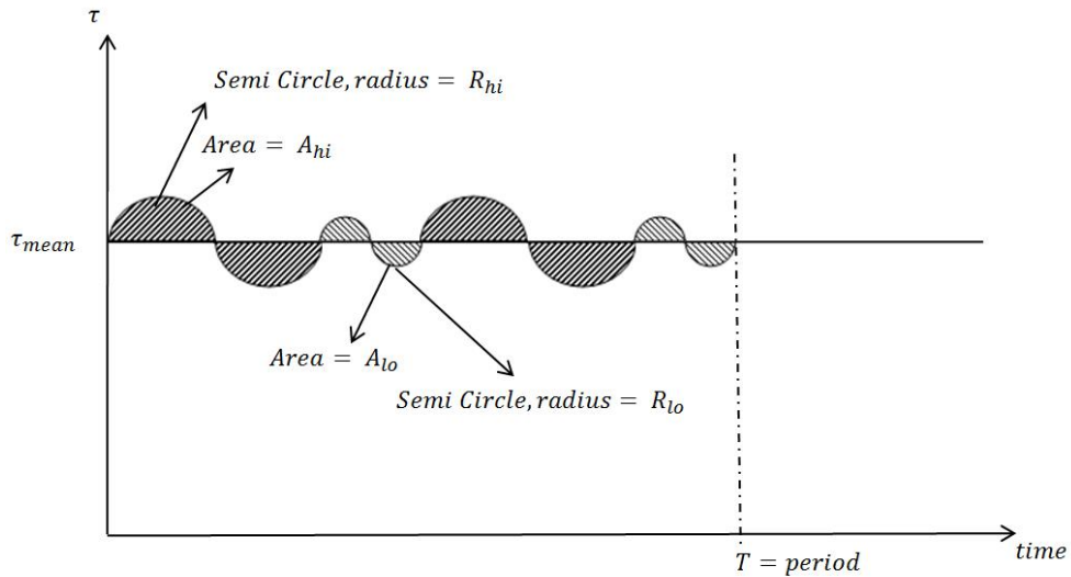
Figure A.12. Torque Versus Time Plot of the Second Counter Example
