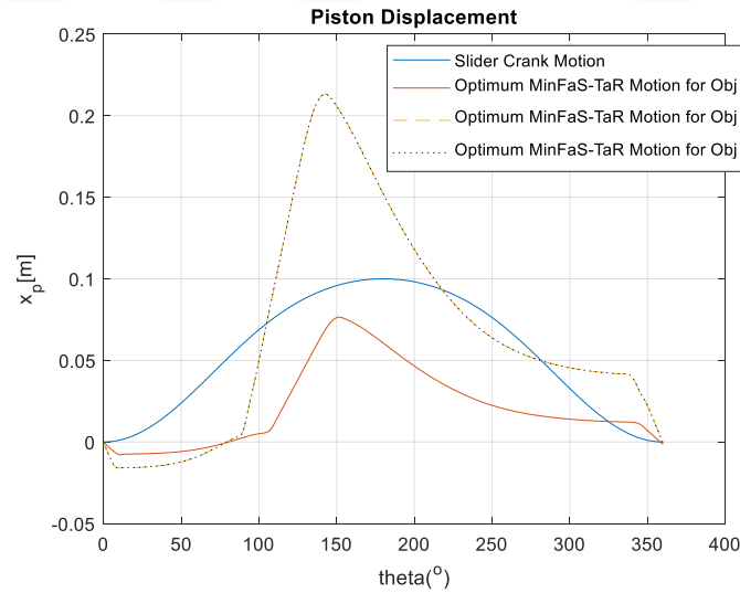
Figure A.23. The Piston Displacements of the Optimum MinFaS-TaR based Compressor and the Slider Crank Based Compressors for Case-2
