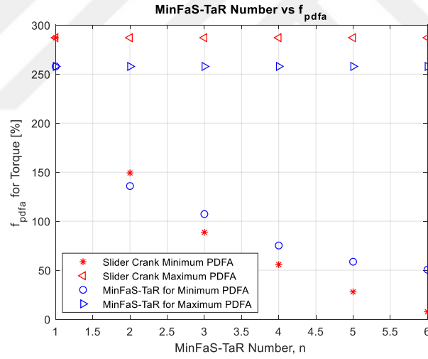
Figure 4.24. Minimum and Maximum Values of \{f_{\Sigma}(\theta)\}_{pdfa} , where f(\theta) is \tau(\theta) , for Multi-Cylinder Slider Crank Based Compressors and for Compressors Which Utilize Multiple MinFaS-TaR Mechanisms
