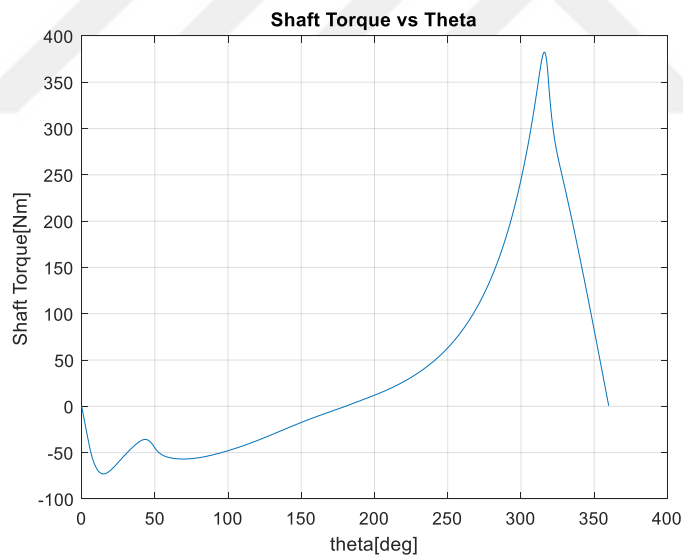
Figure A.4. Shaft Torque of the Conventional, Slider Crank Based Reciprocating Compressor
