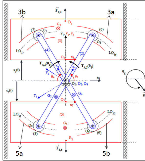
Figure 4.26. The MinFaS-TaR Mechanism [3]
