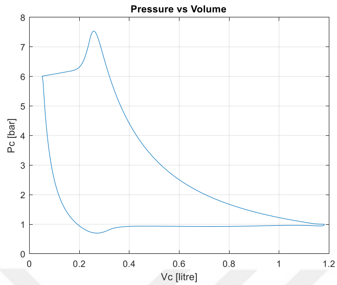
Figure A.3. PV Diagram of the Conventional, Slider Crank Based Reciprocating Compressor
