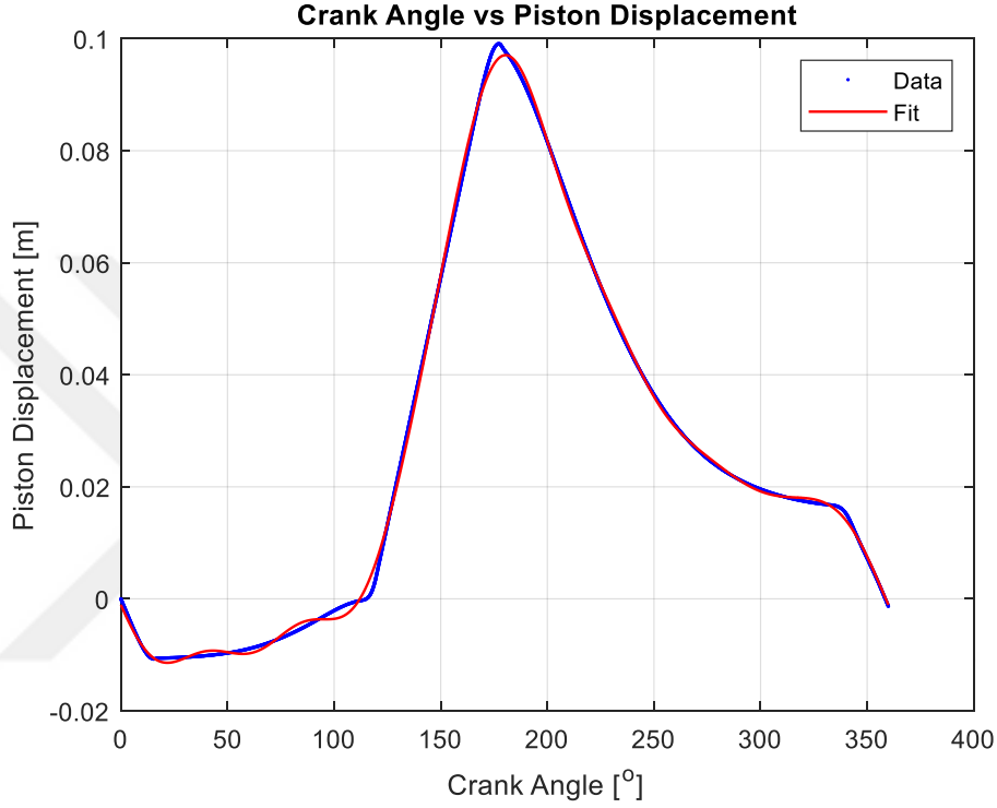
Figure 4.11. Fourier Curve Fit on the Data
