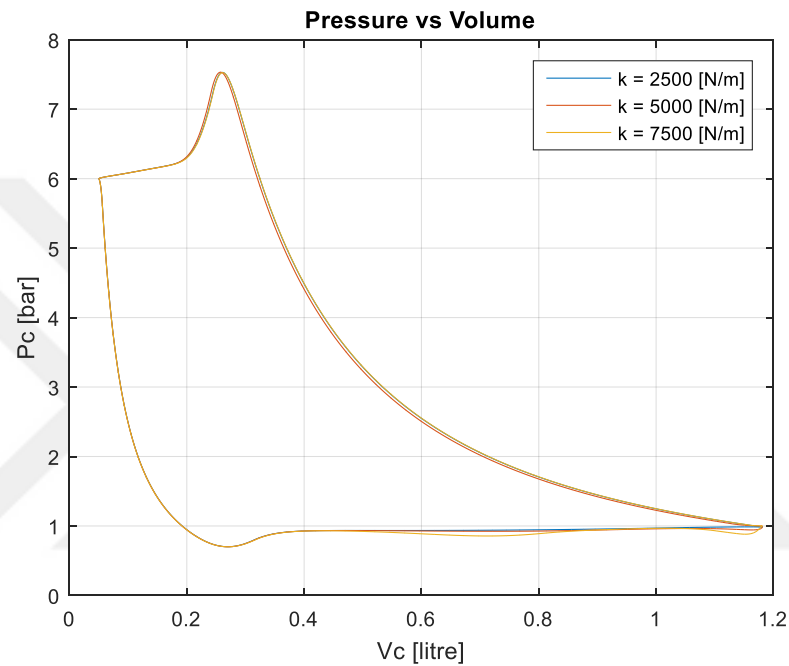
Figure 3.8. P-V Diagram for the Parametric Analysis of Inlet Valve Spring Constant
