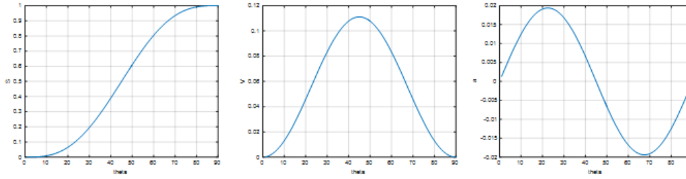
Figure 3.14. Cycloidal Motion Position, Velocity and Acceleration Curves
