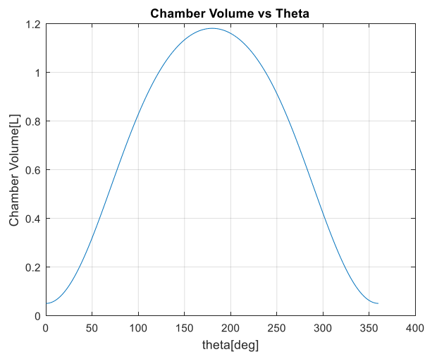
Figure A.2. Chamber Volume of the Conventional, Slider Crank Based Reciprocating Compressor
