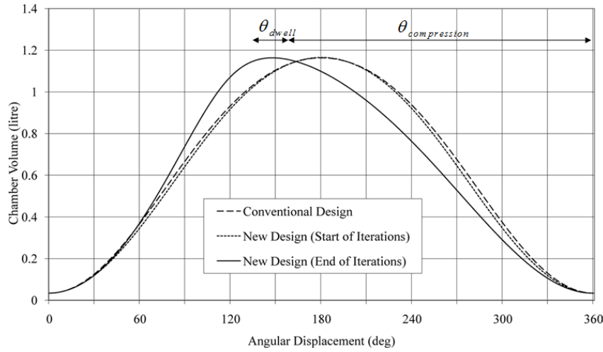
Figure 1.6. Optimum Piston Motion Curve Found by Sultan et al. [7]
