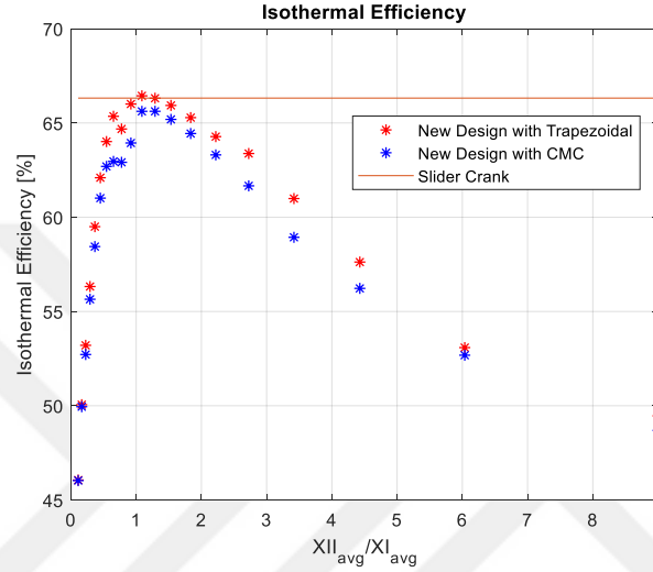
Figure 3.17. Isothermal Efficiency versus (X'_{II})_{avg}/(X'_I)_{avg}
