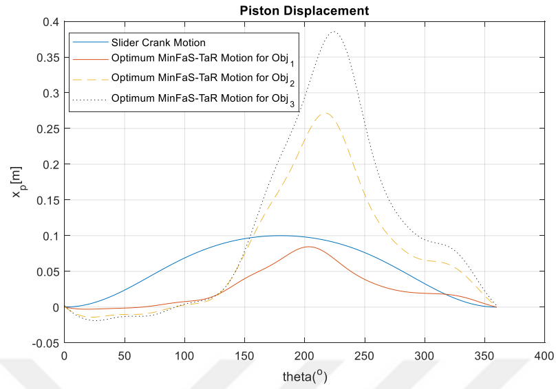
Figure A.26. The Piston Displacements of the Optimum MinFaS-TaR based Compressor and the Slider Crank Based Compressors for Second Stage of Two-Stage Compressor for Case-5
