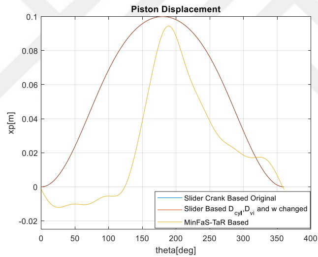
Figure 4.15. The Piston Displacements of the Optimum MinFaS-TaR based Compressor and the Slider Crank Based Compressors
