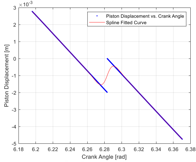
Figure 4.6. Spline Fit for the Periodicity
