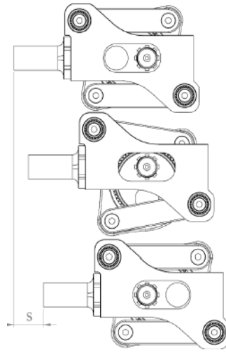
Figure 1.7. Efficient Motion Converter [8]
