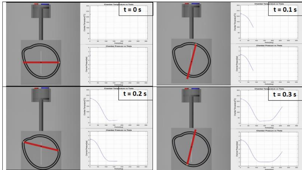
Figure 4.31. Snapshots of the Visual Simulation of the Assembly of Link 3a and the Corresponding Cylinder
