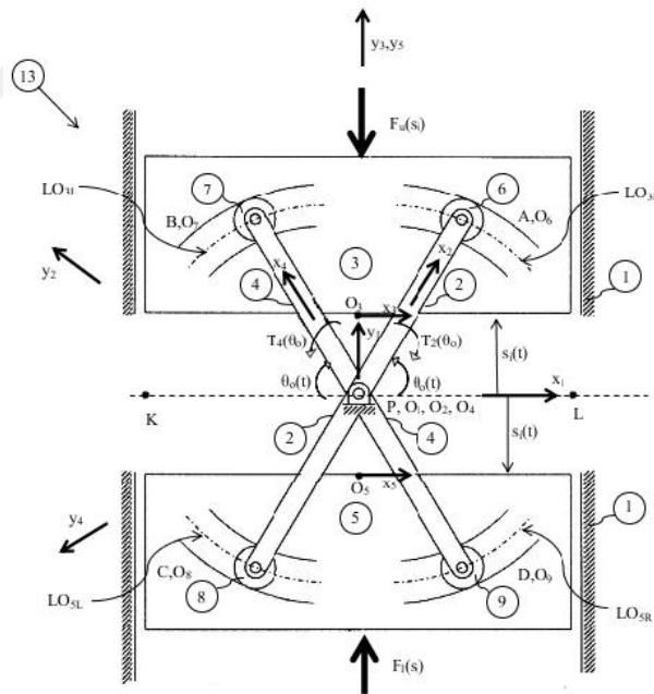
Figure 1.2. MinFaS-TaR Mechanism[1]
