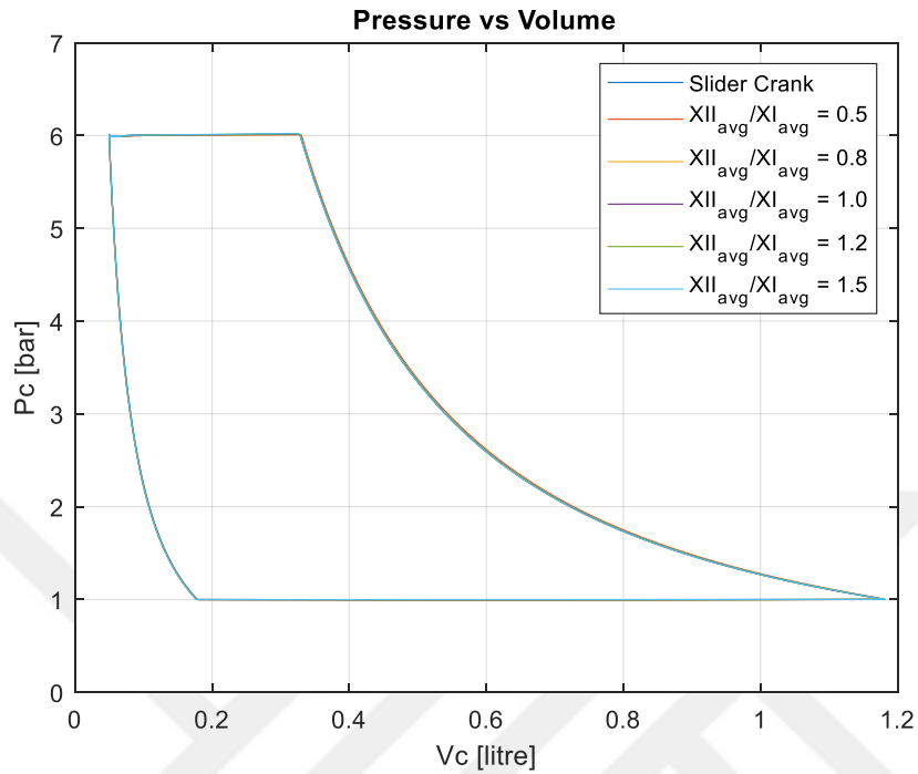
Figure A.20. PV Diagrams of Case A5 for Cases M1-M6
