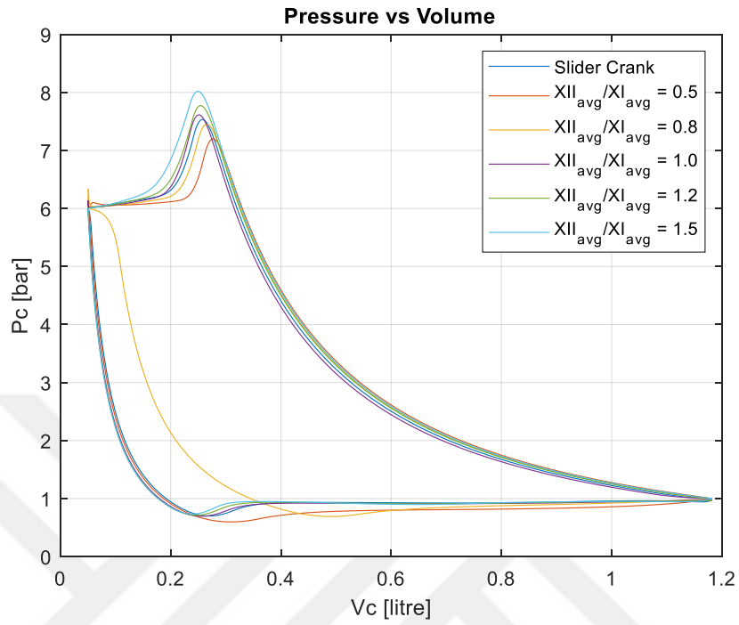
Figure A.18. PV Diagrams of Case A3 for Cases M1-M6
