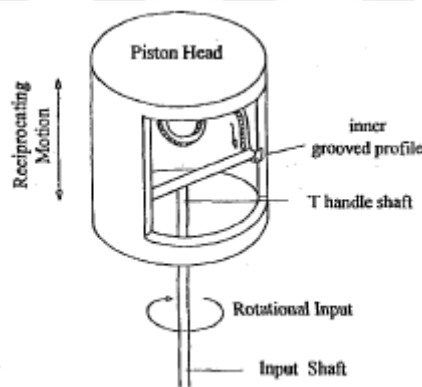
Figure 1.4. Rotaprocating Compressor [4]
