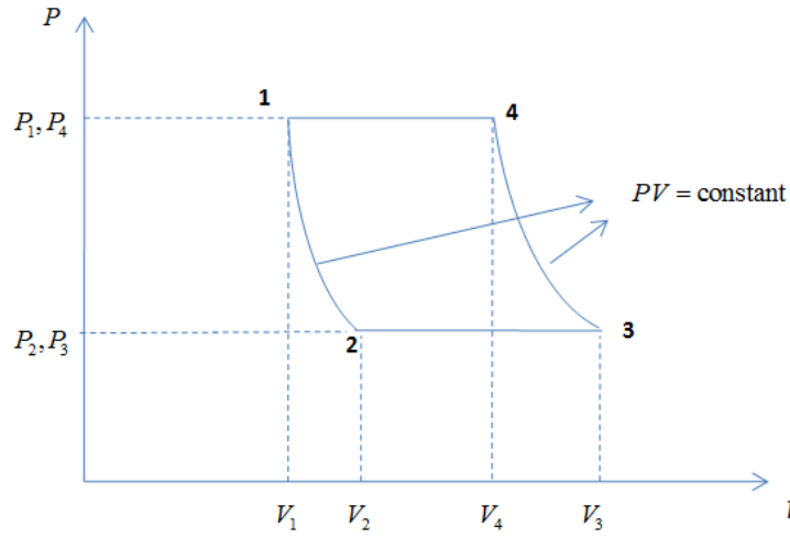
Figure 3.3. Pressure vs Volume Graph of an Isothermal Compressor
