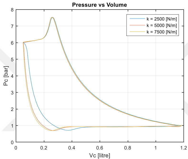
Figure 3.7. P-V Diagram for the Parametric Analysis of Outlet Valve Spring Constant
