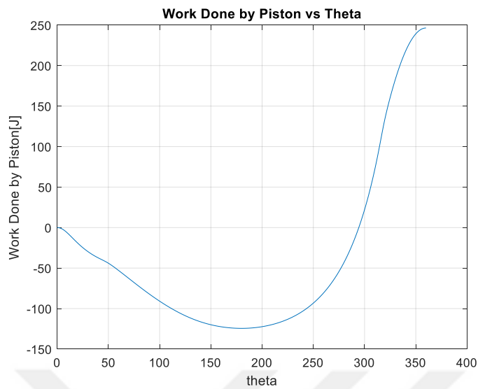
Figure A.7. Work Done for the Conventional, Slider Crank Based Reciprocating Compressor
