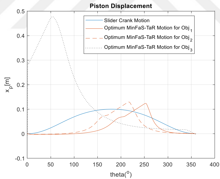
Figure A.27. The Piston Displacements of the Optimum MinFaS-TaR based Compressor and the Slider Crank Based Compressors for Case-6
