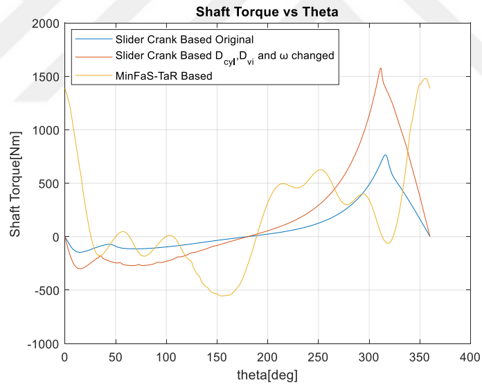
Figure 4.17. The Motor Torques of the Optimum MinFaS-TaR based Compressor and the Slider Crank Based Compressors
