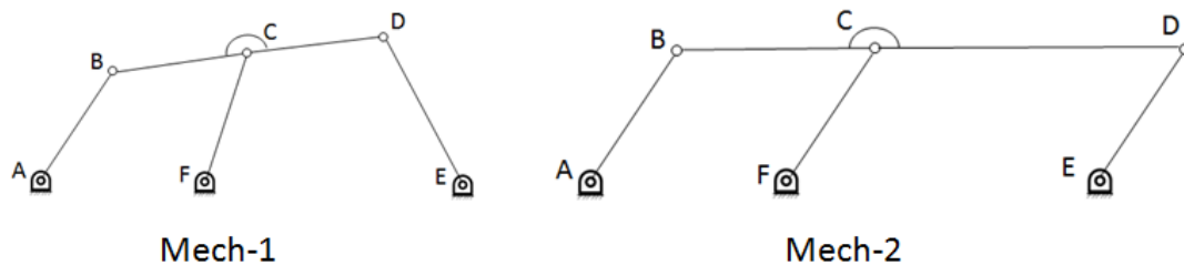
Figure 1.1. Overconstrained Mechanism
