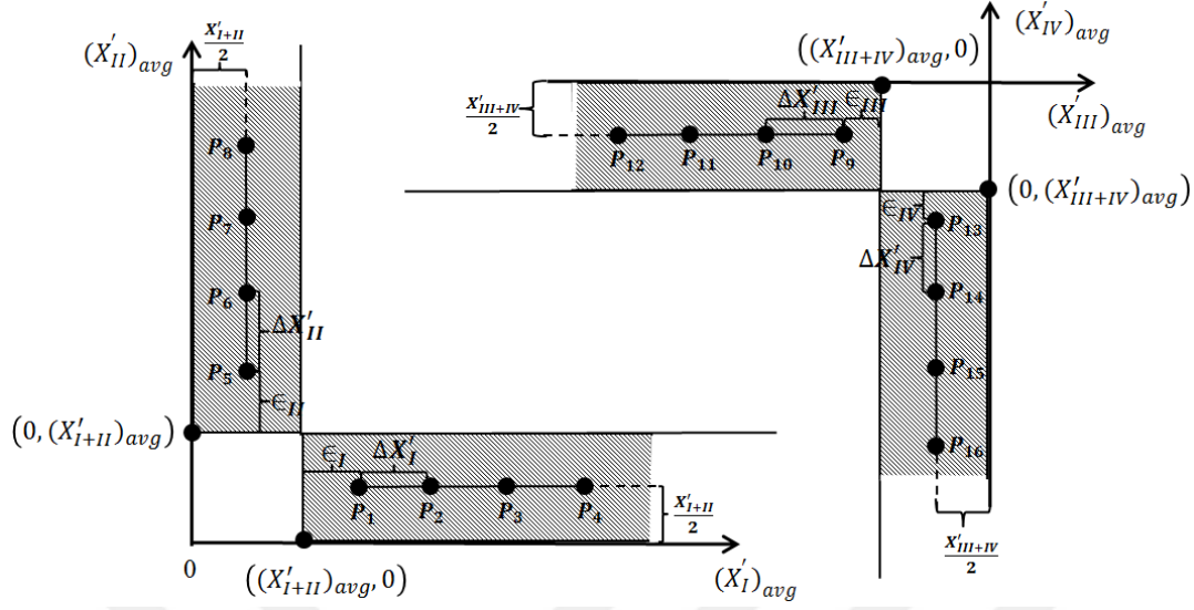
Figure 4.3. 6-5-6-5 Polynomial Brute Force Search Points
