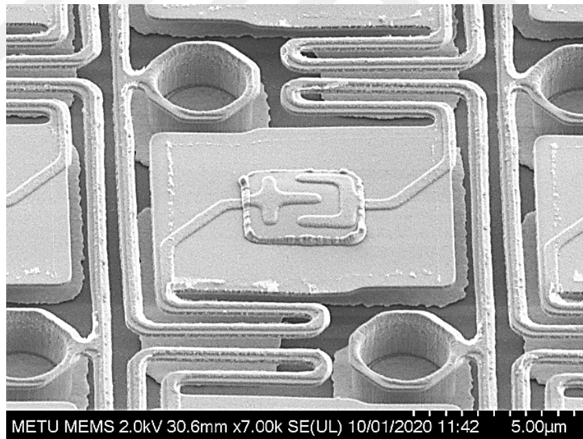
Figure 3.22: SEM images of “Design #18” of the wafer #5 with 12 μm pixel pitch.
