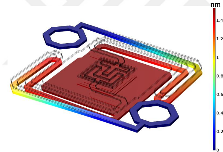
Figure 2.15: Magnitude of displacement for design #18 under 1000g applied in -z direction (the display is exaggerated).
