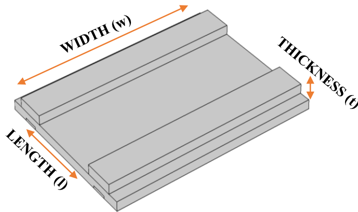
Figure 2.1: Side view of the standard type planar electrodes.
