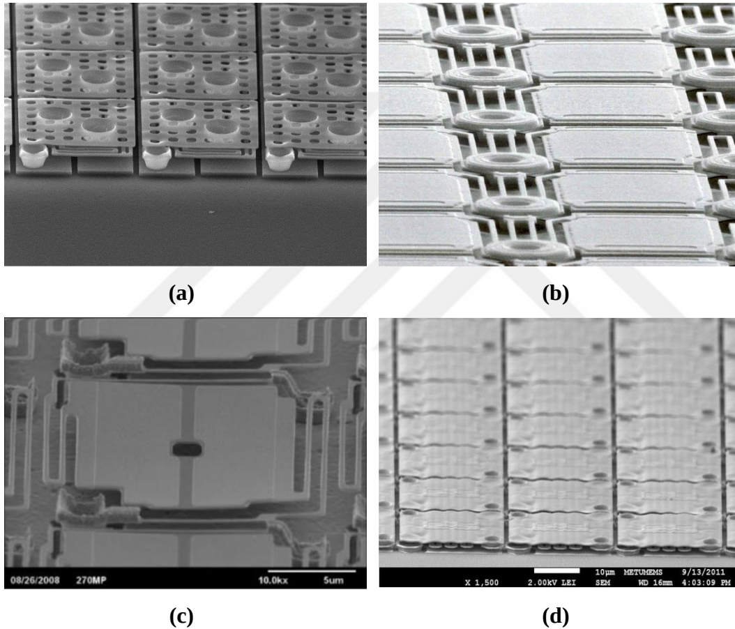
Figure 1.9: SEM images of microbolometer FPA's that fabricated by (a) VOx umbrella design microbolometer from DRS [42], (b) VOx bolometer from BAE [43], (c) a-Si/a-SiGe microbolometer from L-3 Communications [27], and (d) YBCO microbolometer from METU [35].
