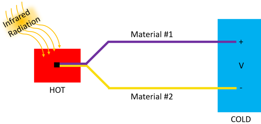
Figure 1.4: The basic representation of the thermoelectric detector.
