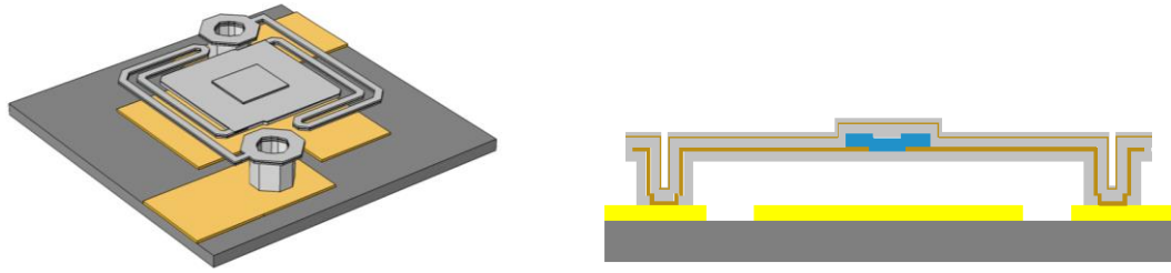
h) Releasing the pixel with removing the sacrificial layer.
