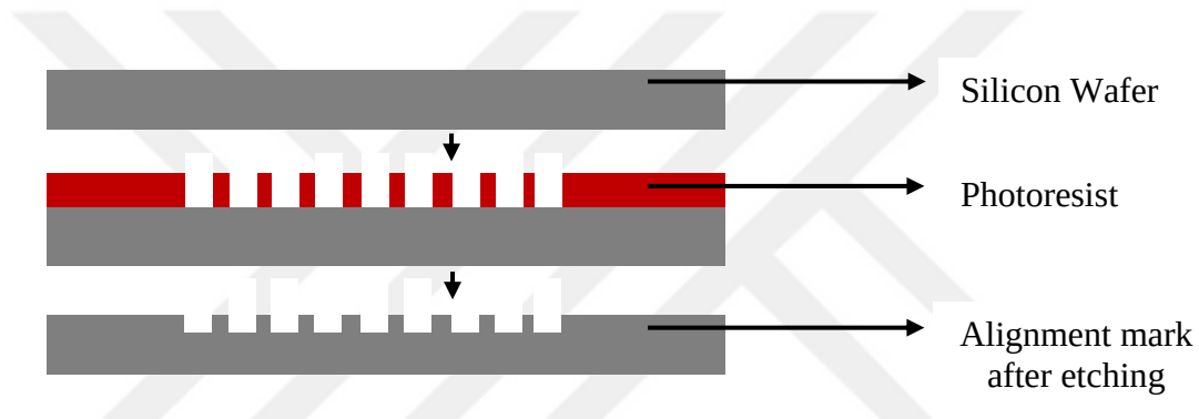
Figure 3.3: 2-D perspective of marker process on the silicon wafer.
