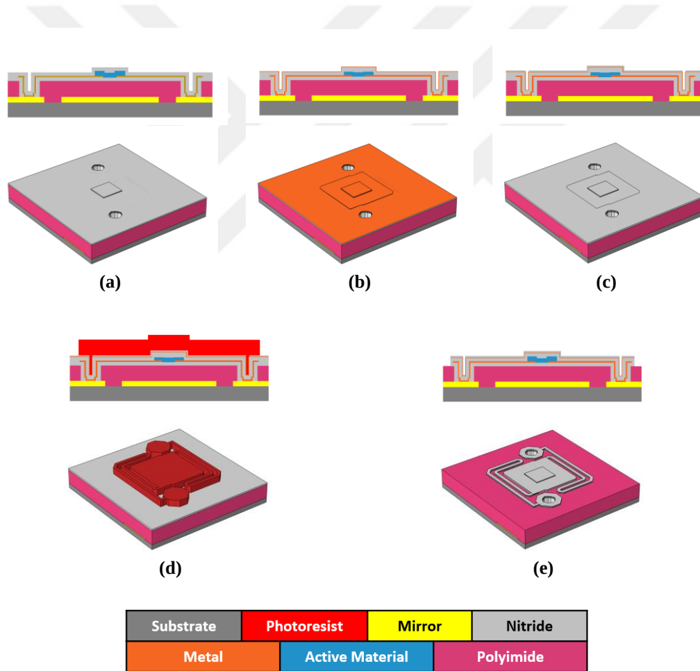
Figure 3.18: 2-D and 3-D perspective of the constructing structural layers, absorber layer, and pixel arm/body structure (a) 2 nd structural layer deposition, (b) absorber layer deposition, (c) 3 rd structural layer deposition, (d) lithography, and (e) etch.
