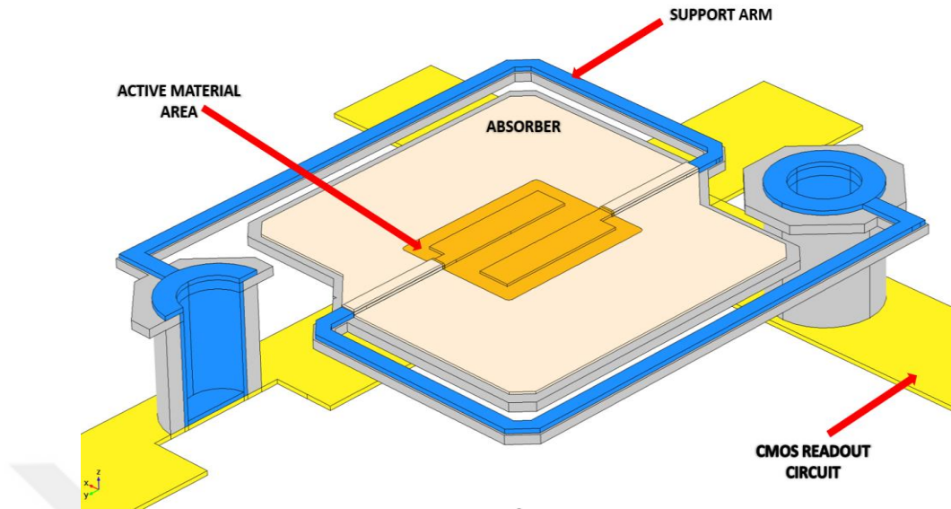
Figure 1.6: A general graphical representation of resistive microbolometer pixel.
