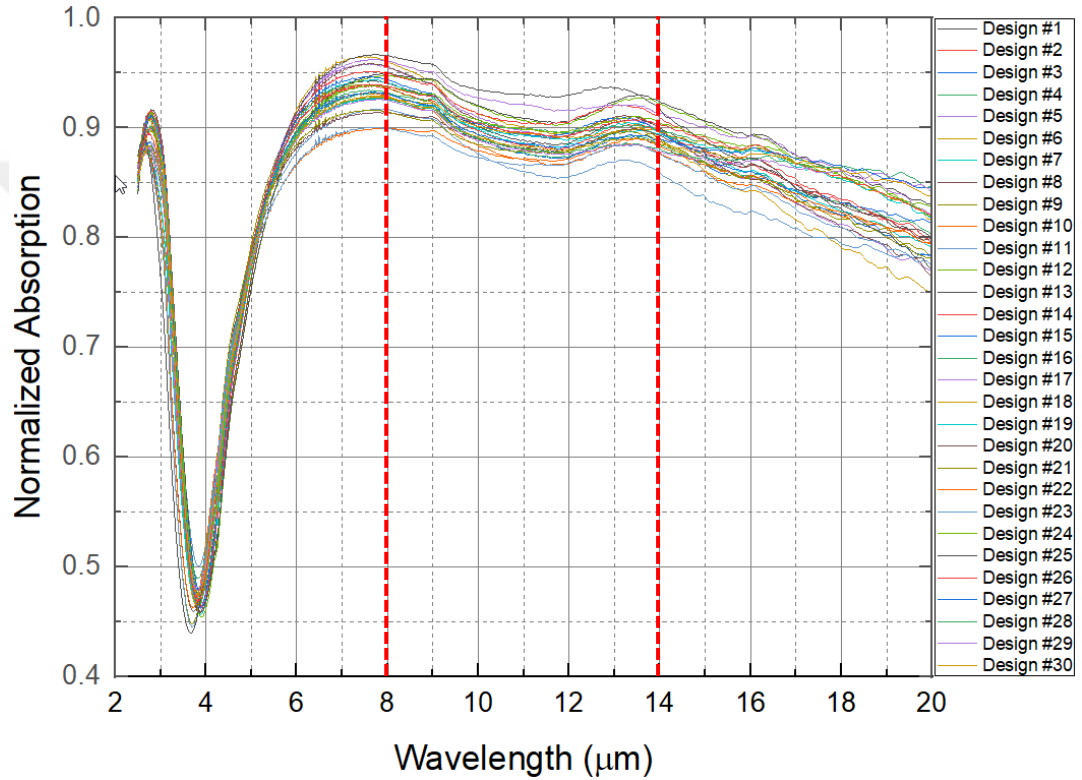
Figure 4.11: Absorption measurement for each design # at wafer #3 with desired absorption window 8-12 \mu\text{m} .
