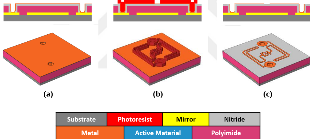
Figure 3.14: 2-D and 3-D perspective of the metal layer formation after (a) deposition, (b) lithography, and (c) etch.
