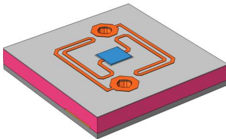
e) Deposition the active material with top electrode metal and pattern these layers together.
