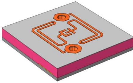
d) Deposition and patterning of the metal layer for arms and electrodes.
