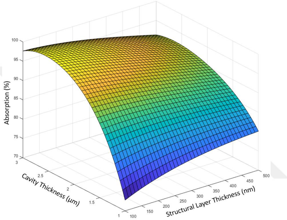
Figure 2.7: Variations in absorption (%) with structural layer and sacrificial cavity layer thickness change.
