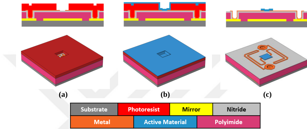
Figure 3.17: 2-D and 3-D perspective of the active material formation after (a) lithography, (b) deposition, and (c) lift-off.
