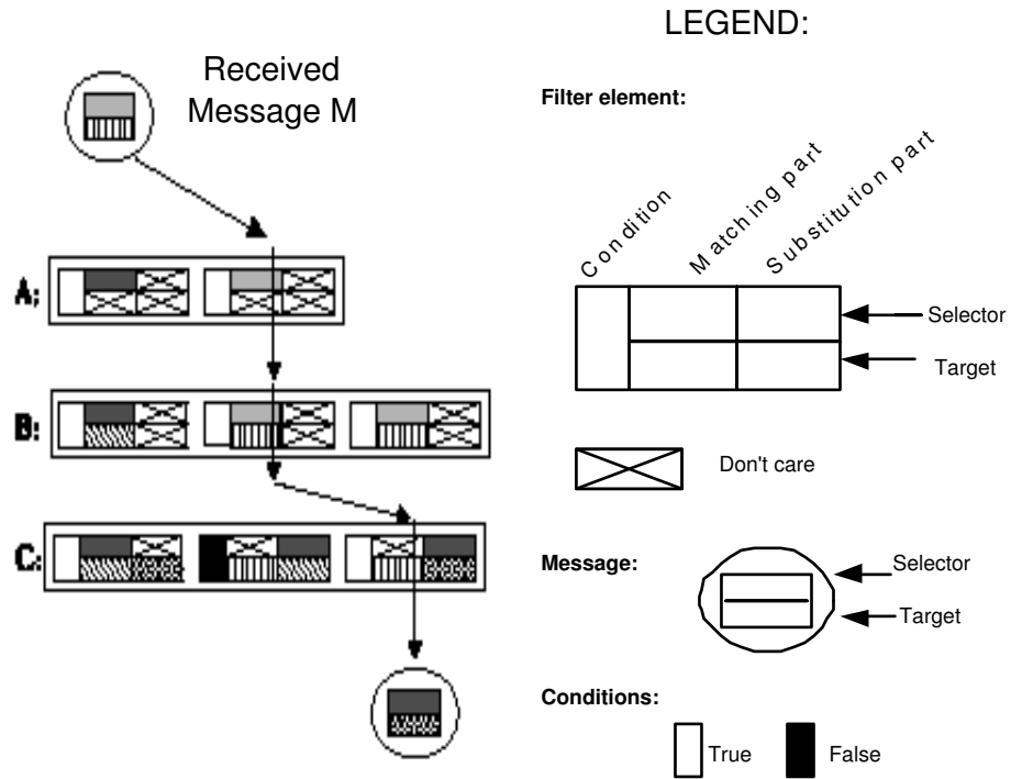
Figure 4.3: Message evaluation by filters
