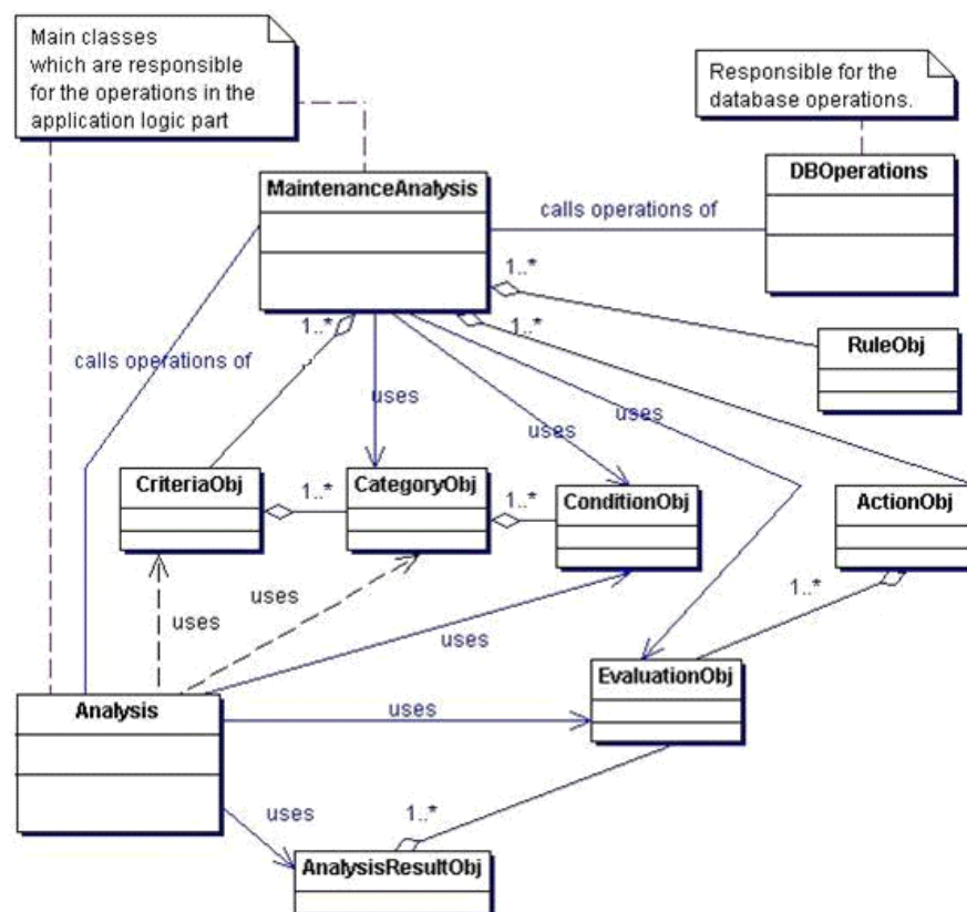
Figure 6.19: Class diagram of the ALAT
