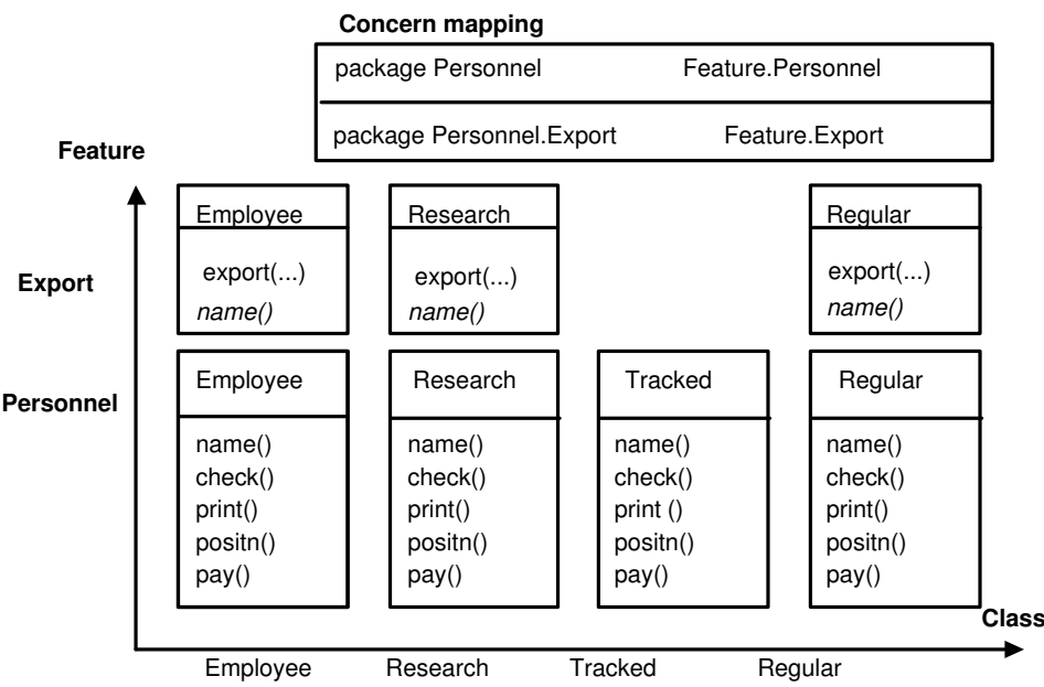
Figure 4.12: Hyperspace solution - Step 3
