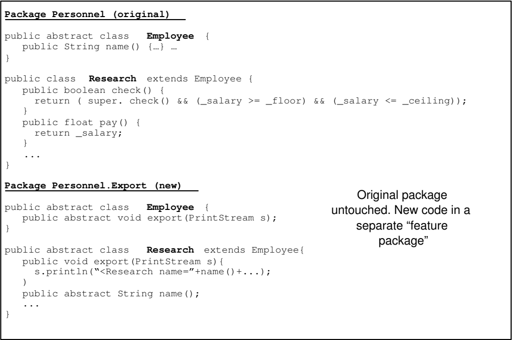
Figure 4.11: Hyperspace solution - Step 2
