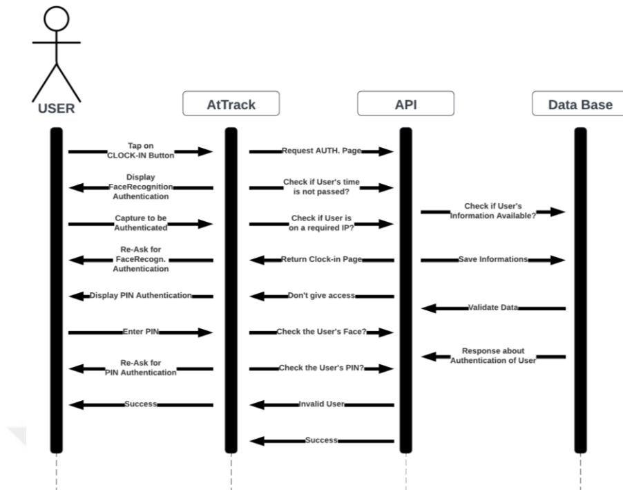
Figure 4.4. User sequence diagram.
