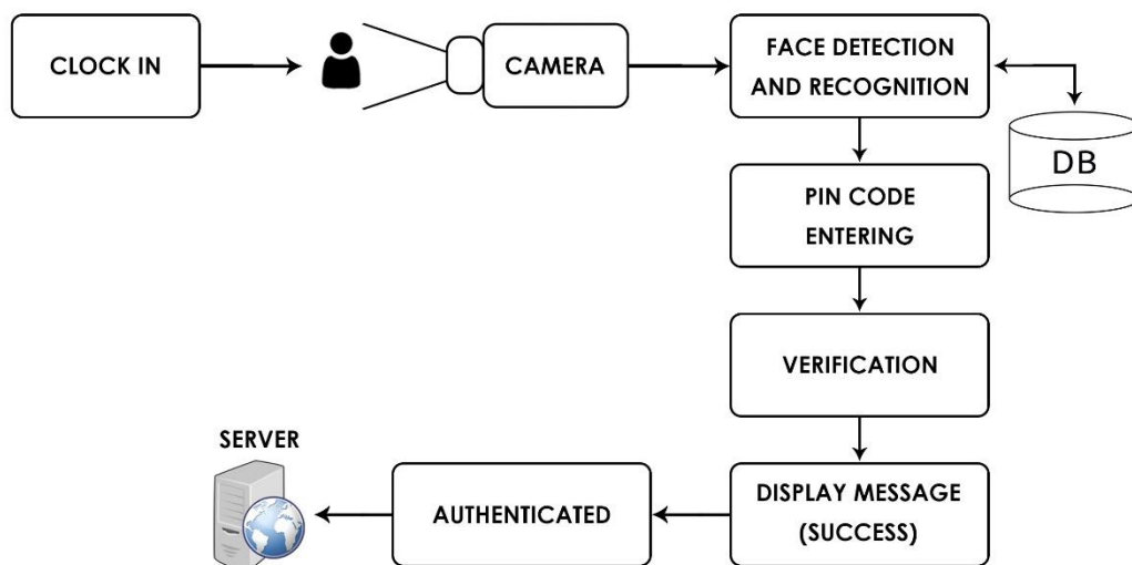
Figure 3.1. Generalized model of the proposed system.
