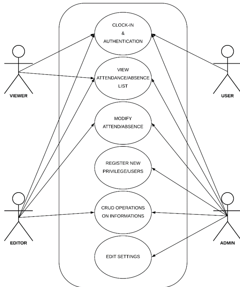
Figure 3.4. Application and roles use-case diagram.
