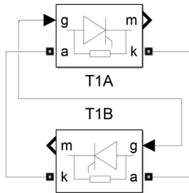
Figure 5.11. Thyristor tap switch Matlab model
