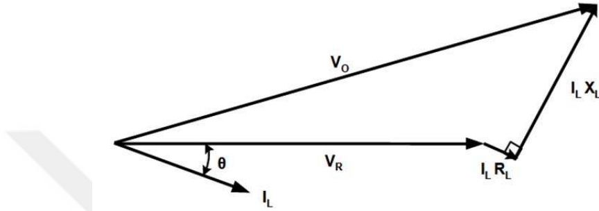
Figure 4.30. Phasor Diagram for LDC
