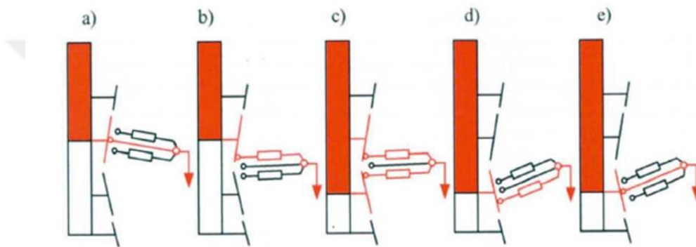
Figure 3.3. Mechanical tap changer operation with only selector switch (Korpikiewicz & Mysiak, 2017)
