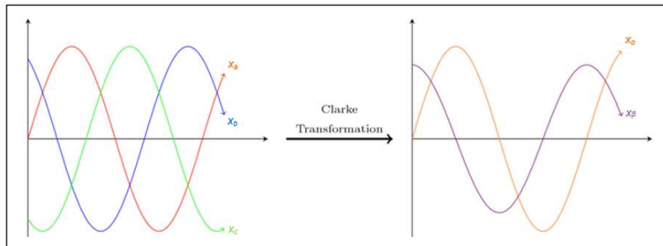
Figure 5.24. Clarke Transformation
