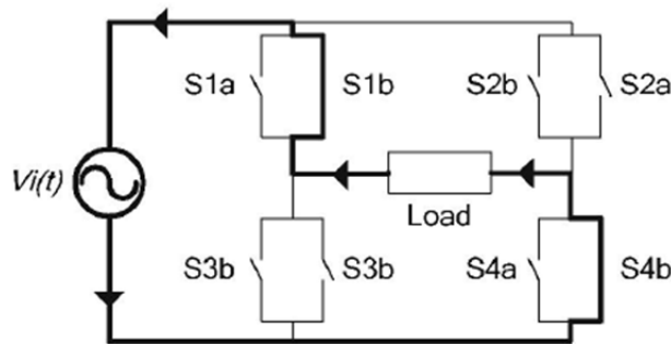
Figure 5.16. SPMC as AC voltage regulator, negative half cycle (Hanafi et al., 2006)
