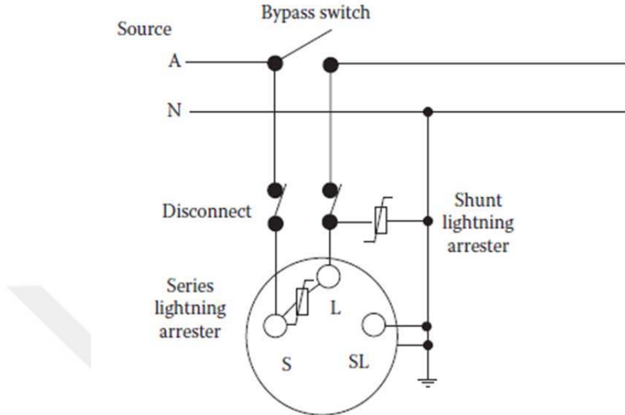
Figure 4.18. SVR connection in a single phase circuit (Colopy, 2012)
