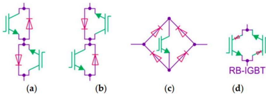
Figure 5.17. (a) common emitter, (b) common emitter, (c) diode bridge, (d) reverse block-IGBT (Szczesniak, 2019)
