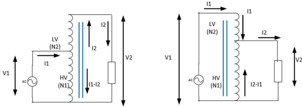
Figure 4.8. Autotransformer operation left is boost, right is buck
