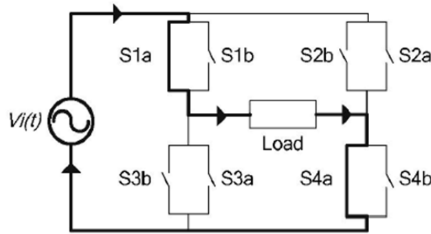
Figure 5.15. SPMC as AC voltage regulator, positive half cycle (Hanafi et al., 2006)
