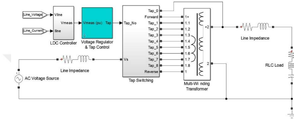
Figure 5.2. Single phase conventional SVR model
