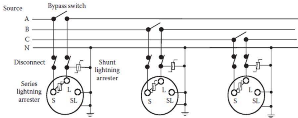
Figure 4.20. Connection of three SVRs for a three-phase, four-wire, multigrounded wye circuit regulation (Colopy, 2012)
