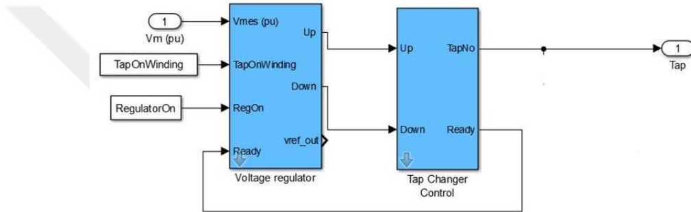
Figure 5.4. Modeling of tap changer control unit
