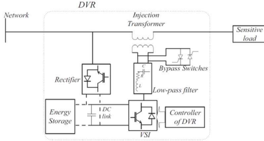
Figure 2.7. Structure of DVR (Taher et al., 2018)
