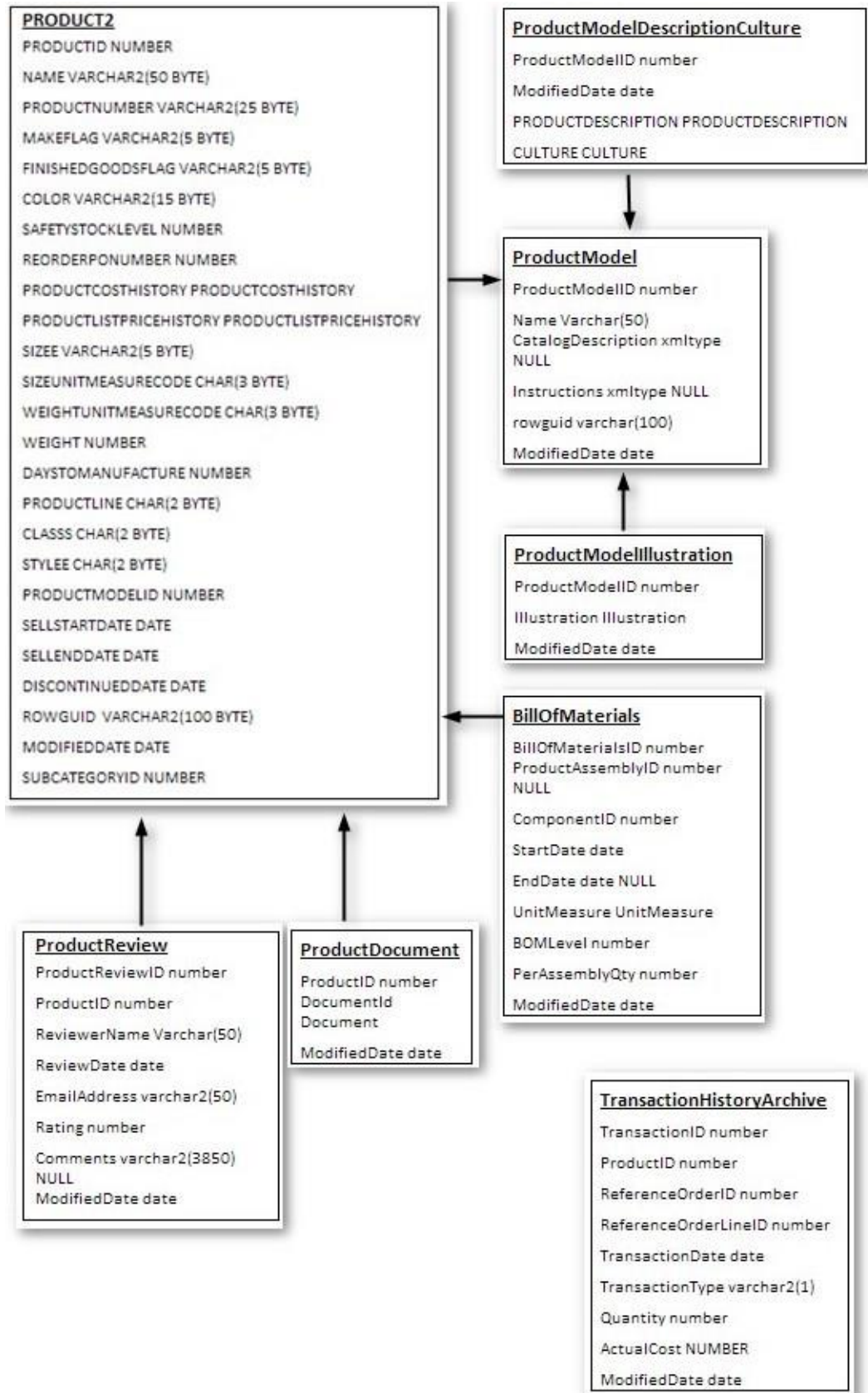
Figure 5.6 Oracle Adventure Works, relational, bitemporal and semi-structured database diagram Part 2
