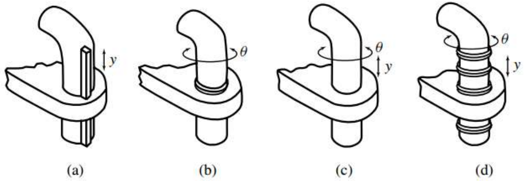
Figure 1.4 Examples of mechanical Joints: a) Prismatic joint b) Revolute joint, c) Cylindrical Joint d) Screw Joint. [2]
