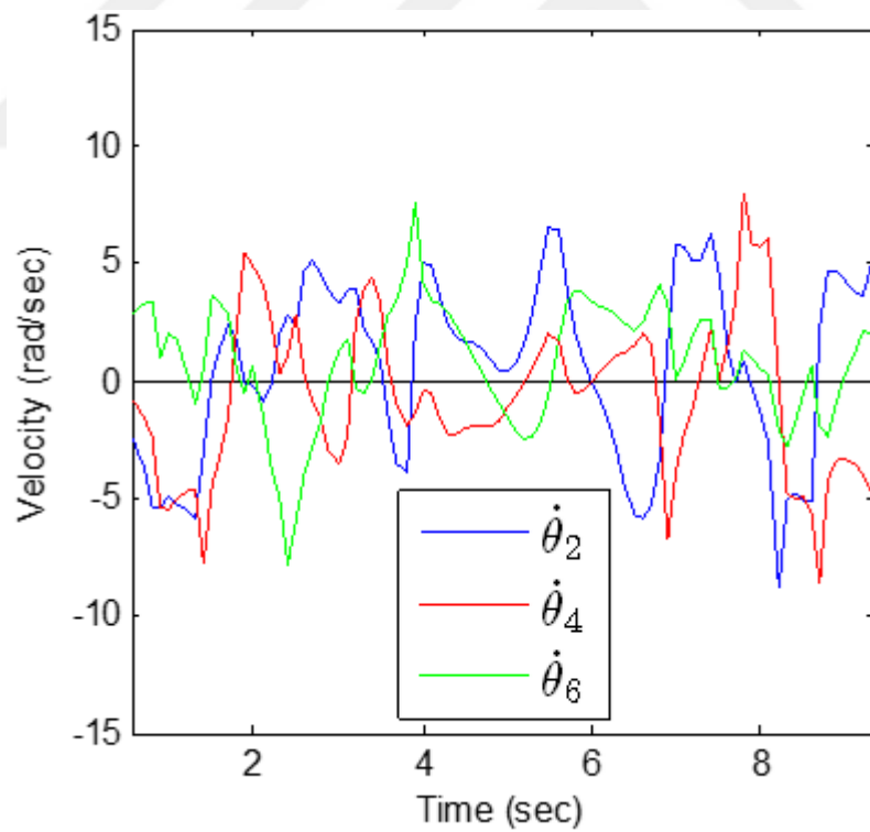
Figure 4.32 Angular velocities of parallel planar manipulator
