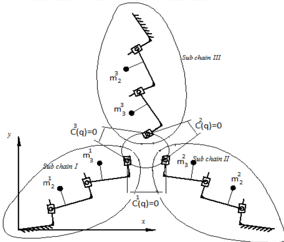
Figure 4.29 Parallel planar manipulator formed by a generalized three PRPR open chain linkage.
