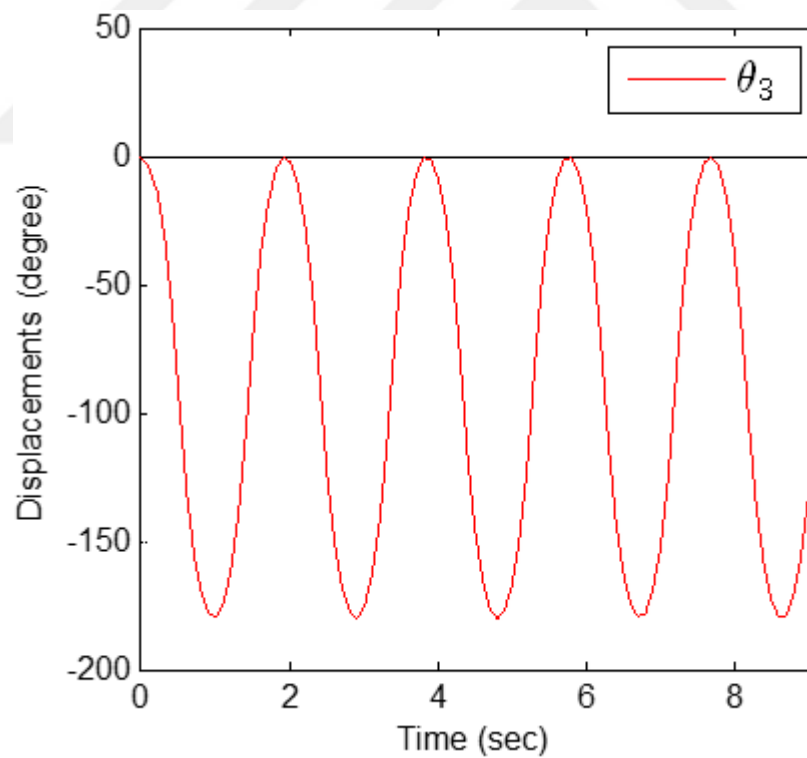
Figure 4.17b Angular displacements of the double slider mechanism
