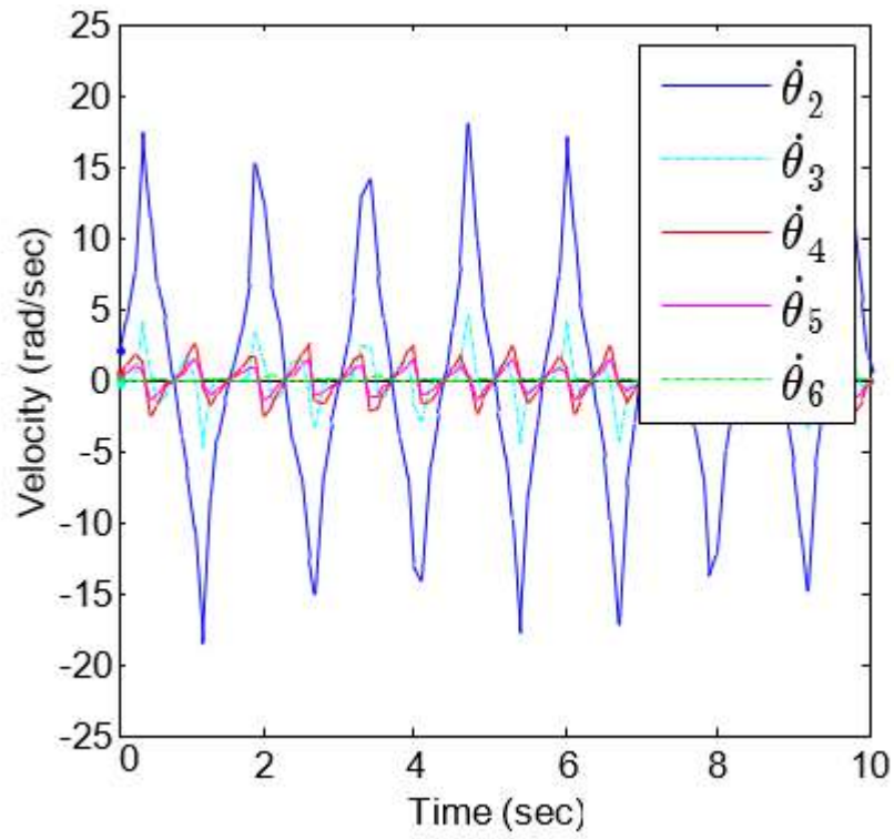
Figure 4.11 Angular velocities of the six bar mechanism
