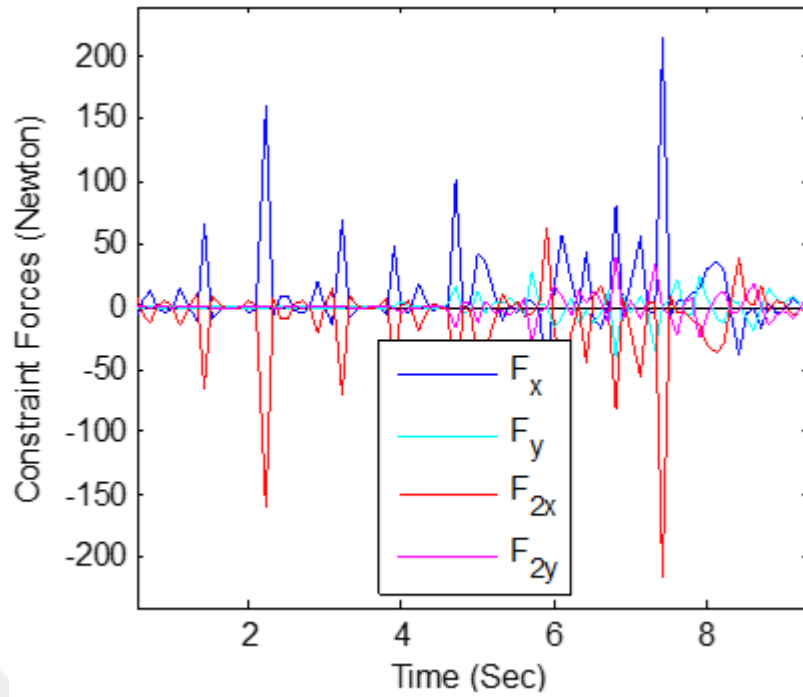
Figure 4.27 Constraint forces of the five bar mechanism at tip points
