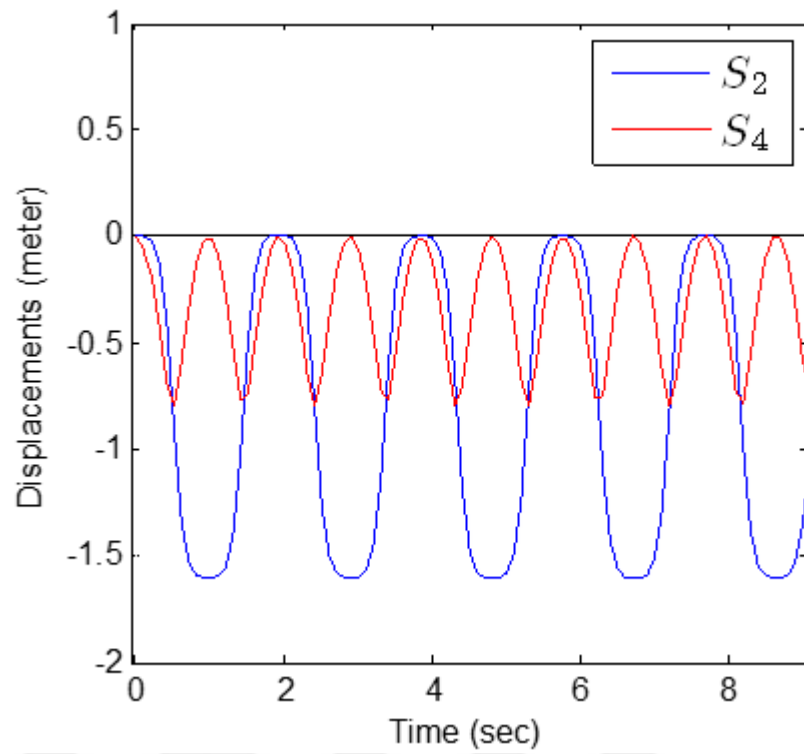
Figure 4.17a Linear displacements of the double slider mechanism
