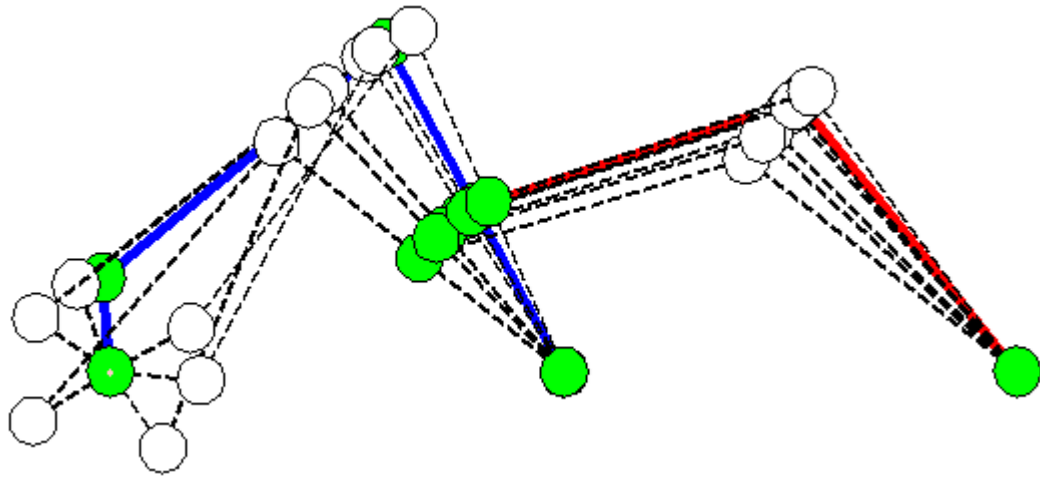
Figure 4.9 Chrono-cyclograph of the six bar mechanism formed by a generalized PRPRPR (first sub chain, drawn in solid line) and a PRPR (second sub chain, drawn in dotted line) open chain linkage.
