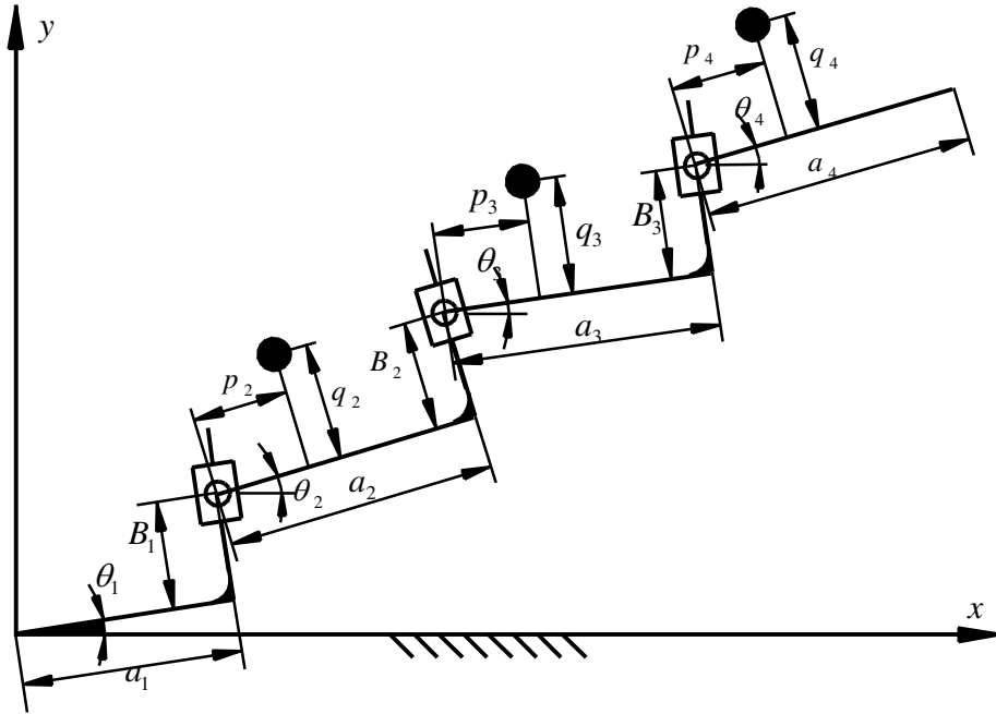
Figure 3.1 Generalized PRPRPR open chain linkage for modeling all possible topologies of open chain planar robot manipulator [26].
