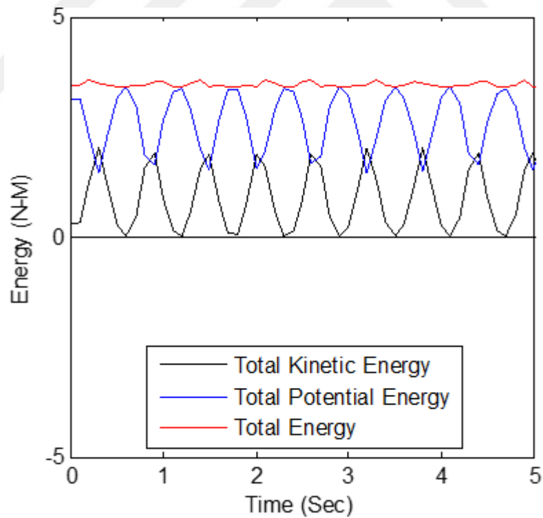
Figure 4.7 Kinetic, potential and total energy of the four bar.
