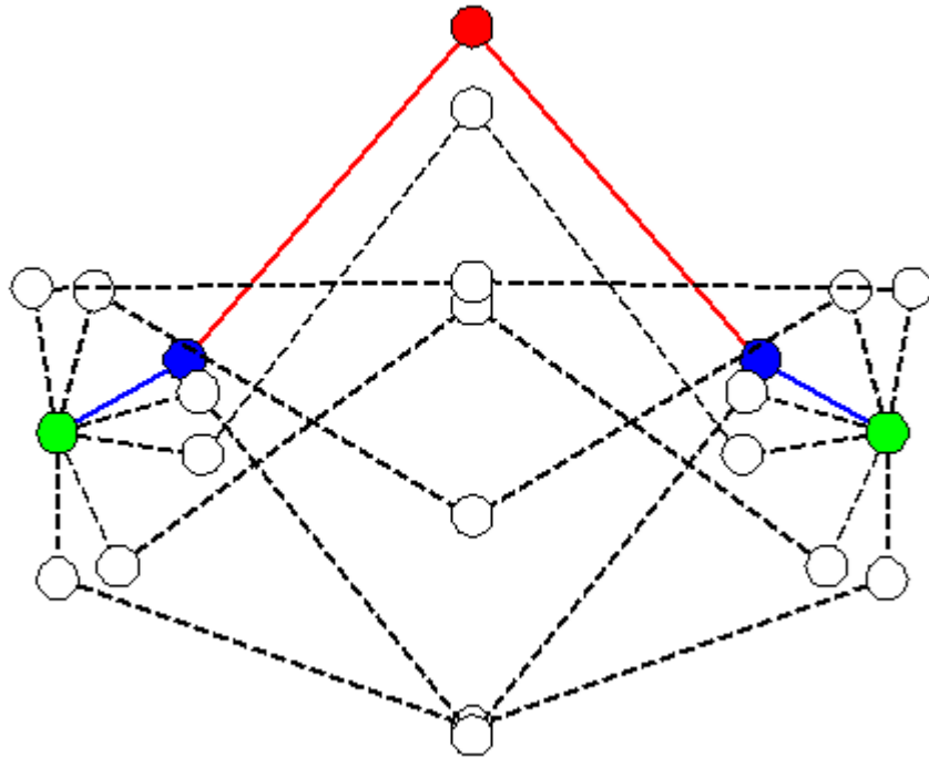
Figure 4.23 Five bar mechanism formed by a generalized PRPR (first sub chain) and a PRPR (second chain) open chain linkage.
