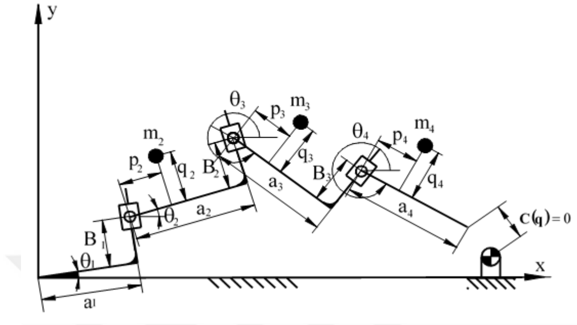
Figure 4.1 Generalized PRPRPR open chain linkage for modeling a four bar.
