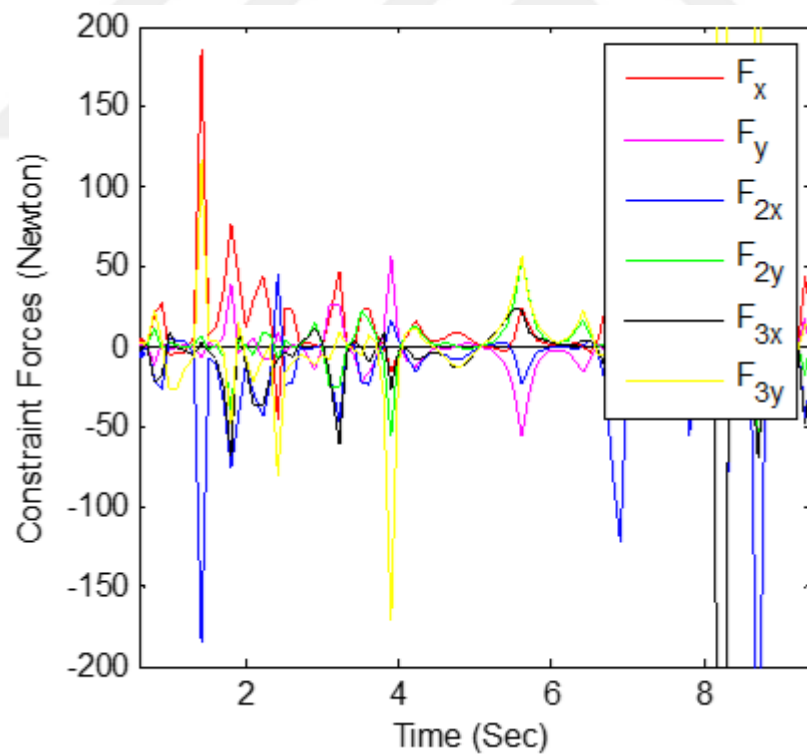
Figure 4.34 Constraint forces of parallel planar manipulator
