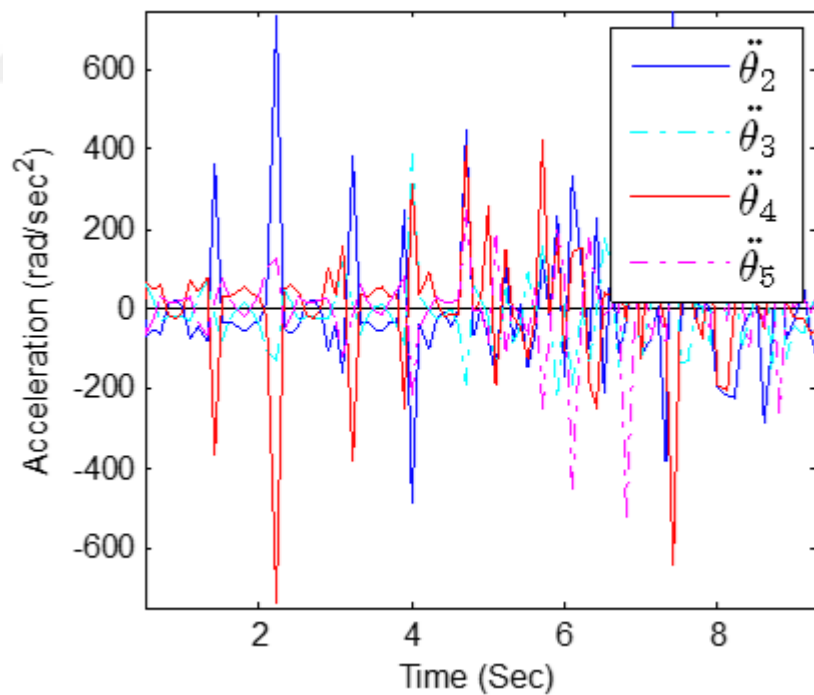
Figure 4.26 Angular accelerations of the five mechanism
