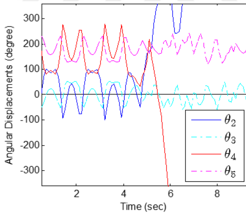
Figure 4.24 Angular displacements of the five bar mechanism
