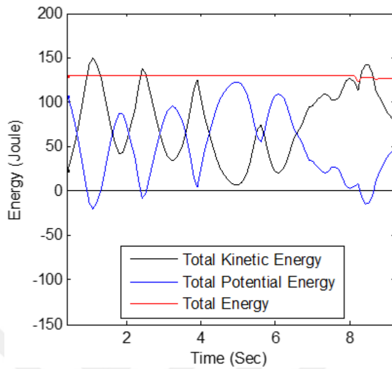
Figure 4.35 Kinetic, potential and total energy of parallel planar manipulator
