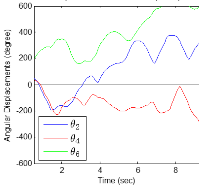
Figure 4.31 Angular displacements of parallel planar manipulator
