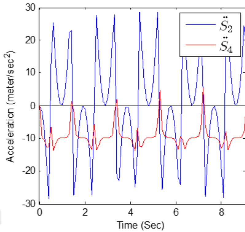
Figure 4.19a Linear accelerations of the double slider mechanism
