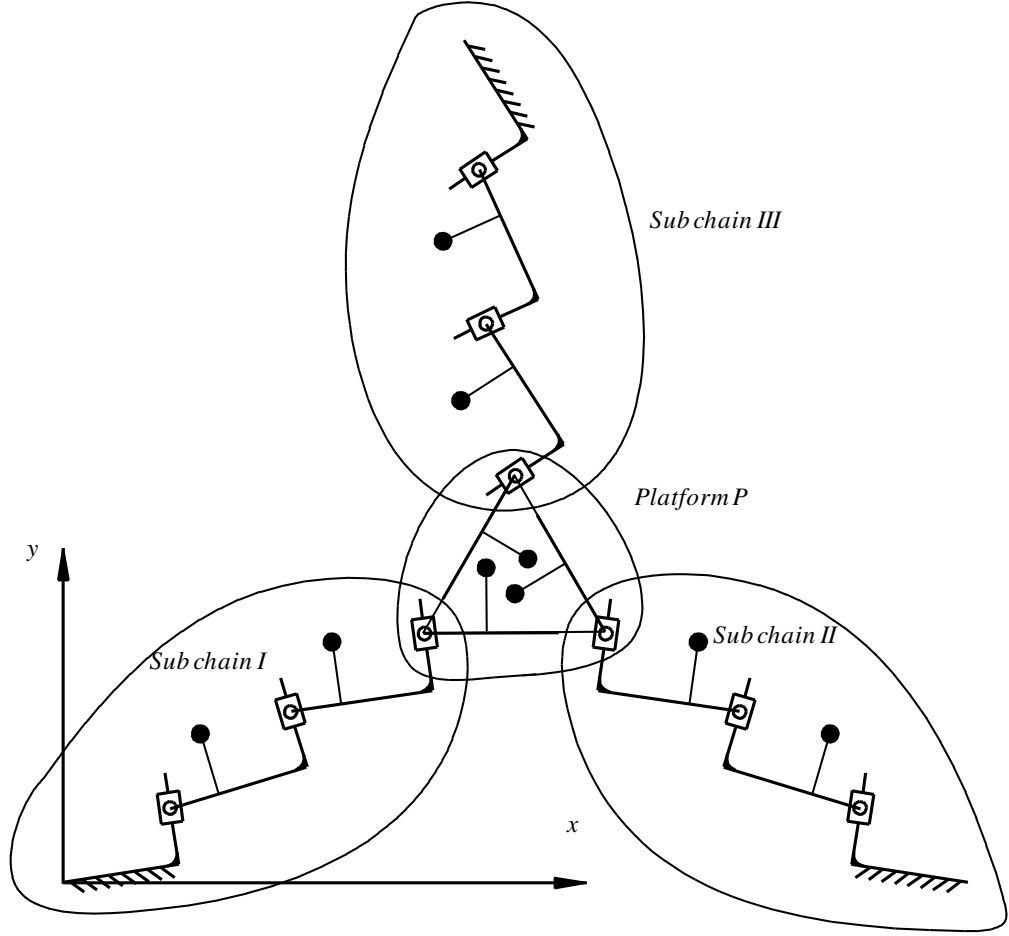
Figure 3.2 A generalized model of planar parallel manipulator with its sub open chains.
