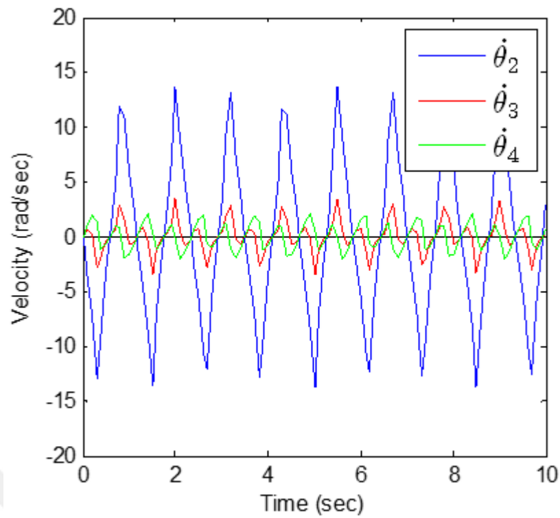
Figure 4.4 Angular velocities of the four bar links.
