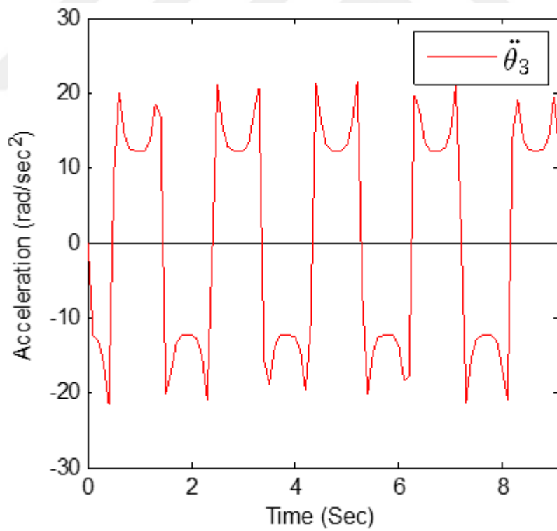
Figure 4.19b Angular accelerations of the double slider mechanism
