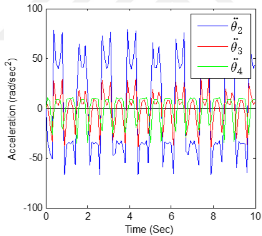
Figure 4.5 Angular accelerations of the four bar links.
