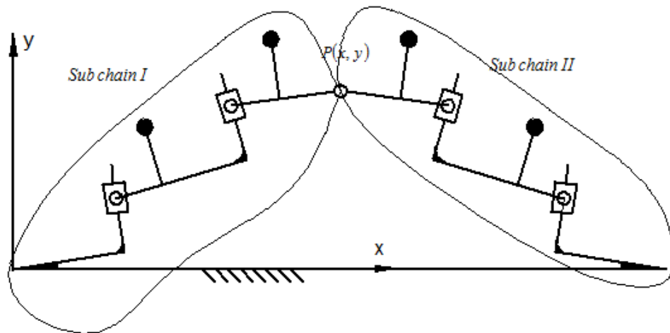
Figure 4.22 Five bar mechanism formed by a generalized PRPR (first sub chain) and a PRPR (second chain) open chain linkage.
