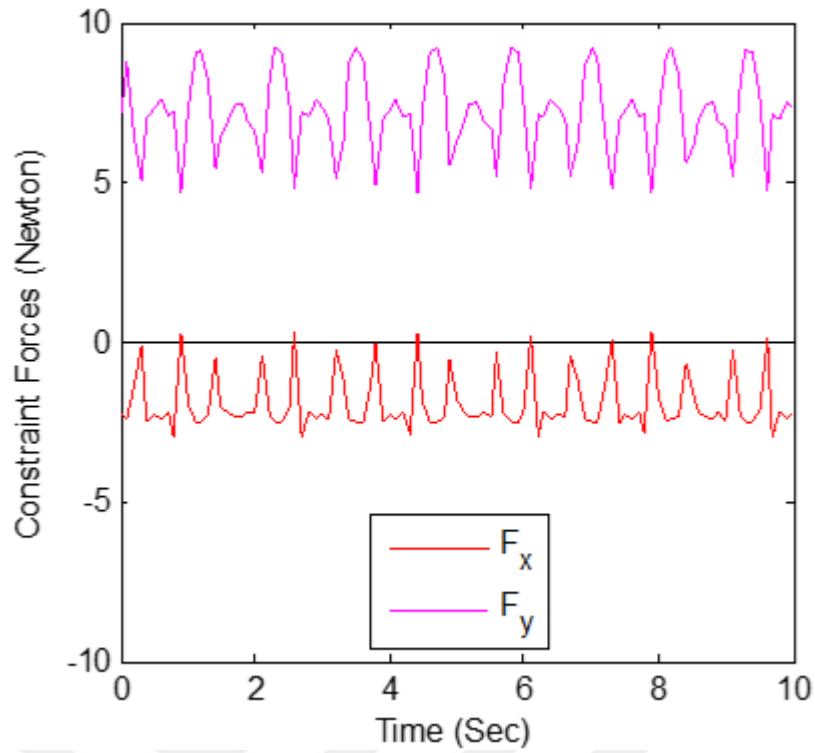
Figure 4.6 Constraint forces of the four bar links at tip points
