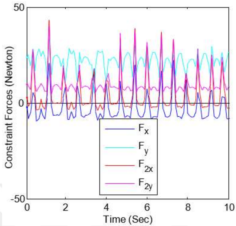
Figure 4.13 Constraint forces of the six bar mechanism links at tip points
