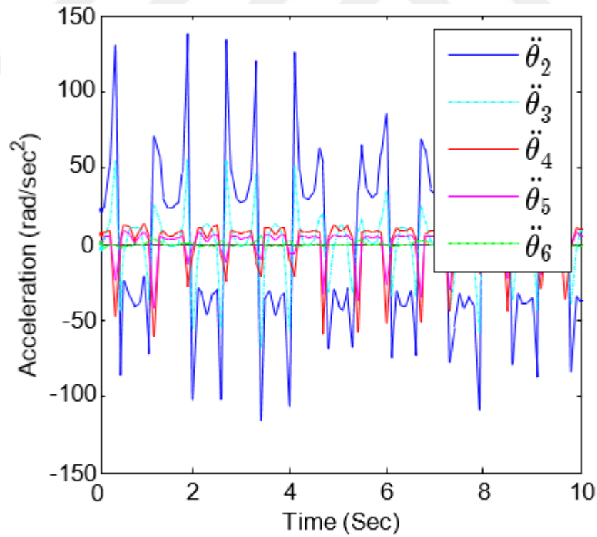
Figure 4.12 Angular accelerations of the six bar mechanism.
