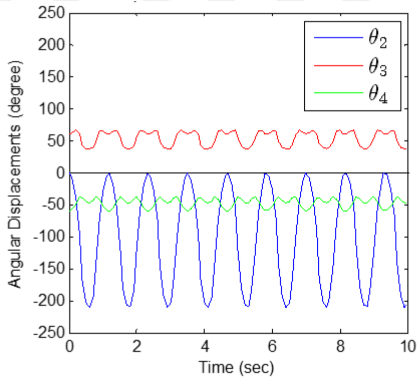
Figure 4.3 Angular displacements of the four bar links.
