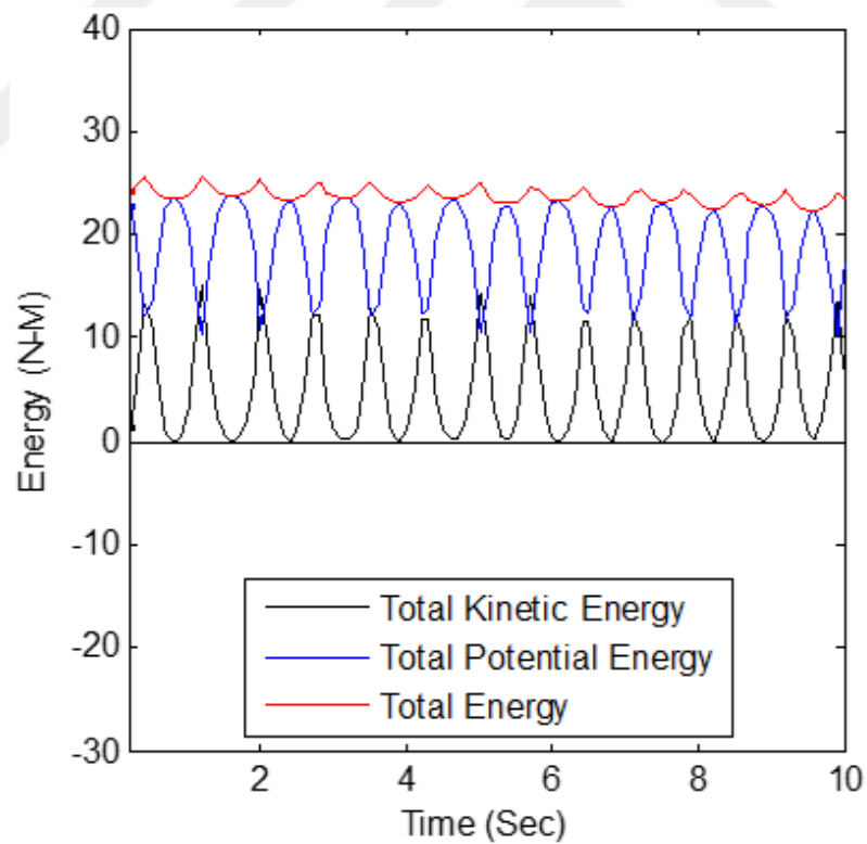
Figure 4.14 Kinetic, potential and total energy of the six bar
