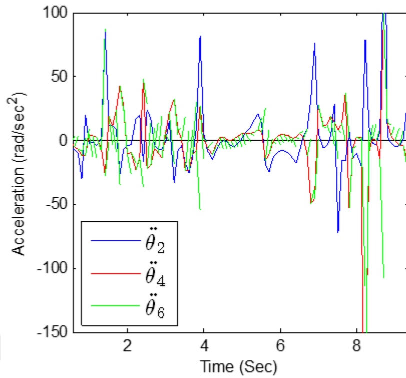
Figure 4.33 Angular accelerations of parallel planar manipulator
