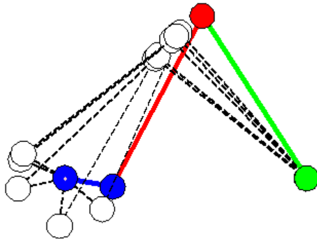
Figure 4.2 Chrono-cyclograph of the four bar.
