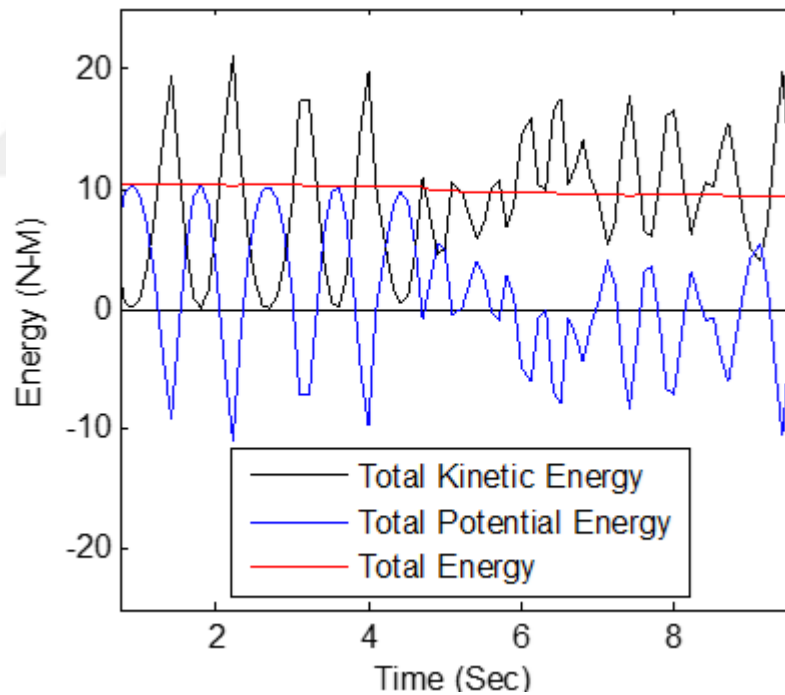
Figure 4.28 Kinetic, potential and total energy of the five bar mechanism
