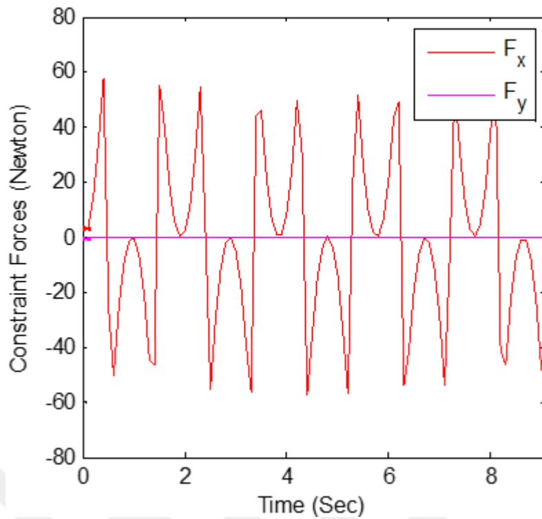
Figure 4.20 Constraint forces of the double slider mechanism at tip points
