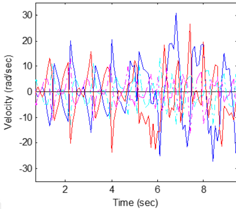
Figure 4.25 Angular velocities of the five bar mechanism
