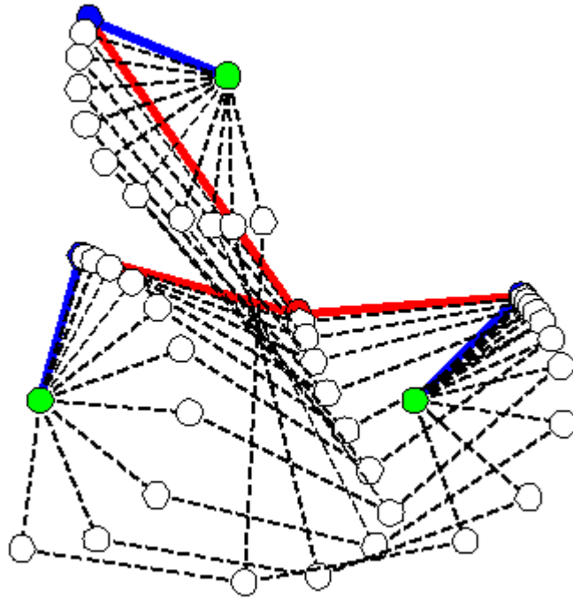
Figure 4.30 Chrono-cyclograph of parallel planar manipulator
