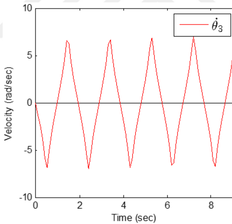
Figure 4.18b Angular velocities of the double slider mechanism
