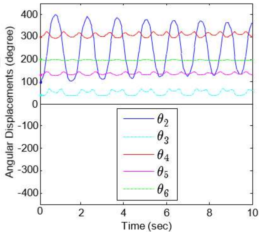
Figure 4.10 Angular displacements of the six bar mechanism.
