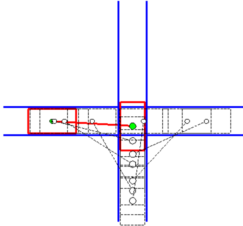
Figure 4.16 Chrono-cyclograph of the double slider mechanism.
