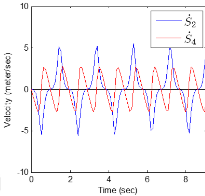
Figure 4.18a Linear velocities of the double slider mechanism
