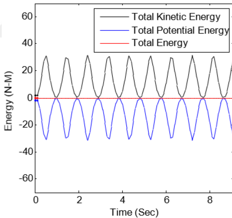
Figure 4.21 Kinetic, potential and total energy of the double slider mechanism
