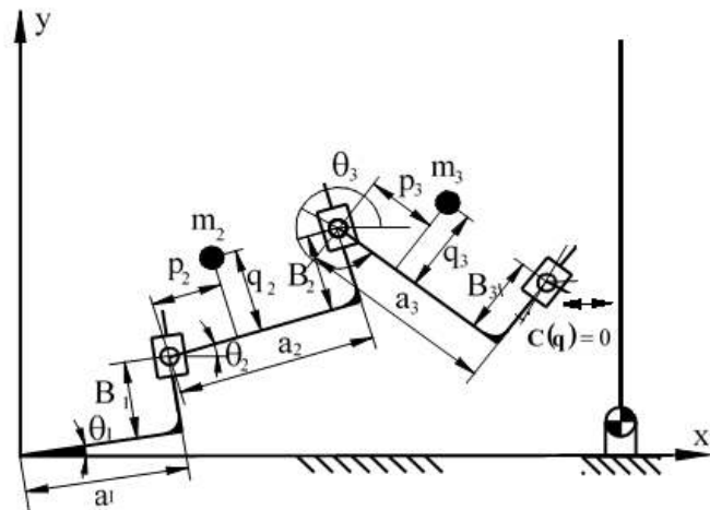
Figure 4.15 Generalized PRPR open chain linkage for modelling a double slider mechanism
