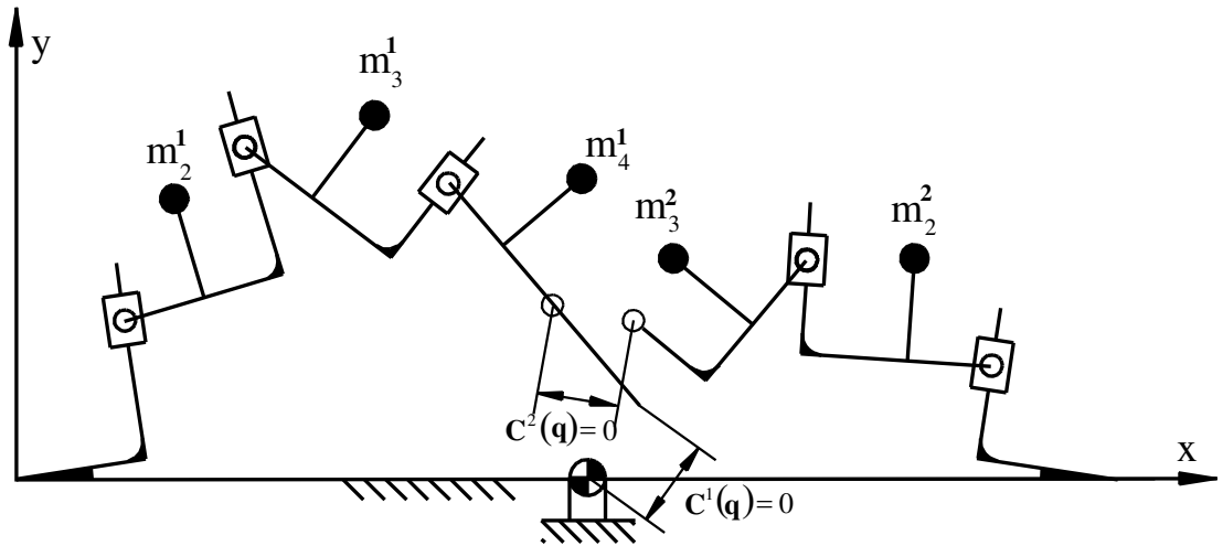
Figure 4.8 Six bar mechanism formed by a generalized PRPRPR (first sub chain) and a PRPR (second chain) open chain linkage.
