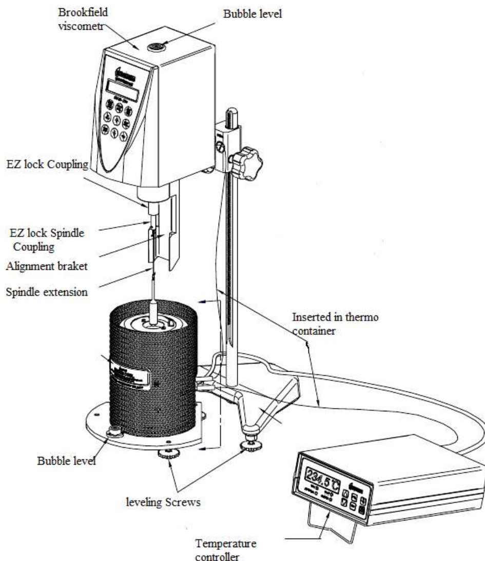
Figure 4.1 Brookfield rotational viscometer
