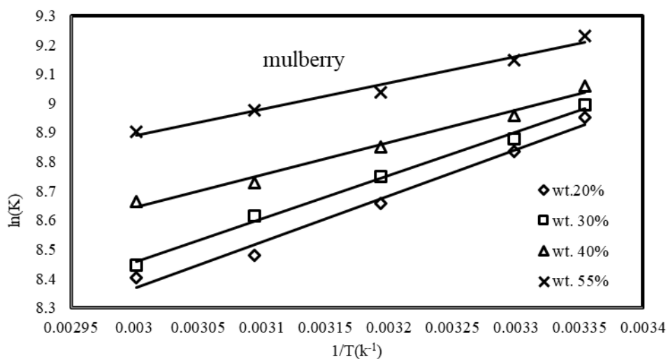
Figure 5.34 Temperature effect on consistency coefficient for the various mulberry molasses concentrations
