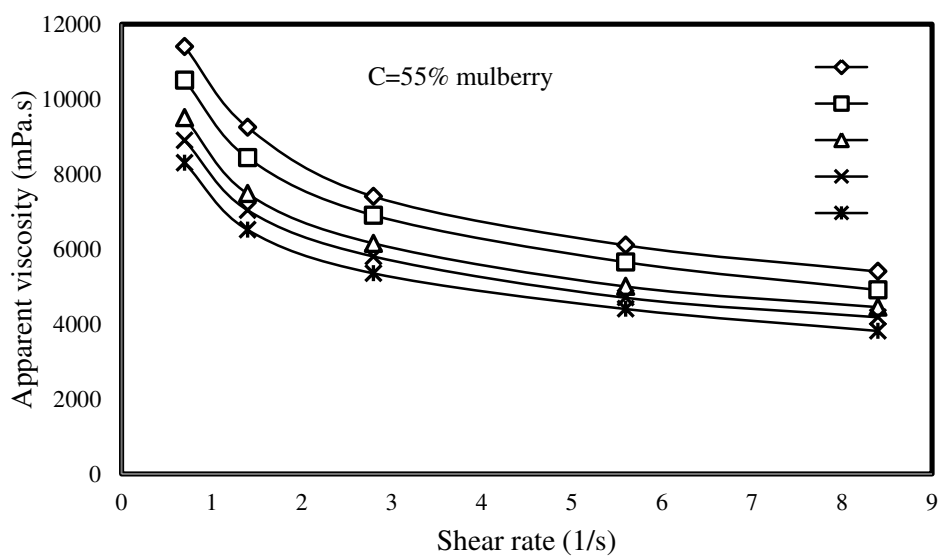
Figure 5.24 Variation of apparent viscosity with shear rates at different temperatures for a 55 % mulberry molasses in sesame paste
