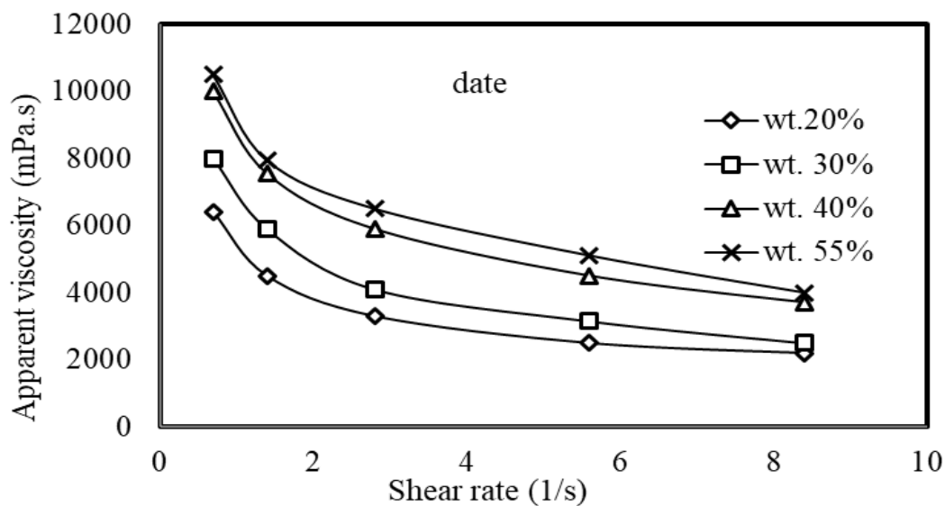
Figure 5.37 Relationships between apparent viscosities and shear rates of date molasses/sesame paste blends at 40°C
