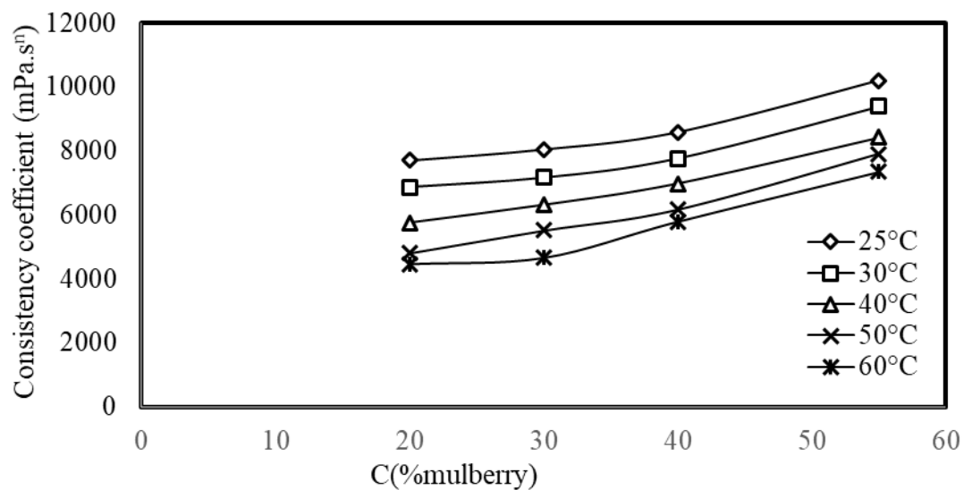
Figure 5.43 The effect of mulberry molasses concentration on consistency coefficients at various temperatures
