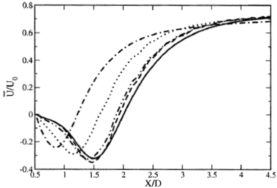
Figure 19: Sensitivity study for the mean streamwise velocity along the wake centerline ( Y/D = 0 ) for a single cylinder at Re_{D,U_0} = 3900 , — case 1; \cdots , case 2; -- case 3; -\cdot- , case 4; and \cdots , case 5. [7]
