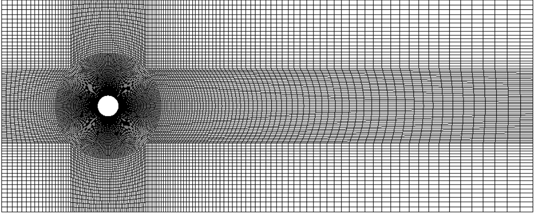
Figure 10: Mesh for Re = 100
