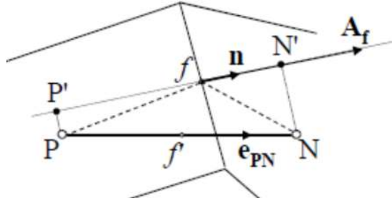
Figure 4: Sketch of geometric parameters [25]
