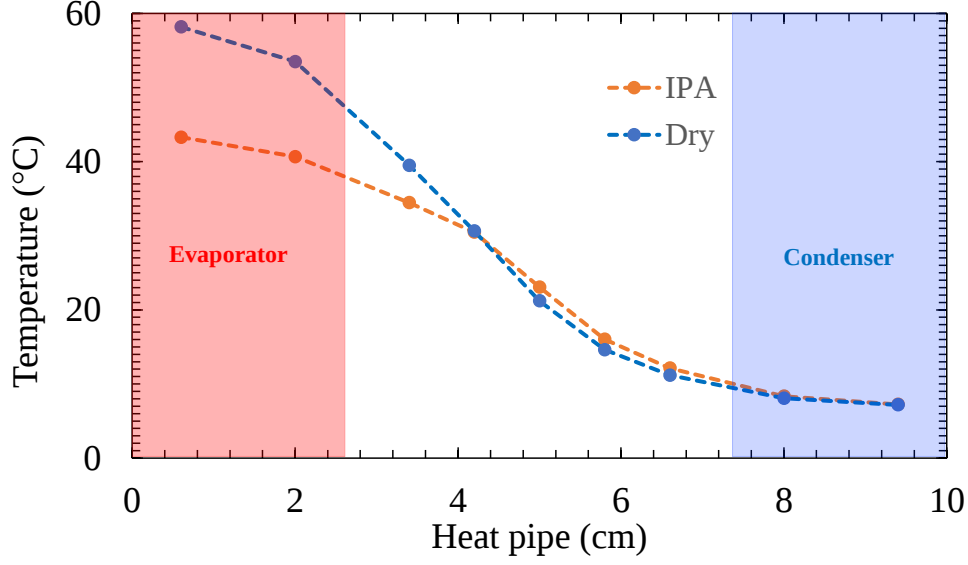
Figure 3.11: Aluminum flat plate heat pipe preliminary experiment
