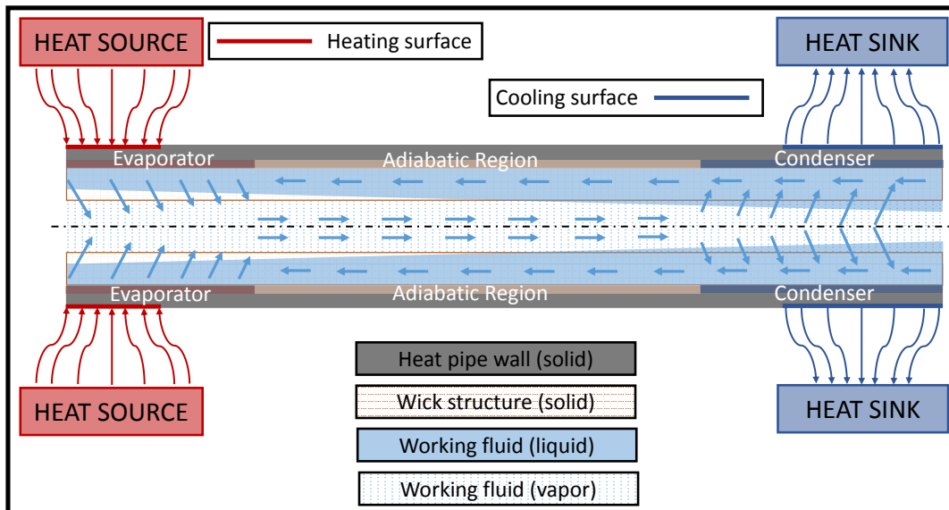
Figure 1.1: Heat pipe working principle
