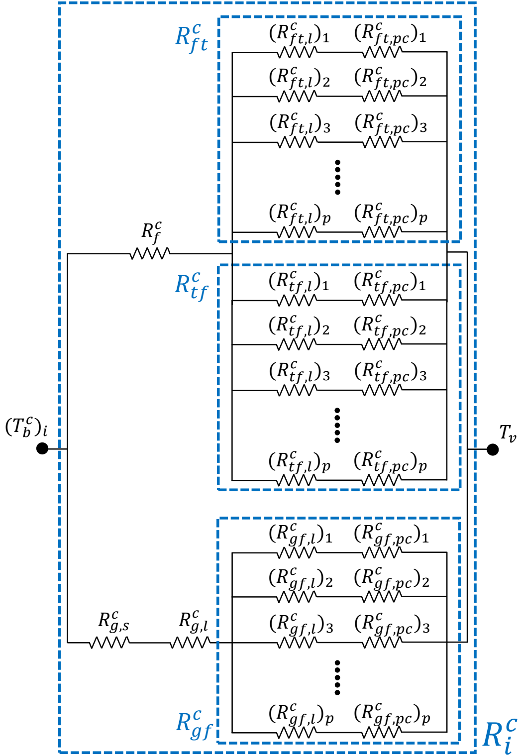
Figure 2.10: Electrical analogy of the thermal resistance network at a condensing section
