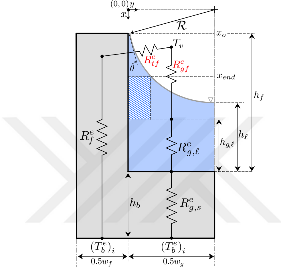
Figure 2.4: Schematic representation of the thermal resistance network at an evaporating section
