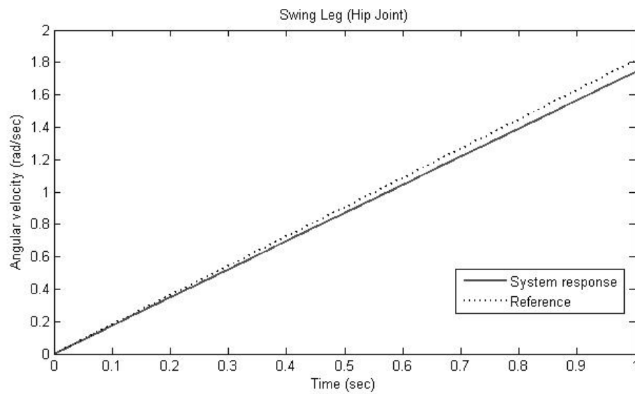
Figure 7.4 Control simulation result for the hip joint of the swing leg. The system response is compared with the reference hip velocity.
