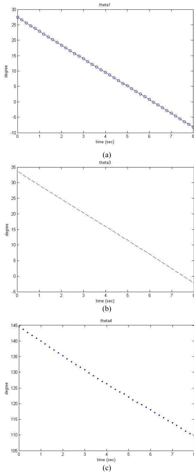
Figure 7.11 Calculated joint variables for the knee mechanism. (a) for \theta_1 , (b) for \theta_3 and (c) for \theta_4 . Walking duration is set to 8 seconds.
