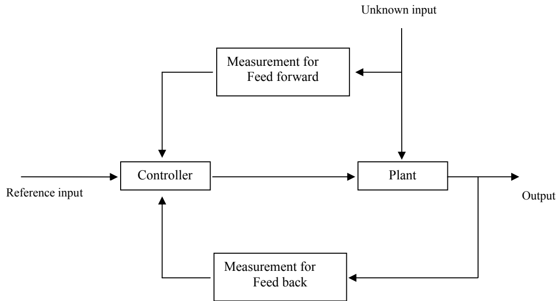
Figure 4.1 System with feed forward and feedback control
