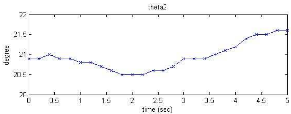
Figure 7.7 Angular change of knee joint variable, which is the reference input to the knee motor of the artificial hybrid leg. Walking duration is set to 5 seconds.
