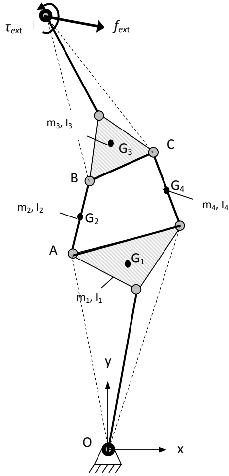
Figure 3.5 Representation of acting forces and torques on the hybrid artificial leg.
