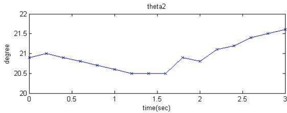
Figure 7.13 Angular change of knee joint variable, which is the reference input to the knee motor of the artificial hybrid leg. Walking duration is set to 3 seconds.
