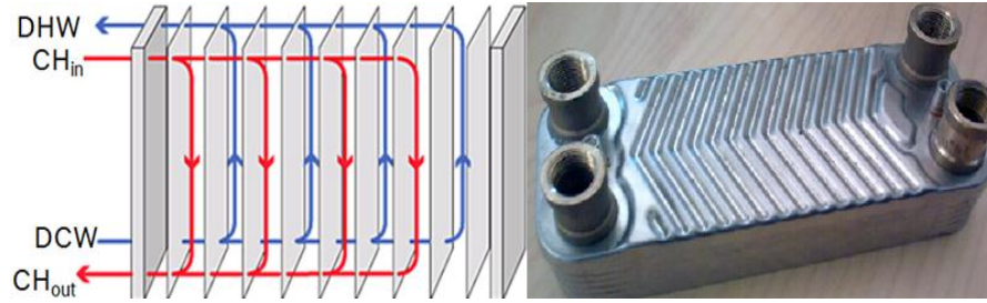
Figure 2.9 Plate heat exchanger and its working principle.
