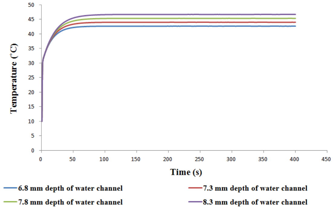
Figure 6.34 Effects of different water channel depths on the flue gas outlet temperature of the primary DHW concept.
