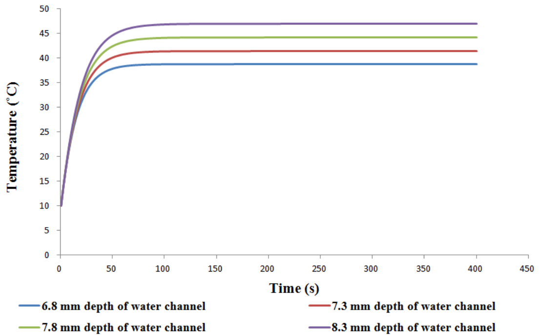
Figure 6.35 Effects of different water channel depths on the wall temperature of the primary DHW concept.
