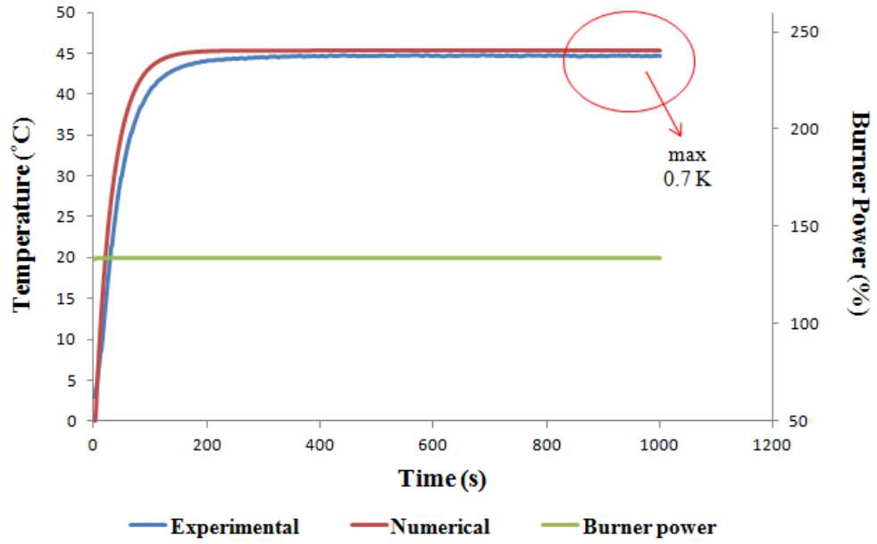
Figure 6.18 Experimental and numerical DHW inlet and outlet temperature difference of the 24-plate PHE and the conical HC combination in eco mode at 8.7 l/min.
