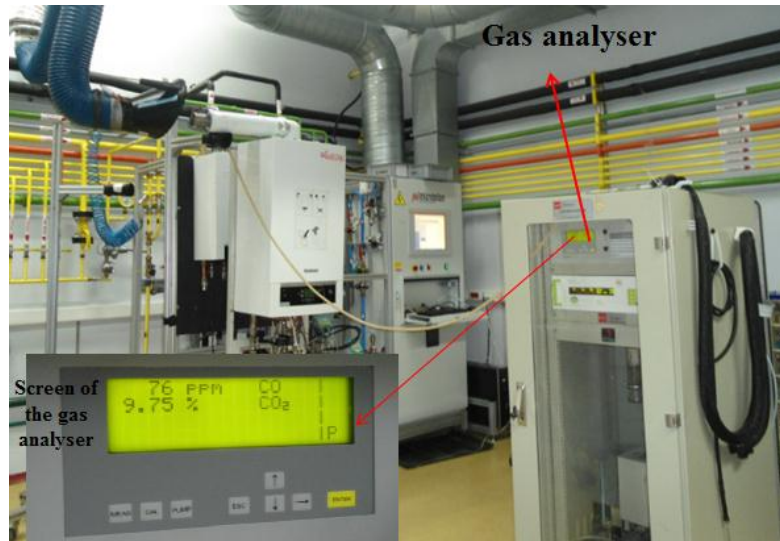
Figure 5.2 Gas analyzer checking the CO and CO 2 level of the appliance.
