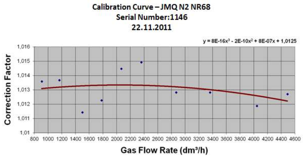
Figure B.1 Calibration curve of the gas meter
