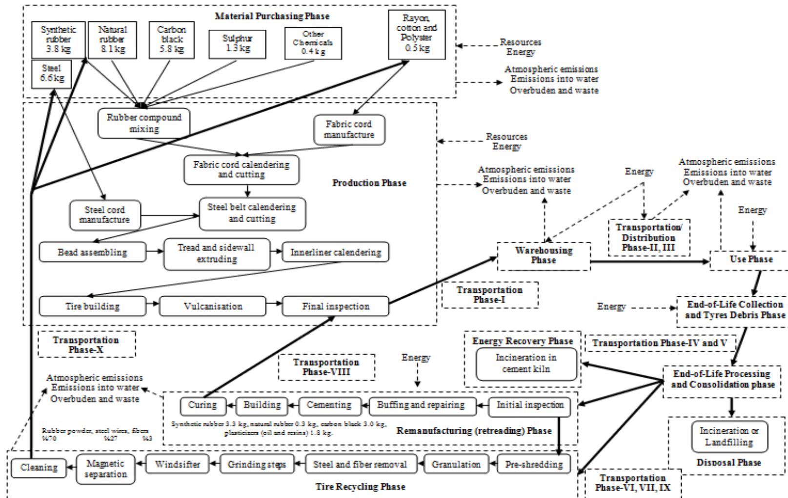
Figure 5.5 LCA boundries and process tree of a tire throughout the different life cycle phases
