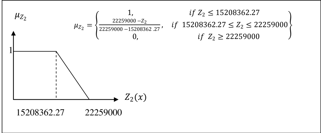
Figure 5.23 Modified membership function of fuzzy minimum Z_2 (in iteration 2)
