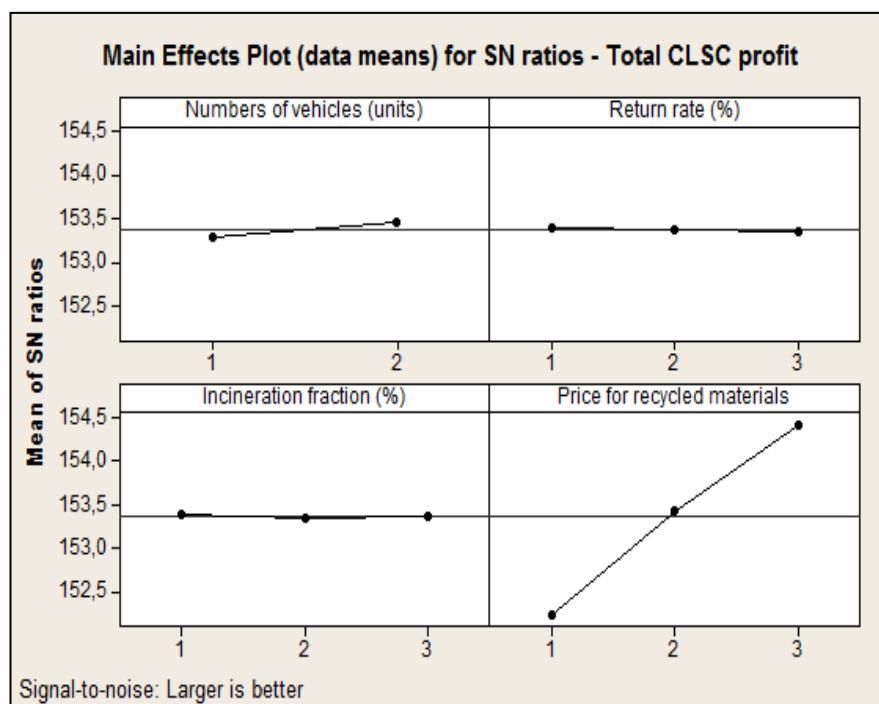
Figure 5.28 The main factor effects obtained from S/N ratios for total CLSC profit in case-1
