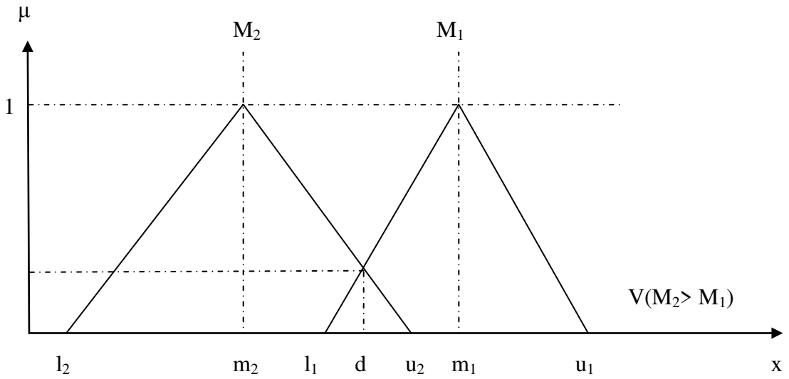
Figure 4.10 The intersection between M_1 and M_2 (Ozdaglu, 2007; Zhu, Jing, and Chang, 1999)
