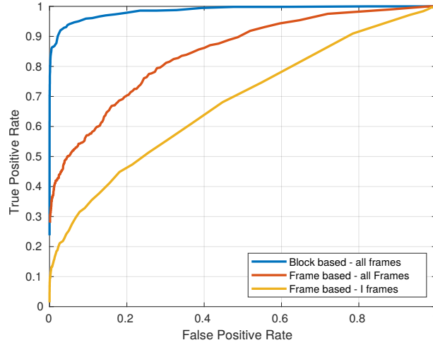
Figure 4.18. Computed ROC curves for all natural non-stabilized YouTube videos at 1080p in vision dataset - natural vs. natural
