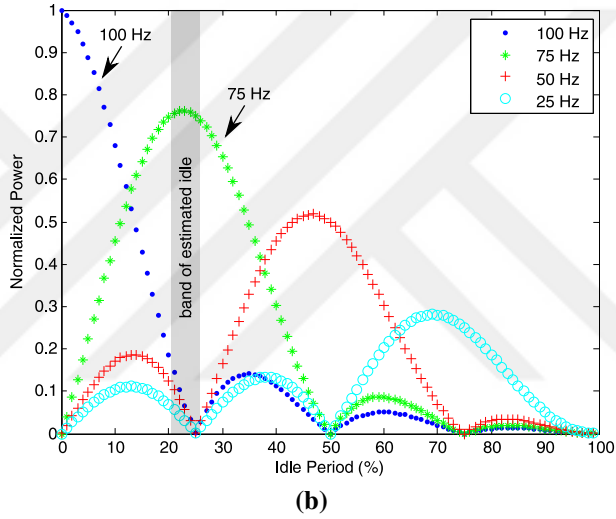
Figure 4.15. (a) Fourier Spectrum obtained for the 25 fps- 720p video taken by the Nikon D3100, video-6; (b) constructed model of reference: variation in position of the primary ENF harmonic depending on idle duration in the same video - the range of idle duration was obtained between 20% and 25% - alias ENF is detected at DC component for this frame rate, hence idle period for this case cannot be estimated via the vertical phase method
