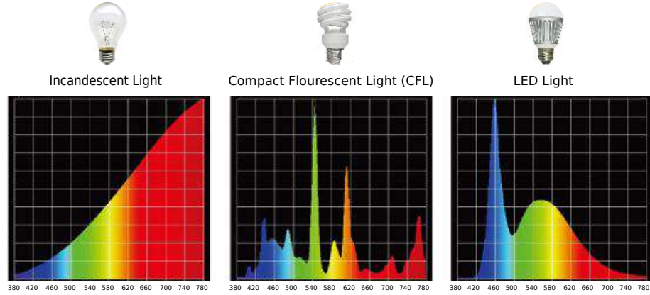
Figure 4.17. Spectra for different light sources
