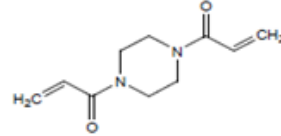
1,4-bisakrilol Piperazin
