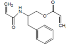
N,O-bisakrilol Fenilalaninol
