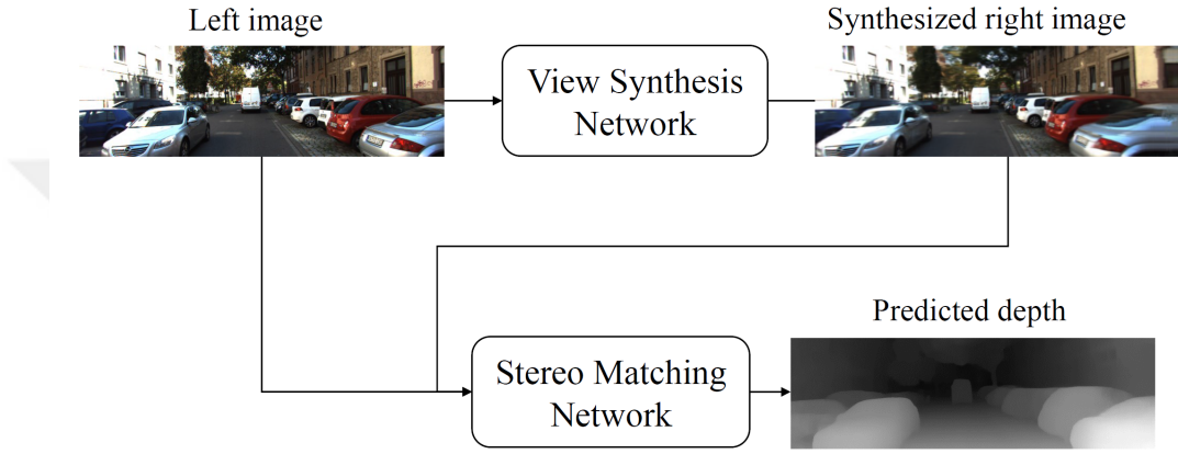
Figure 2.13: Luo et al. [15]'s Network Architecture.
