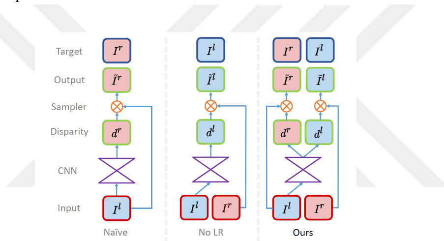
Figure 2.8: Godard et al. [10]'s left-right consistency check method.
