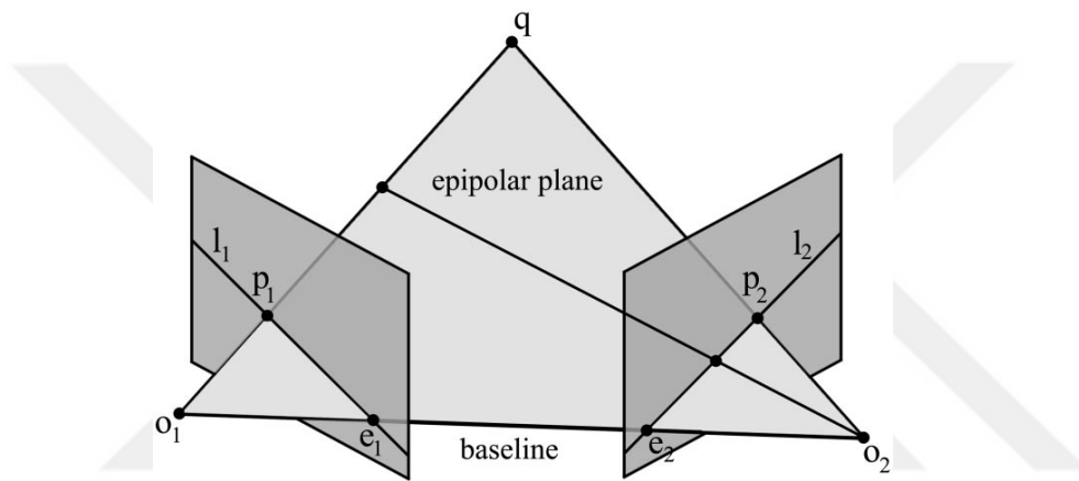
Figure 2.1: Epipolar Geometry [3].
