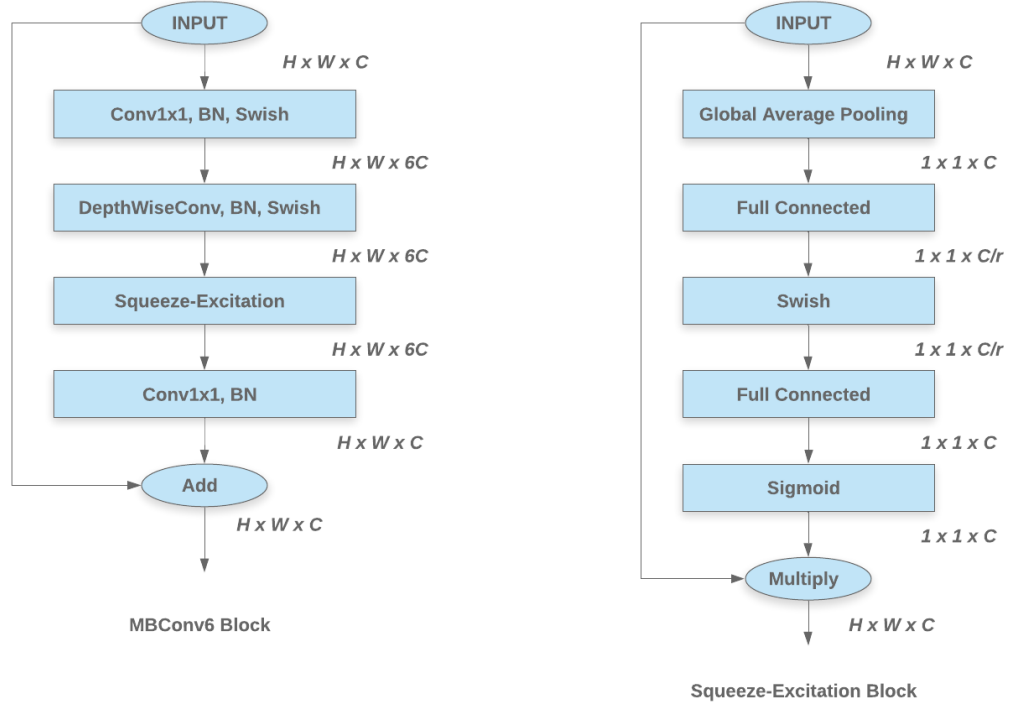
Figure 2.17: MBConv6 Block and Squeeze-Excitation Block
