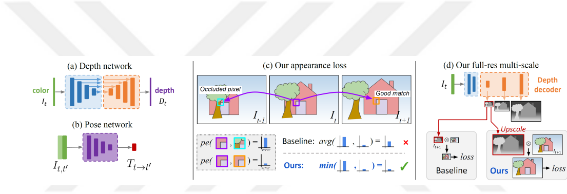
Figure 2.11: Godard et al. [13]’s Network Architecture (Monodepth2).
