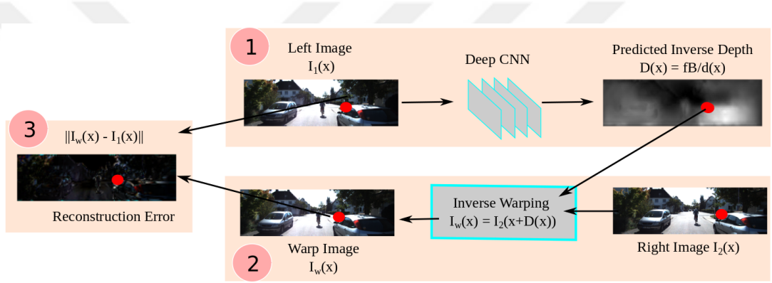
Figure 2.7: Garg et al. [9]'s training method.
