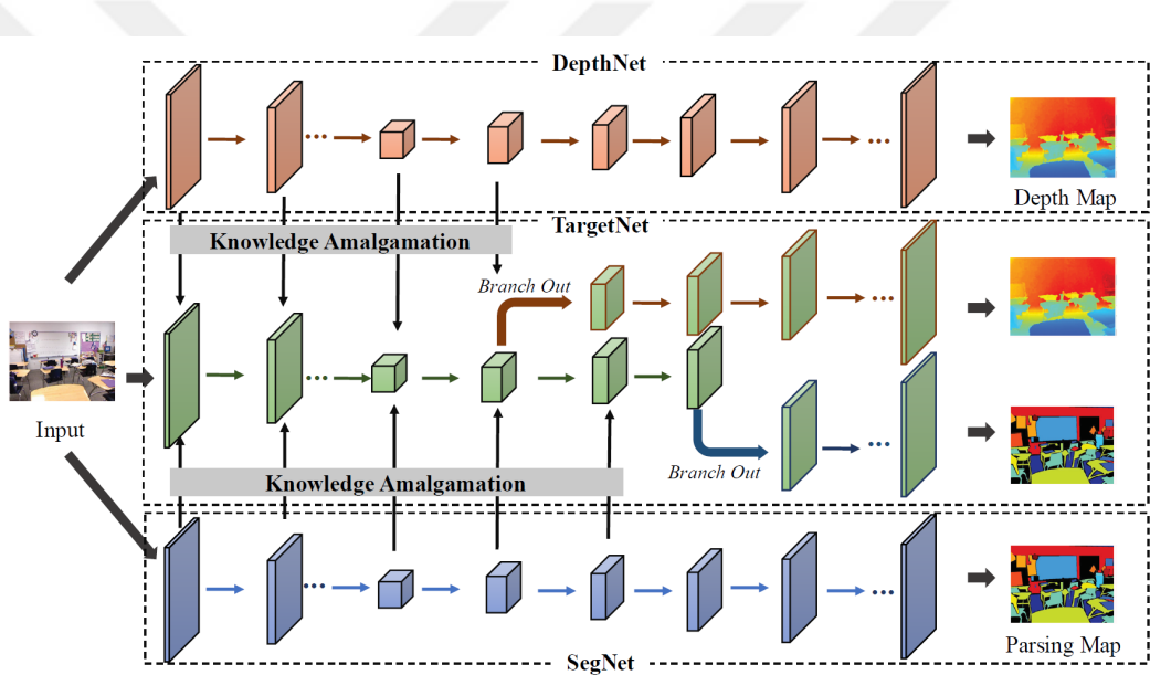
Figure 2.20: Ye et al. [20]’s network structure.
