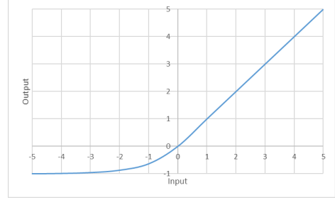
(b) eLU Activation Function
