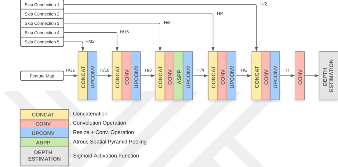
Figure 3.4: Decoder structure used in our network.
