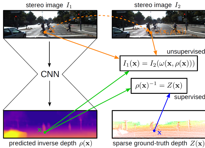
Figure 2.12: Kuznetsov et al. [14]'s Network Structure.
