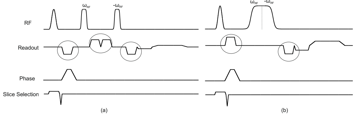
Figure 4.1: MR flow imaging pulse sequences using B_1 gradients and Bloch Siegert shift. Note that crusher gradients are indicated by the circles.
