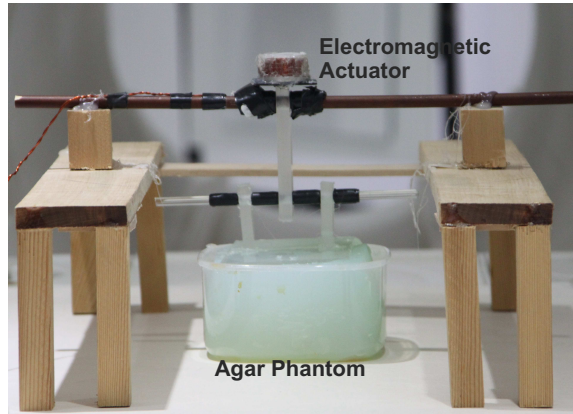
Figure 4.9: MR elastography setup using electromagnetic actuator, direction of the motion is along the z-axis.
