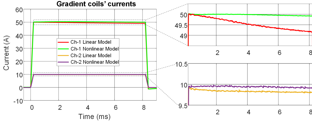
Figure 3.7: Experiment results. The comparison of the coils' currents generated using the linear and nonlinear models. The reference inputs are trapezoid waveforms with the amplitude of 50A and 10A for ch-1 and ch-2, respectively. Both channels have the same rise time ( 200\mu s ).
