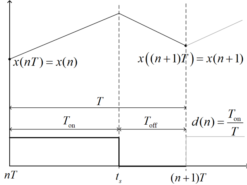
Figure 3.2: A single circuit variable (the inductor current, for example) time dependence over a period of PWM ( T ) with the PWM's on and off duration. The duty cycle, d(n) , is defined as the ratio of T_{on} to ( T ).
