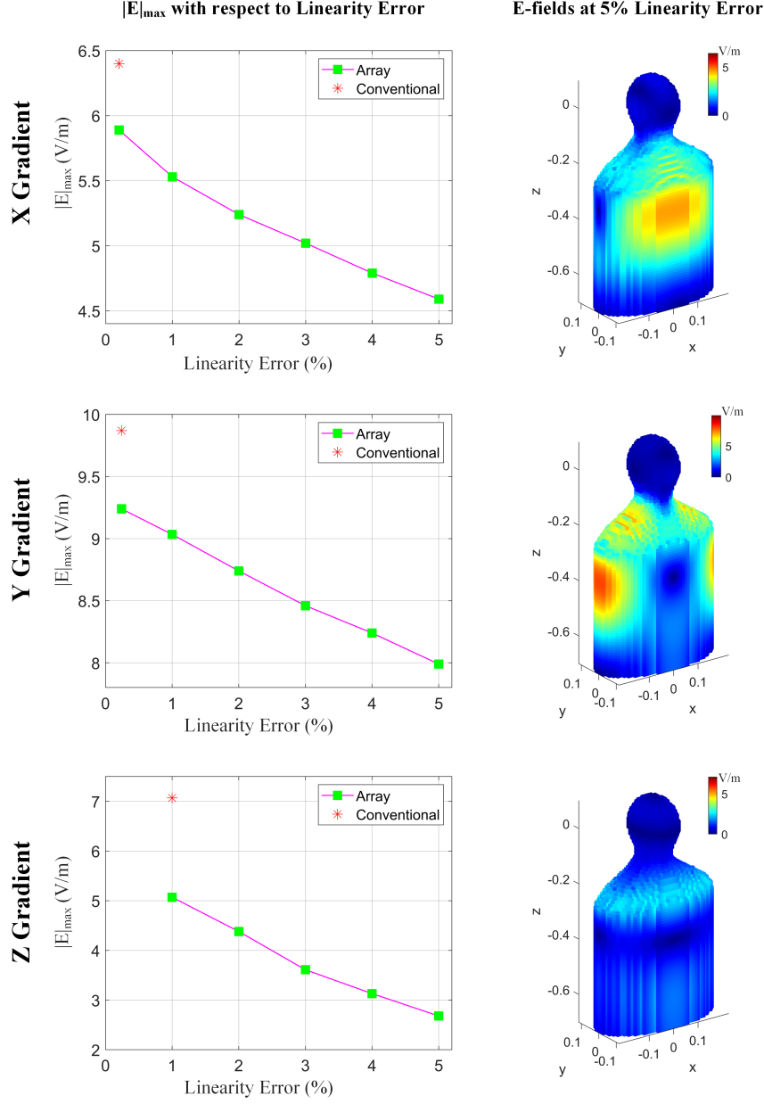
Figure 2.9: The left column depicts the |E|_{\max} with respect to the linearity error. Conventional designs have almost perfect linearity in a small ROL (120mm). The gradient array coil can generate the desired gradient with the same linearity while the induced E-field is minimized. By optimizing the feeding current with different linearity errors, it is possible to reduce the E-fields even further. The right column displays the E-field for X, Y, and Z gradients (array) at a 5% linearity error.
