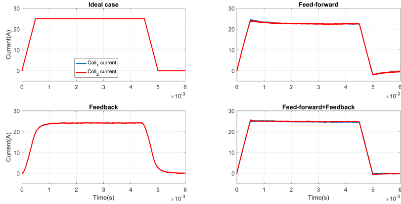
Figure A.3: Experiments: gradient coil current for feed-forward only, feedback only, and feed-forward+feedback controllers.
