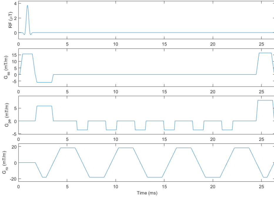
Figure 4.3: Part of a single TR for a single slice of the multi-shot EPI pulse sequence used for imaging. The next shot for the same slice is scanned 156 ms later, making the effective TR for a single slice 156 ms. The next slice is scanned immediately after, which allows maximum use of the readout gradient.
