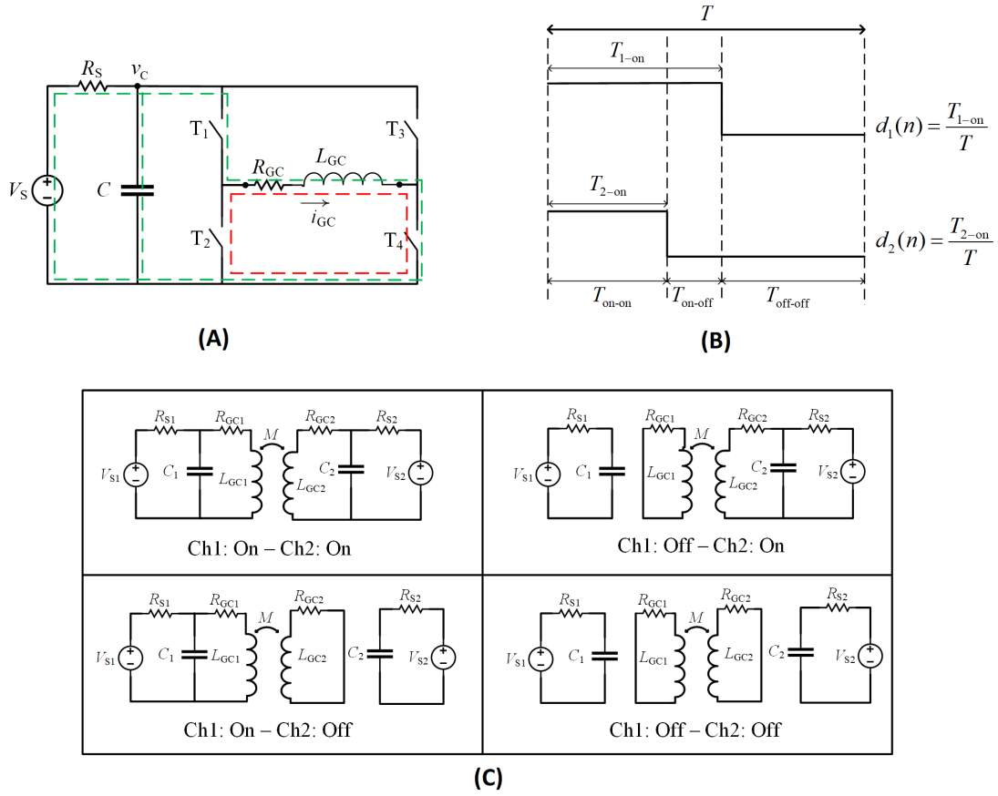
Figure 3.3: (A) single-channel gradient system circuit including amplifier, power supply with parallel decoupling capacitor, and the gradient coil. The green path shows the circuit during T_{\text{on}} , and the red one is for T_{\text{off}} . (B) PWMs for channel1 and channel2 assuming d_1 > d_2 and (C) Different states of two-channel system circuit which covers any combination of d_1, d_2 .
