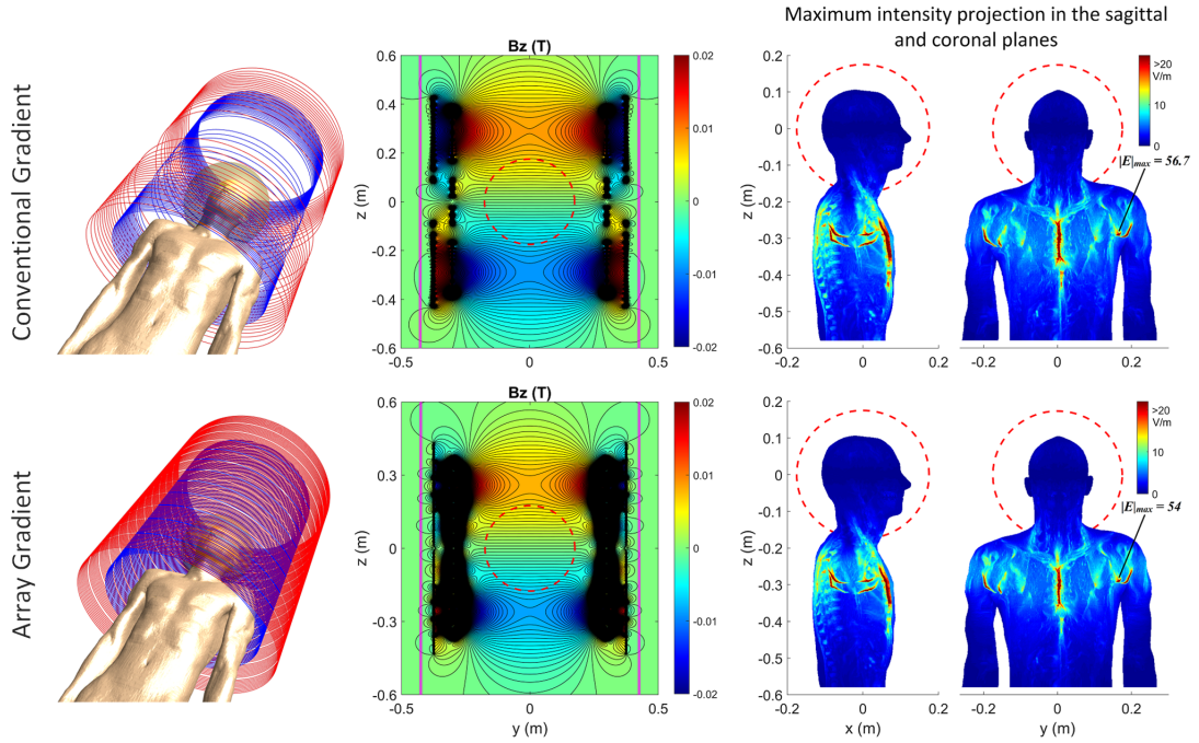
Figure 2.4: Comparison of conventional and array coils. Both coils have almost similar performance. The current RMS for the conventional and array coils are 330A and 350A, respectively.
