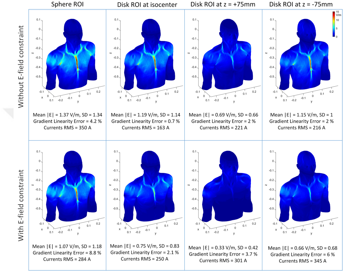
Figure 2.7: Comparison of average induced E-fields within body volume.
