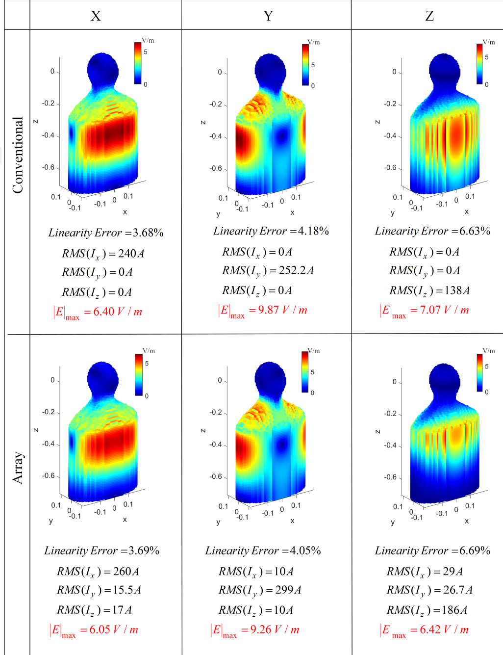
Figure 2.8: Comparison of gradient array and conventional coil. The maximum linearity error is the same for both designs; however, by using a slightly higher current RMS in the array coil, the maximum E-field is reduced for all three gradients.
