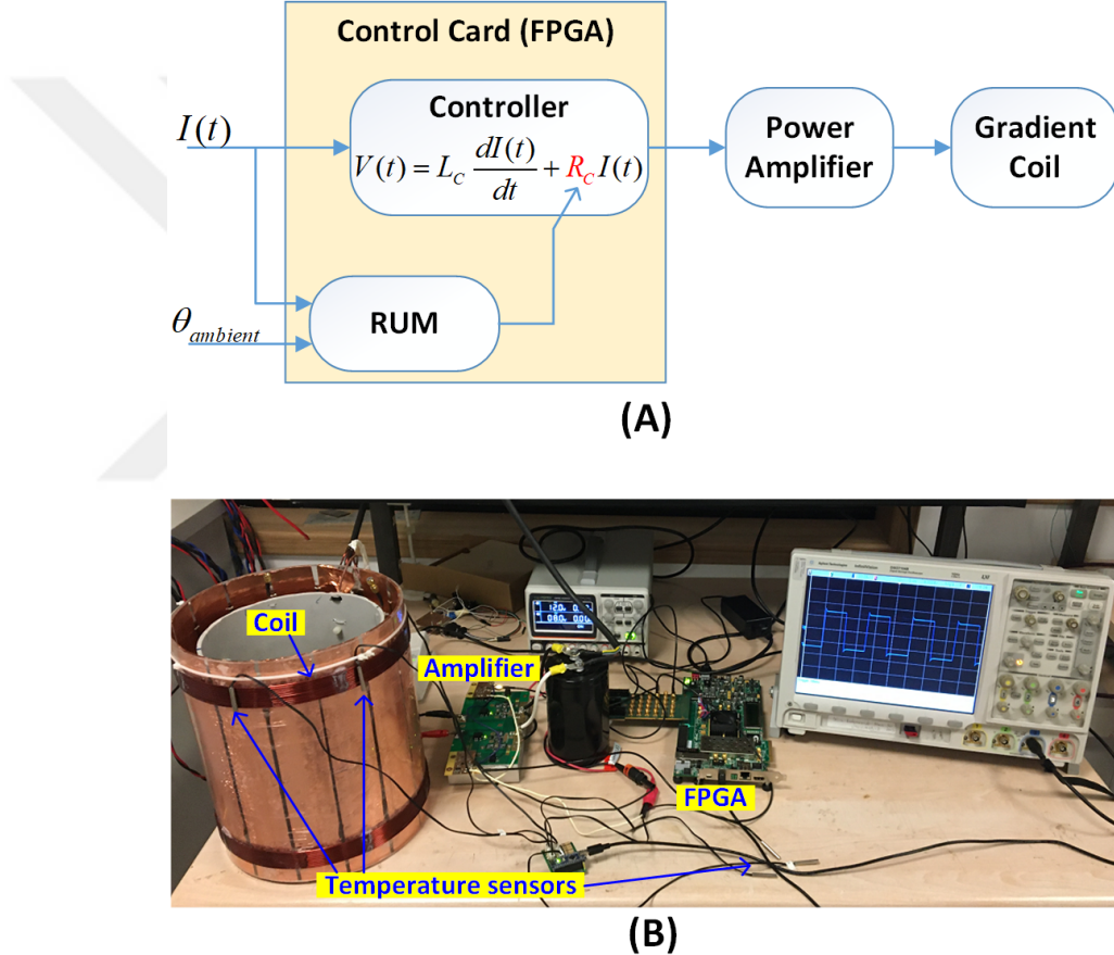
Figure 4.1: (A) the block diagram of gradient system with feed-forward controller, including the updating block. (B) Measurement setup. There are six temperature sensors; three of them measure the coil winding temperature, and the other three measure the ambient temperature. The average temperature is used in calculations.
