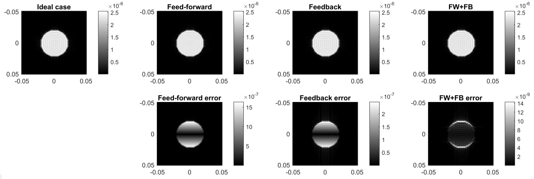
Figure A.4: Image simulations, ideal case and for each controller (first row), difference images (second row).
