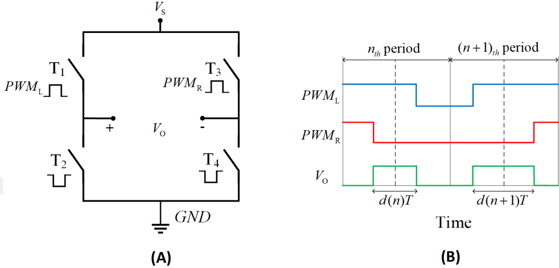
Figure 3.1: (A) Full-bridge power amplifier configuration (B) The center-aligned approach for two periods of PWM. The waveforms for the high-side transistors ( T_1 and T_3 ) are shown in the figure. The low-side transistors ( T_2 and T_4 ) are switched with the complementary logic.
