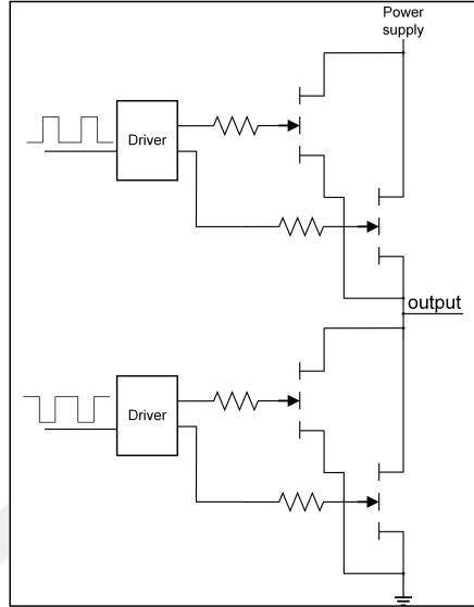
Figure B.1: Simplified circuit diagram of 150V/50A half-bridge for gradient array applications using eGaN transistors. Two parallel transistors are used as a switching element. Two of these modules are used for one full bridge driver.
