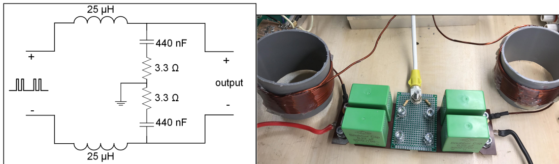
Figure B.2: Circuit diagram and fabricated differential one stage LC filter. Cut-off frequency is about 50kHz to attenuate ripple current with 1MHz frequency. Capacitor values are decreasing towards our switching frequency which degrades attenuation ratio.
