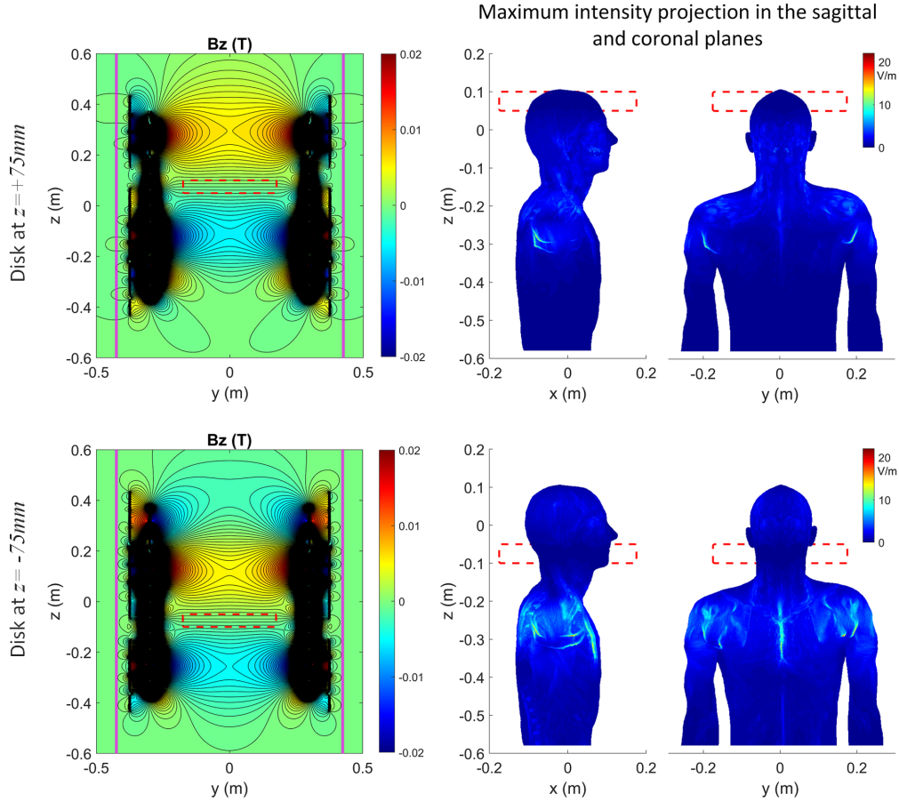
Figure 2.6: B-field and E-field of array coil when optimized for a disk-shaped ROL at z = +75mm and z = -75mm .
