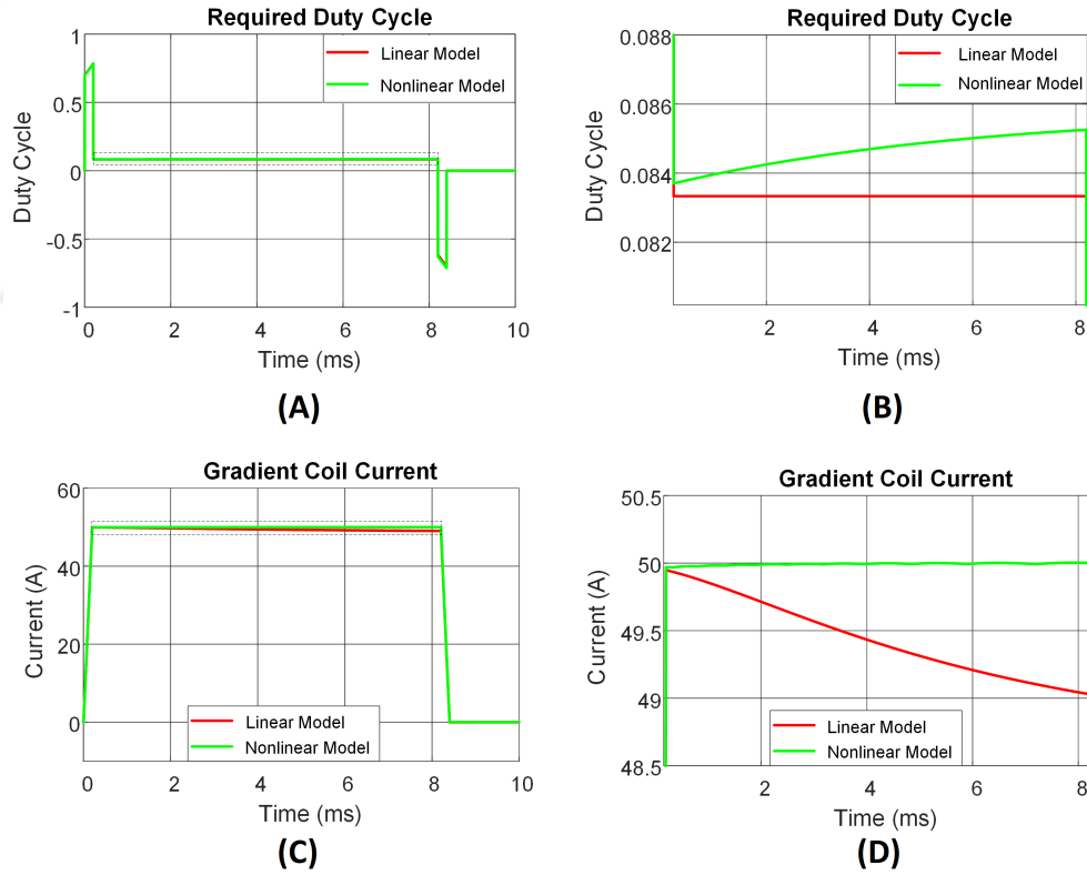
Figure 3.6: Simulation results: (A) Calculated required duty cycles for linear first-order and nonlinear second-order models. (B) a zoomed-in view of the flat-top region, which clearly shows the difference between the output of linear and nonlinear controllers. (C) The gradient coil's current after applying the duty cycles acquired in (A). It demonstrates that the nonlinear controller compensates for the current droop over the flat top region. (D) a zoomed-in view of C for the flat-top period.
