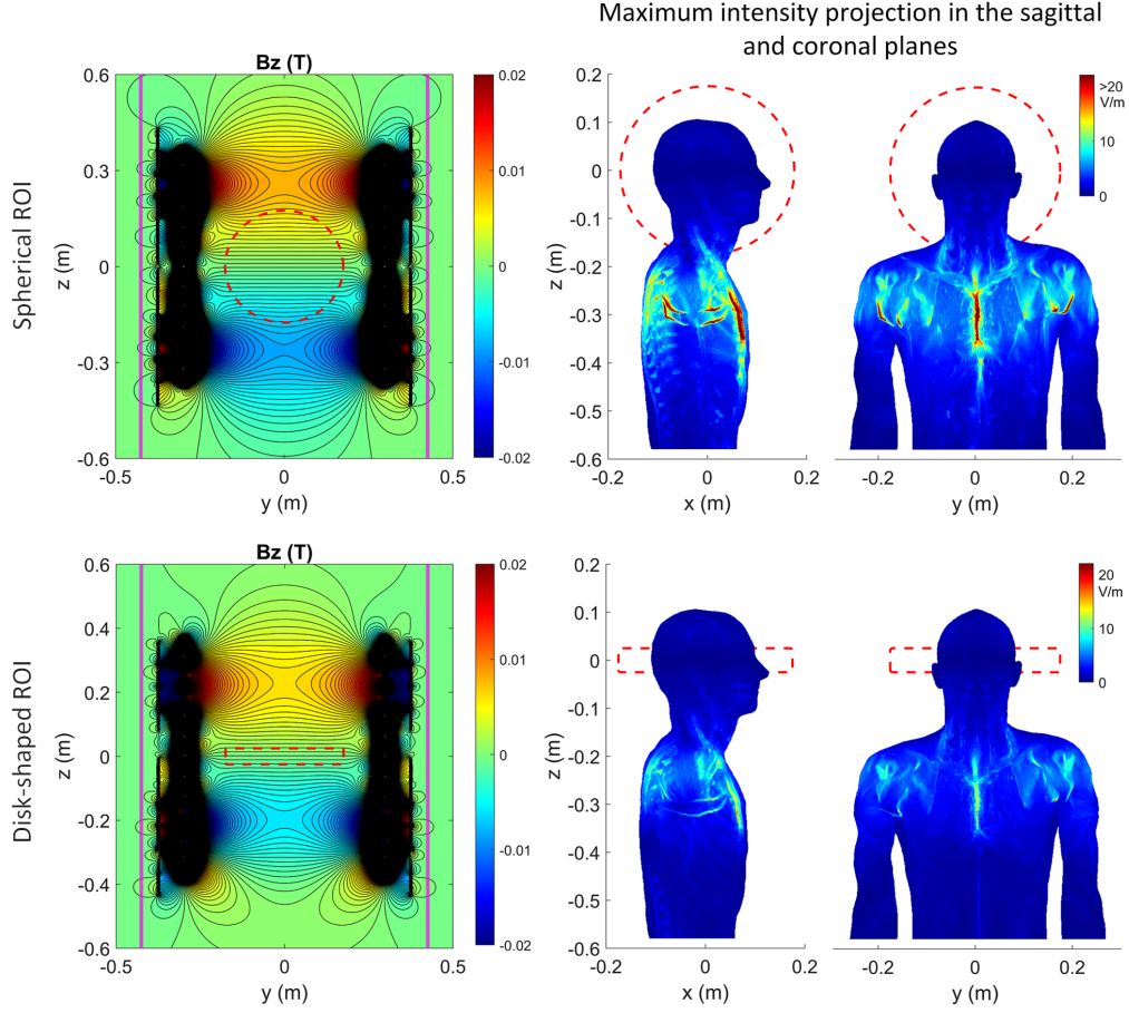
Figure 2.5: Comparison of spherical and disk-shaped ROLs. The linearity error for the spherical ROL is 4.2% and for the disk-shaped ROL is 2.1%. The currents RMS for the spherical and disk-shaped ROLs is 350A and 250A, respectively.
