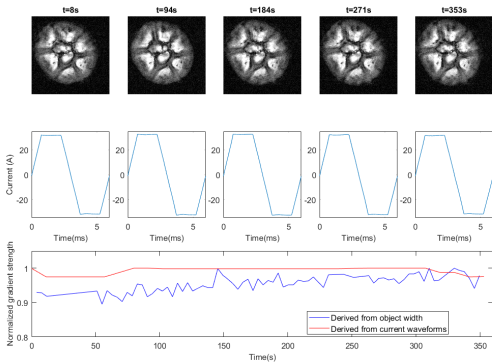
Figure 4.8: MRI experiment results with resistance prediction.
