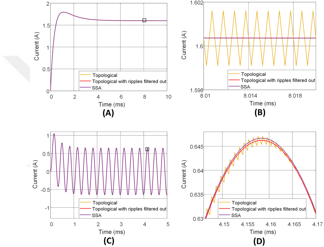
Figure 3.5: Time response comparison of the topological model of gradient system (yellow) and the SSA model (purple). Red curve shows the average of topological model with ripples filtered out. (A) Constant duty cycle, d = 0.5 . (B) Zoomed-view of a small region depicted by a square in panel A. The topological model average is precisely followed by the SSA model (normalized maximum error = 0.0012%). (C) Varying duty cycle (3kHz sinusoidal), and (D) Zoomed-view of the region specified by a square in panel C. Even in this case, varying duty cycle, the SSA gives an excellent approximation of the topological model (normalized maximum error = 0.16%). This error is duty cycle-dependent, and it increases as the duty cycle increases. The frequency of 3kHz (as an example) is used here, which is within the common range of gradient operation frequency.
