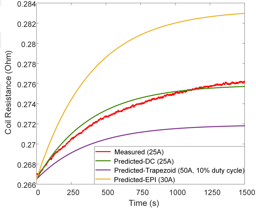
Figure 4.5: The red and green curves show the measured and predicted resistance, respectively. The difference between them is mainly due to the power amplifier heating, which is not considered in the prediction. Applying different current waveforms will result in different predictions; for example, a trapezoid (50A peak amplitude and 10% duty cycle) and EPI ( \pm 30A ).
