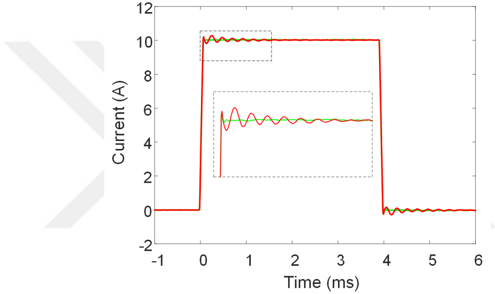
Figure 3.8: Oscillations on the current after switching on/off the gradient coil inside the scanner (the red waveform). These oscillations are removed by using the gradient current transfer function and modifying the input waveform accordingly (the green one).
