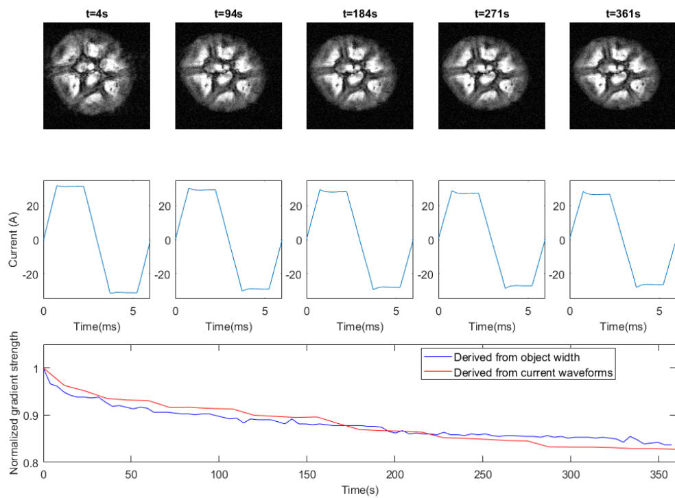
Figure 4.7: MRI experiment results without resistance prediction.
