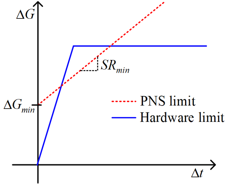
Figure 2.2: PNS and hardware thresholds.
