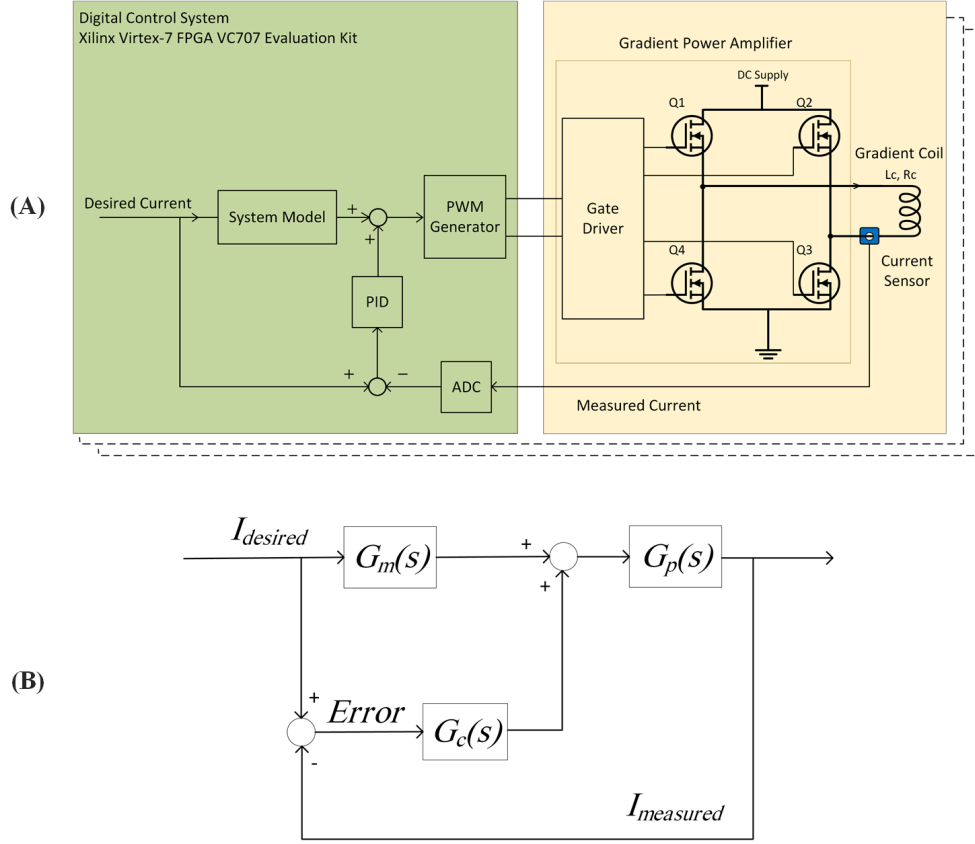
Figure A.1: (A) the schematic of the gradient array system. A combination of feed-forward and feedback provides the desired voltage. Generated PWM signals will amplify and apply to the gradient coil. The analog data coming from the current sensor will be digitized and used in the feedback loop. (B) All the system can be shown by 3 transfer function blocks in the frequency domain. G_p(s) contains all the analog part. G_m(s) and G_c(s) are the model of system and controller transfer functions, respectively.
