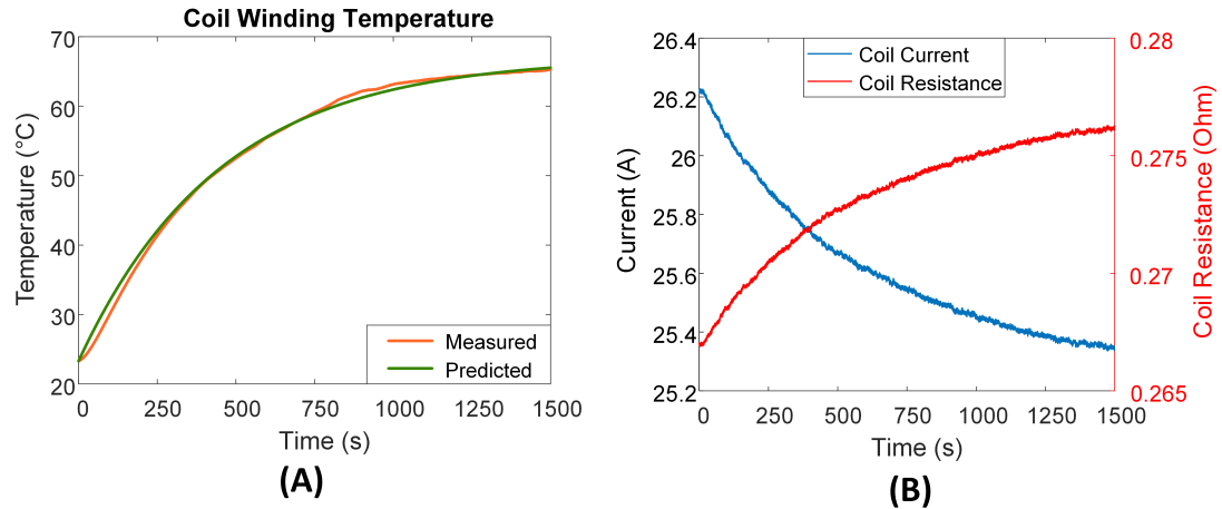
Figure 4.4: Measured and predicted coil temperature are shown in (A), demonstrating the accurate prediction of coil temperature variations using the thermal equation. (B) depicts the coil current and resistance versus time when a constant voltage is applied to the coil, which indicates an exponentially increase in the resistance and consequently decrease in the current.
