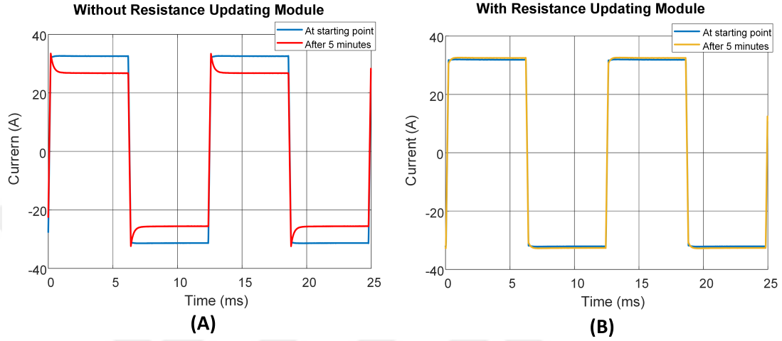
Figure 4.6: A 5-minute EPI waveform was applied to the coil, and the currents were captured at the start and end of the period. (A) show the currents without updating the coil resistance in the model, which results in a 17% reduction in the current amplitude after 5 minutes. Adding the updating feature will compensate for the reduction and provide the desired waveform during the operation period (B).
