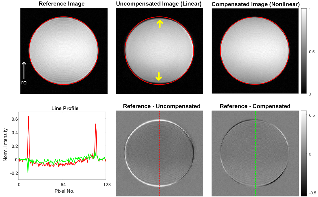
Figure 3.9: Phantom images acquired in the coronal plane using the GRE pulse sequence (single slice). The uncompensated and compensated images are taken by applying the currents provided with the linear and nonlinear models, respectively, as a readout gradient (in z direction, indicated by white arrow). The droop in the readout gradient when using the linear model results in image deformation (shrinking) indicated by yellow arrows. The normalized error images and the line profiles show a significant improvement in the image quality for the compensated image (acquired using the nonlinear model).
