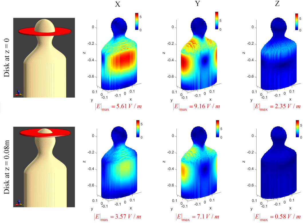
Figure 2.10: E-field plots for all gradients when the linearity is required within a disk in the z-direction (20mm thickness). First row: disk at the iso-center, second row: the disk is shifted in the positive z direction.
