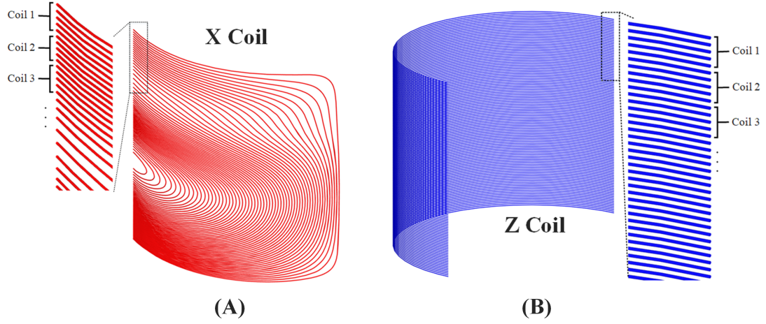
Figure 2.3: (A) Half of the X coil quarter (5 and 3 loops in a bundle for primary and shield, respectively). (B) Half of the Z coil. Both the primary and shield coils consist of 48 bundles with 5 loops per bundle.
