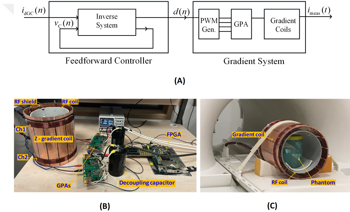
Figure 3.4: (A) The overall gradient chain block diagram, including the feed-forward controller and different components of the gradient system. (B) Benchtop installation, which is located in the equipment room. (C) The imaging setup including gradient coil, RF coil, TR switch, and phantom.
