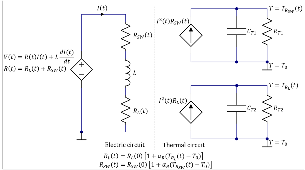
Figure 4.2: The total system model that is separated by the electrical and thermal parts. All temperatures given are effective temperatures stemming from the lumped model.
