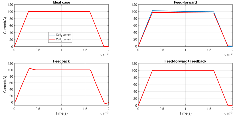
Figure A.2: Simulations: gradient coil current for feed-forward only, feedback only, and feed-forward+feedback controllers.
