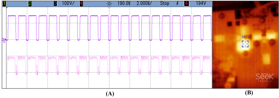
Figure B.3: (A) Measured PWM signals at the input (bottom) and output (top) of the H-bridge with 150V supply without load at 1MHz effective switching frequency. (B) Temperature increase of GaN transistors to 38°C from room temperature for about five minutes of operation condition in (A).
