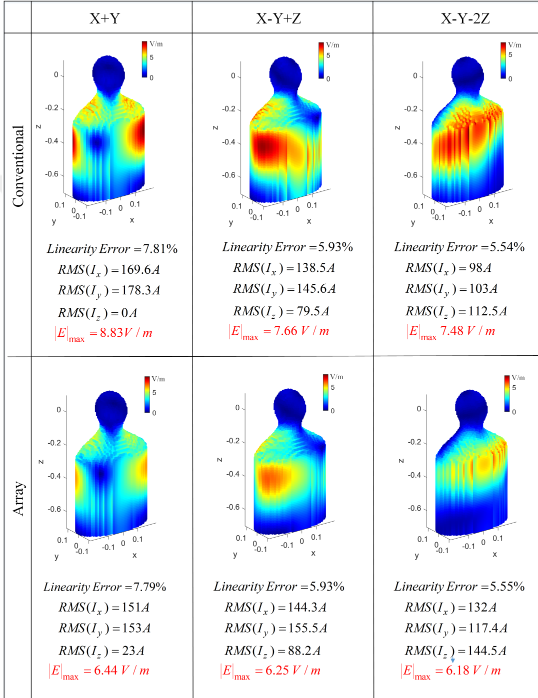
Figure 2.11: Off-center oblique slice: the slice is chosen in X+Y axis (at 0.1m distance from the center with 40mm thickness), the other two can be used as phase encoding or readout direction. For the slice selection gradient there is a 36% increase in PNS thresholds. For the X-Y+Z and X-Y-2Z axes, PNS thresholds are increased by 22% and 21%, respectively.
