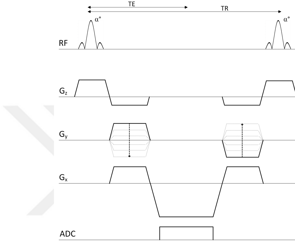
Figure 3.1: Pulse sequence diagram balanced steady state free precession (bSSFP) sequence.
