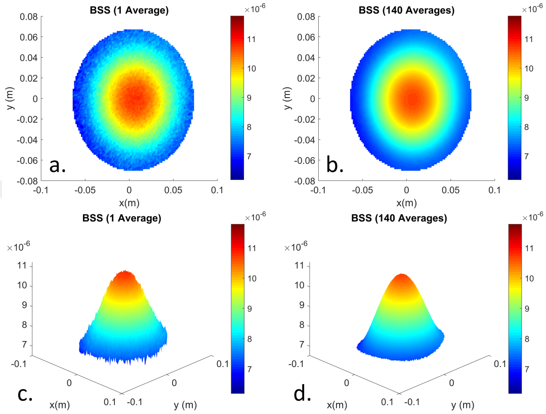
Figure 4.6: Experimental B_1 maps are taken by using Bloch-Siegert shift based method. (a) B_1 map without any averaging, (b) B_1 map with 140 averages, (c,d) are the same as (a,b) and they are drawn as 3D surface plot.
