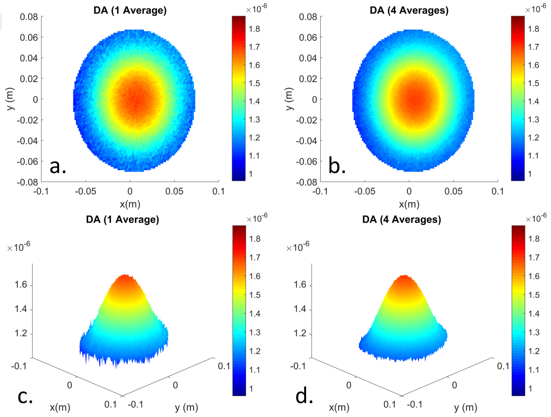
Figure 4.4: Experimental B_1 maps are taken by using double angle method. (a) B_1 map without any averaging, (b) B_1 map with 4 averages, (c,d) are the same as (a,b) and they are drawn as 3D surface plot.
