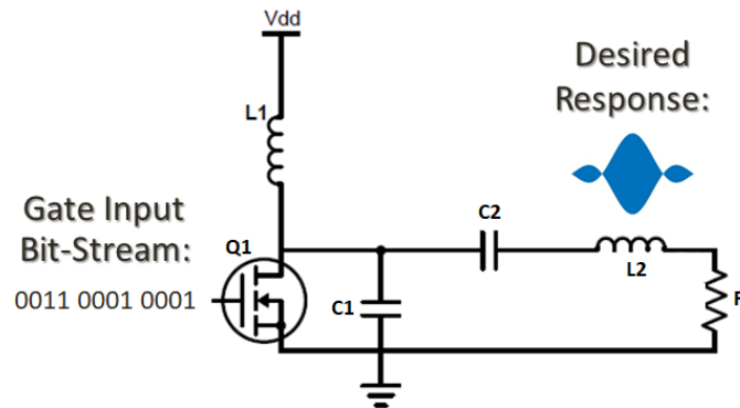
Fig. 2.4 – The gate modulation concept illustrated. By removing the supply modulation block, and by controlling the digital input of the gate of the amplifier, it is aimed to achieve both the amplitude and frequency modulation of the output waveform.
