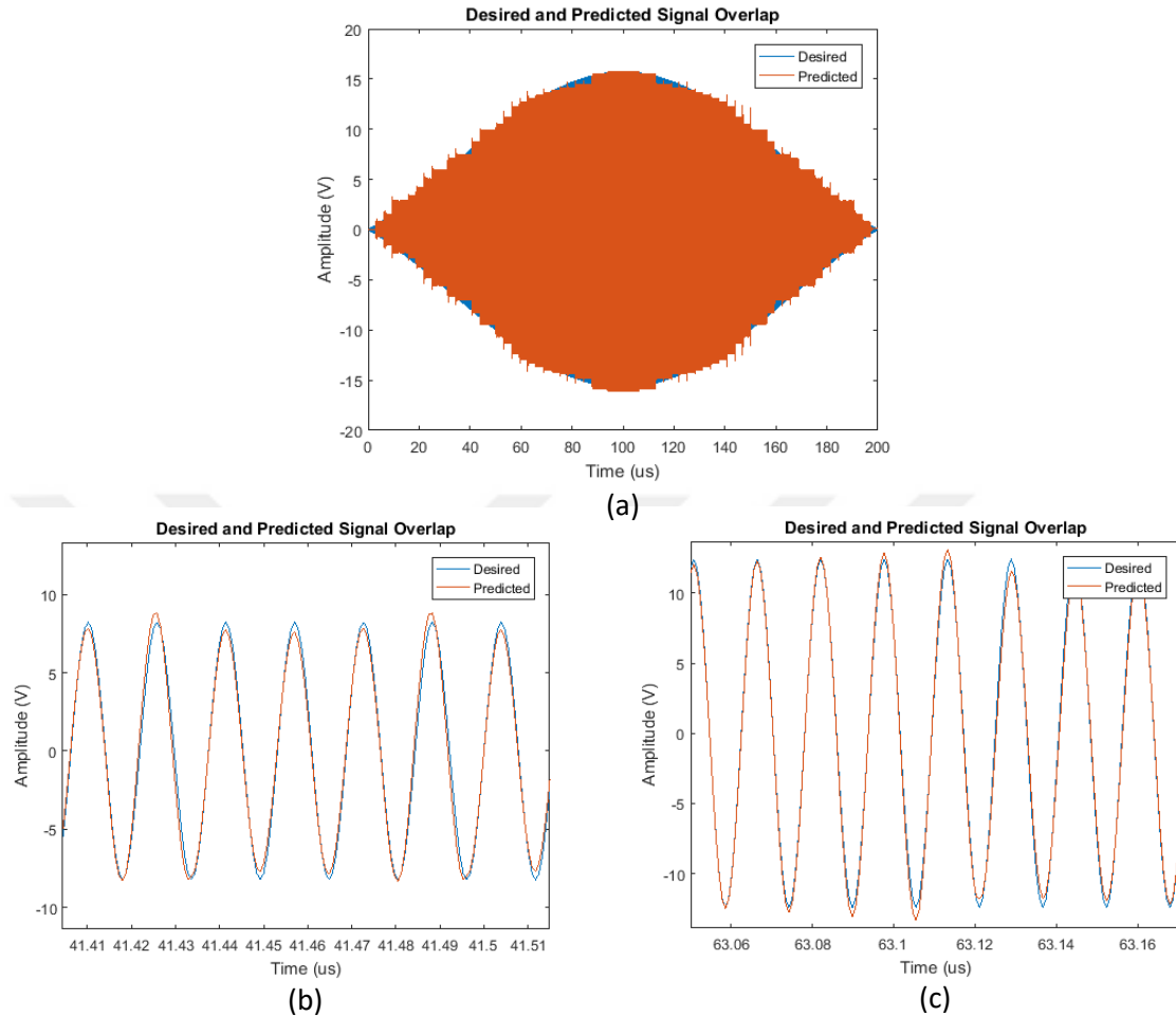
Fig. 4.11 – (a) The predicted output waveform plotted on top of the desired output waveform for the sinc pulse of duration 200 \mu\text{s} with a subsection duration of 3.125 \mu\text{s} . (b-c) Zoomed-in versions of the same plot for two of the subsections.
