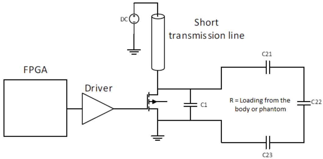
Fig. 2.2 – Modified class-E amplifier design. The RF choke inductor had been replaced with an equivalent transmission line. The transmit coil was designed such that it served as the load network of the amplifier as well. The driver and FPGA blocks are also shown. [2]
