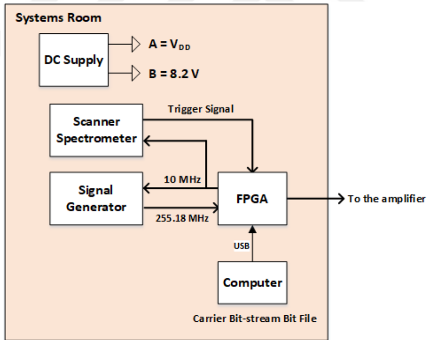
Fig. 3.16 – The updated setup in the systems room. A 10 MHz signal is generated by the FPGA and is fed to the signal generator and the scanner spectrometer for synchronization
