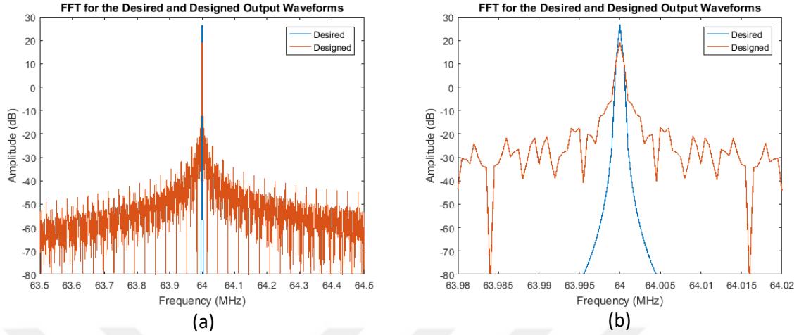
Fig. 4.14 – The overlapped FFT plots of the desired and predicted output waveforms. (a) The FFT plots in 1 MHz bandwidth show no harmonic peaks. (b) The zoomed-in version is shown. The FFT plots of the desired and designed output waveforms show 26.4 dB and 19 dB amplitude respectively at the center frequency (64 MHz).
