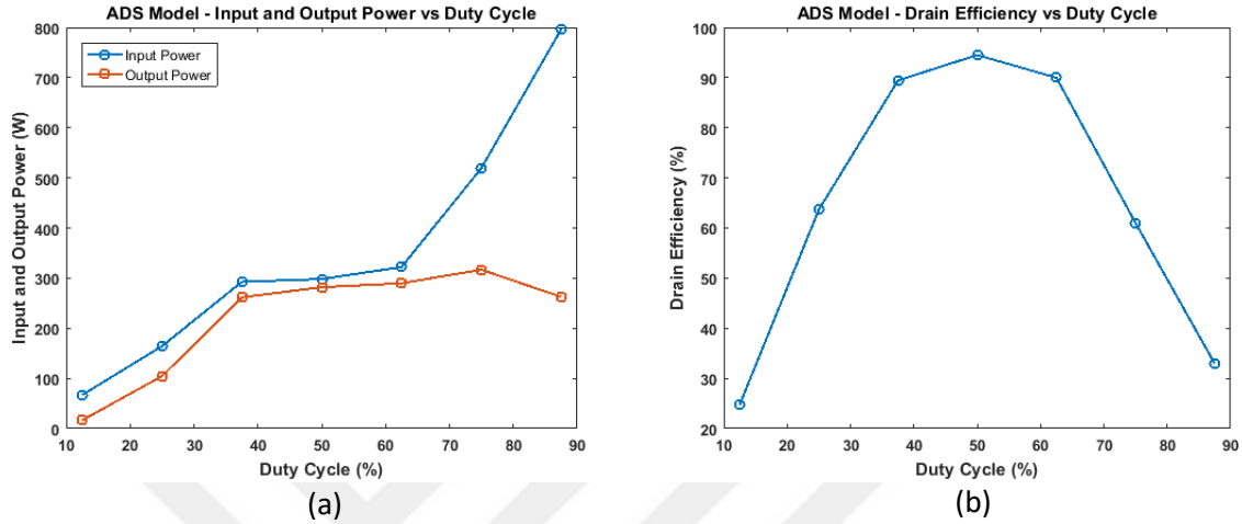
Fig. 4.5 – a) Input and output power vs. the duty cycle of the gate input signal for the ADS model of the class-E amplifier. b) Associated drain efficiency vs. the duty cycle.
