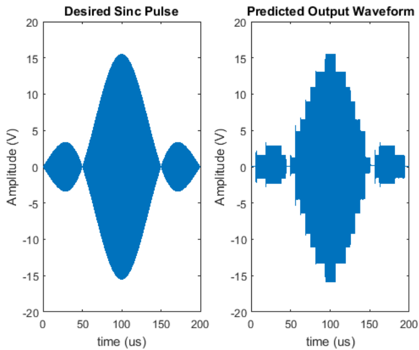
Fig. 4.7 – The desired (left) and predicted (right) output waveforms for the sinc pulse of duration 200 \mu\text{s} with a subsection duration of 6.25 \mu\text{s} .
