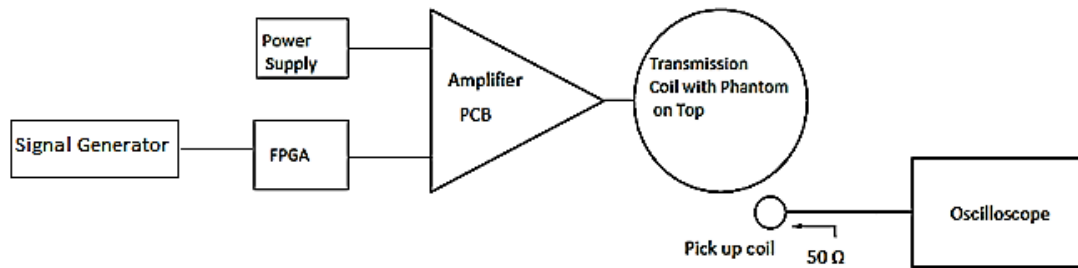
Fig. 3.9 – The block diagram of the experimental setup for bench-top experiments [3].
