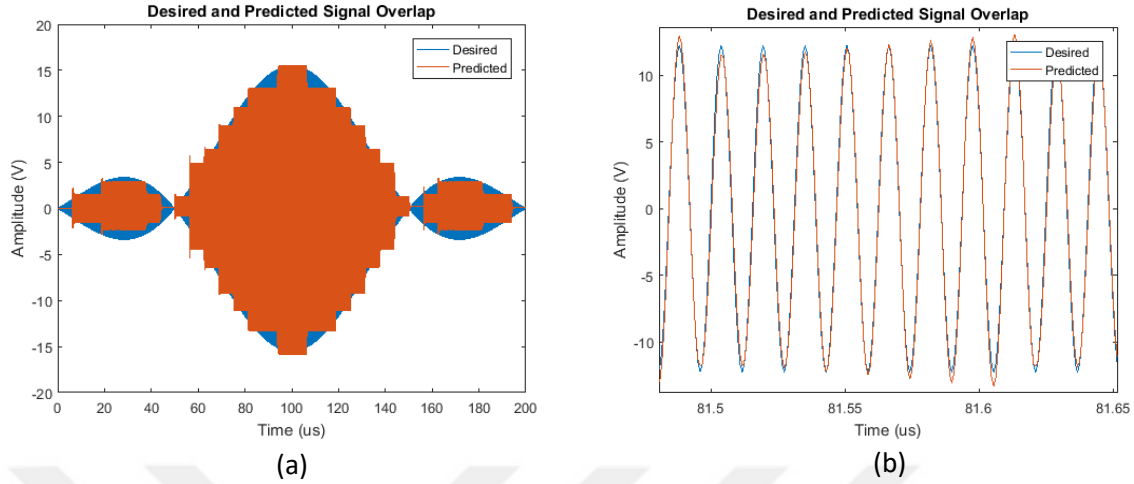
Fig. 4.8 – (a) The predicted output waveform plotted on top of the desired output waveform for the sinc pulse of duration 200 \mu\text{s} with a subsection duration of 6.25 \mu\text{s} . (b) Zoomed-in version of the same plot for one of the subsections.
