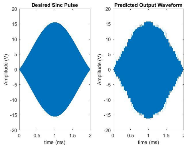
Fig. 4.13 – The desired (left) and predicted (right) output waveforms for the apodized sinc pulse of duration 2 ms
