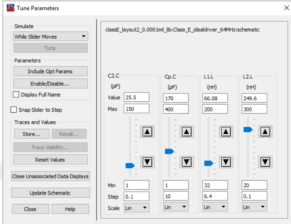
Fig. 3.3 – The load-network tuning environment in the circuit simulator
