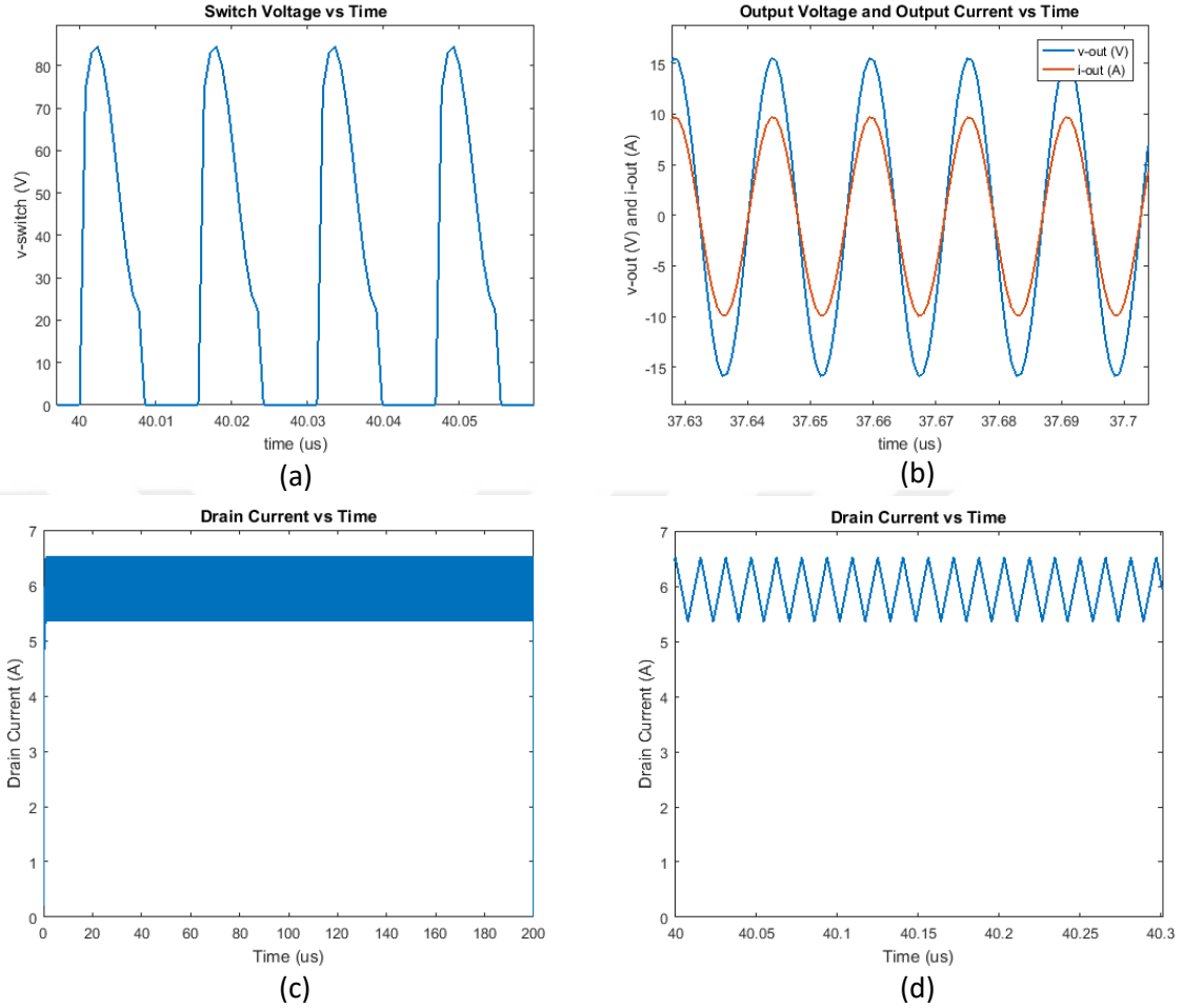
Fig. 4.2 – The amplifier model 2 implementation results. a) Switch voltage vs. time. b) Output voltage and output current vs. time. c) Drain current vs. time (Zoomed-out). d) Zoomed-in version of the drain current vs. time at steady-state.
