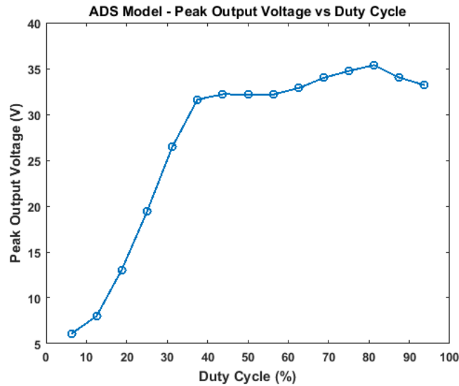
Fig 4.4 – Peak output voltage vs. the duty cycle of the gate input signal for the ADS model of the class-E amplifier
