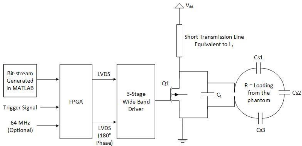
Fig. 3.5 – Block diagram of the hardware implemented to test the designed bit-streams
