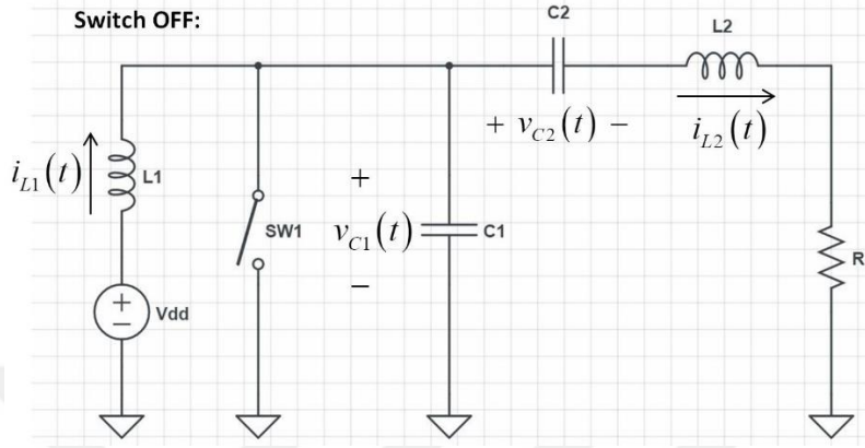
Fig. 2.9 – The schematic diagram for the switch-off case of the amplifier model 2
