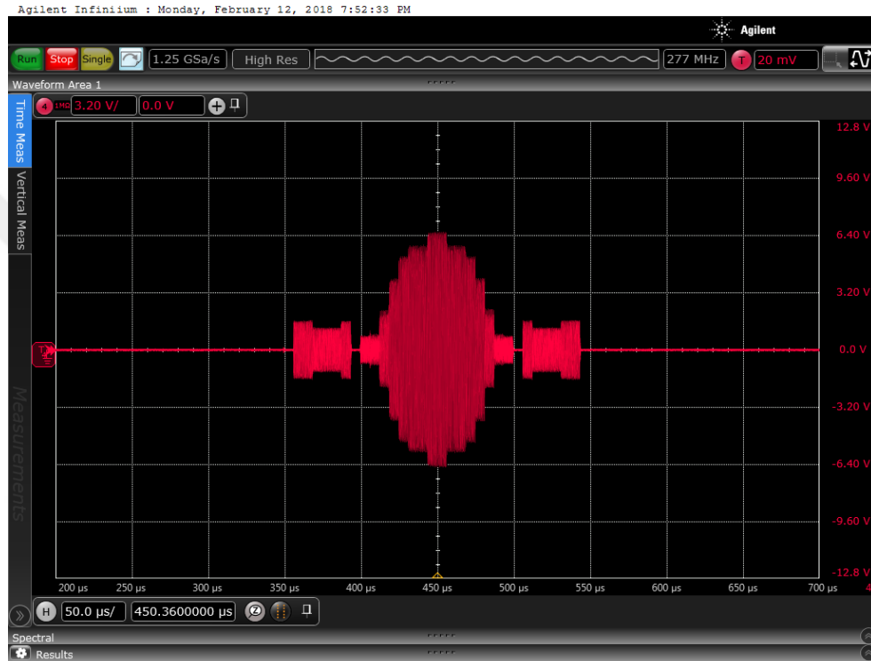
Fig. 4.16 – Gate modulated output waveform of the amplifier when the carrier bit-stream designed for a duration of 200 \mu\text{s} with a subsection duration of 6.25 \mu\text{s} is implemented.
