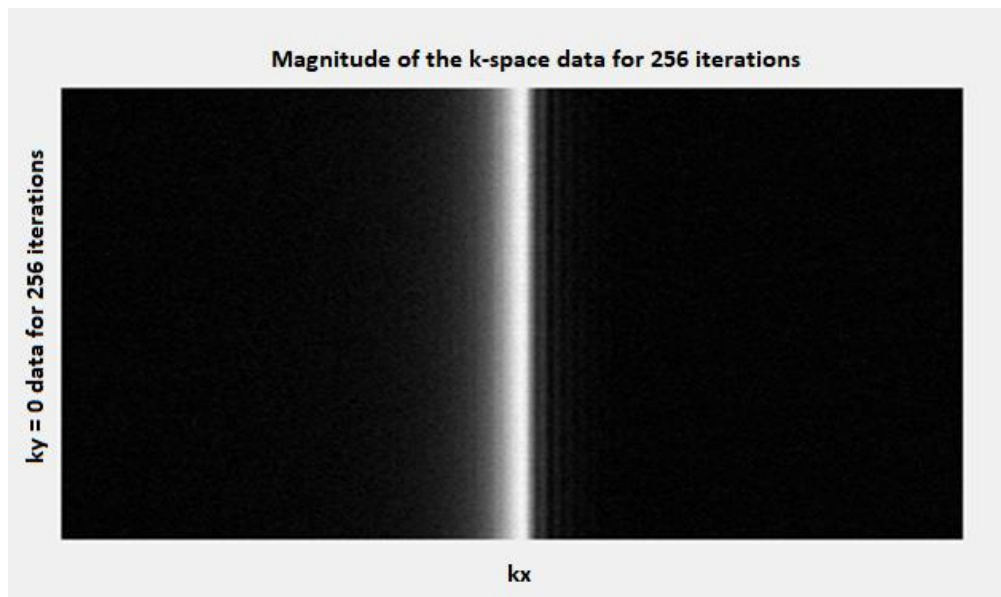
Fig. 3.15 - The k-space magnitude of the data from a single receive channel obtained from the MRI experiment conducted with phase encoding turned off after the implementation errors in the FPGA code were resolved. It can be observed from the diagram that no discontinuities occur in the transmission of the RF pulse.
