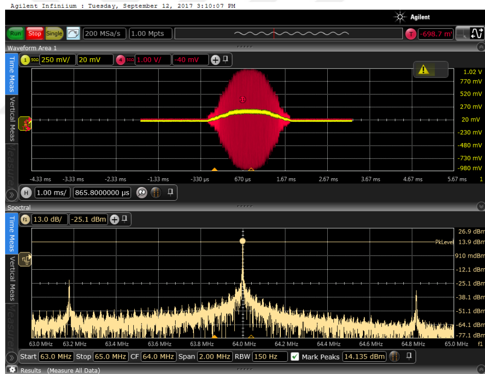
Fig. 4.19 – Gate modulated output waveform of the amplifier (2 ms) and the associated FFT in 2 MHz bandwidth. The FFT shows a 14.135 dBm peak value at the central frequency (64 MHz) with a 10 dB difference in magnitude to the nearest harmonic components under a bandwidth of 2 MHz.
