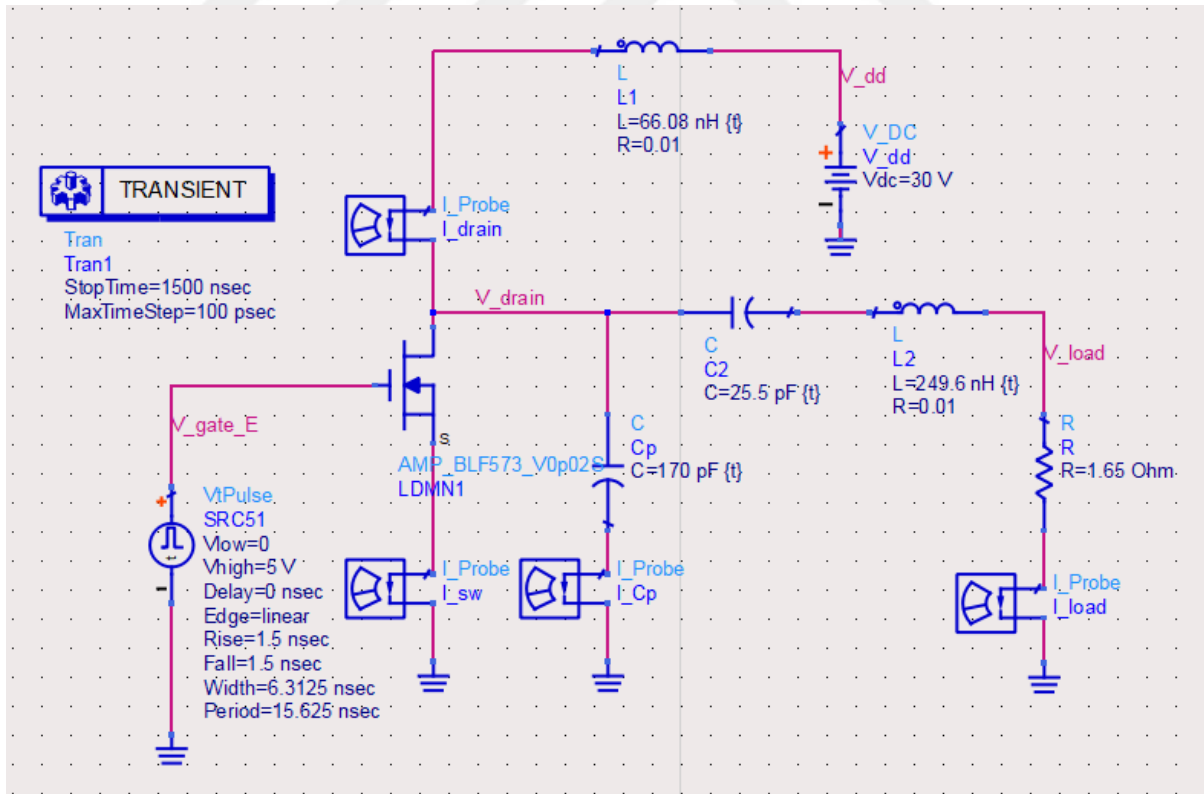
Fig. 3.2 – Schematic diagram of the class-e amplifier model with realistic switch
