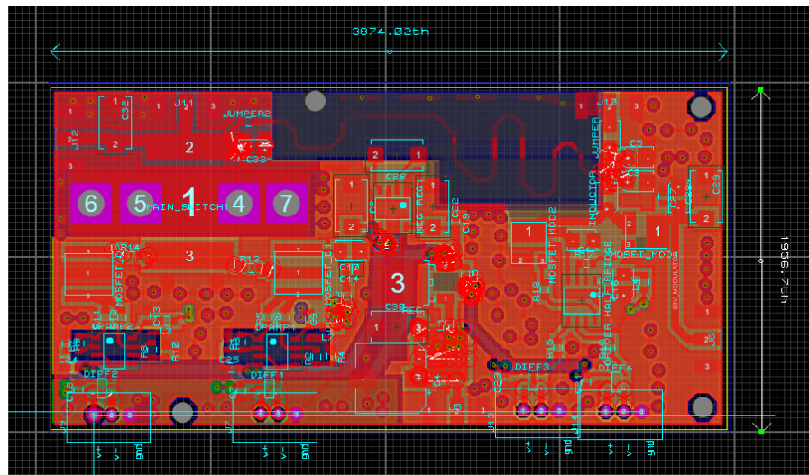
Fig. 3.8 – The design layout of the amplifier PCB including the supply modulation block as well as the integrated micro-strip transmission line (dimensions: 100 mm by 50 mm) [2]
