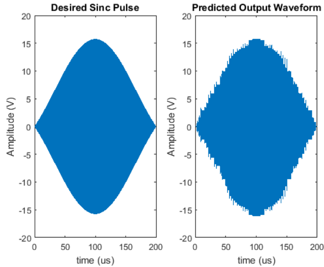
Fig. 4.10 – The desired (left) and predicted (right) output waveforms for the sinc pulse of duration 200 \mu s with a subsection duration of 3.125 \mu s. The spikes observed in the amplitudes of the predicted output waveform (right) correspond to the transient states of each subsection and are minimized based on careful designing of the bit-stream patterns.
