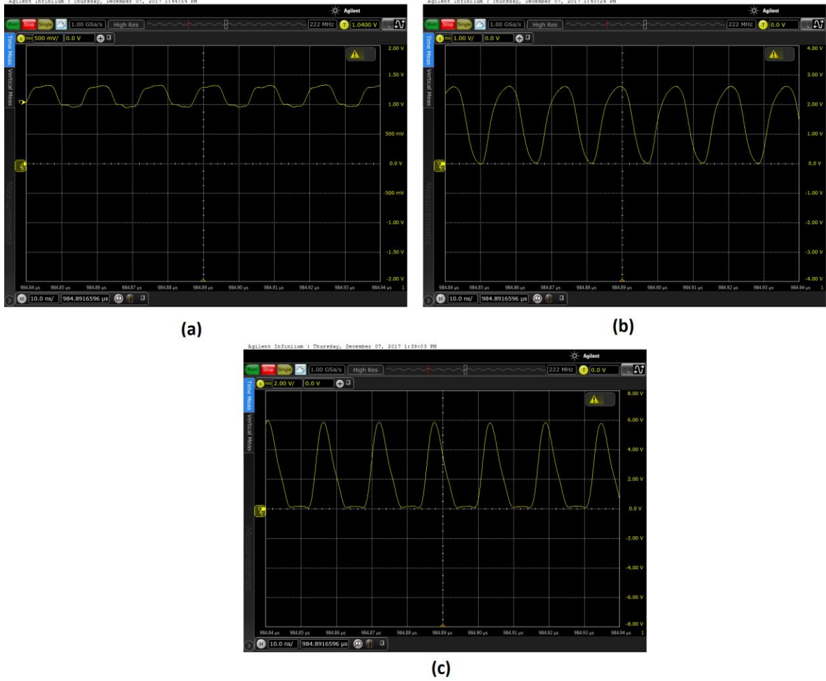
Fig. 4.15 – Hardware implementation results when the amplifier PCB is run with a 50% duty cycle signal at the gate of the amplifier (0011). a) LVDS signals sent by the FPGA to the driver part of the amplifier PCB. b) The signal at the output of the driver part and input to the gate of the amplifier. c) Switch-voltage vs. time. ZVS and ZVDS conditions are satisfied.
