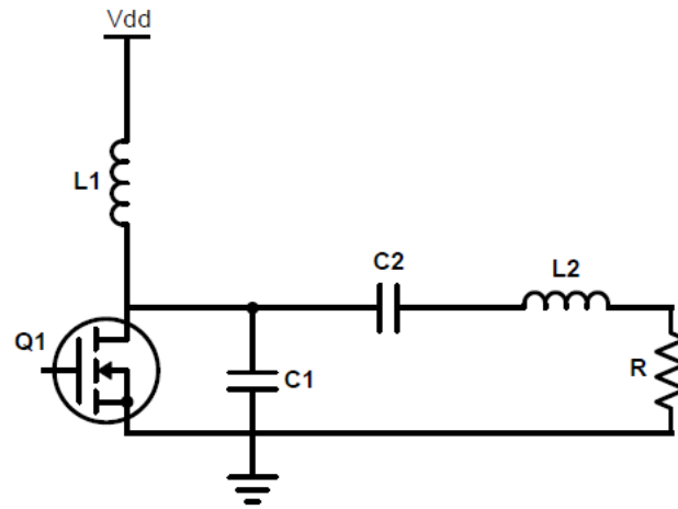
Fig. 2.1 – Conventional class-E amplifier
