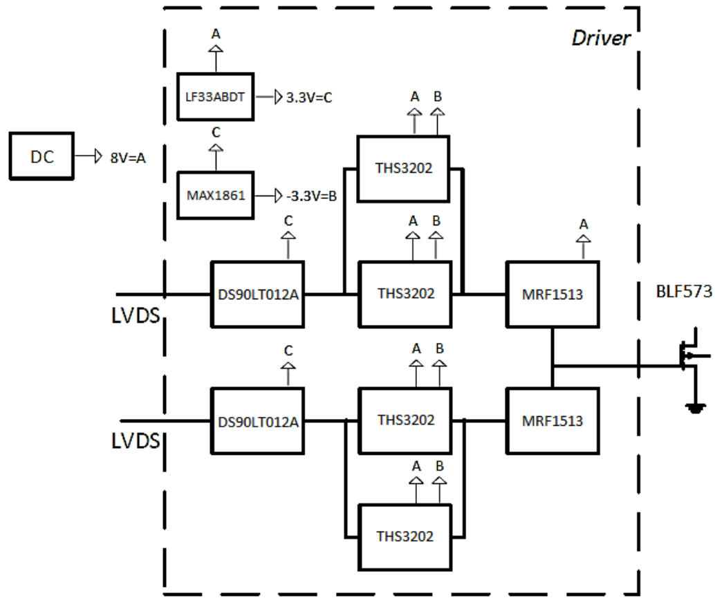
Fig. 3.6 – The block diagram showing different components of the 3-stage driver circuit [2, 3]
