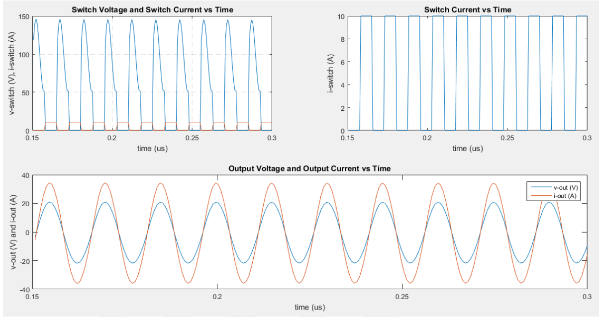
Fig. 4.1 – The amplifier model 1 implementation results. a) Switch voltage and switch current vs. time. b) Switch current vs. time. c) Output voltage and output current vs. time.
