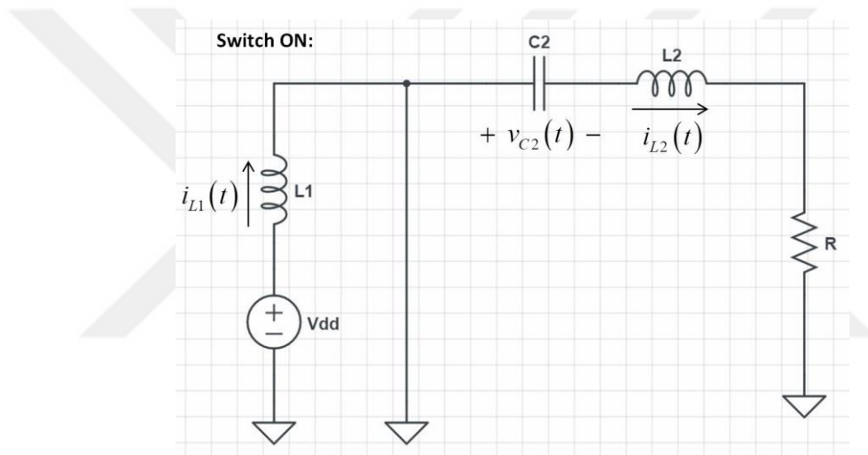
Fig. 2.8 – The schematic diagram for the switch-on case of the amplifier model 2
