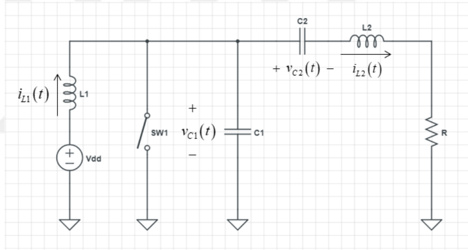
Fig. 2.7 – Amplifier model 2 schematic. The previous ideal constant-current source assumption in model 1 is now replaced by an RF choke inductor assumption at the drain of the amplifier. Again, an ideal, lossless switch is considered in place of the transistor.
