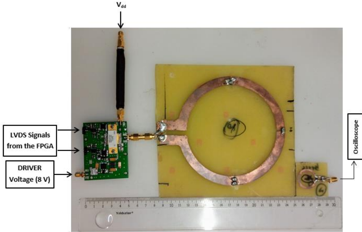
Fig. 3.10 – The hardware setup for bench-top experiments. The FPGA sends the LVDS signals to the amplifier PCB (consisting of the driver and amplifier circuitry). An external transmission line equivalent to RF choke inductor is shown connected at the drain of the amplifier. The output waveform is monitored on the oscilloscope via a 2 cm diameter receiver coil placed near the transmit coil loaded with phantom.
