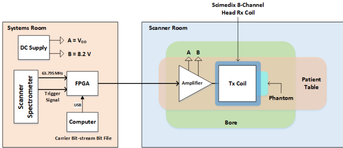
Fig. 3.11 – The block diagram of the experimental setup for MRI experiments
