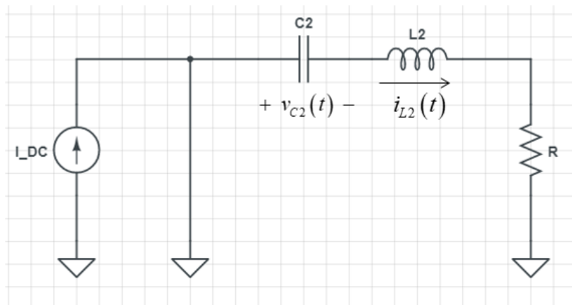
Fig. 2.6 – The schematic diagram for the switch-on case of the amplifier model 1
