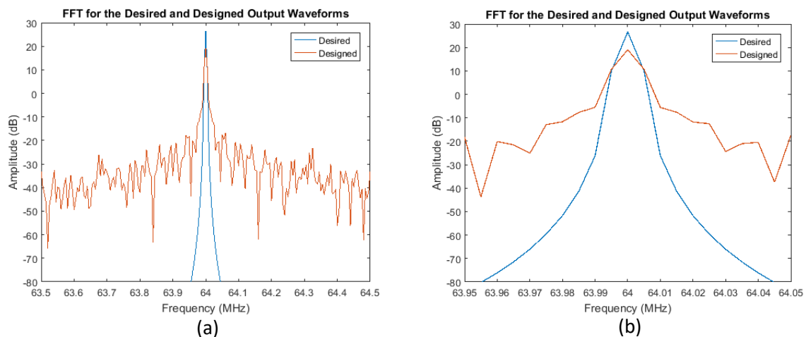
Fig. 4.12 – The overlapped FFT plots of the desired and predicted output waveforms. (a) The FFT plots in 1 MHz bandwidth show no harmonic peaks. (b) The FFT plots in 0.1 MHz bandwidth are shown. The FFT plots of the desired and designed output waveforms show 26.6 dB and 19 dB amplitude respectively at the center frequency (64 MHz).
