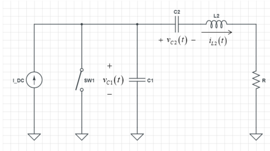
Fig. 2.5 – Amplifier model 1 schematic. An ideal constant-current source is assumed instead of the RF choke inductor at the drain of the amplifier. The transistor is replaced by an ideal switch with zero internal losses.
