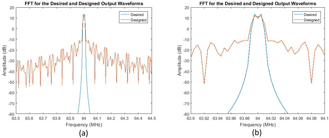
Fig. 4.9 – The overlapped FFT plots of the desired and predicted output waveforms. (a) The FFT plots in 1 MHz bandwidth show no harmonic peaks. (b) The FFT plots in 0.2 MHz bandwidth are shown. The FFT plots of the desired and designed output waveforms show 9.7 dB and 11.2 dB amplitude respectively at the center frequency (64 MHz).
