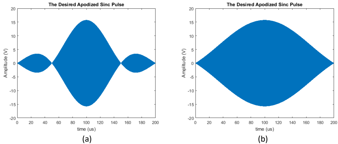
Fig. 3.4 – The desired sinc waveforms each of duration 200 \mu\text{s} . a) The desired sinc waveform with one main lobe and two side lobes. b) The desired sinc waveform with one main lobe.
