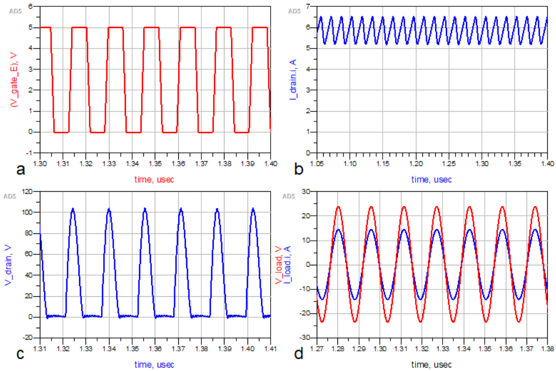
Fig. 4.3 – The circuit simulator implementation results. a) Gate voltage vs. time. b) The drain current vs. time. c) The switch-voltage vs. time. d) The output voltage and output current vs. time.
