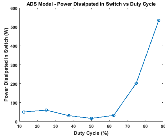
Fig. 4.6 – Power dissipated in the switch vs. the duty cycle of the gate input signal for the ADS model of the class-E amplifier
