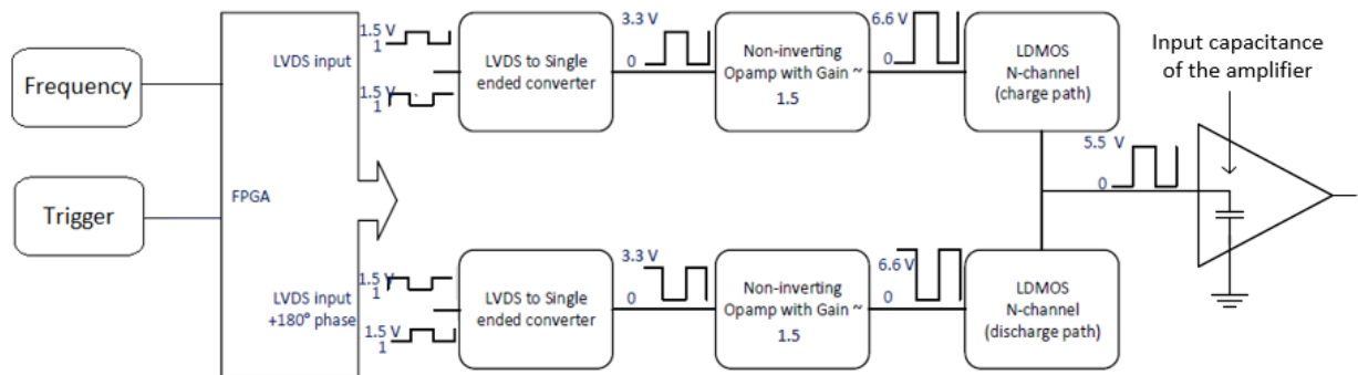
Fig. 2.3 – Three-stage wideband driver design [2, 3]
