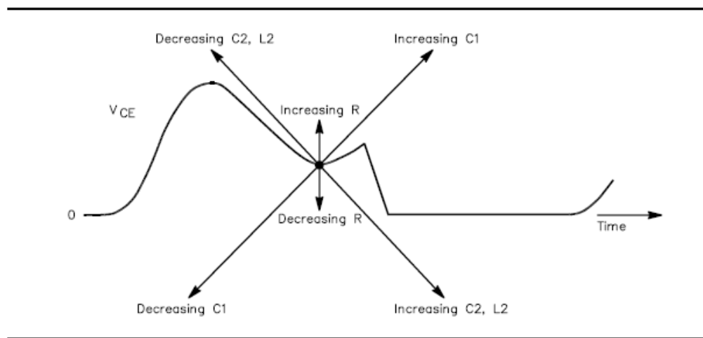
Fig. 3.1 – The effects of adjusting the load network components on the switch-voltage waveform [35]
