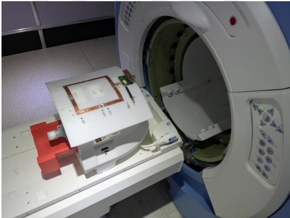
Fig 3.12 – MRI experiment setup: Inside the scanner room – The amplifier PCB was connected to the custom made square-loop transmit coil placed on top of the 8-channel receiver head coil, and the cylindrical phantom placed under the head coil was excited with the custom generated 2 ms sinc pulse while the scanner's transmit system was off.
