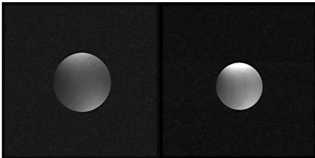
Fig. 4.21 – MR image obtained at 50 W input power (TE/TR = 15ms/200ms) at different FOV (Field of Views) after the phase inconsistencies and synchronization issues have been resolved.
