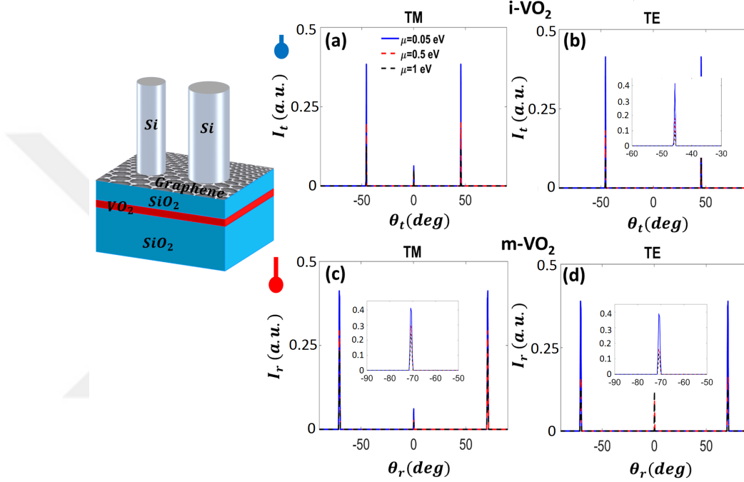
Figure 5.4: Effects of changes in \mu of a single-layer graphene on the normalized far-field intensities of the split beams for the i - VO_2 [(a), (b)] and m - VO_2 cases, and both polarizations. Schematic of the unit cell is illustrated on the left hand side.
