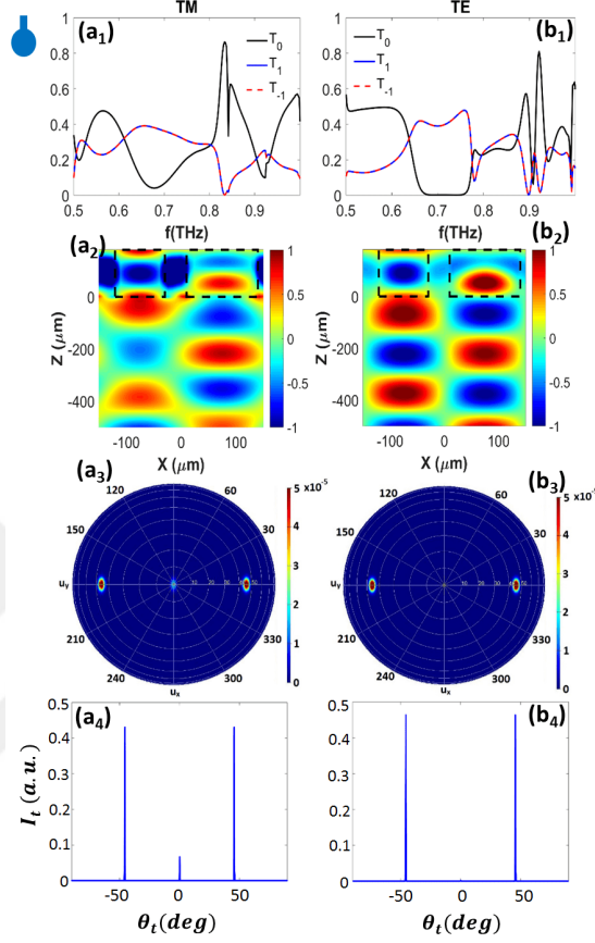
Figure 5.2: Normal incidence transmittive responses of the beam splitter for the i\text{-VO}_2 case. (a 1 ) different orders of light transmission through the metasurface within 0.5 THz to 1 THz. (a 2 ) and (a 3 ) the electric field mode profile and the polar plot of the far-field distribution at 0.7 THz. In agreement with (a 3 ), the normalized far-field intensity of transmitted power is shown in (a 4 ). (b 1 )-(b 4 ) are similar to (a 1 )-(a 4 ) but for TE polarization.
