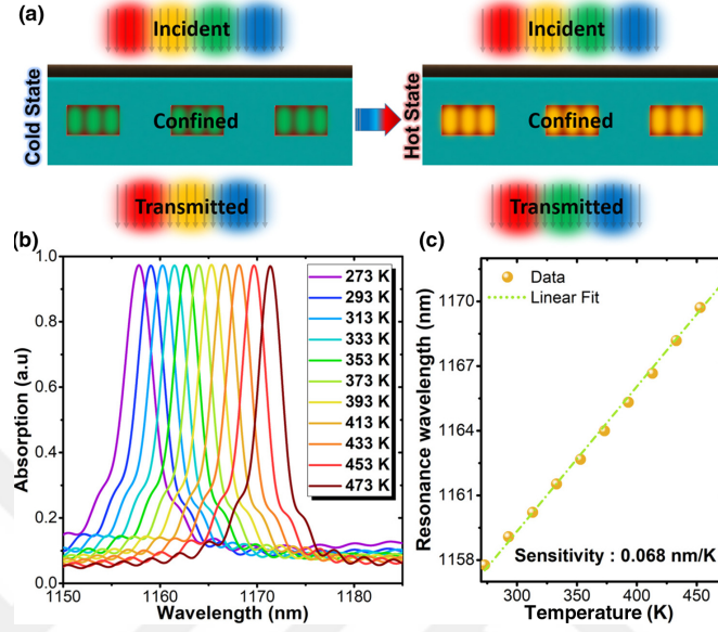
Figure 2.4: (a) Illustration of red shift of the absorption peak as the temperature is increased. (b) Absorption spectrum change with temperature. (c) Resonance wavelengths for different applied temperature values and linear fit in order to find the thermo-optical sensitivity of the proposed device.
