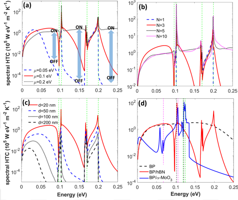
Figure 4.4: SHTC of the BP/hBN parallel-plate structure for different values of (a) \mu(N = 3, d = 20\text{nm}) , (b) N(\mu = 0.1\text{eV}, d = 20\text{nm}) , and (c) d(N = 3, \mu = 0.1\text{eV}) (d) compares the SHTCs of BP, BP/hBN, and BP/ \alpha - \text{MoO}_3 structures for N = 3, \mu = 0.1\text{eV}, d = 20\text{nm} . The vertical dashed lines in (d) are the edges of the RBs of \alpha - \text{MoO}_3 , and the resonances of the SHTC for the BP/ \alpha - \text{MoO}_3 parallel-plates occur at the upper edges; i.e., the ENZ frequencies.
