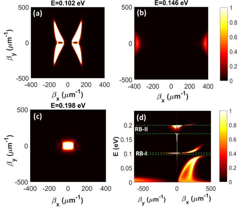
Figure 4.3: Density plots of \xi(\hbar\omega, \beta_x, \beta_y) for hBN-covered BP parallel-plate structure at (a) \hbar\omega = 0.102\text{eV} , (b) \hbar\omega = 0.146\text{eV} , and (c) \hbar\omega = 0.198\text{eV} ; horizontal dashed lines in (d) are the edges of the RBs of hBN; and the high- \xi regions indicate the supported hybrid SPP-HPP modes.
