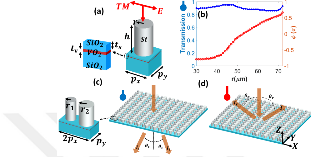
Figure 5.1: (a) Schematic of the metasurface unit cell. (b) i-VO 2 radius dependence of transmission and the phase delay at f = 0.7 \text{ THz} . (c) and (d) illustrate schematic and different operations of the metasurface with the split angle \theta_i and intensity I_i ( i = t, r ) for the i-VO 2 and m-VO 2 cases, respectively. The binary unit cell is also illustrated in panel (c).
