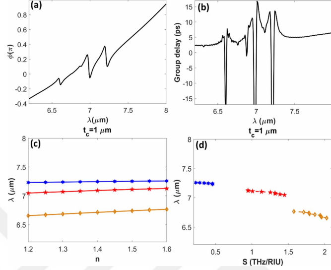
Figure 3.3: Slow-light and sensing features of the hBN-based metasurface for the i-VO 2 case. (a) Phase of transmitted light through the metasurface and the corresponding group delay that is shown in panel (b). (c) Dependence of the resonance frequencies, the three deeps in transmission in figure 2(a) (i.e. \lambda_0 , \lambda_1 and \lambda_3 ), versus changes in the refractive index of the covering medium with thickness of 1 \mu\text{m} . (d) The corresponding sensitivity of the structure for the resonances investigated in panel (c).
