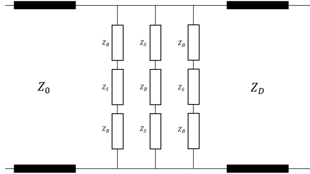
Figure 1.14: Circuit model of a two different conductive sheet combined
