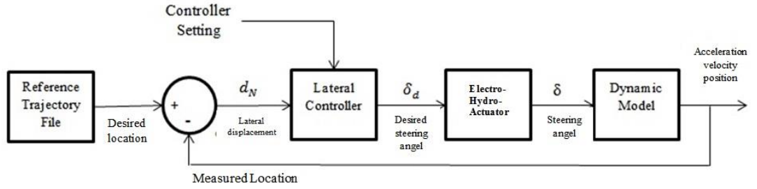
Figure 2.4: Block diagram of the auto-steering test-bed
