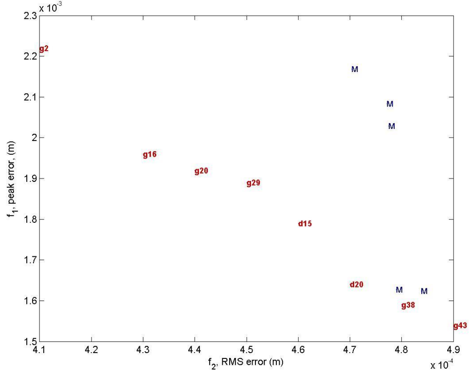
Figure 4.4: Pareto-front obtained by weighted sum DE method where each solution is marked by 100\alpha
