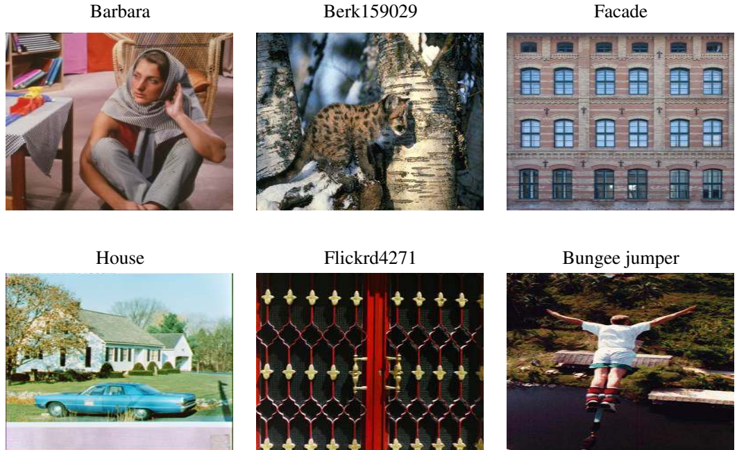
Figure 3.2: Test images.
