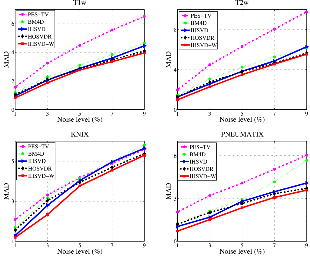
Figure 4.8: MAD comparison on synthetic data under Rician noise of various levels [Numerical results are tabulated in Appendix H].
