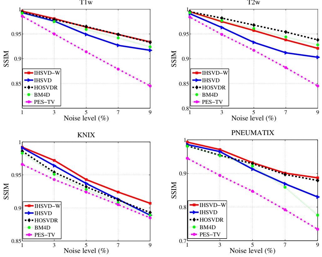
Figure 4.7: SSIM comparison on synthetic data under Rician noise of various levels [Numerical results are tabulated in Appendix H].
