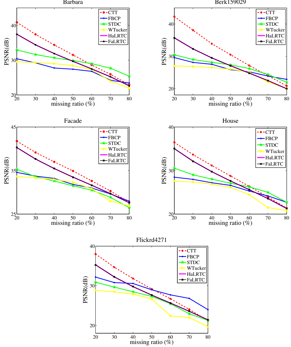
Figure 3.3: PSNR (dB) comparison of different algorithms on five color images at various missing ratios.
